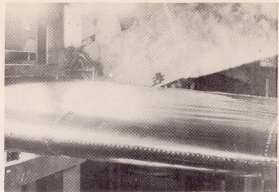
Figure 9.- Bottom surface of wing under half-limit load of condition III with zero pressure, showing tension wrinkles.
