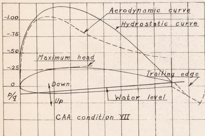
Figure 8. — Hydrostatic and approximate aerodynamic normal pressure curves for top surface (inverted) airfoil section at panel center.
