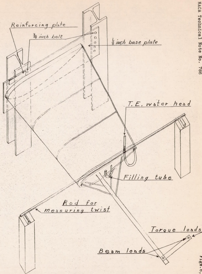
Figure 6. — Arrangement of apparatus for hydrostatic test.
