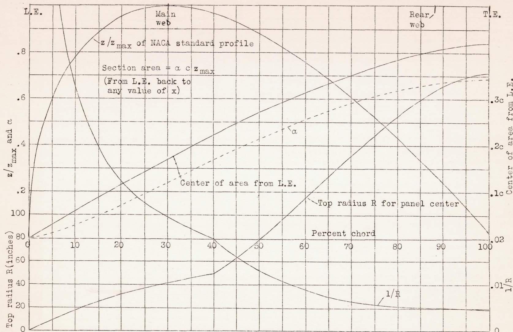
Figure 7.- Geometrical characteristics of wing section.
