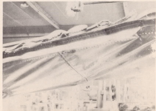
Figure 14.- Top surface of wing after beam failure under a combination of water and shot loading.
