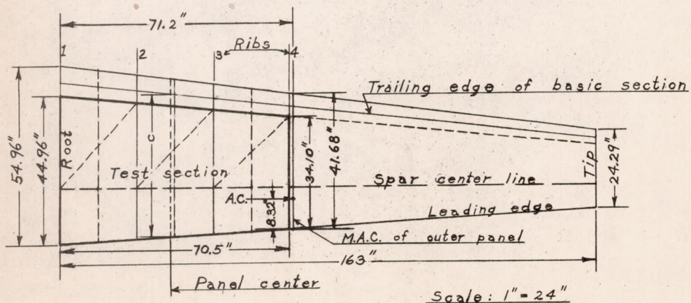
Figure 4. — Plan of outer wing panel. (At panel center, c = basic chord = 44.00 inches.)
