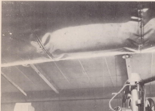
Figure 11.- Top skin bulge under limit load of CAA condition III with zero internal pressure.
