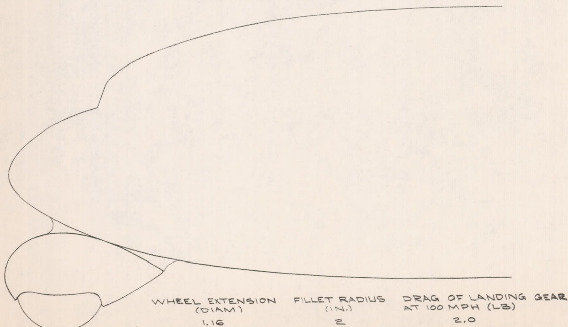
FIGURE 20.- COMPLETE FAIRING I, POSITION B.
