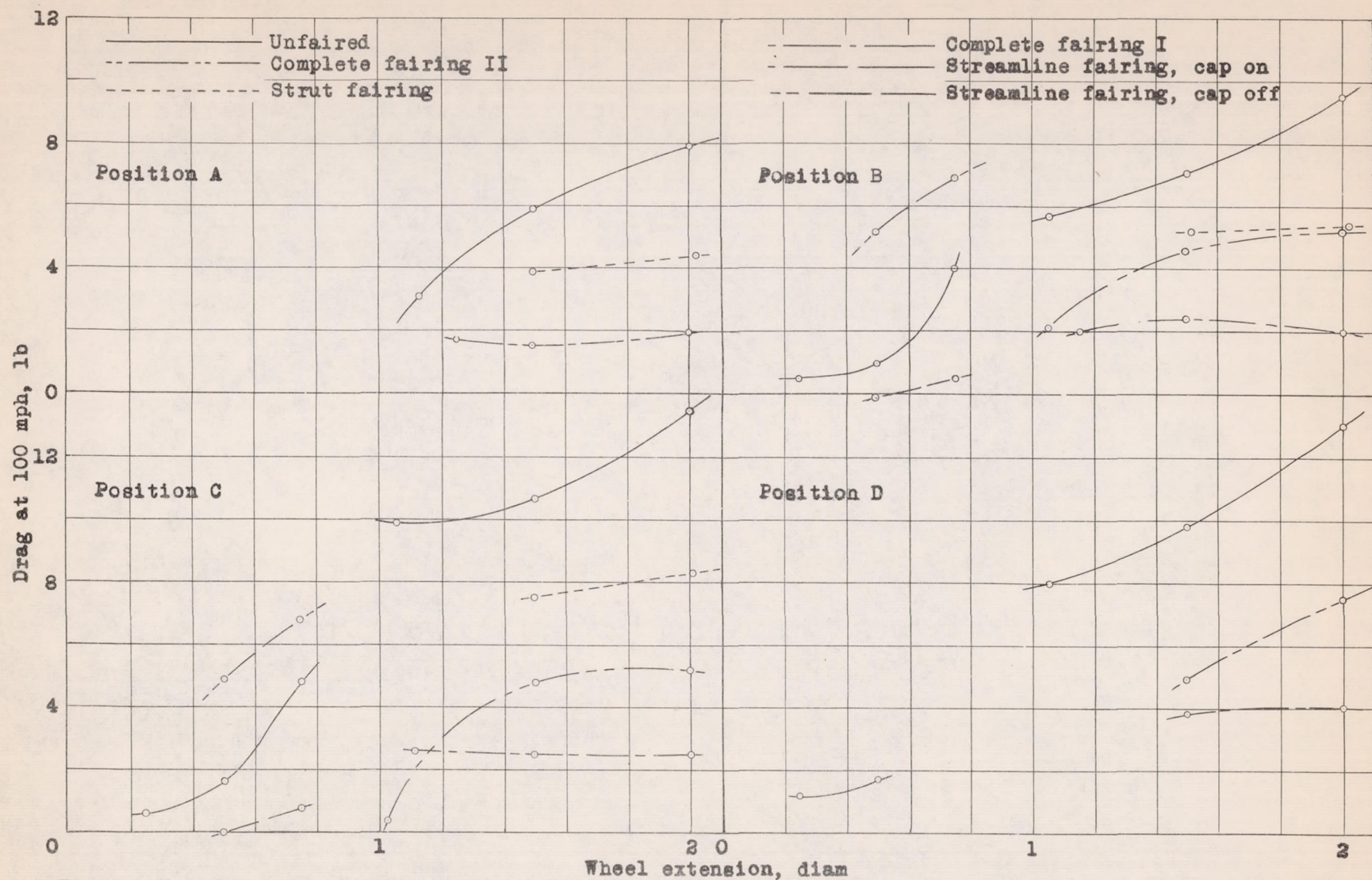
Figure 33.- Relation of wheel extension to drag of landing gear. The wheel opening is open for all partly retracted conditions (all extensions less than 1 diameter) but is closed for all of the others.
