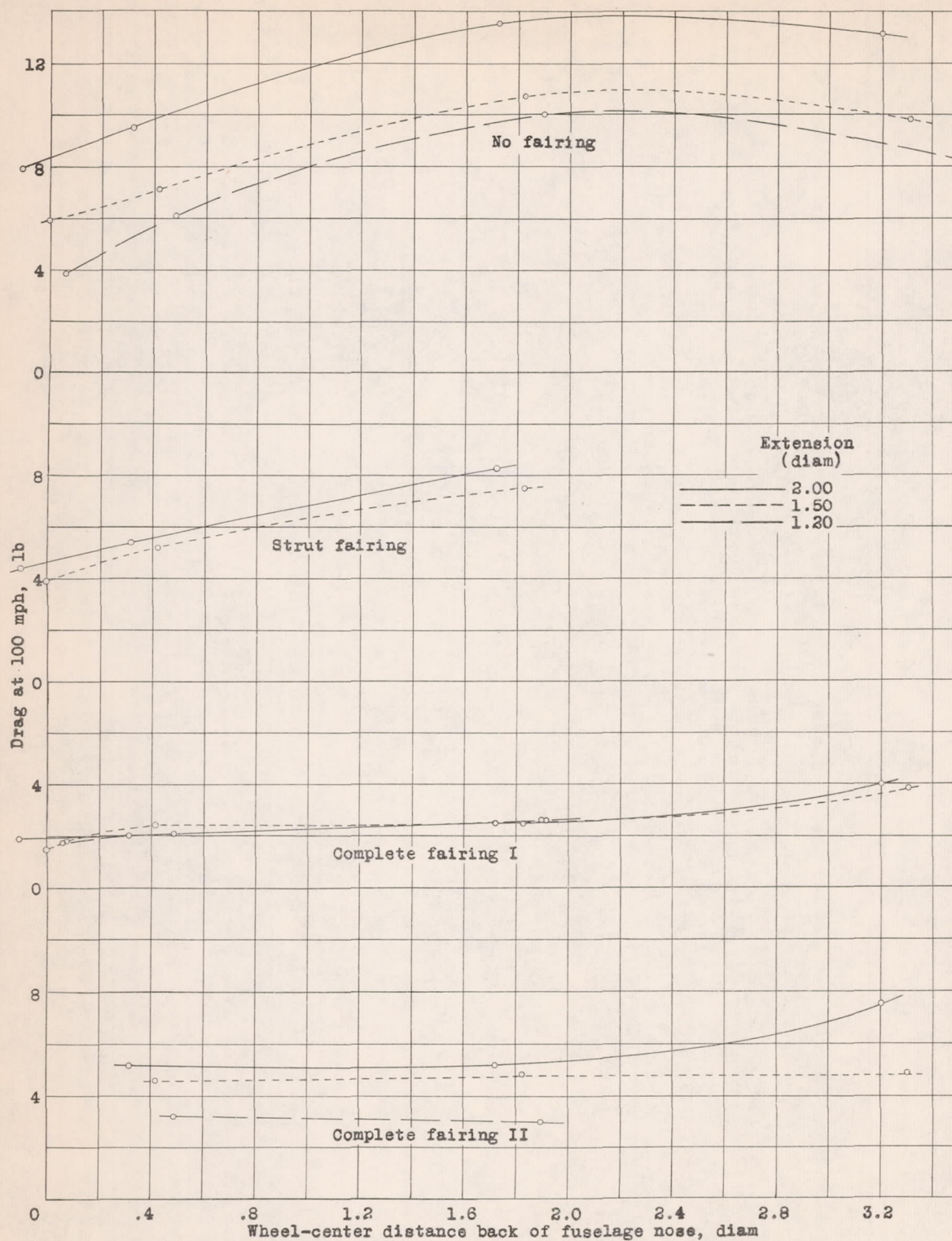
Figure 34.- Relation of drag of nonretracted landing gear to distance back of nose.
