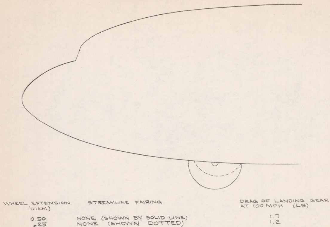
FIGURE 31.- LANDING GEAR PARTLY RETRACTED, POSITION D.
