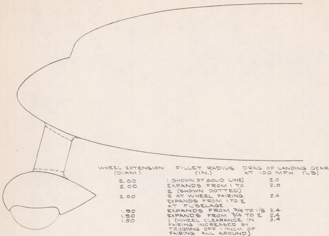
FIGURE 19.- COMPLETE FAIRING I, POSITION B.
