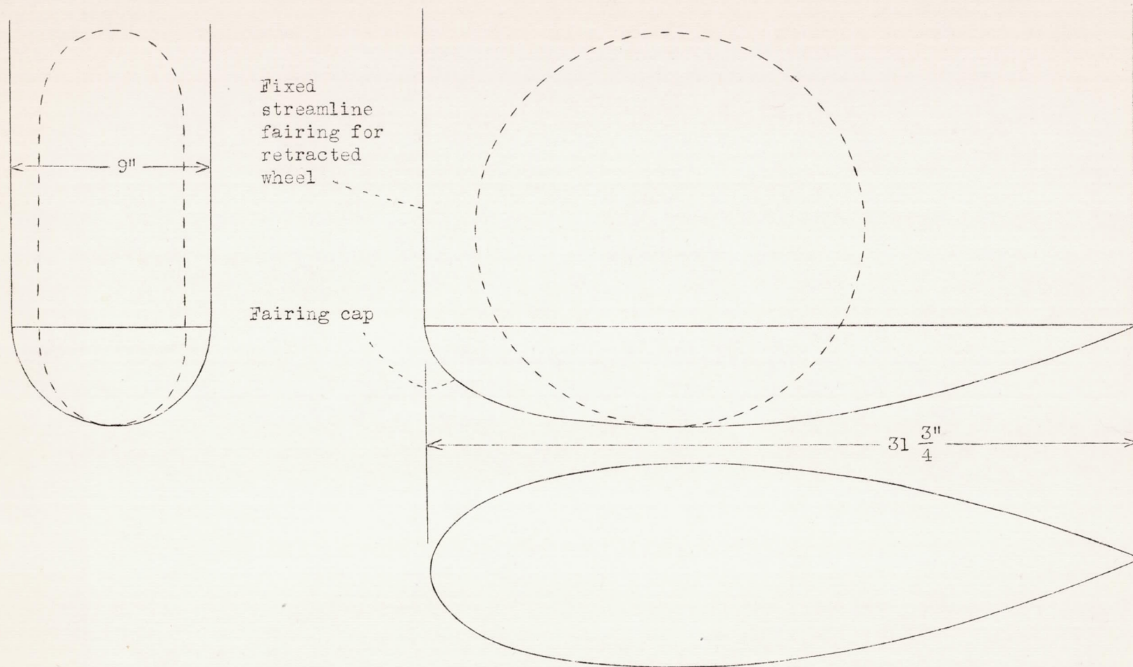
Figure 6.- Fairing for partly retracted landing gear.
