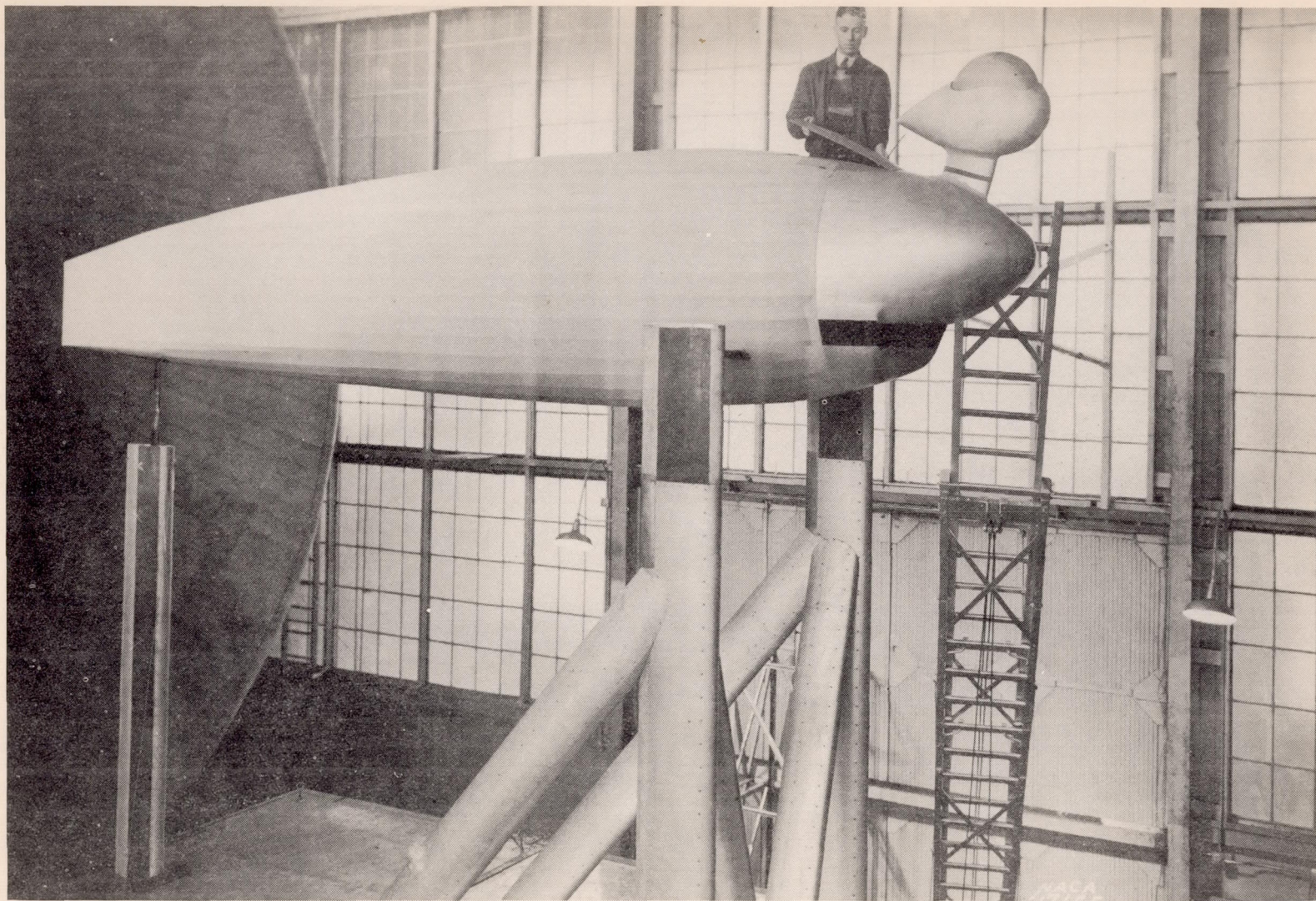
Figure 1. - Fuselage and landing gear with complete fairing I mounted in the 20-foot wind tunnel. Wheel extended 1.5 diameters in position B.
