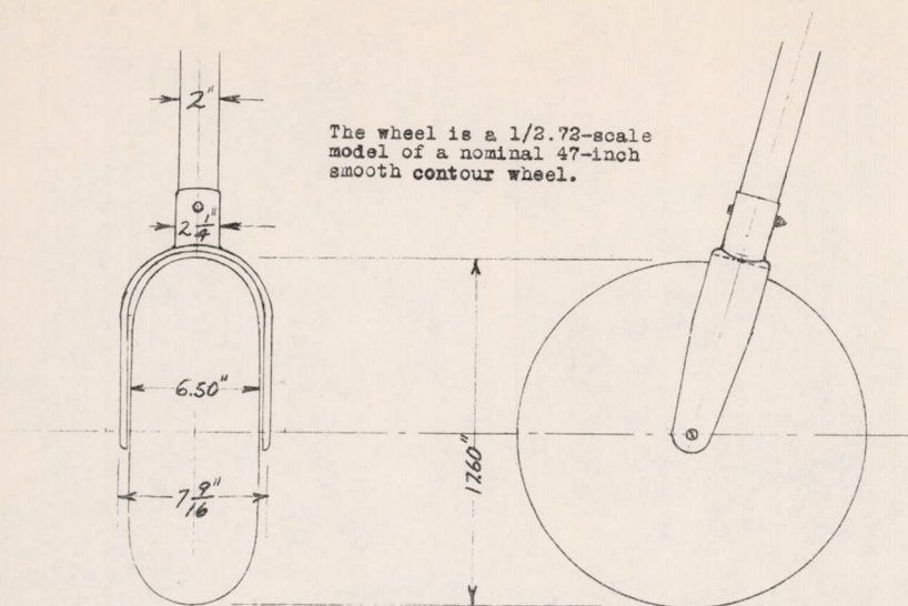
Figure 2.- Unfaired landing gear.
