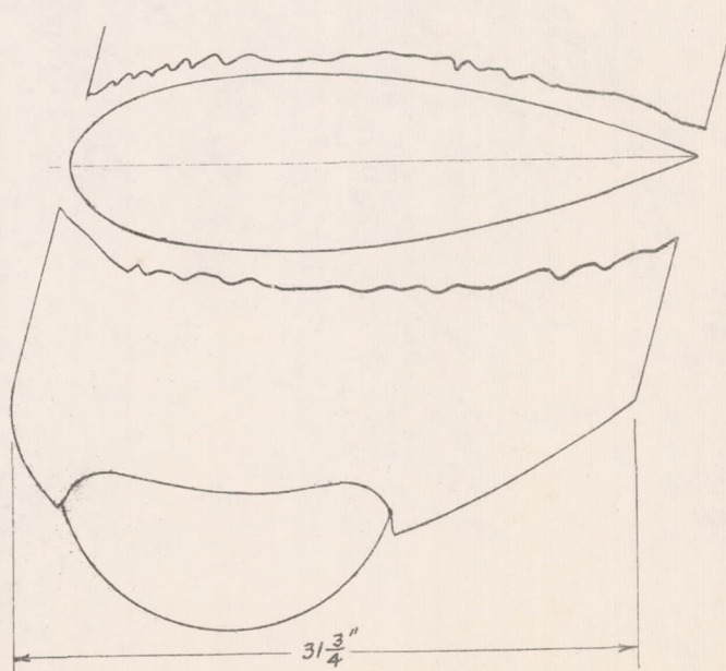
Figure 5.- Landing gear with complete fairing II.
