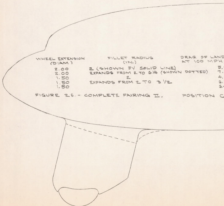
FIGURE 25.-COMPLETE FAIRING II, POSITION B.
