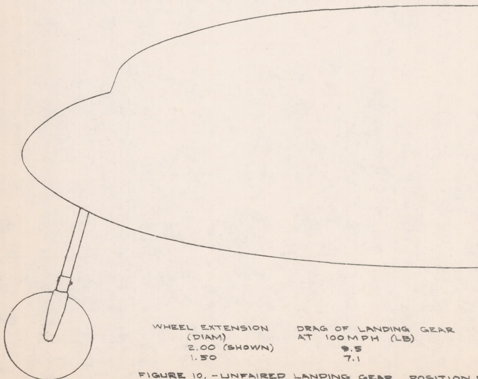
FIGURE 10. - UNFAIRED LANDING GEAR. POSITION B.
