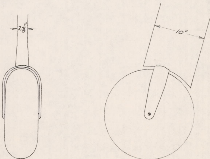
Figure 3.- Landing gear with strut fairing.
