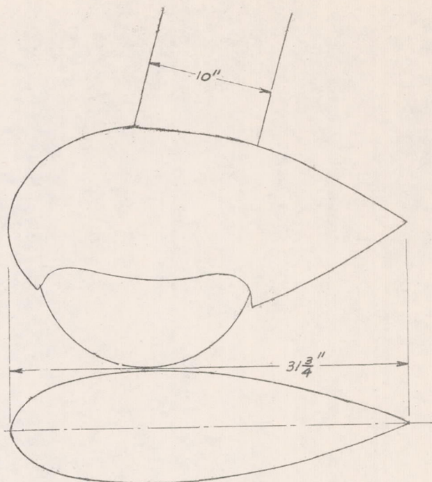
Figure 4.- Landing gear with complete fairing I.
