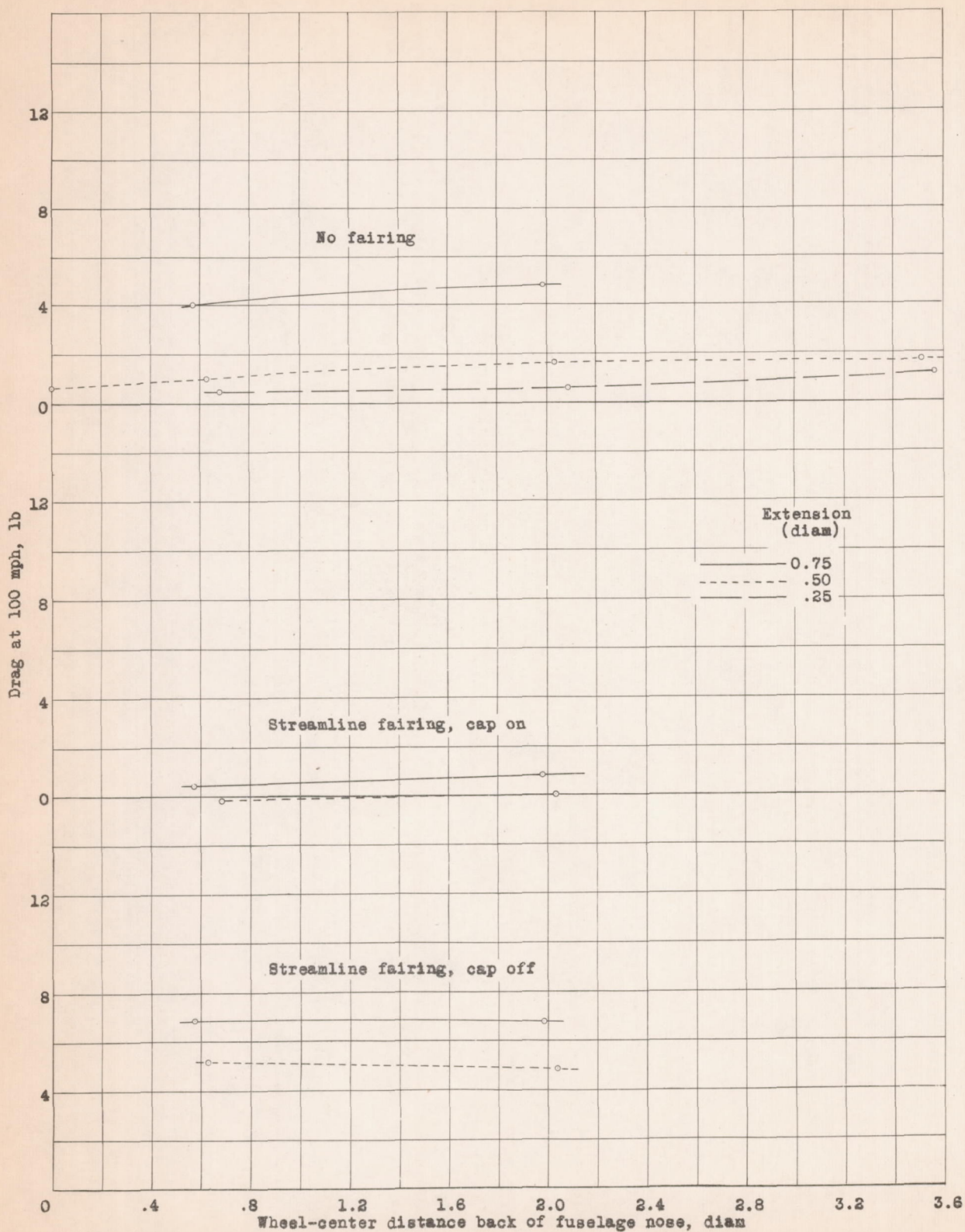
Figure 35.- Relation of drag of partly retracted landing gear to distance back of nose.
