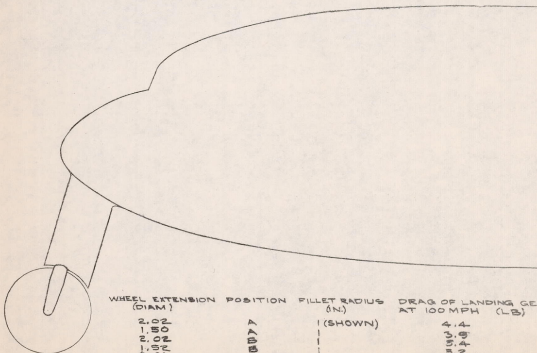
FIGURE 15.- UNFAIRED LANDING GEAR. POSITION D
