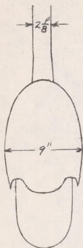
Figure 4.- Landing gear with complete fairing I.
