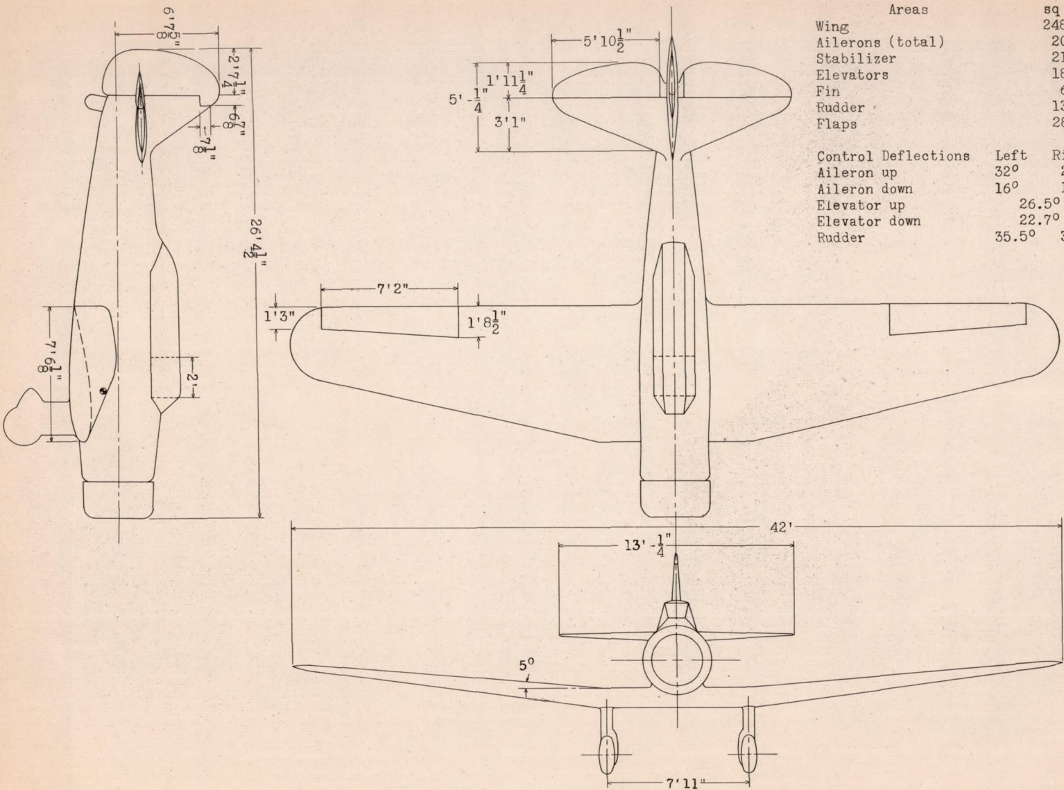
Figure 3.- Three-view drawing of the 1/16 scale model of the airplane. (Dimensions are for full-scale airplane.)
