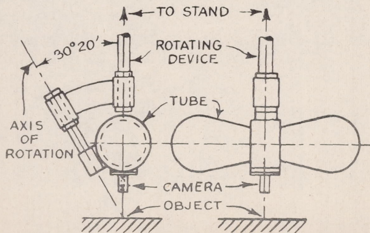
Figure 10.- Arrangement of X-ray tube for stress measurement, (50).
