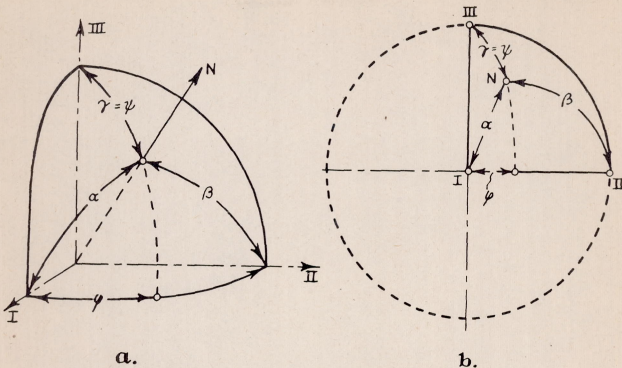
Figure 19.- Direction angles.
