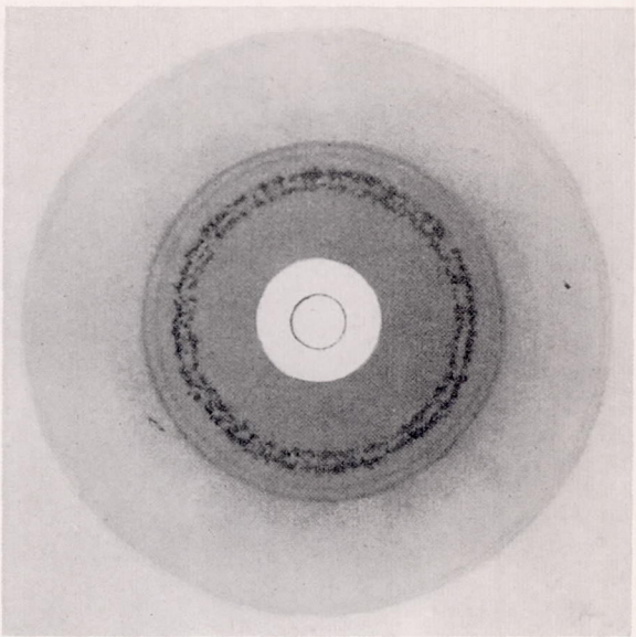
(b) A focusing camera with stationary film.
