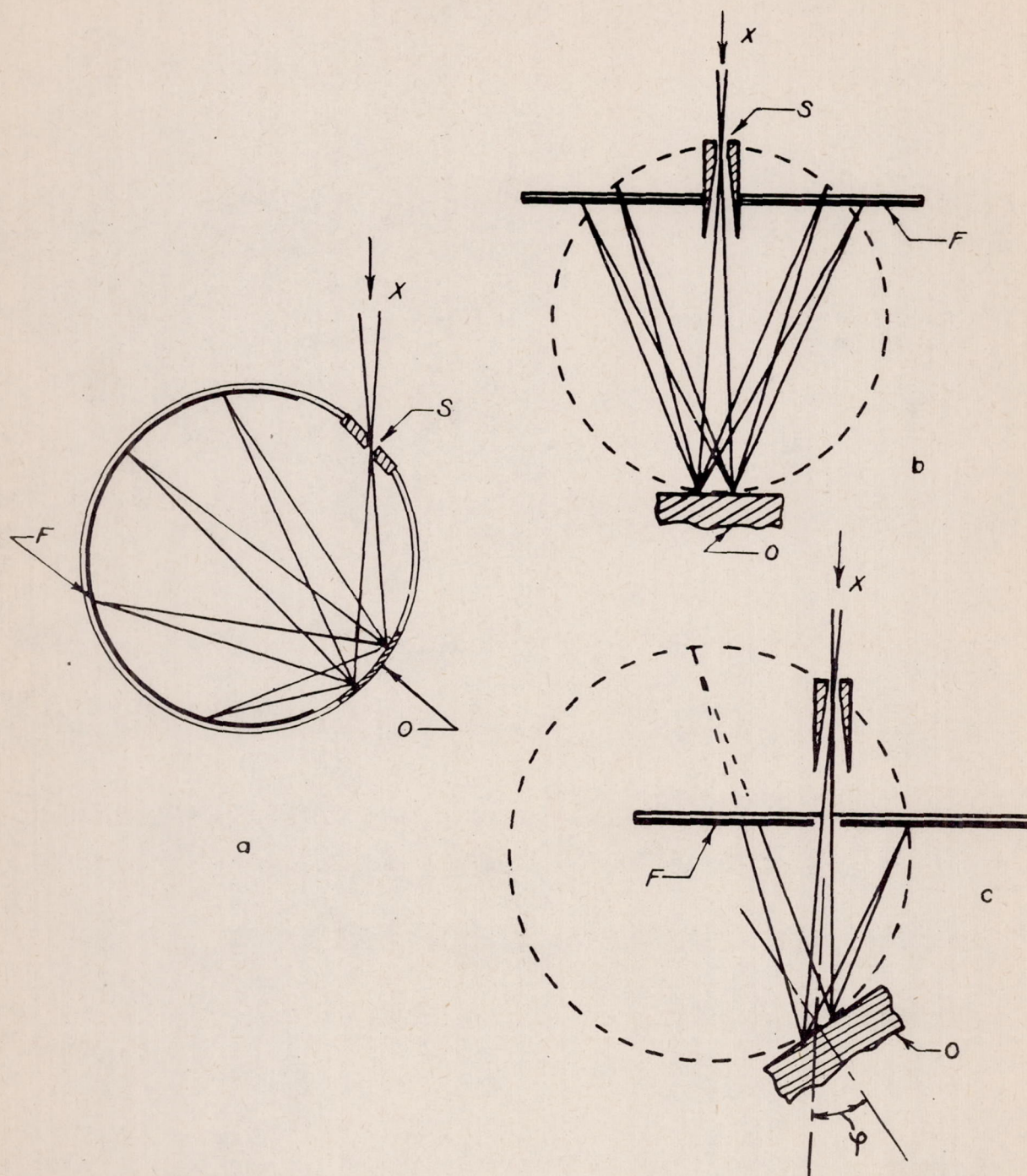
Figure 13.- Focusing conditions.
