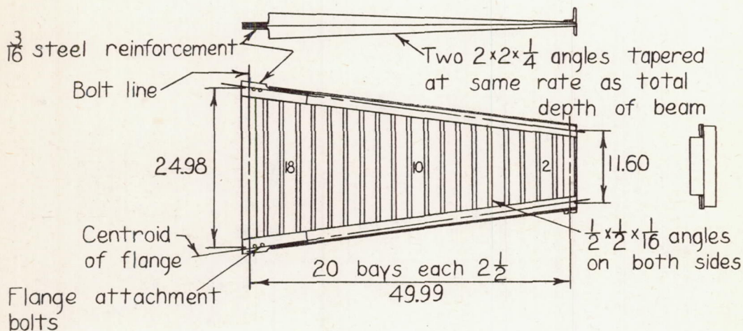
(c) Tapered beam with tapered flange. Web thickness, 0.0379.
