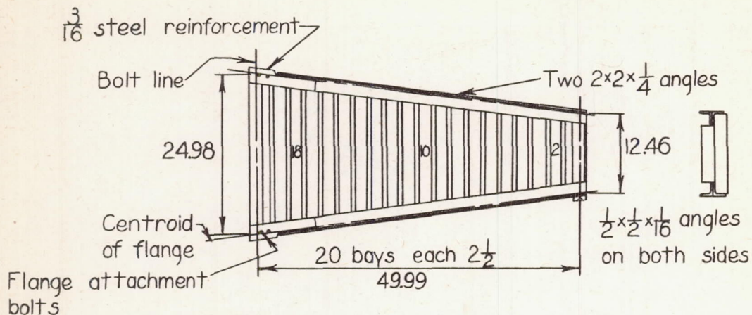
(b) Tapered beam with flanges of constant cross section. Web thickness 0.0392.
