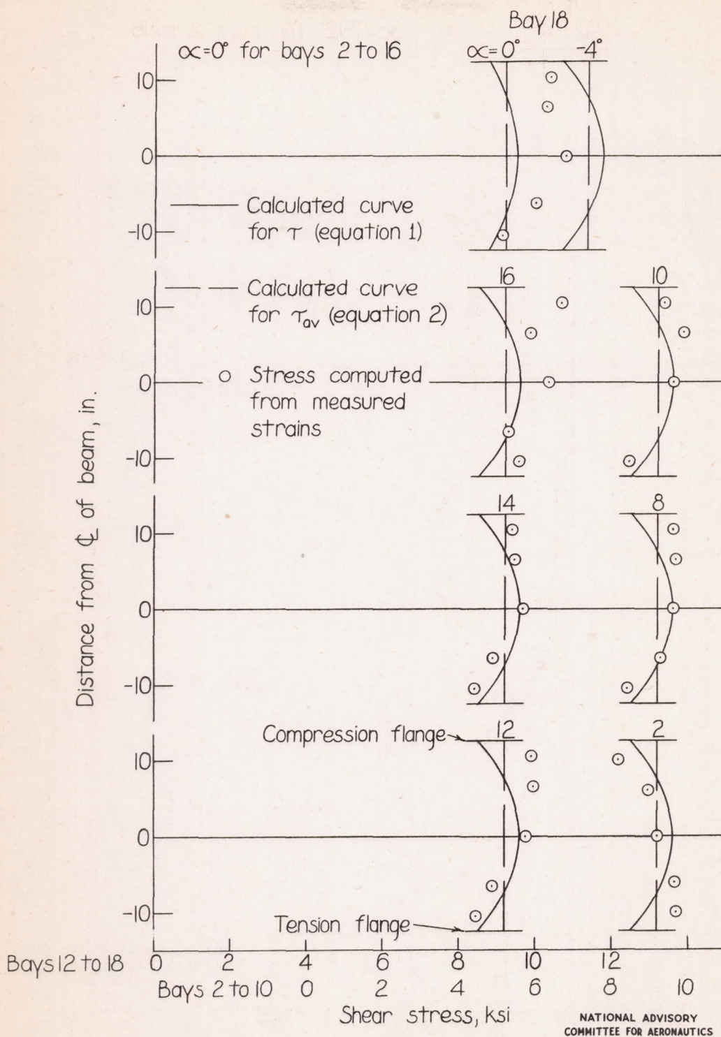
Figure 4.- Measured and calculated shear-stress distribution in the constant-depth beam. P=9 kips.
