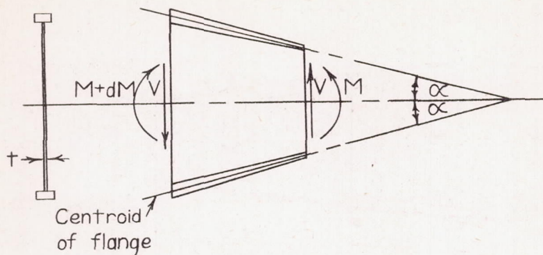
Figure 1.- Positive direction of forces and moments on tapered beams.
