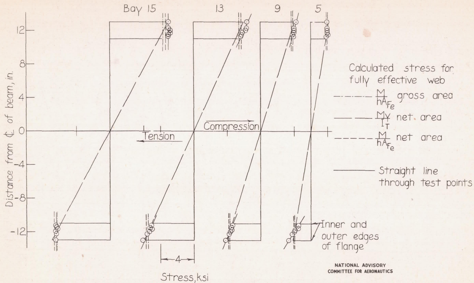
Figure 8.- Distribution of measured and calculated axial flange stress in the constant-depth beam. P=9 kips.
