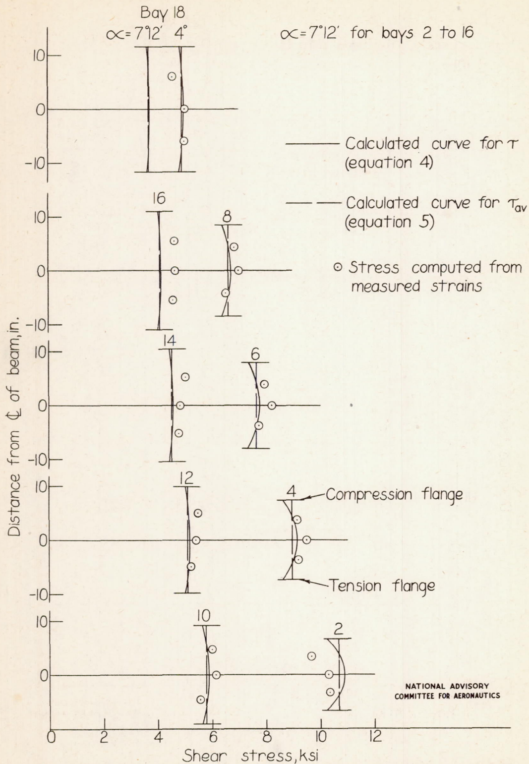
Figure 5.- Measured and calculated shear-stress distribution in the tapered beam with flanges of constant cross section. P=6 kips.
