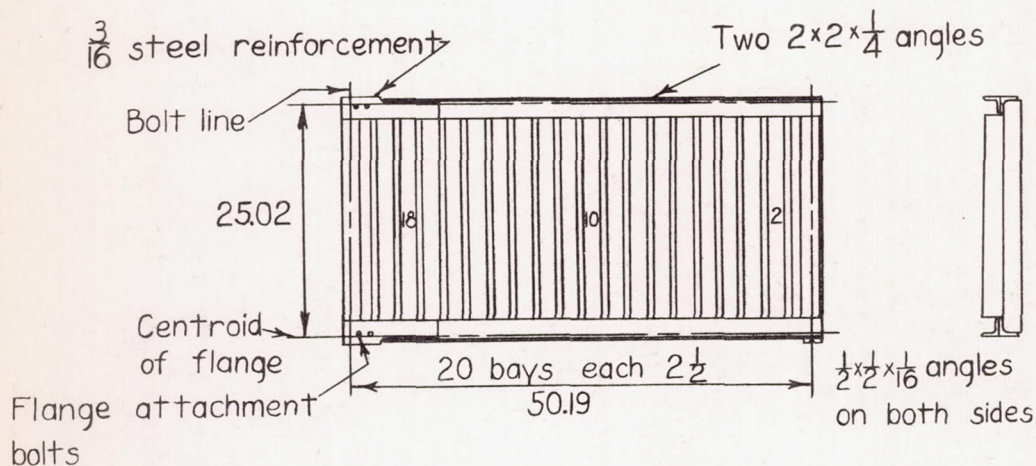
(a) Constant depth beam. Web thickness, 0.0392 .
