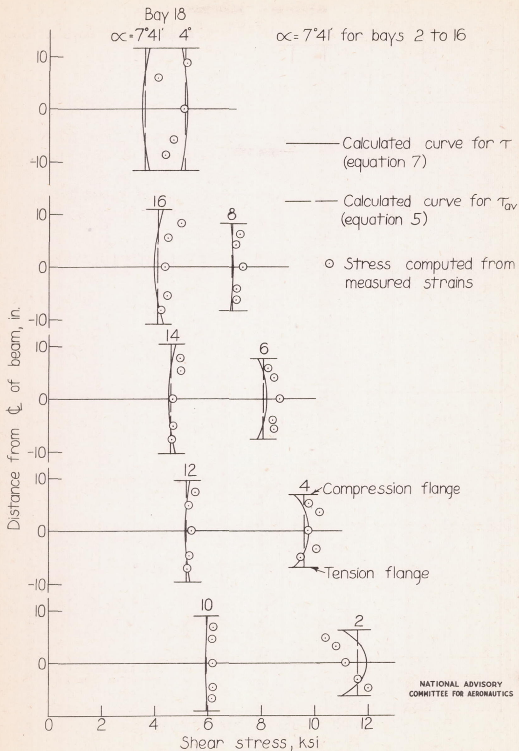
Figure 6.- Measured and calculated shear-stress distribution in the tapered beam with tapered flanges. P=6 kips.
