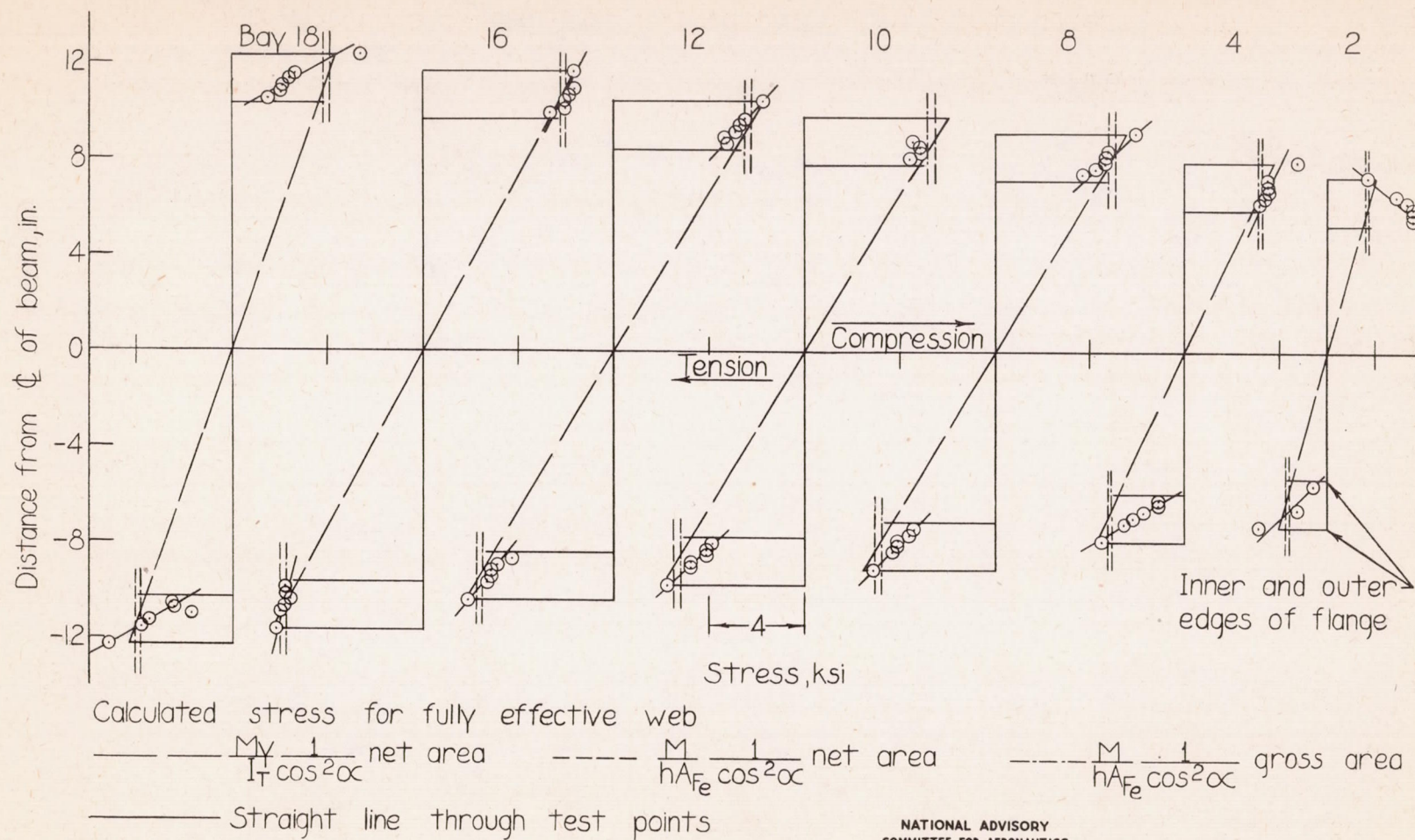
Figure 10.- Distribution of measured and calculated axial flange stress in the tapered beam with tapered flanges. P=6 kips.
