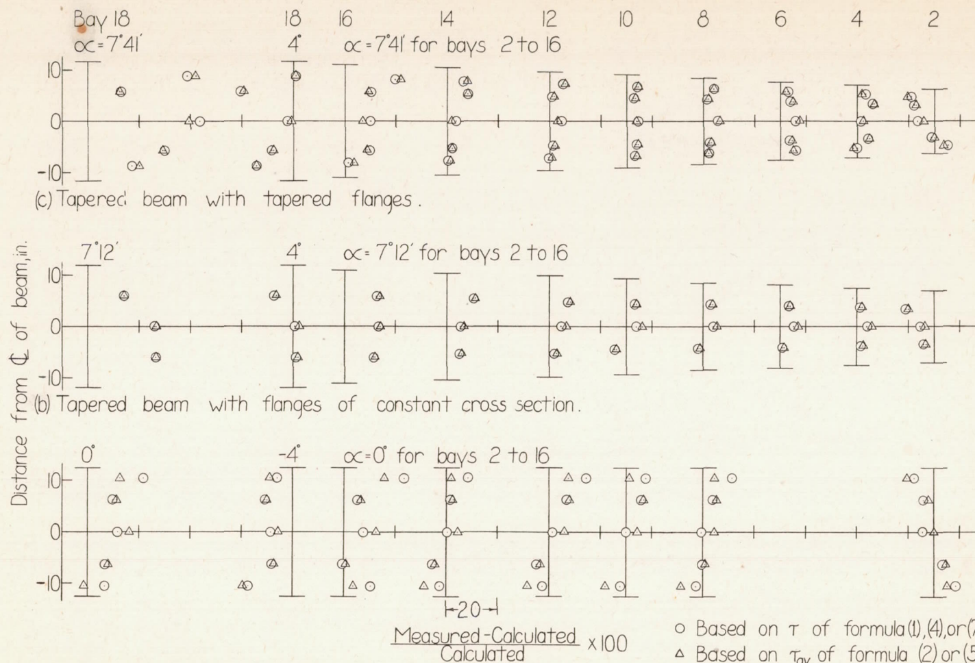
Figure 7.- Differences between measured and calculated shear stresses.
