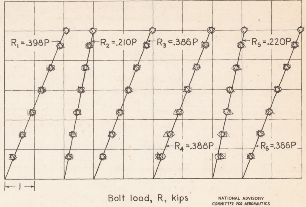
(b) Observed relationships between applied joint load and bolt loads.
