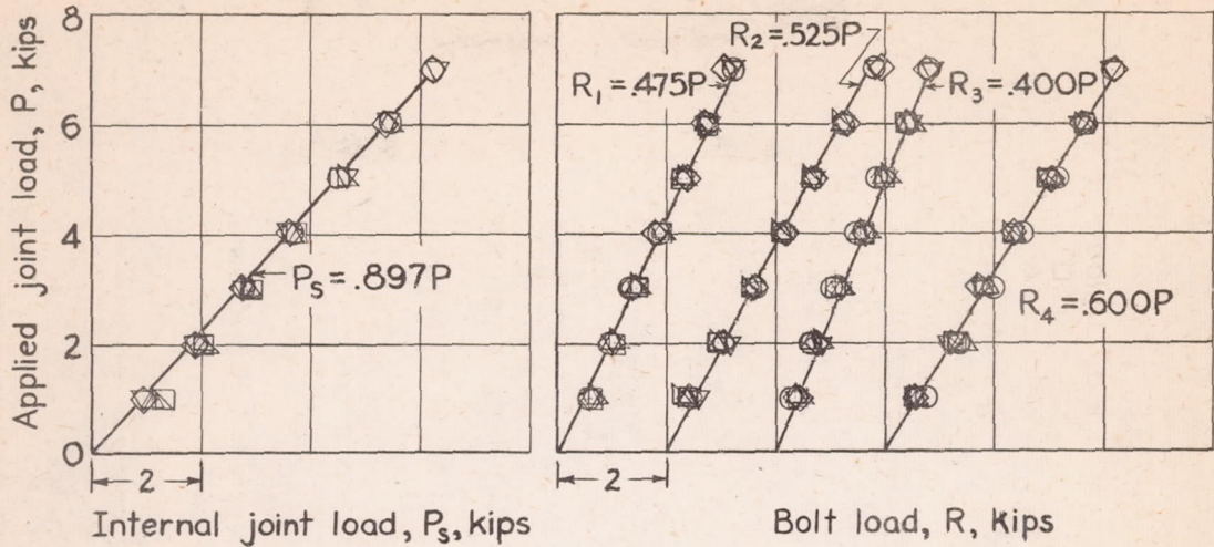
(a) Observed relationship between applied and internal joint loads. (b) Observed relationships between applied joint load and bolt loads.
