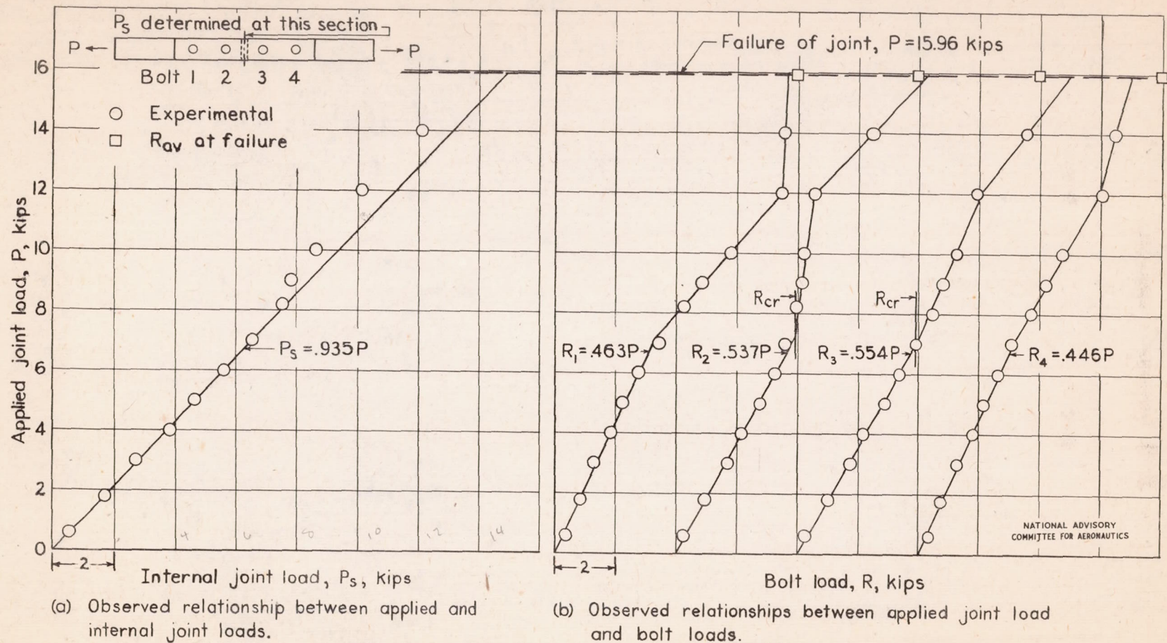
Figure 10.- Joint-load and bolt-load curves for specimen A-1 tested to failure.
