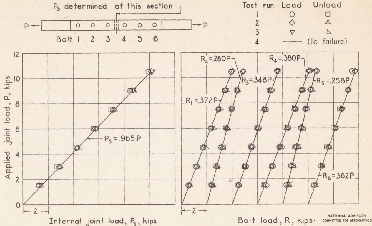
(a) Observed relationship between applied and internal joint loads.
