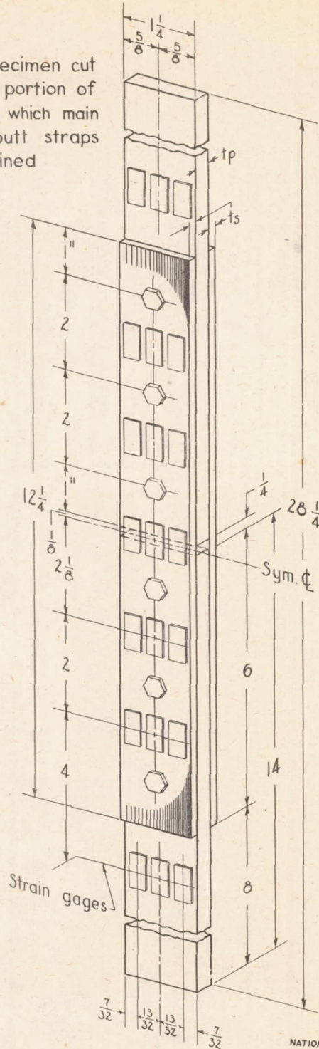
Three-bolt joint, group B
