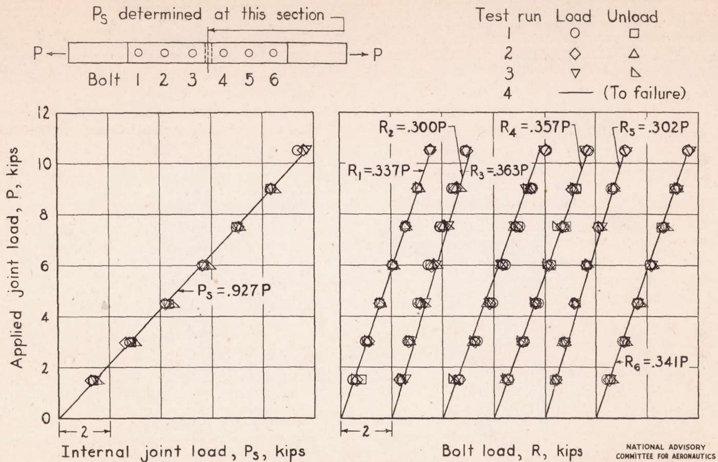
(a) Observed relationship between applied and internal joint loads. (b) Observed relationships between applied joint load and bolt loads.
