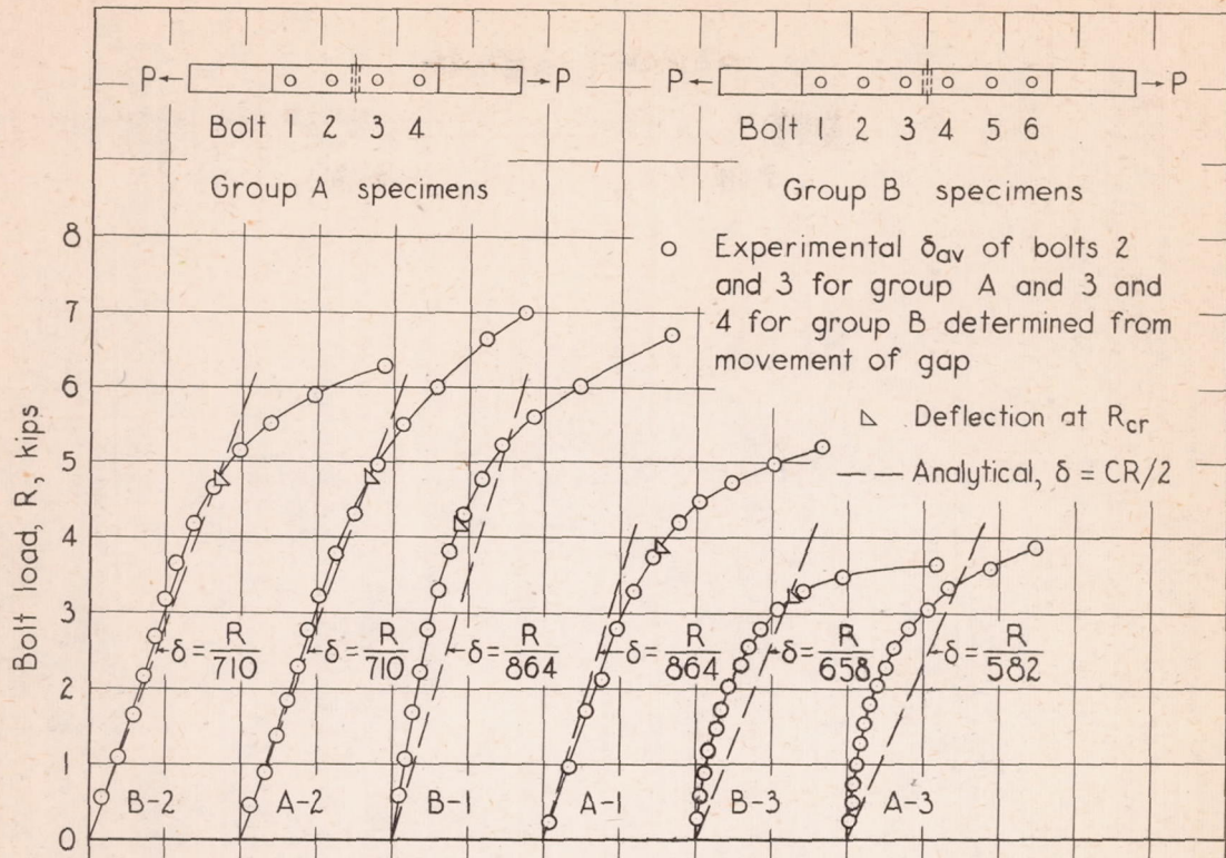
(a) Bolt deflections for specimens of groups A and B; 24S-T plates and heat-treated (125 ksi) alloy-steel bolts.
