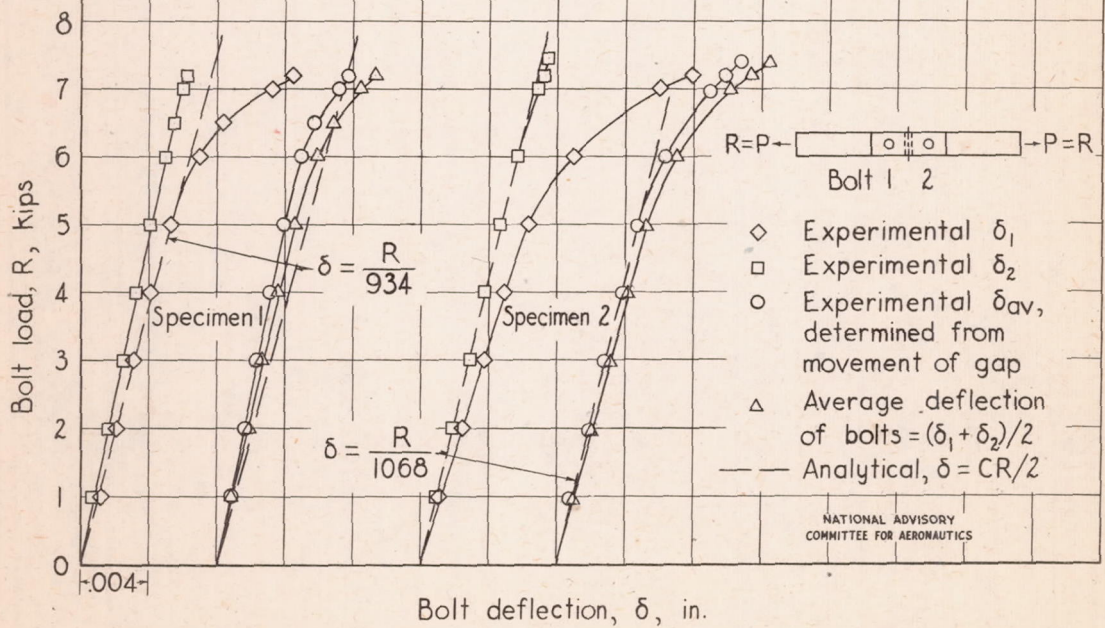
(b) Bolt deflections for auxiliary-shear-test specimens; SAE 6150 steel plates and heat-treated (125 ksi) alloy-steel bolts.
