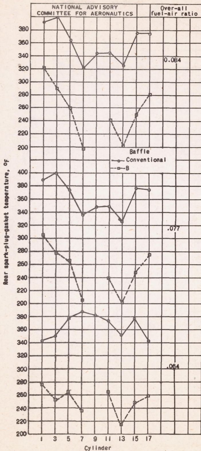
(b) Rear spark-plug-gasket temperature.
