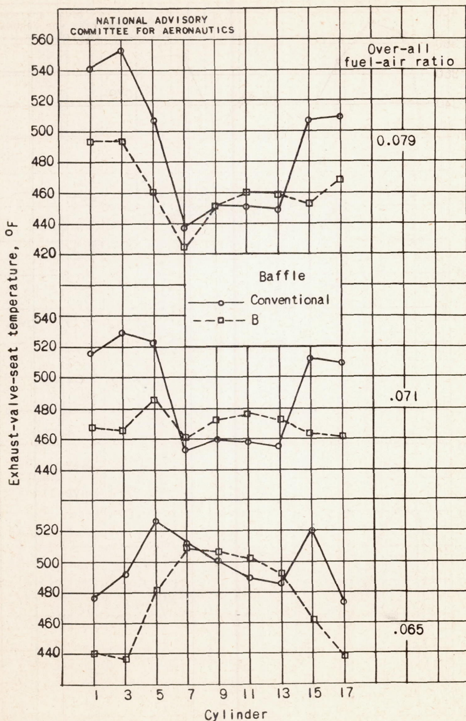
(a) Exhaust-valve-seat temperature.
