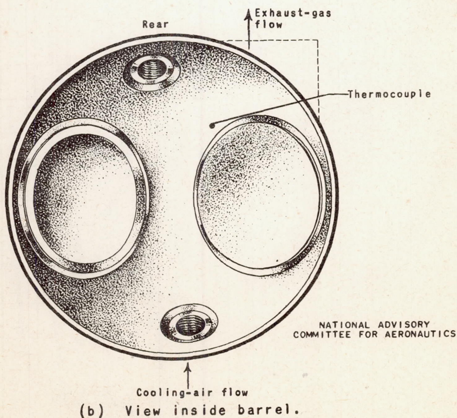
Figure 4. - Location of exhaust-valve-seat thermocouple on a rear-row cylinder of an air-cooled engine.
