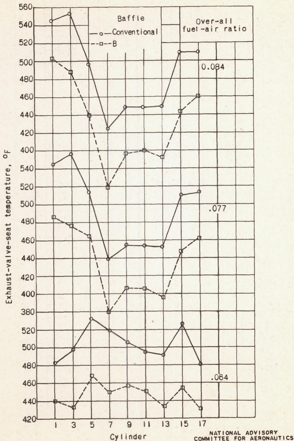
(a) Exhaust-valve-seat temperature.
