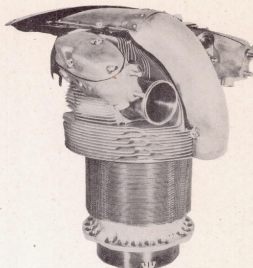
Left rear view of baffle A
