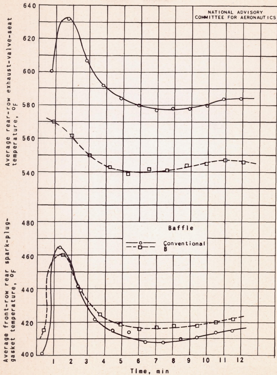
Figure 5. - History of average cylinder-head temperature of cylinders 1, 3, 5, 15, and 17 during take-off and climb.
