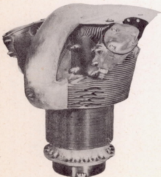
Right rear view of baffle B
