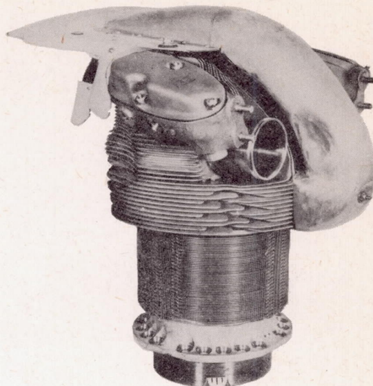
Left rear view of baffle B
