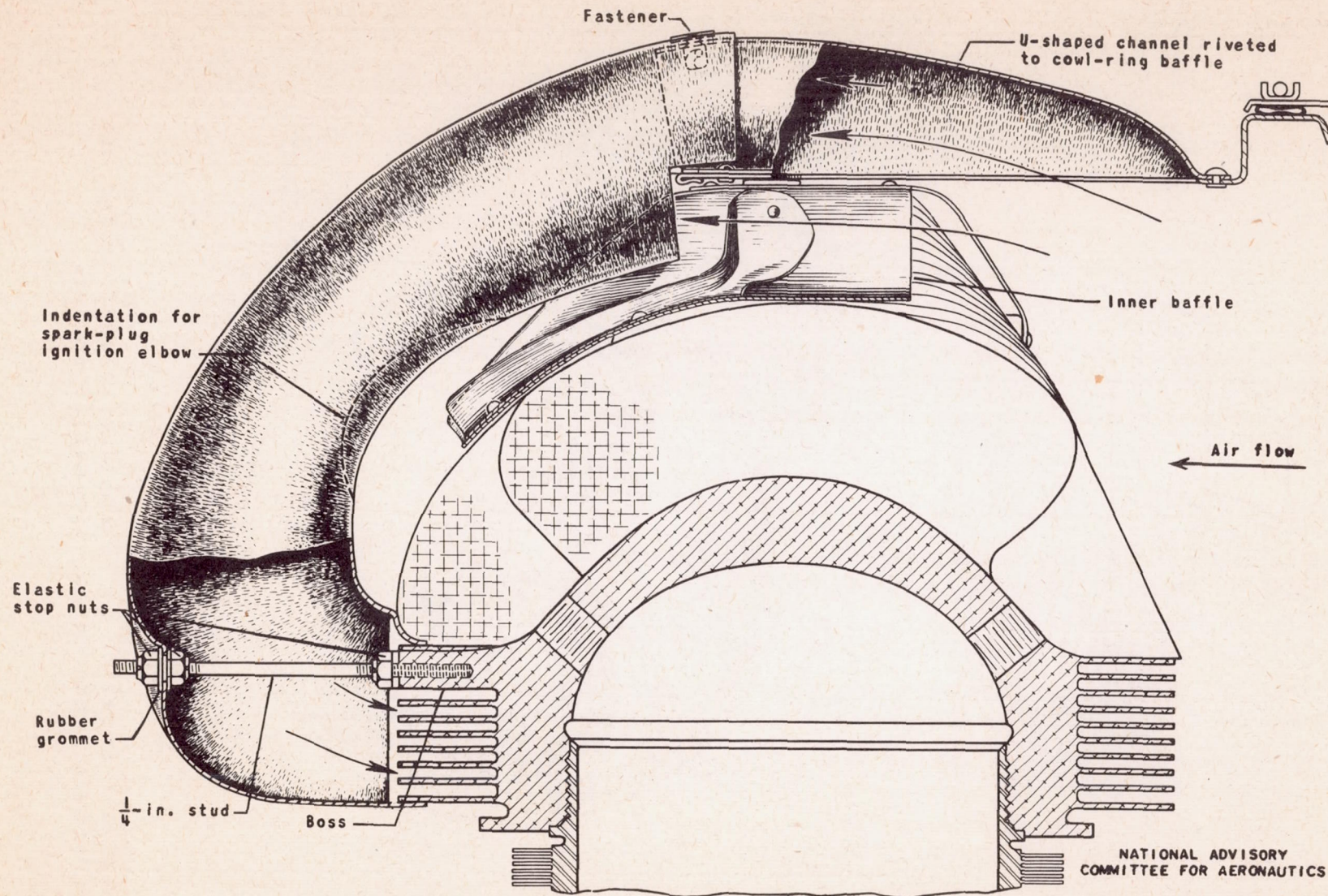
Figure 3. - Cutaway view of ducted baffle B installed on a rear-row cylinder head of an air-cooled engine.
