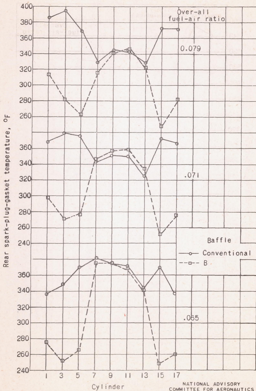
(b) Rear spark-plug-gasket temperature.
