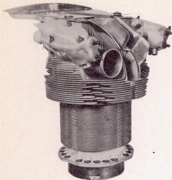
Left rear view of conventional baffle
