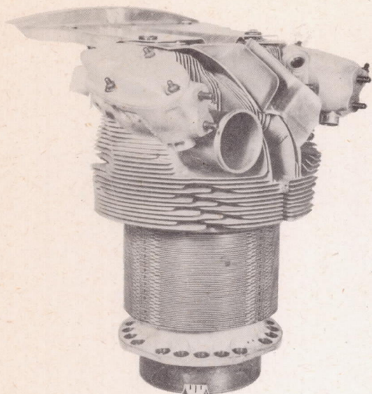
Left rear view of conventional head baffle
