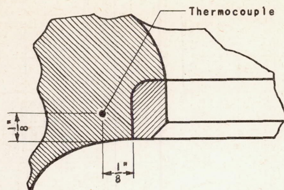
(a) Section through valve seat.
