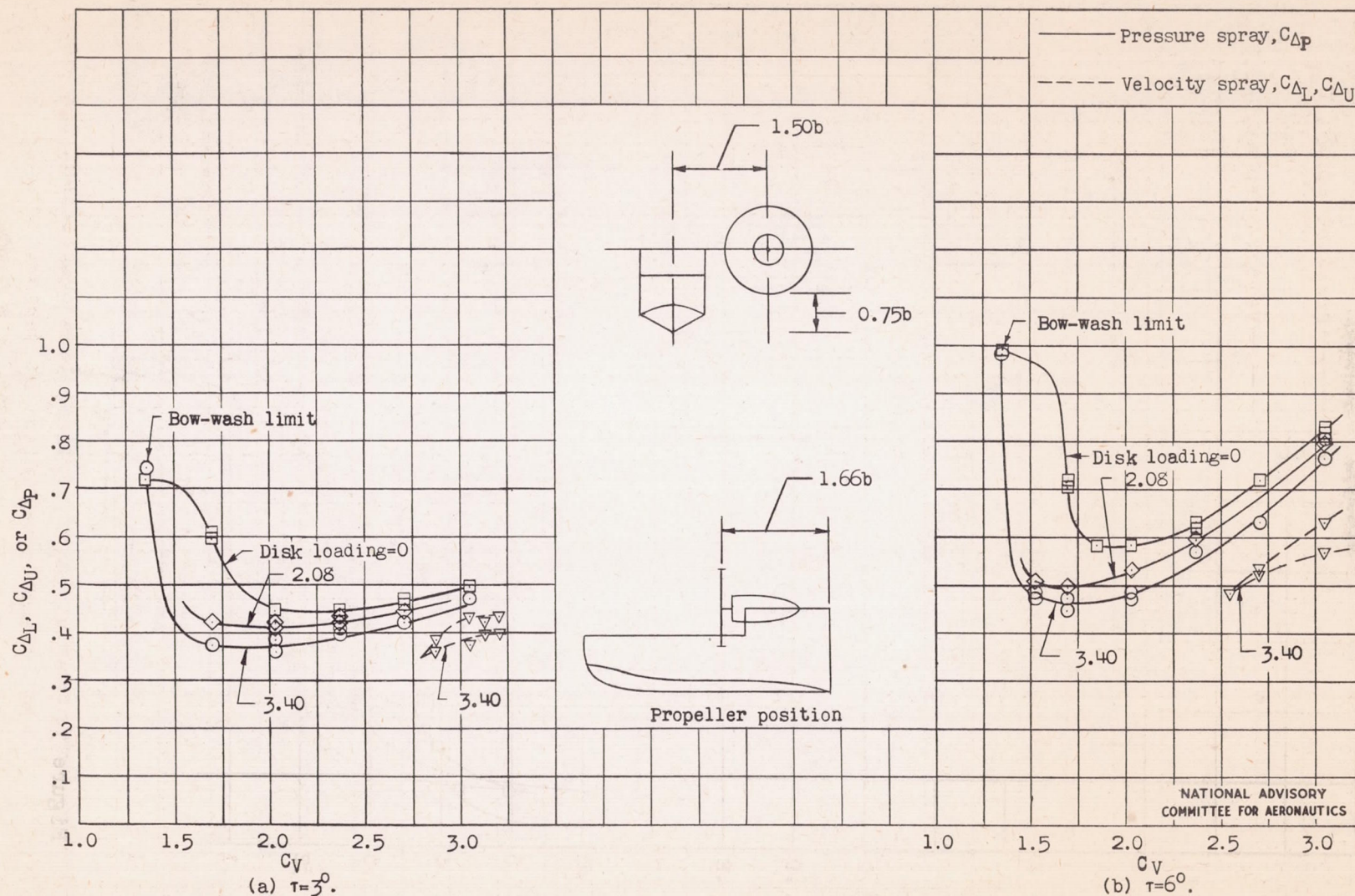
Figure 8.- Variation of critical load coefficient for spray with speed coefficient at various trims for three disk loadings. x = 1.66b ; y = 1.50b ; z = 0.75b .
