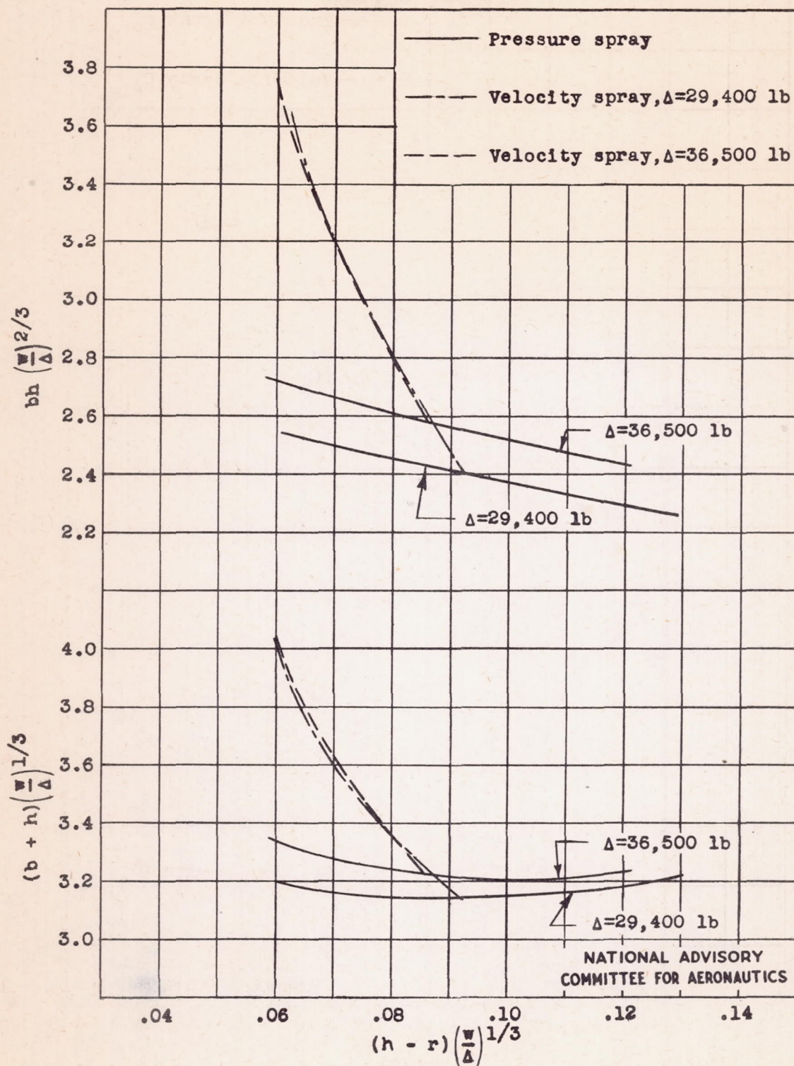
Figure 19.- Effect of vertical position of propellers on frontal area and periphery for a given design load with given spray characteristics.
