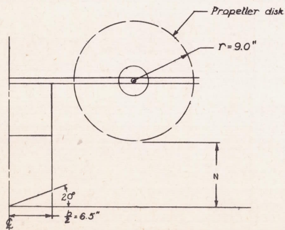
Figure 1. - General arrangement of model.
