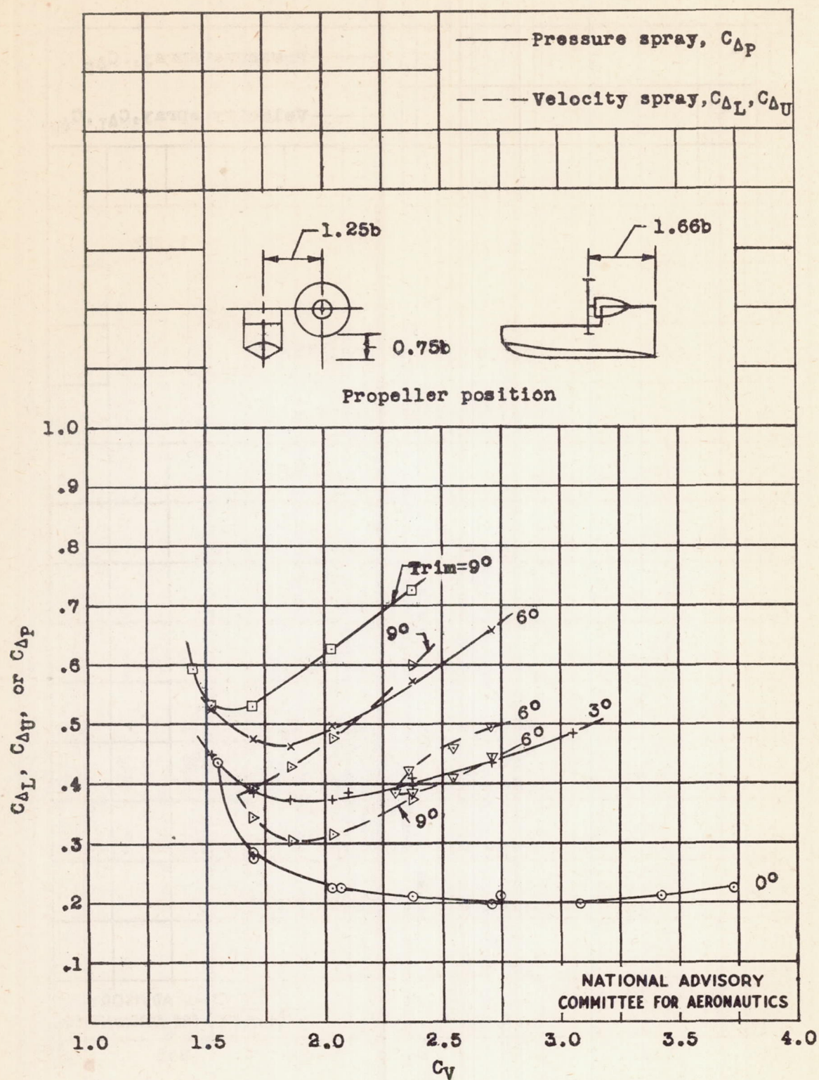
Figure 12.- Variation of critical load coefficient for spray with speed coefficient at various trims.
