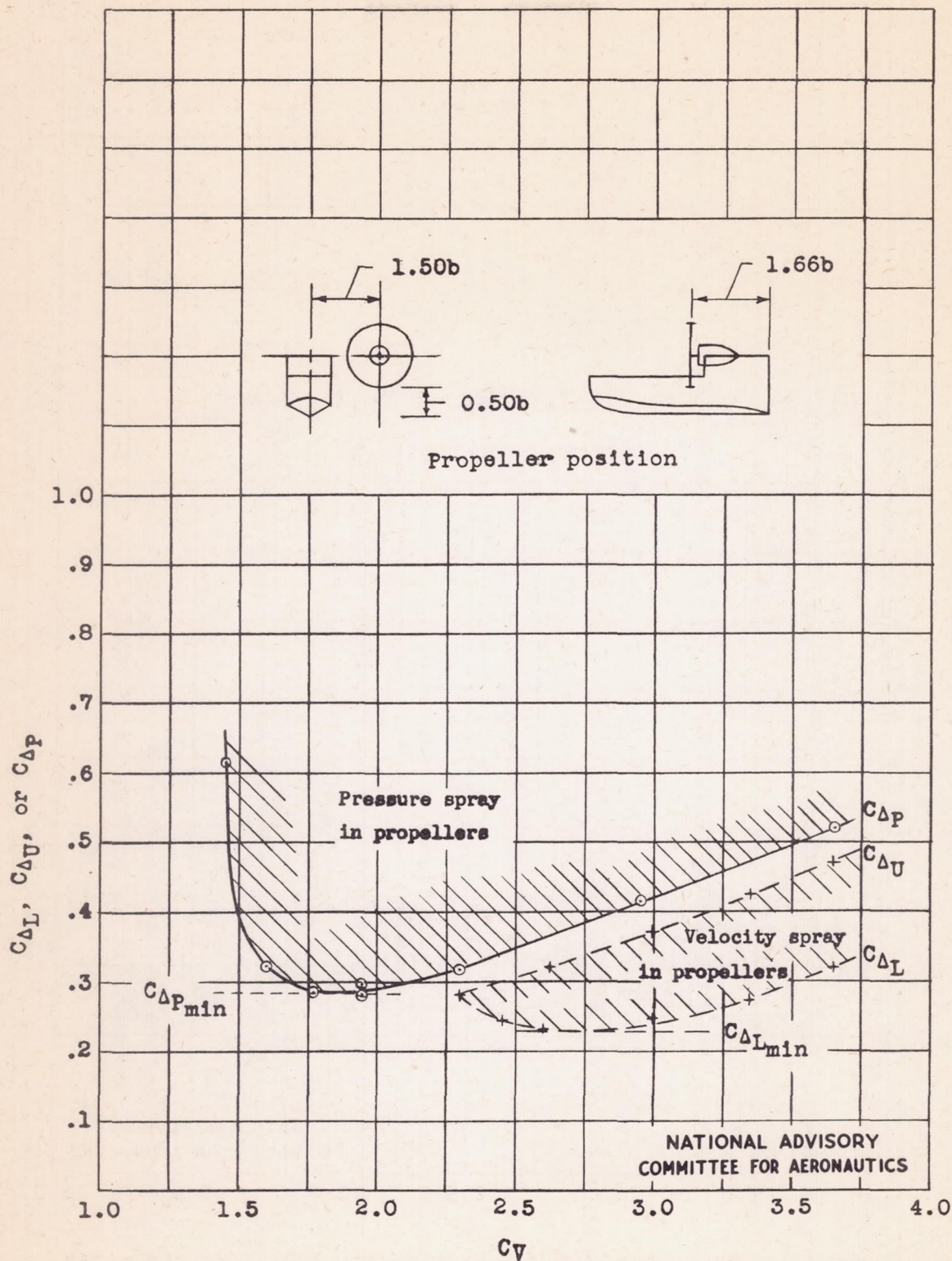
Figure 6.- Typical curves illustrating the coefficients used.
