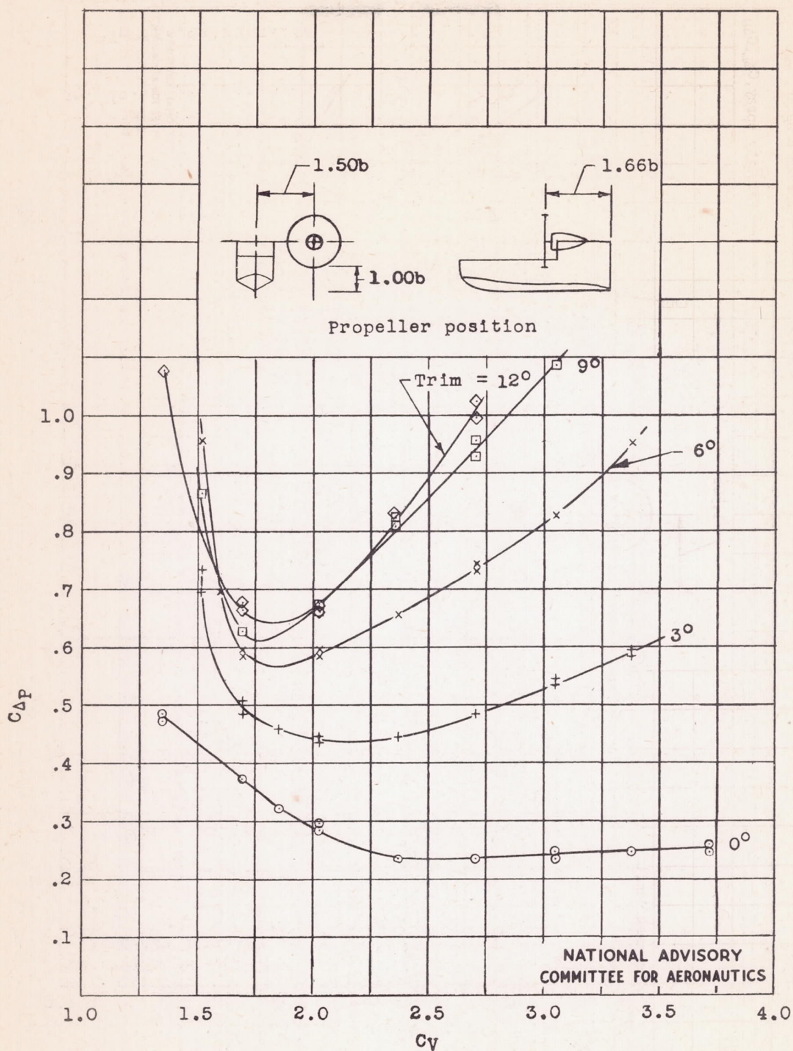
Figure 9.- Variation of critical load coefficient for pressure spray with speed coefficient at various trims.
