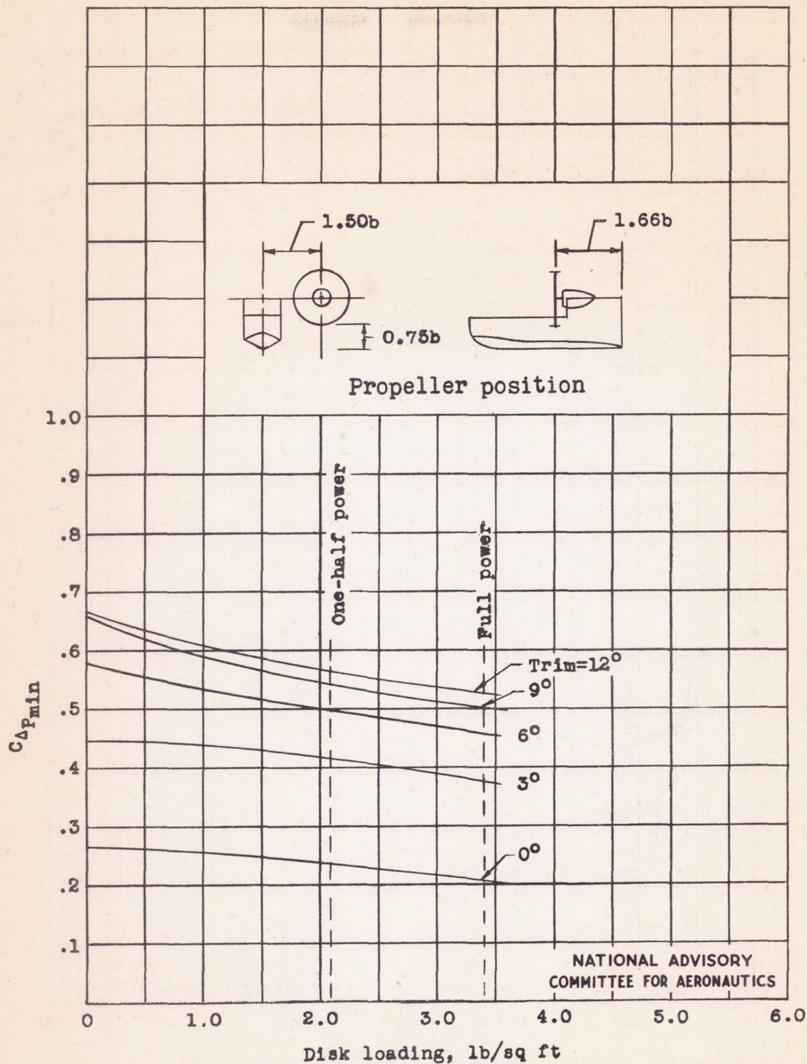
Figure 15.- Effect of disk loading on C_{D_{pmin}} at various trims.
