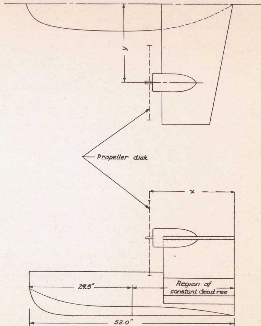
Figure 1. - General arrangement of model.
