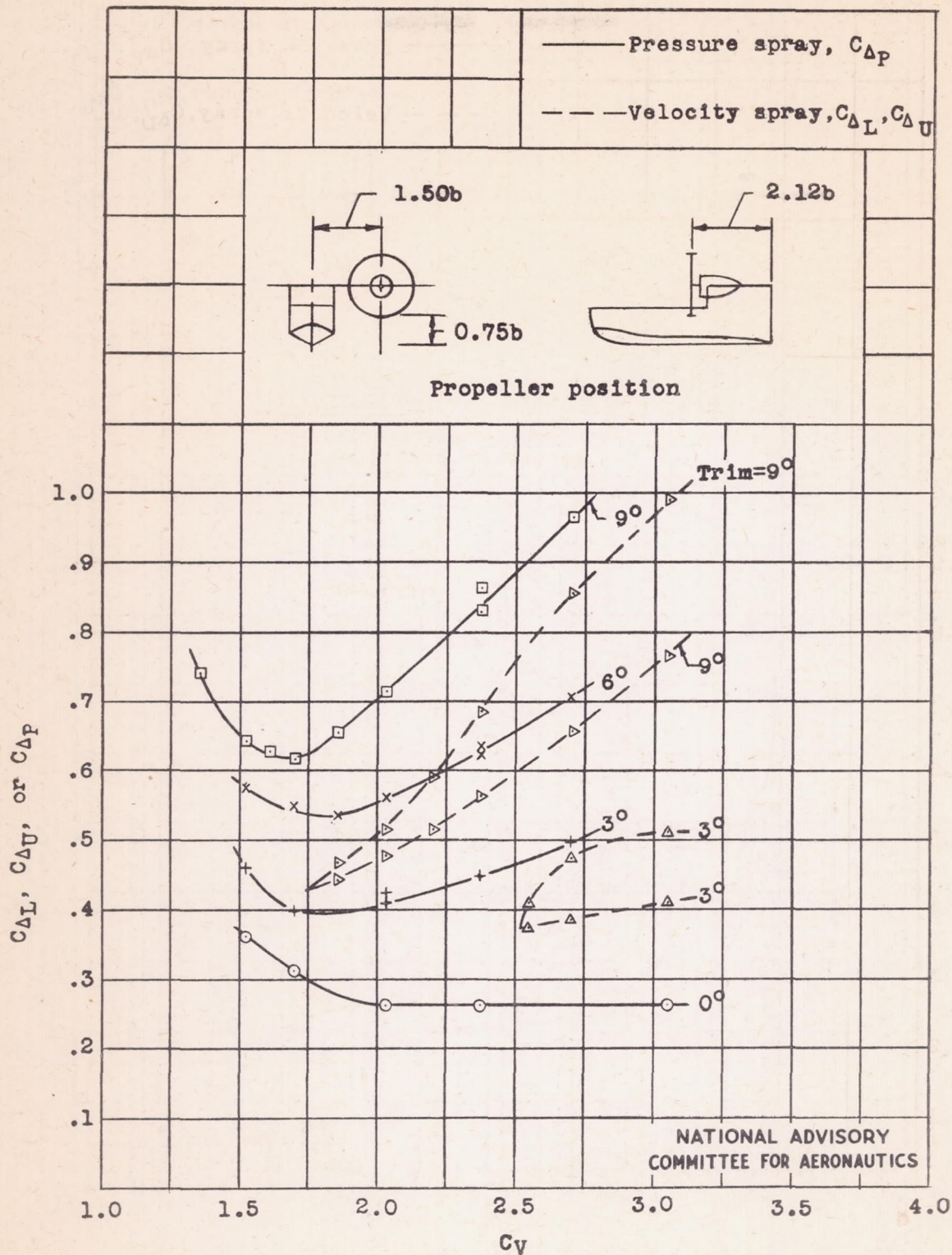
Figure 11.- Variation of critical load coefficient for spray with speed coefficient at various trims.
