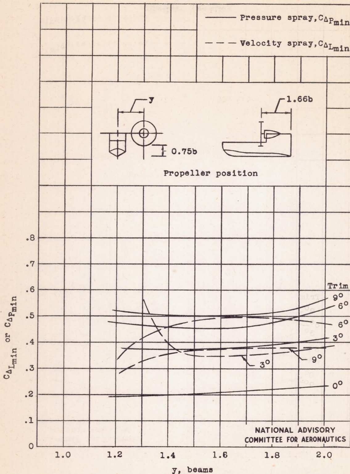
Figure 17.- Effect of lateral position of propellers on C_{\Delta P_{min}} and C_{\Delta L_{min}} .
