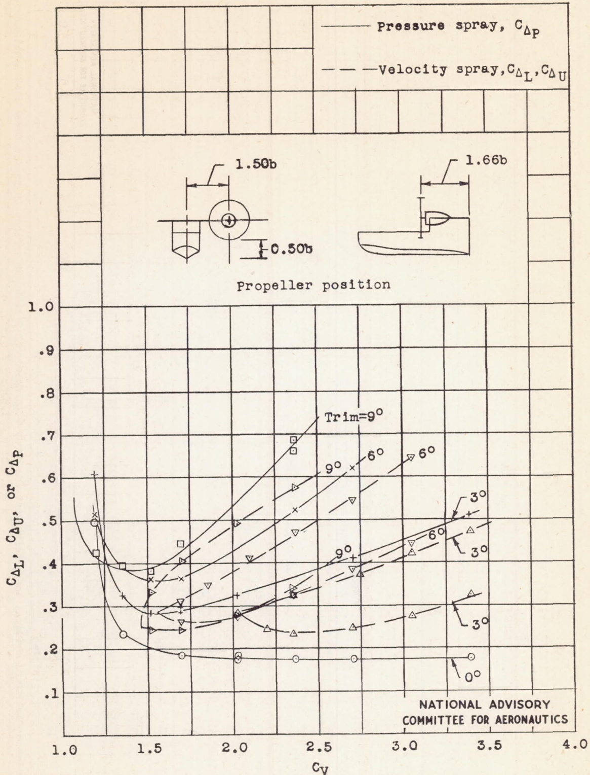
Figure 7.- Variation of critical load coefficient for spray with speed coefficient at various trims.
