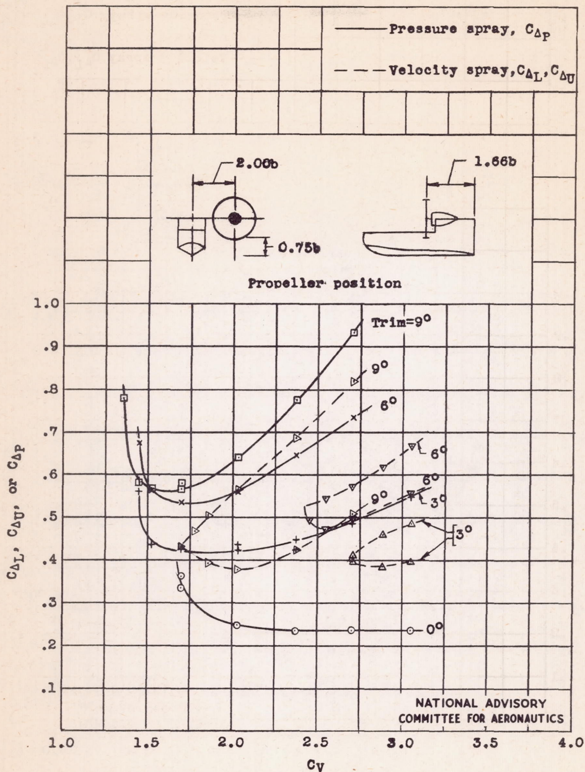
Figure 13.- Variation of critical load coefficient for spray with speed coefficient at various trims.
