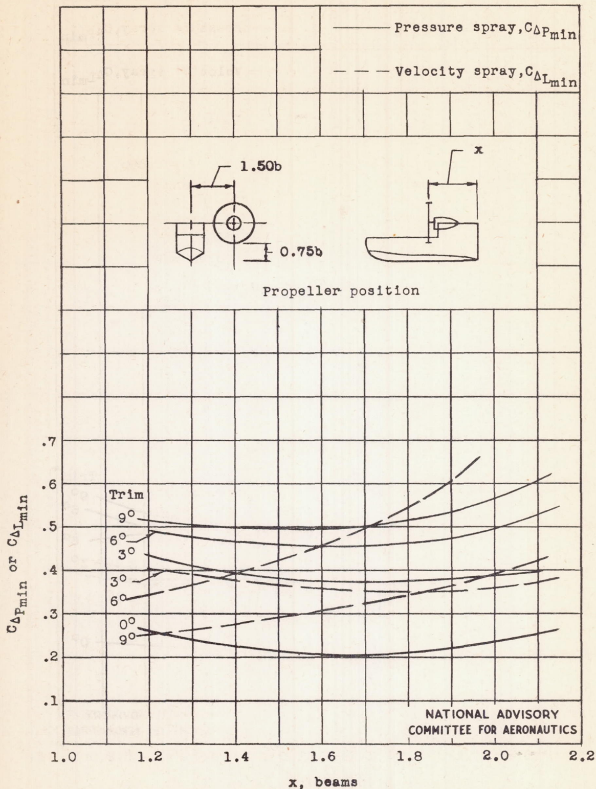
Figure 16.- Effect of longitudinal position of propellers on C_{\Delta P_{min}} and C_{\Delta L_{min}} .
