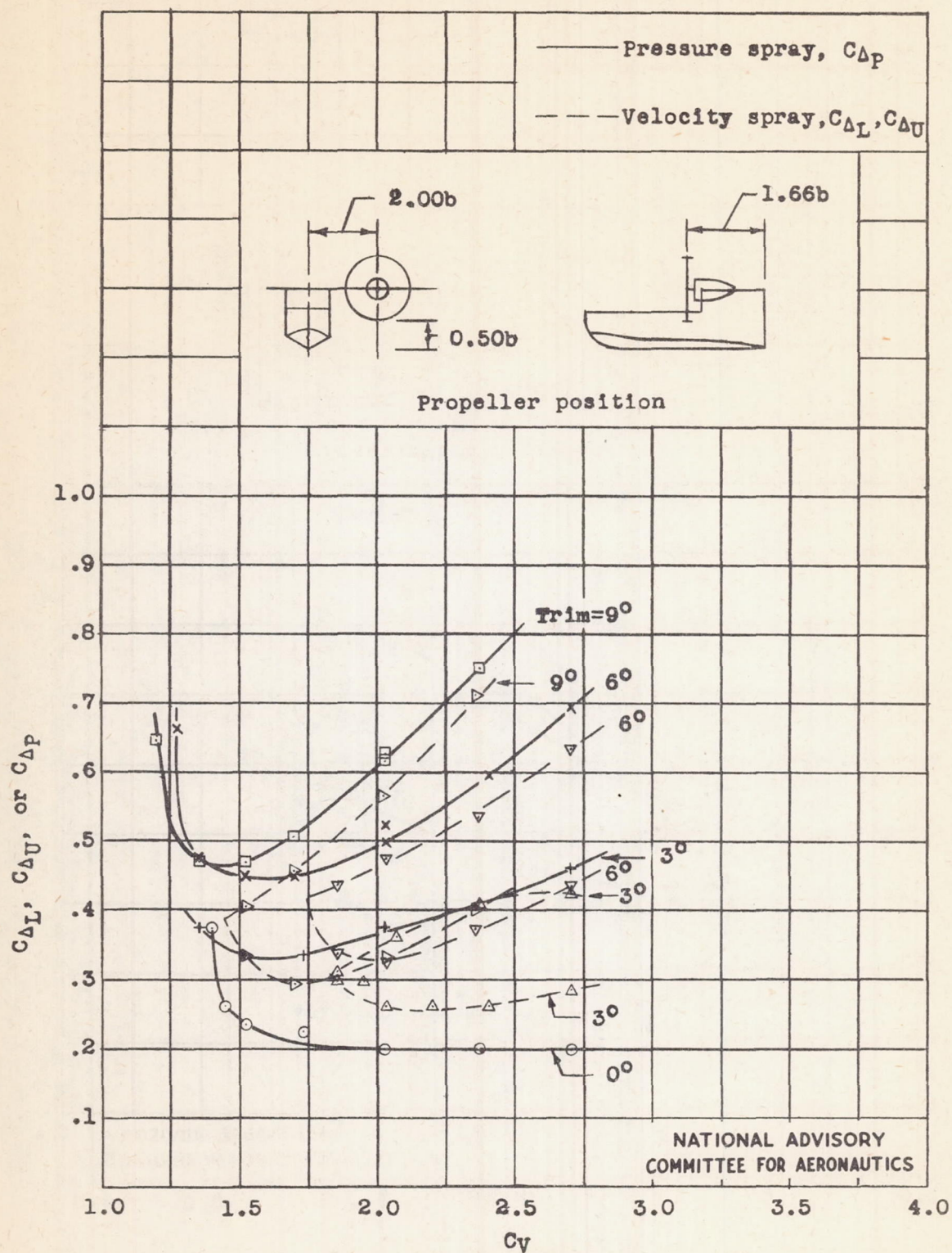
Figure 14.- Variation of critical load coefficient for spray with speed coefficient at various trims.
