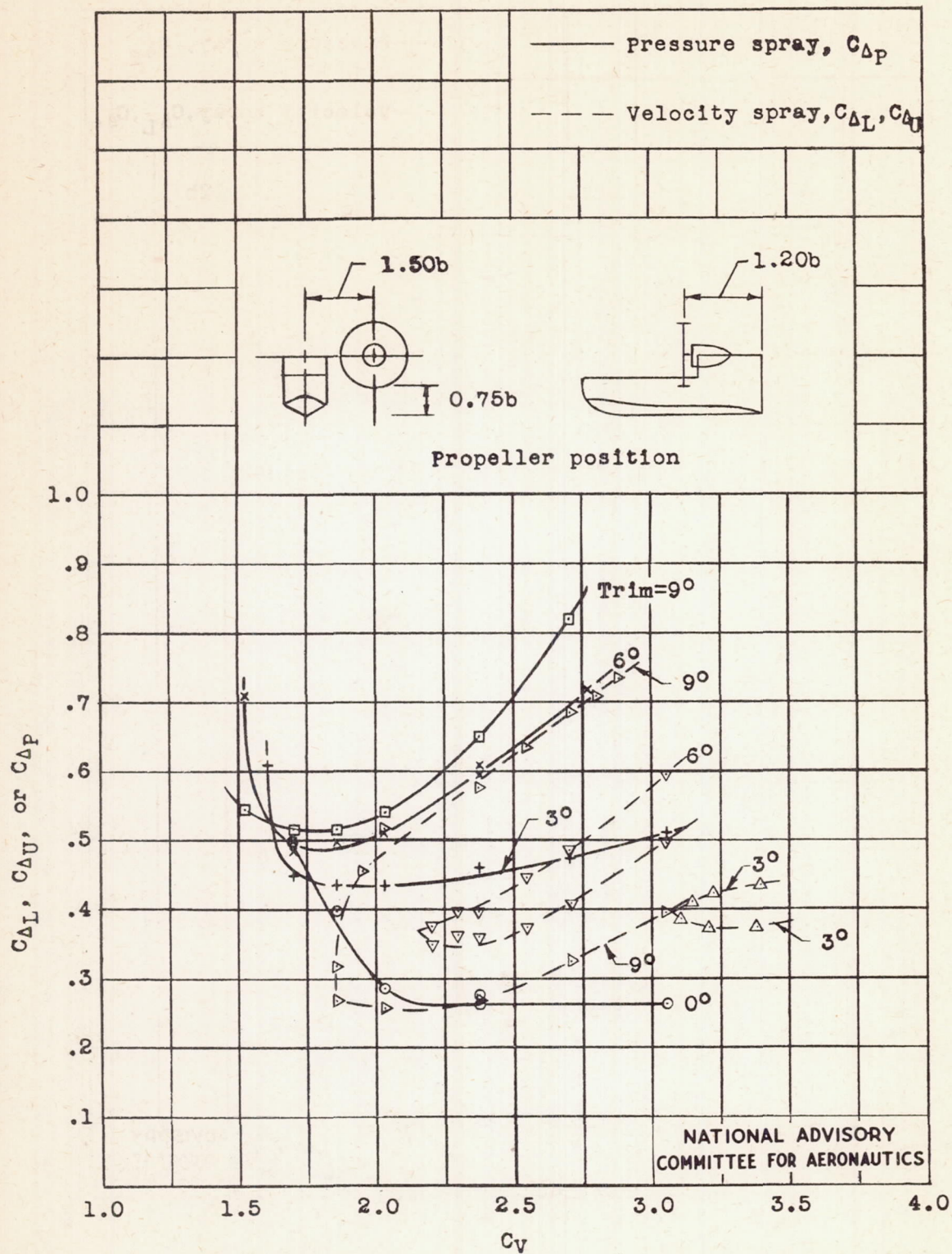
Figure 10.- Variation of critical load coefficient for spray with speed coefficient at various trims.
