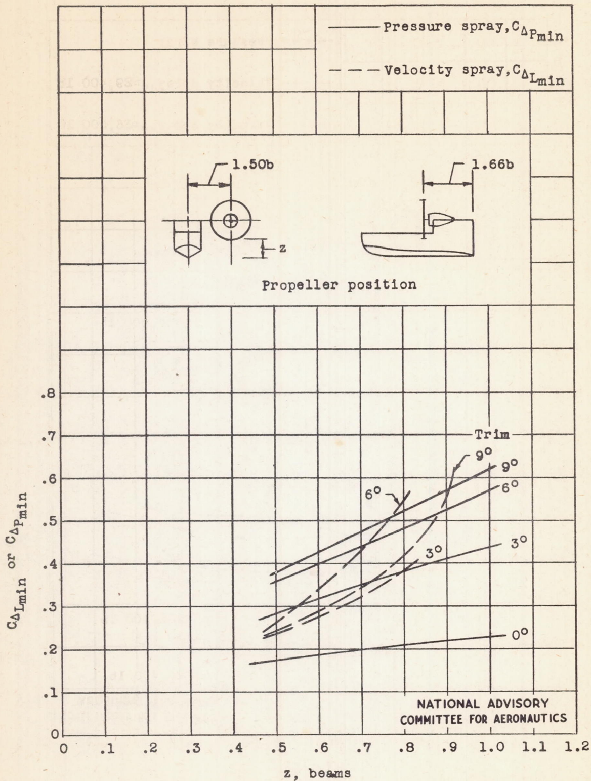
Figure 18.- Effect of vertical position of propellers on C_{\Delta P_{min}} and C_{\Delta L_{min}} .
