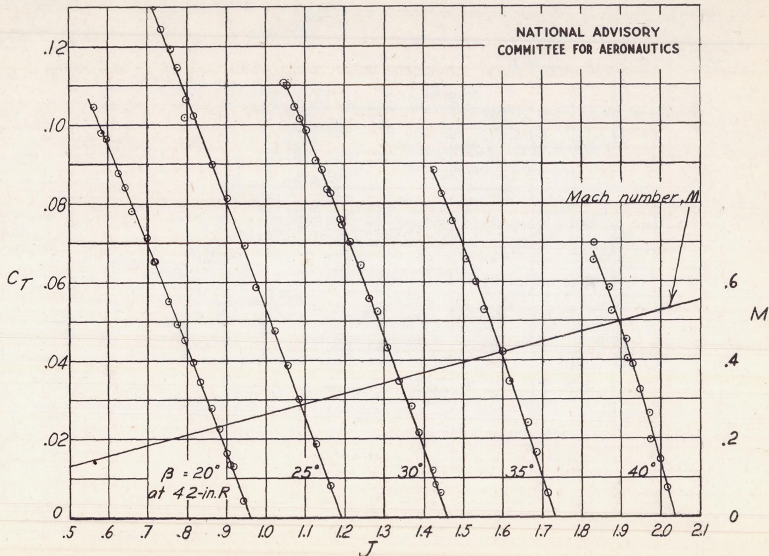
Figure 8.- Variation of thrust coefficient with advance ratio. Clean blades; D=10 feet.
