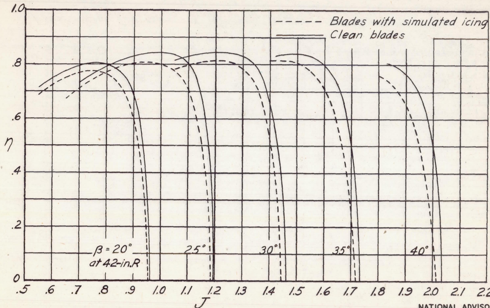
Figure 14.- The effect of icing on propeller efficiency. D = 10 feet.
