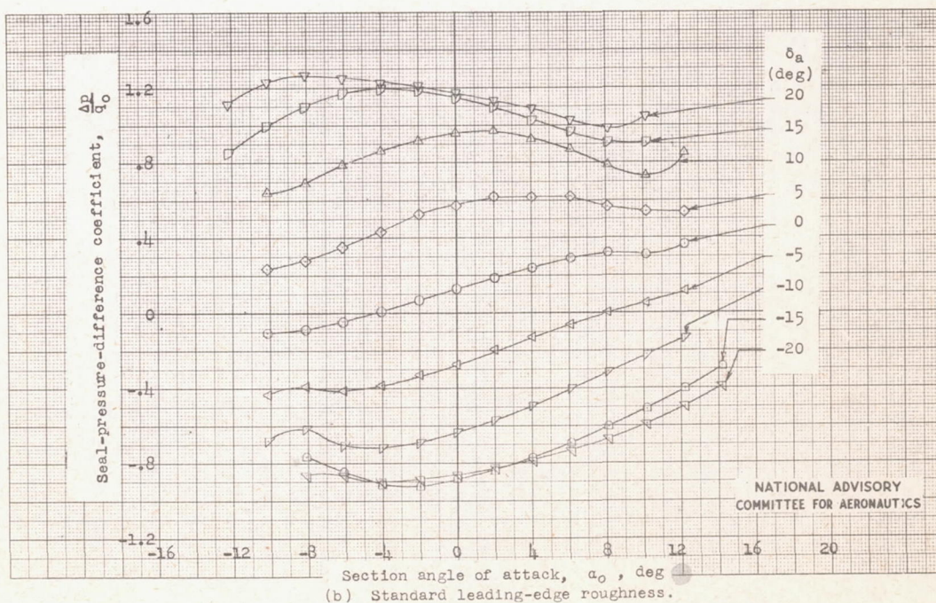
Figure 6.- Variation of \frac{\Delta p}{q_0} with \alpha_0 for a sealed 0.22c internally balanced aileron of true airfoil contour on an NACA 65(112)-213 airfoil section. R = 8 \times 10^6 ; TDT 708.
