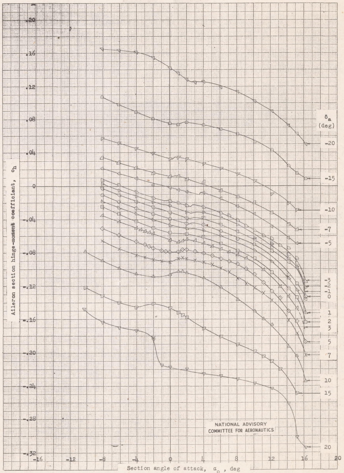
Figure 10.- Hinge-moment characteristics of a sealed 0.22c internally balanced aileron of modified contour on an NACA 65(112)-213 airfoil section. R = 8 \times 10^6 ; tests, TDT 709 and 711.
