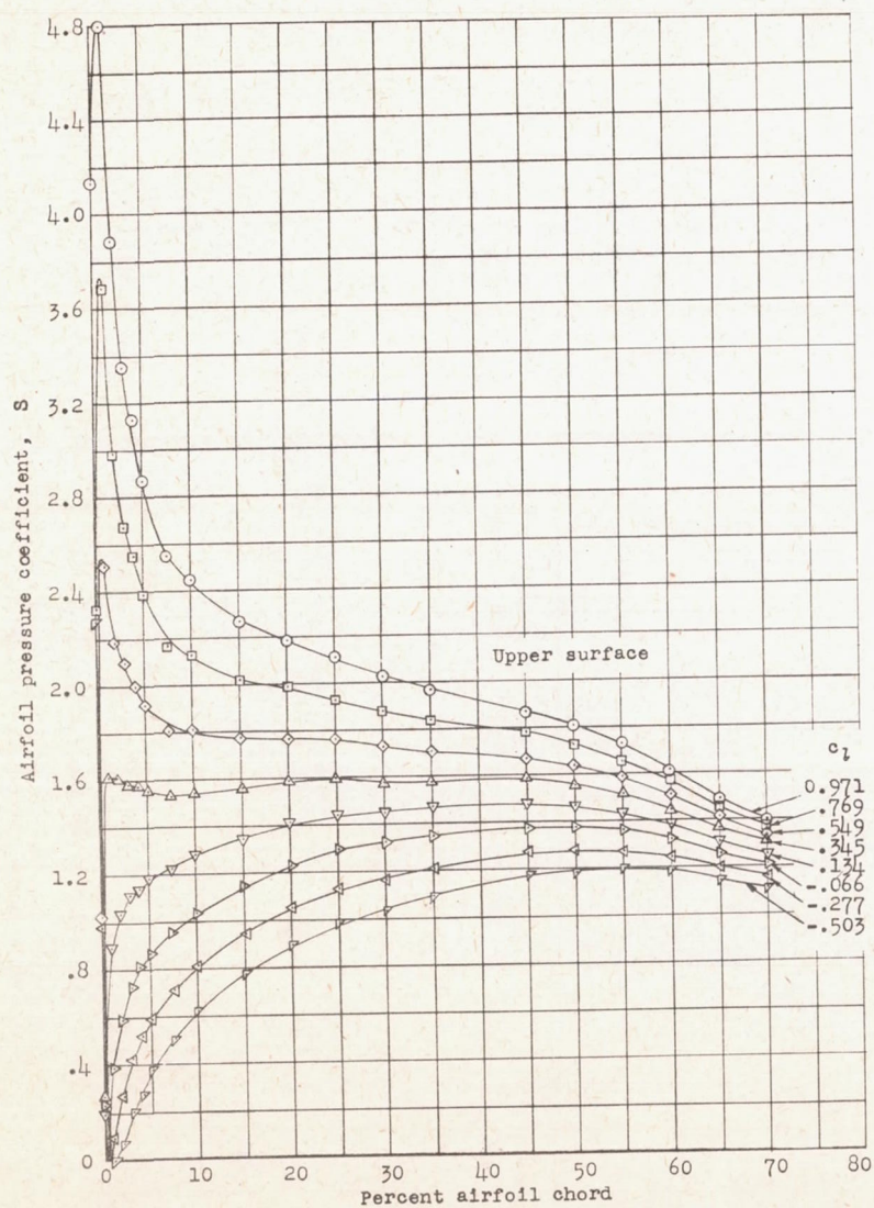
Figure 15.- Experimental pressure distributions for an NACA 65(112)-213 airfoil section equipped with a sealed 0.22c internally balanced aileron. \delta_a = 0^\circ ; tests, TDT 704, 707, and 714.
