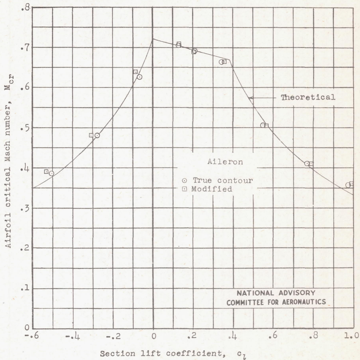
Figure 16.- Variation of predicted critical Mach number with low-speed section lift coefficient for an NACA 65(112)-213 airfoil section equipped with a sealed 0.22c internally balanced aileron. \delta_a = 0^\circ .
