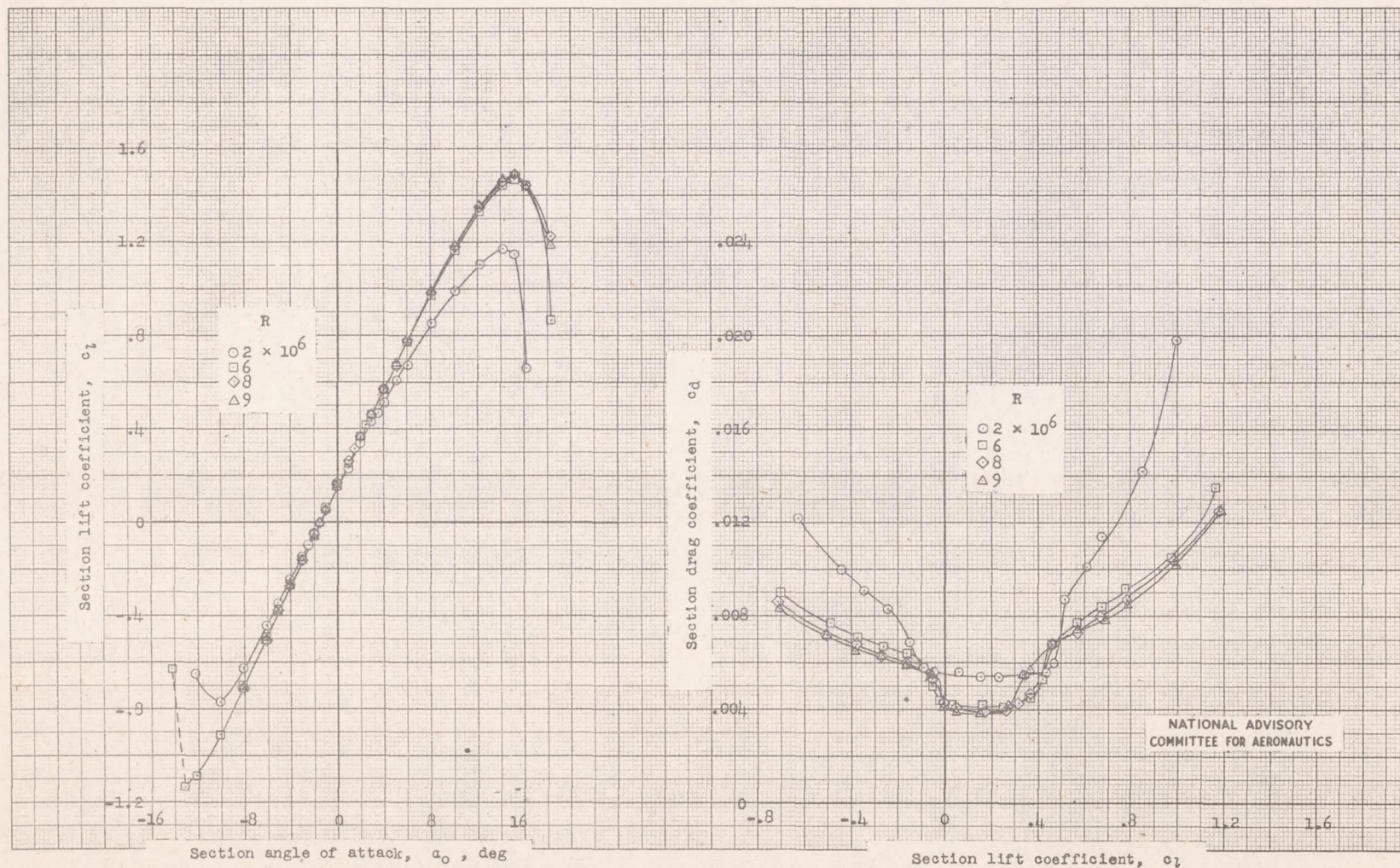
Figure 9 .- Lift and drag characteristics of an NACA 65(112)-213 airfoil section equipped with a sealed 0.22c internally balanced aileron of modified contour. \delta_a = 0^\circ ; tests, TDT 701 and 703.
