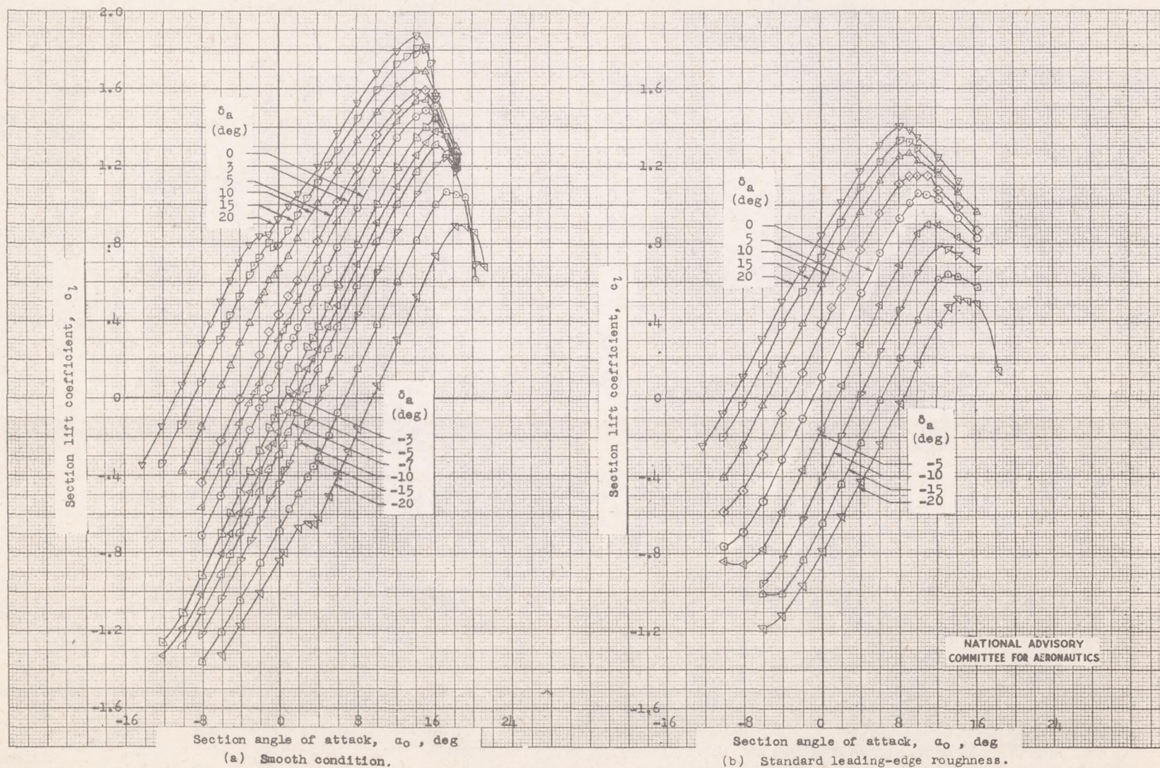
Figure 7.- Lift characteristics of an NACA 65(112)-213 airfoil section equipped with a sealed 0.22c internally balanced aileron of modified contour. R = 8 \times 10^6 ; tests, TDT 701 and 711.
