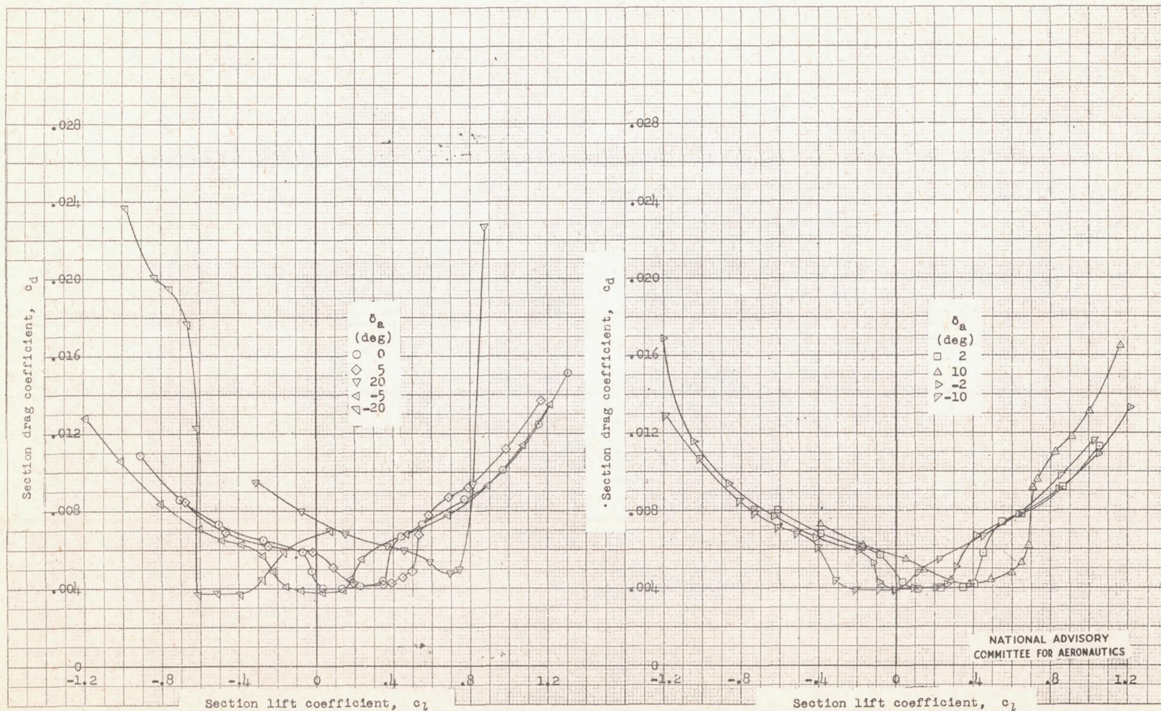
Figure 3.- Drag characteristics of an NACA 65(112)-213 airfoil section equipped with a sealed 0.22c internally balanced aileron of true airfoil contour. R = 8 \times 10^6 ; test, TDT 696.
