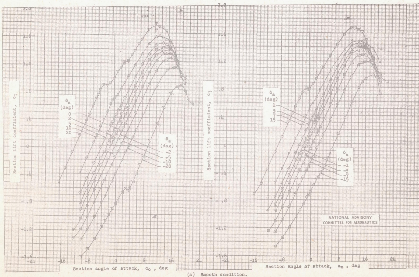
Figure 2.- Lift characteristics of an NACA 65(112)-213 airfoil section equipped with a sealed 0.22c internally balanced aileron of true airfoil contour. R = 8 \times 10^6 ; tests, TDT 696 and 708.
