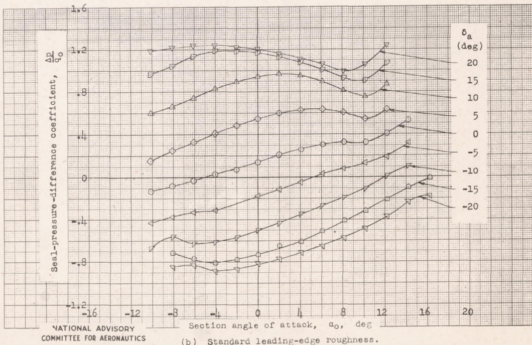
Figure 11.- Variation of \frac{\Delta P}{q_0} with \alpha_0 for a sealed 0.22c internally balanced aileron of modified contour on an NACA 65(112)-213 airfoil section. R = 8 \times 10^6 ; tests, TDT 709 and 711.
