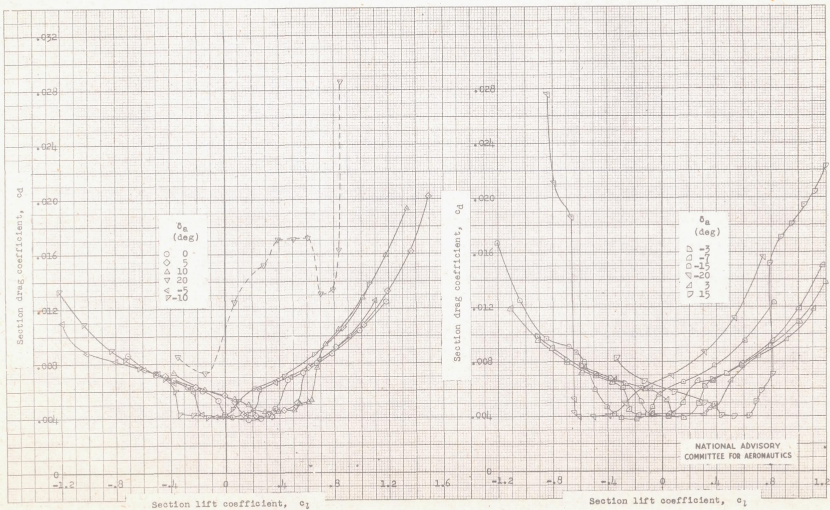
Figure 8 .- Drag characteristics of an NACA 65(112)-213 airfoil section equipped with a sealed 0.22c internally balanced aileron of modified contour. R = 8 \times 10^6 ; smooth condition; test, TDT 701.
