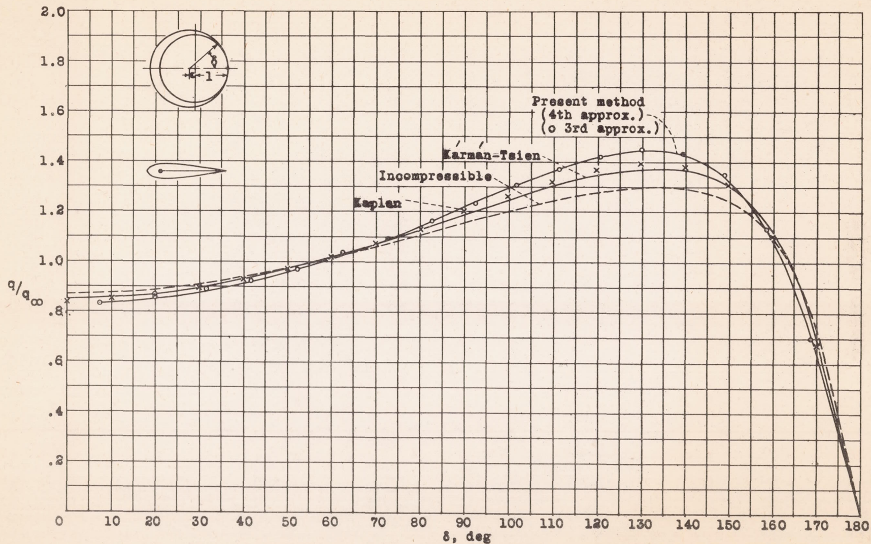
Figure 2.- Velocity distribution along a Joukowski profile ( c = .15 , M_\infty = .685 ).
