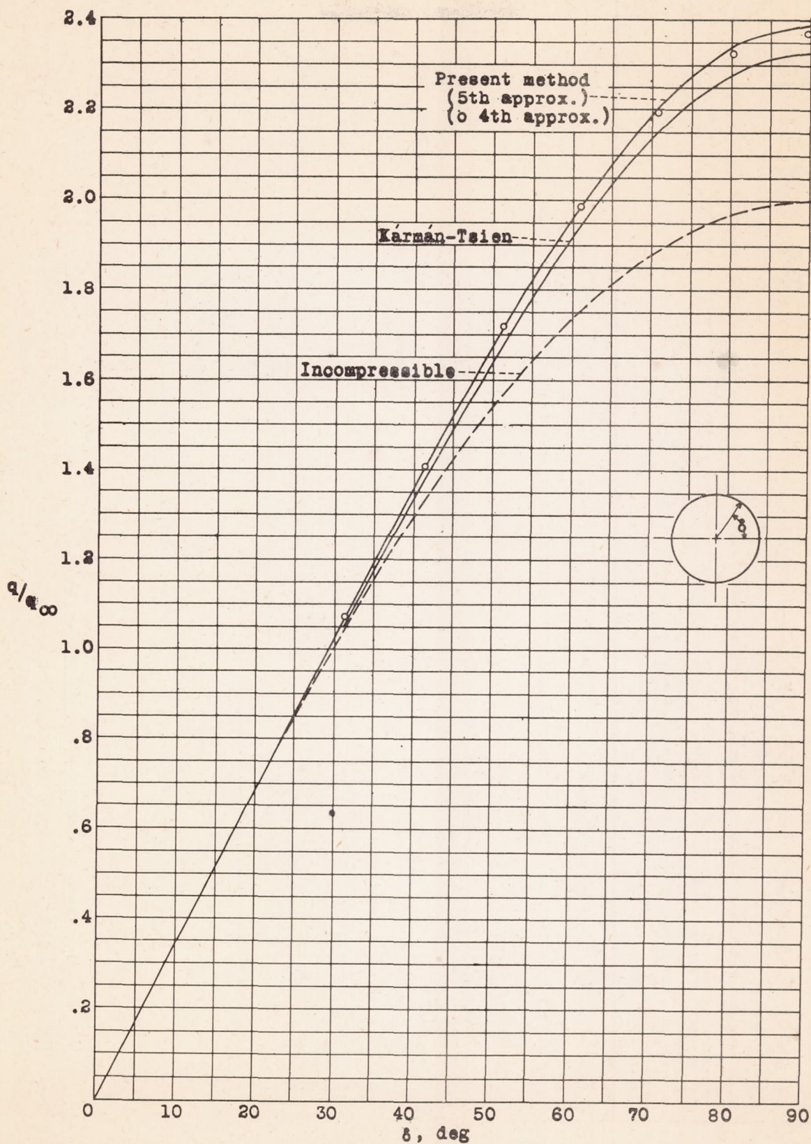
Figure 1.- Velocity distribution along a circle ( M_\infty = 0.406 ).
