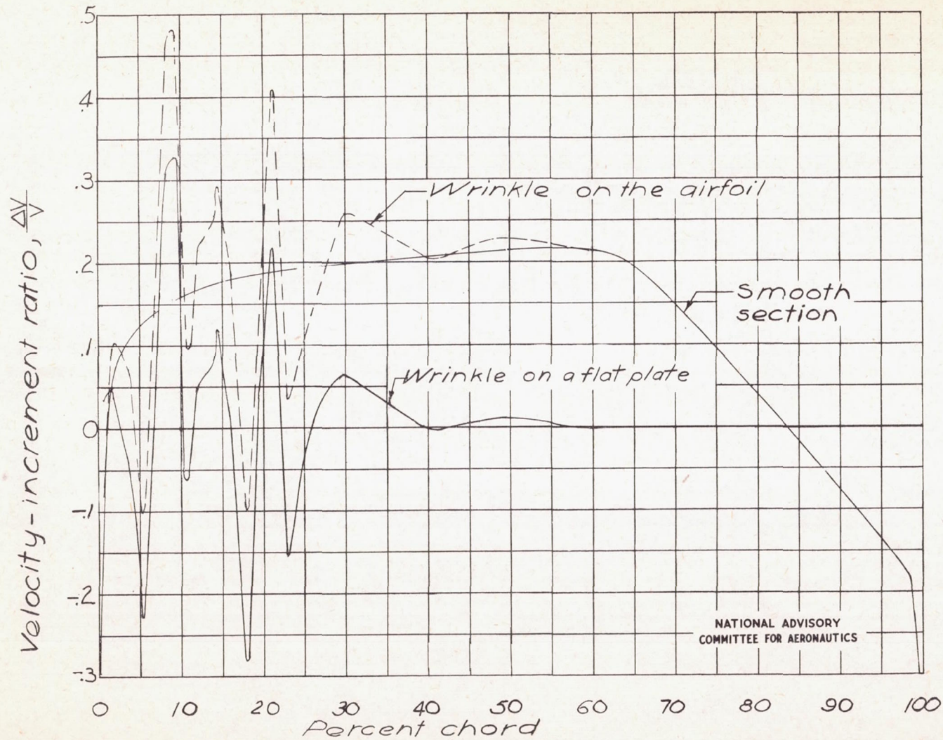
Figure 19. - Theoretical velocity distribution over the upper surface of the smooth NACA 66,1-115 airfoil ( \alpha=0^\circ , M=0.250 ) and over the wrinkle on a flat plate and on the airfoil ( \alpha=0^\circ ).
