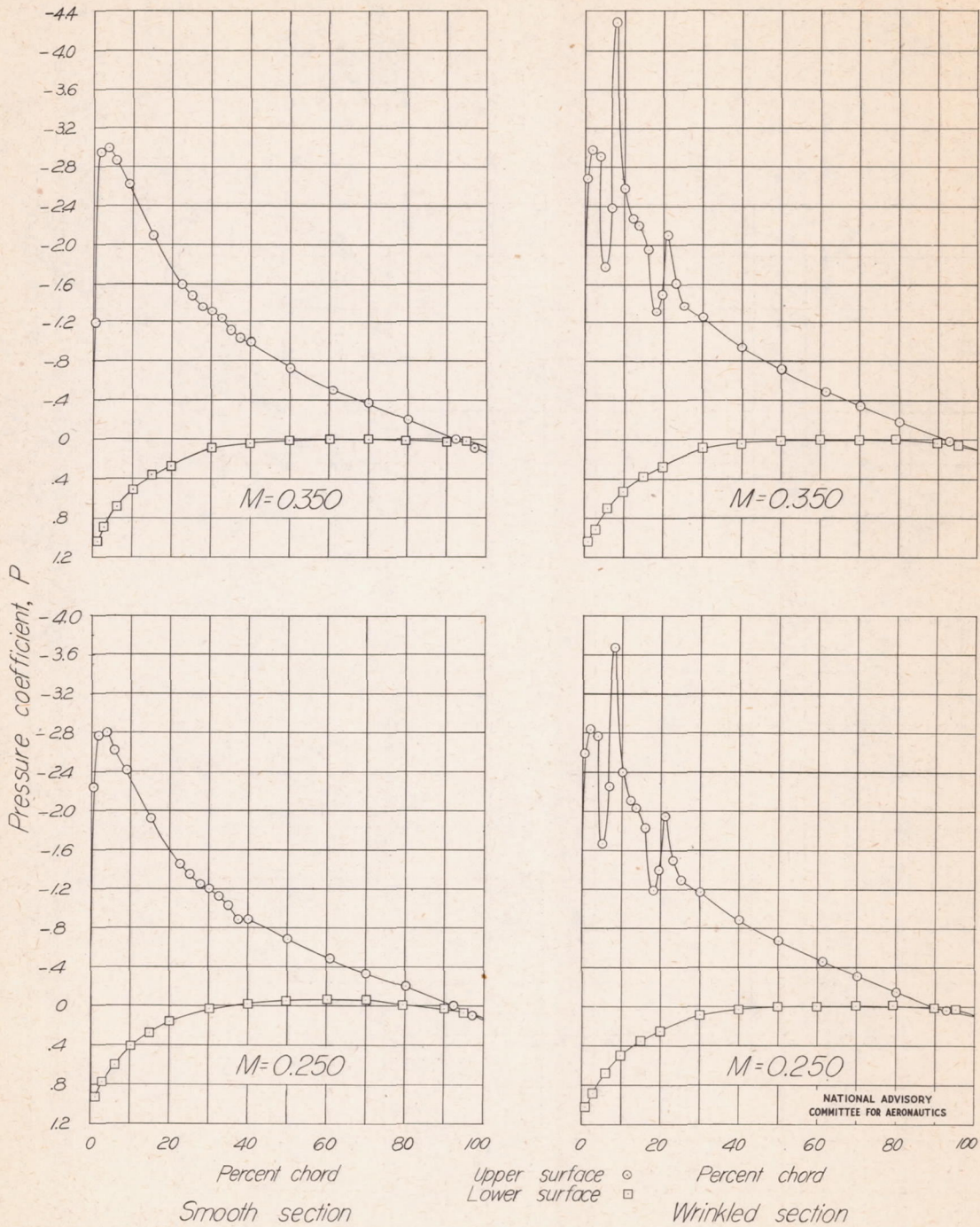
Figure 18.-Pressure distribution over NACA 23015 airfoil. OC=9^\circ
