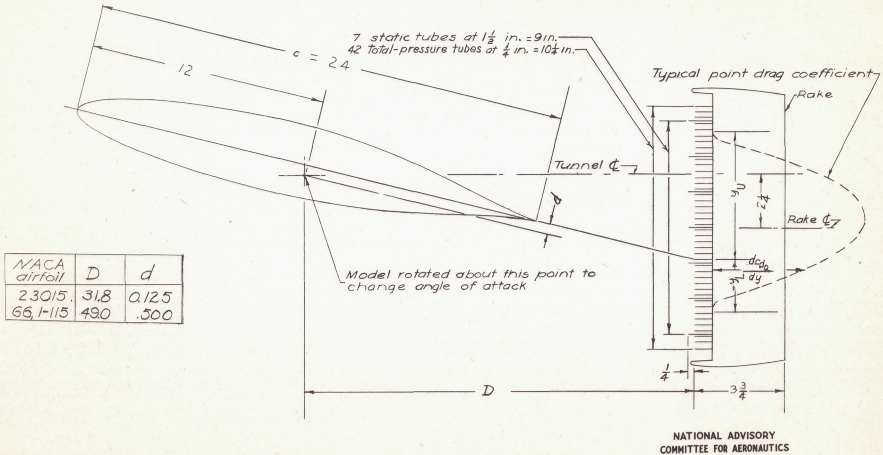
Figure 5.— Schematic diagram of wake-survey apparatus. All dimensions are in inches.
