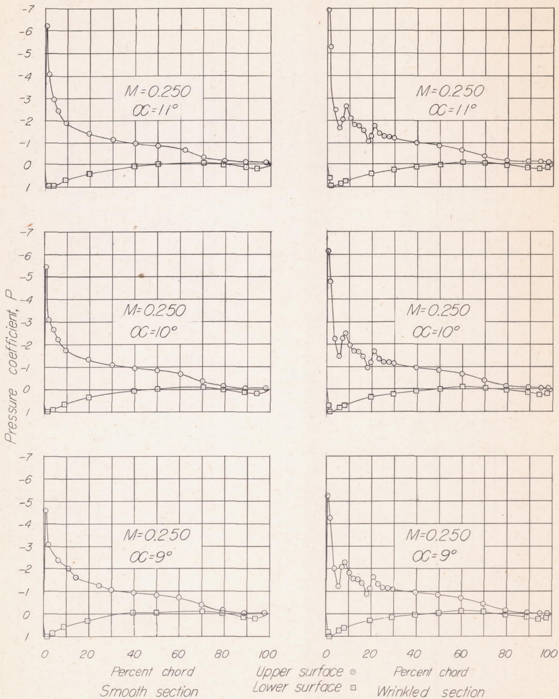
Figure 11.-Pressure distribution over NACA 66,1-115 airfoil. \alpha = 9^\circ, 10^\circ, \text{ and } 11^\circ
