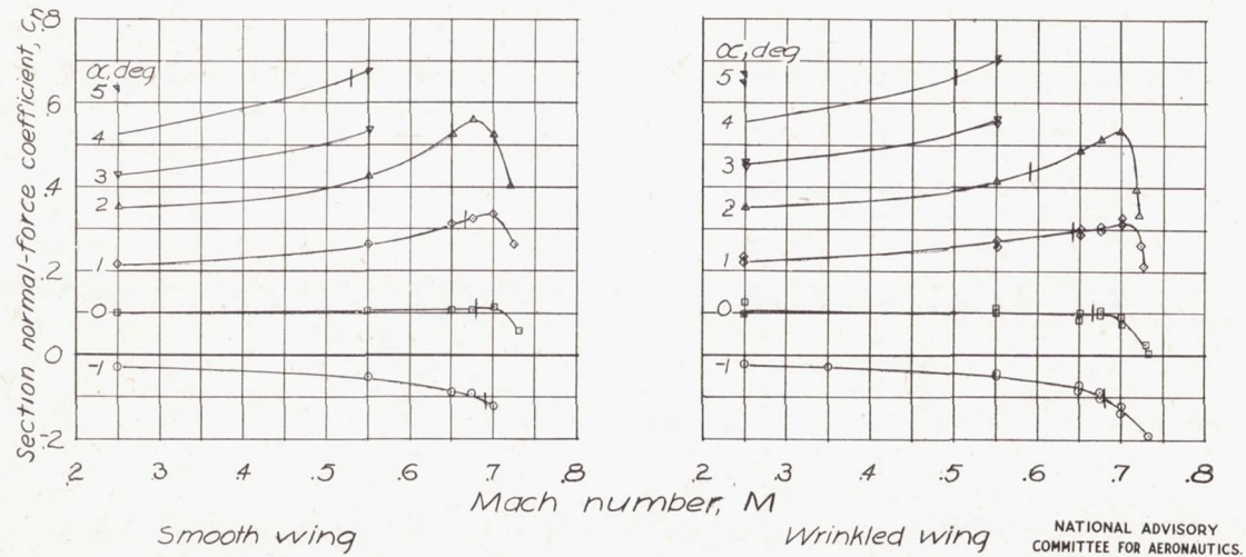
Figure 21. - Variation of normal-force coefficient with Mach number. NACA 66,1-115 airfoil. (Ticks indicate the critical speed.)
