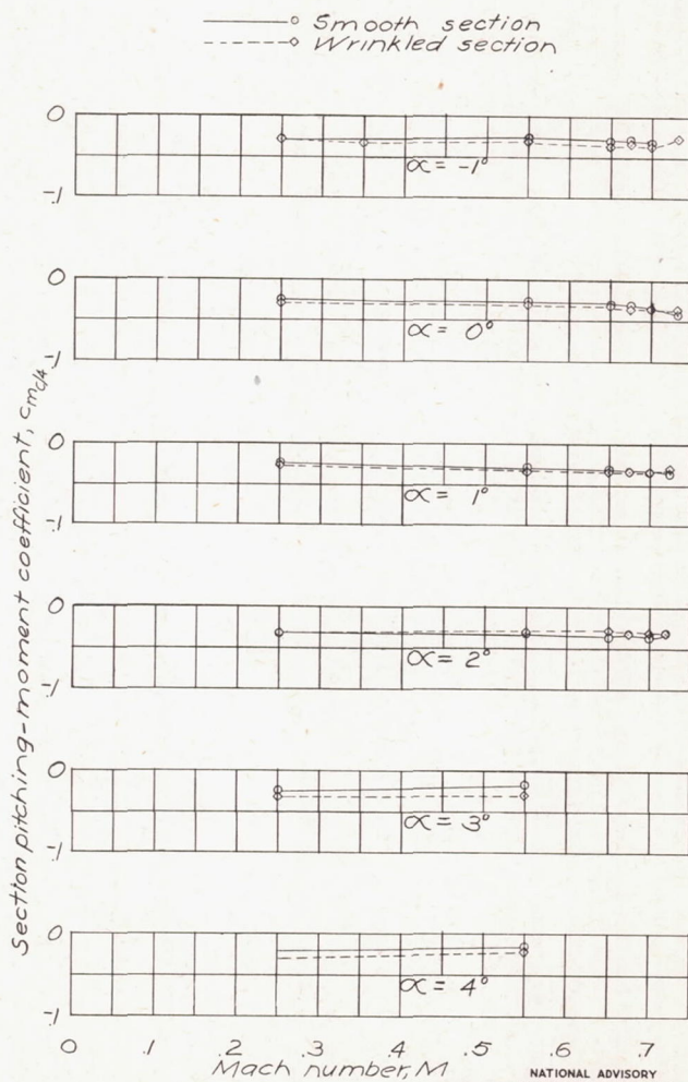
Figure 23.—Variation of section pitching-moment coefficient with Mach number. NACA 661-115 airfoil.
