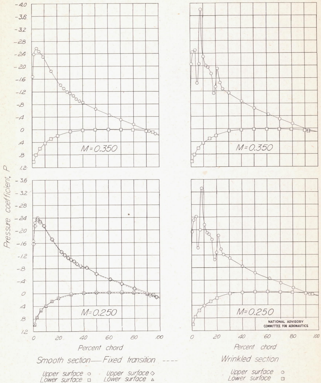
Figure 17.—Pressure distribution over NACA 23015 airfoil. OC=7^\circ
