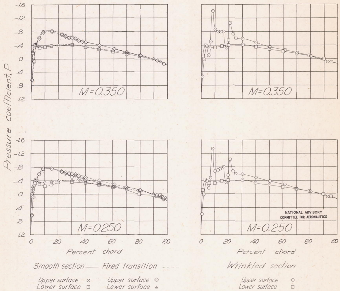
Figure 14.-Pressure distribution over NACA 23015 airfoil. OC=0^\circ .
