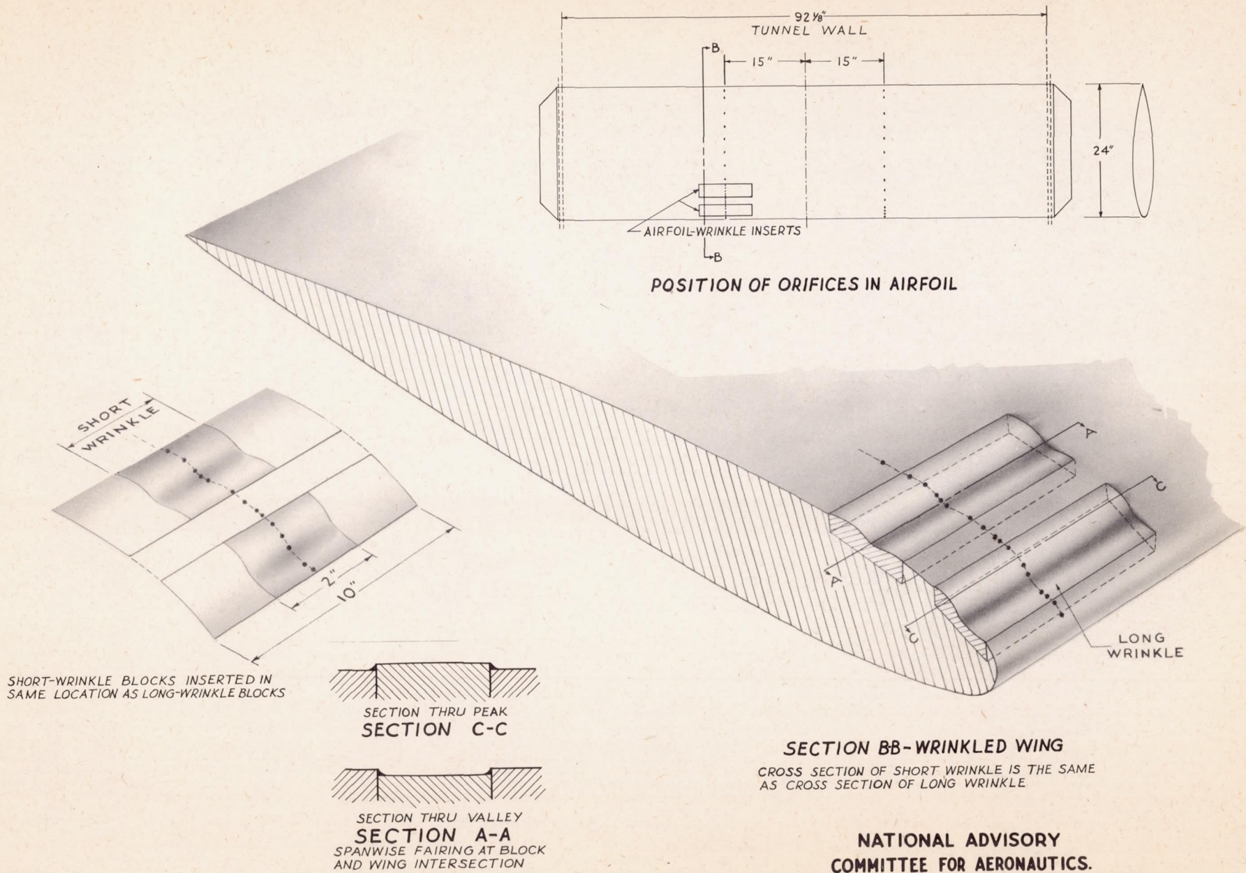
FIGURE 3.- WRINKLE LOCATION AND DETAILS.
