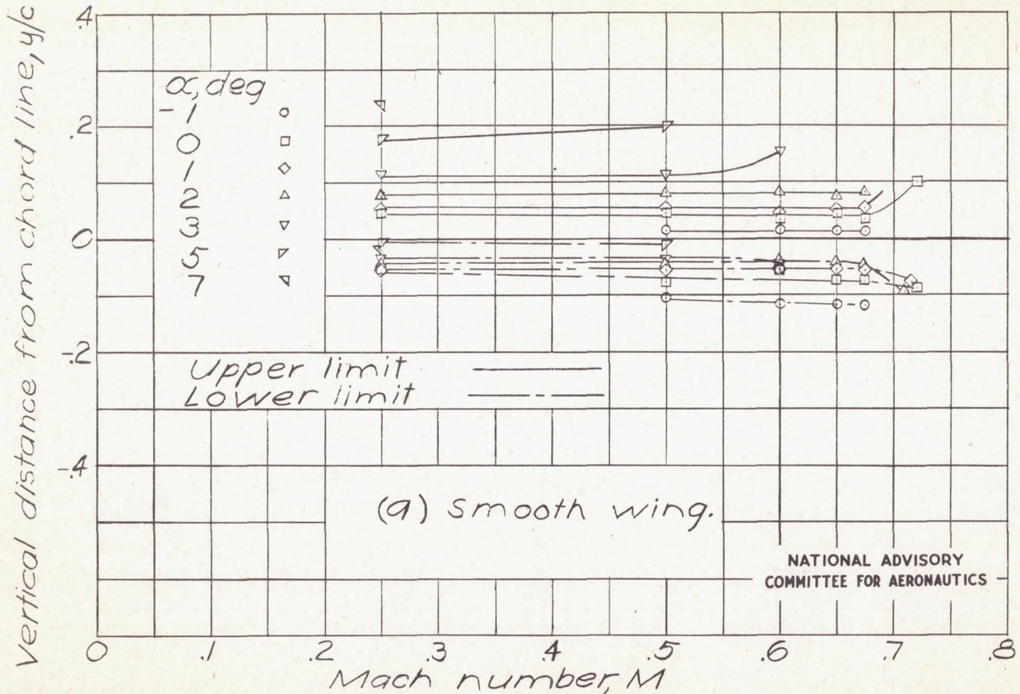
Figure 28. - Wake location 1.54 chords behind trailing edge of NACA 66,1-115 airfoil.
