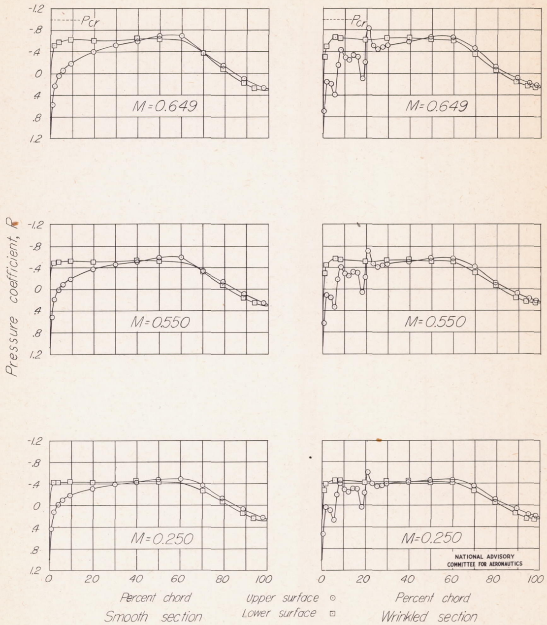
Figure 6. -Pressure distribution over NACA 66,1-115 airfoil. \alpha = -1^\circ
