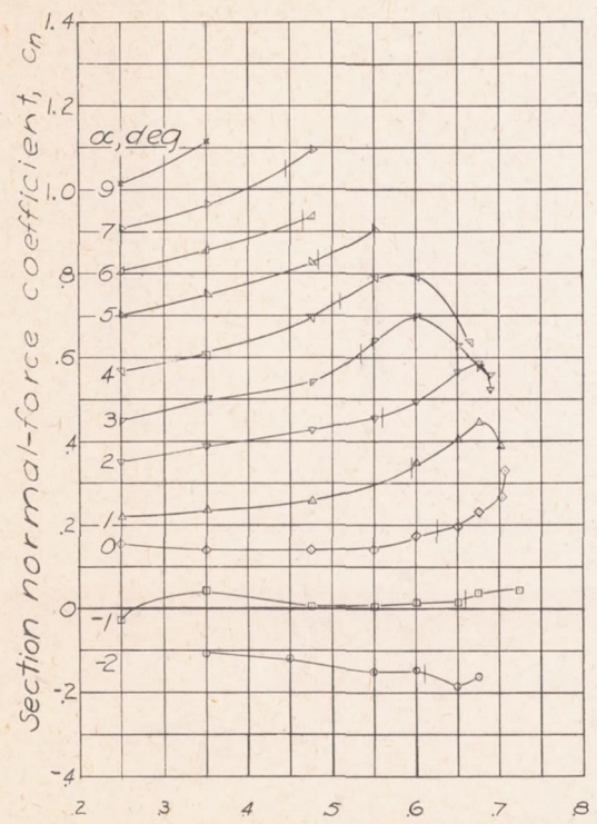
Smooth wing Figure 22. - Variation of section normal-force coefficient with Mach number. NACA 23015 airfoil. (Ticks indicate the critical speed) Wrinkled wing Transition fixed at 0.021 chord on upper surface
