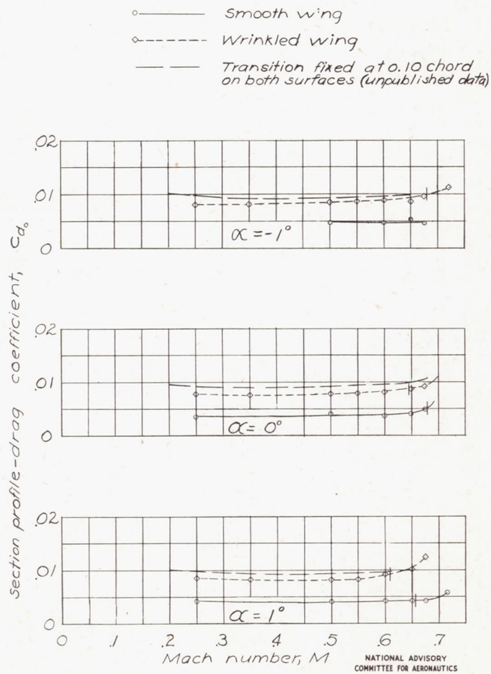
Figure 25. - Variation of section profile-drag coefficient with Mach number. NACA 66,1-115 airfoil. (Ticks indicate the critical speed.)
