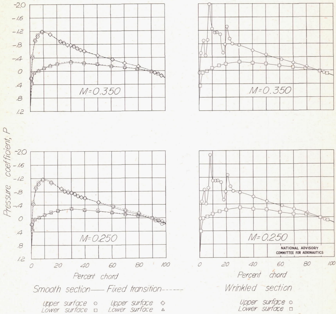
Figure 15.—Pressure distribution over NACA 23015 airfoil. \alpha=2^\circ
