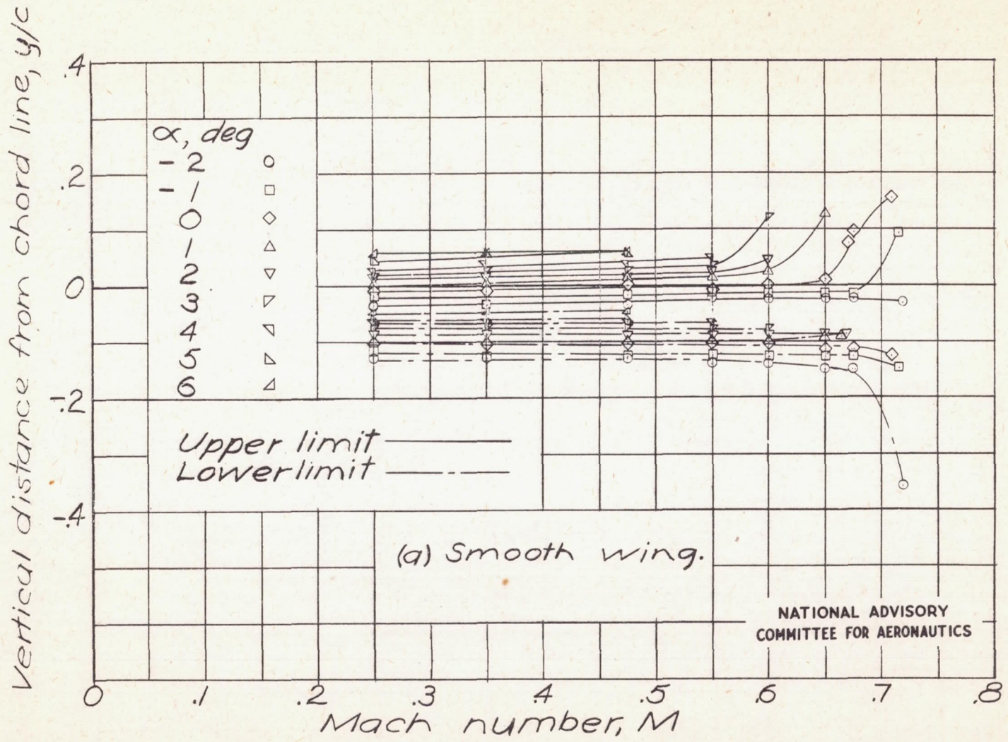
Figure 29. - Wake location 0.826 chord behind trailing edge of NACA 23015 airfoil.
