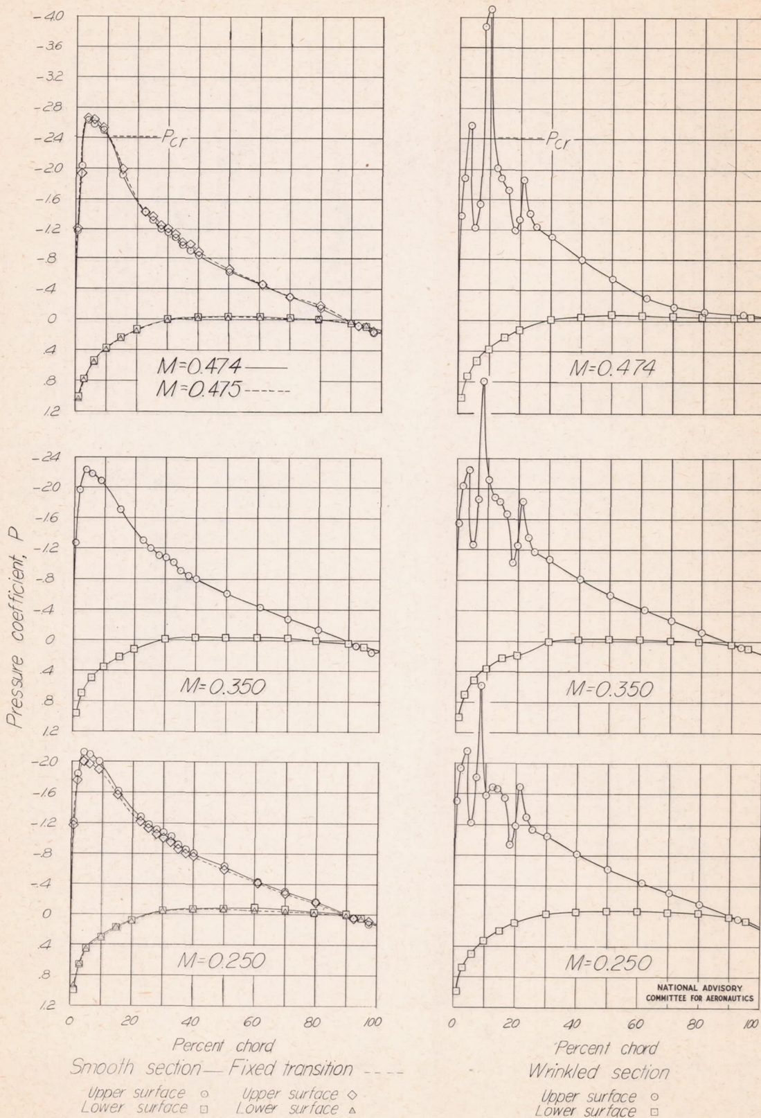
Figure 16. - Pressure distribution over NACA 23015 airfoil. \alpha = 6^\circ
