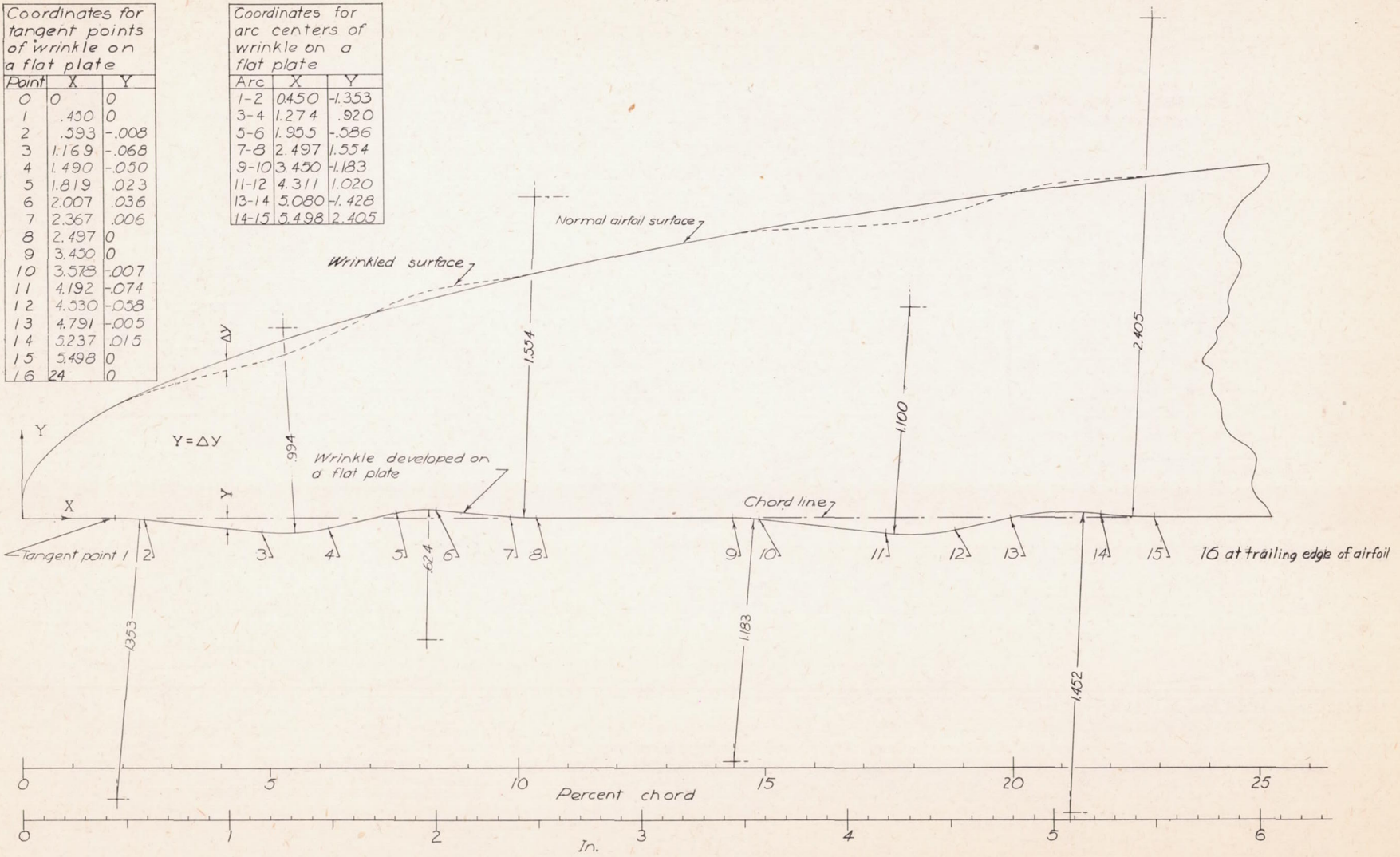
Figure 4.- Upper leading edge of the NACA 661-115 airfoil and dimensions of the wrinkle used for the theoretical pressure distribution. All dimensions are in inches unless otherwise noted.
