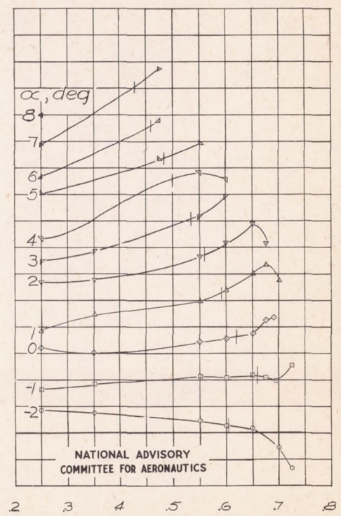
Smooth wing Figure 22. - Variation of section normal-force coefficient with Mach number. NACA 23015 airfoil. (Ticks indicate the critical speed) Wrinkled wing Transition fixed at 0.021 chord on upper surface
