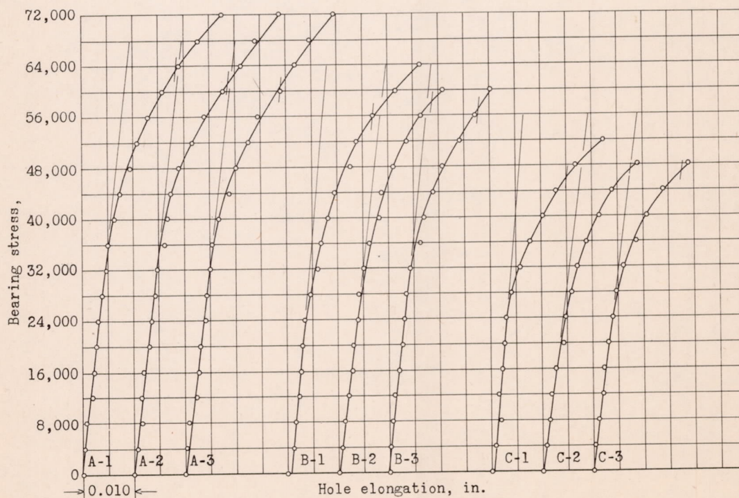
Figure 2.- Bearing stress - hole elongation curves for magnesium alloy castings, 260-T4.
