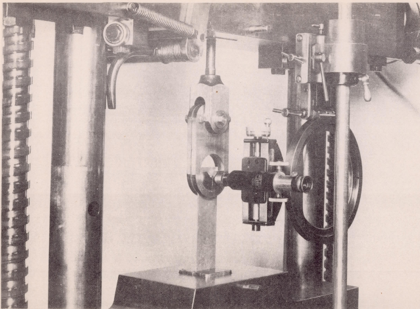
Figure 1.- Arrangement for bearing tests. Pin supports slotted vertically under pin to permit viewing hole deformation.
