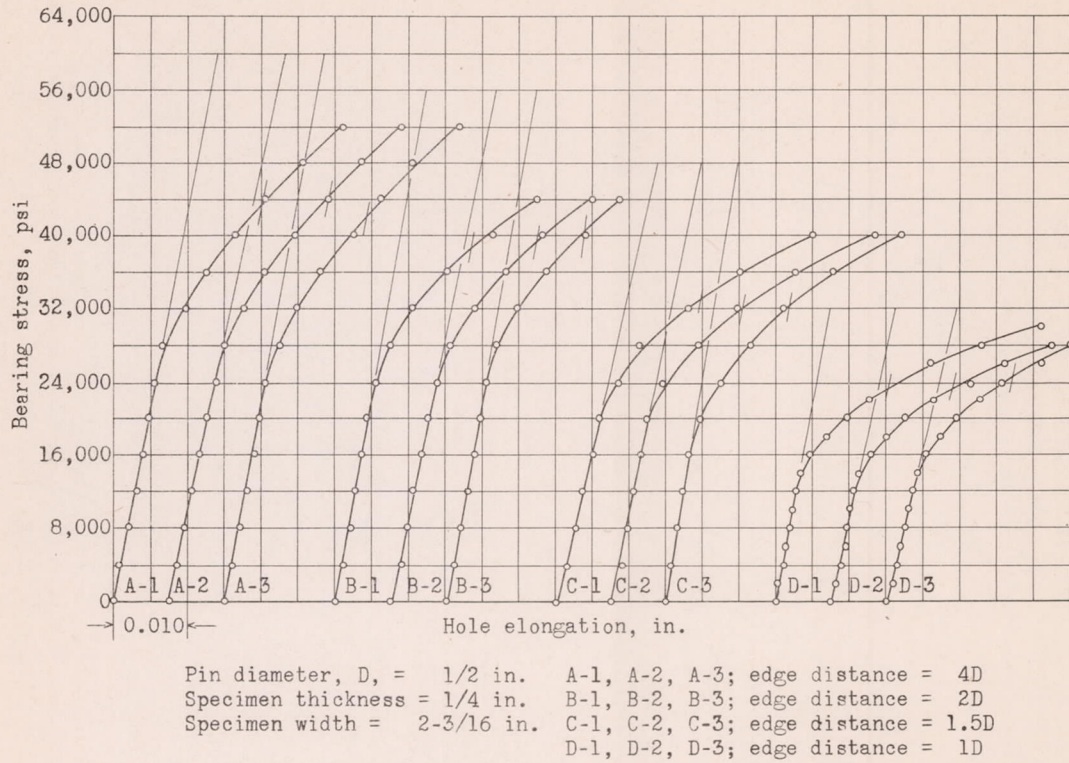
Figure 4.- Bearing stress - hole elongation curves for magnesium alloy castings, 265-T4.
