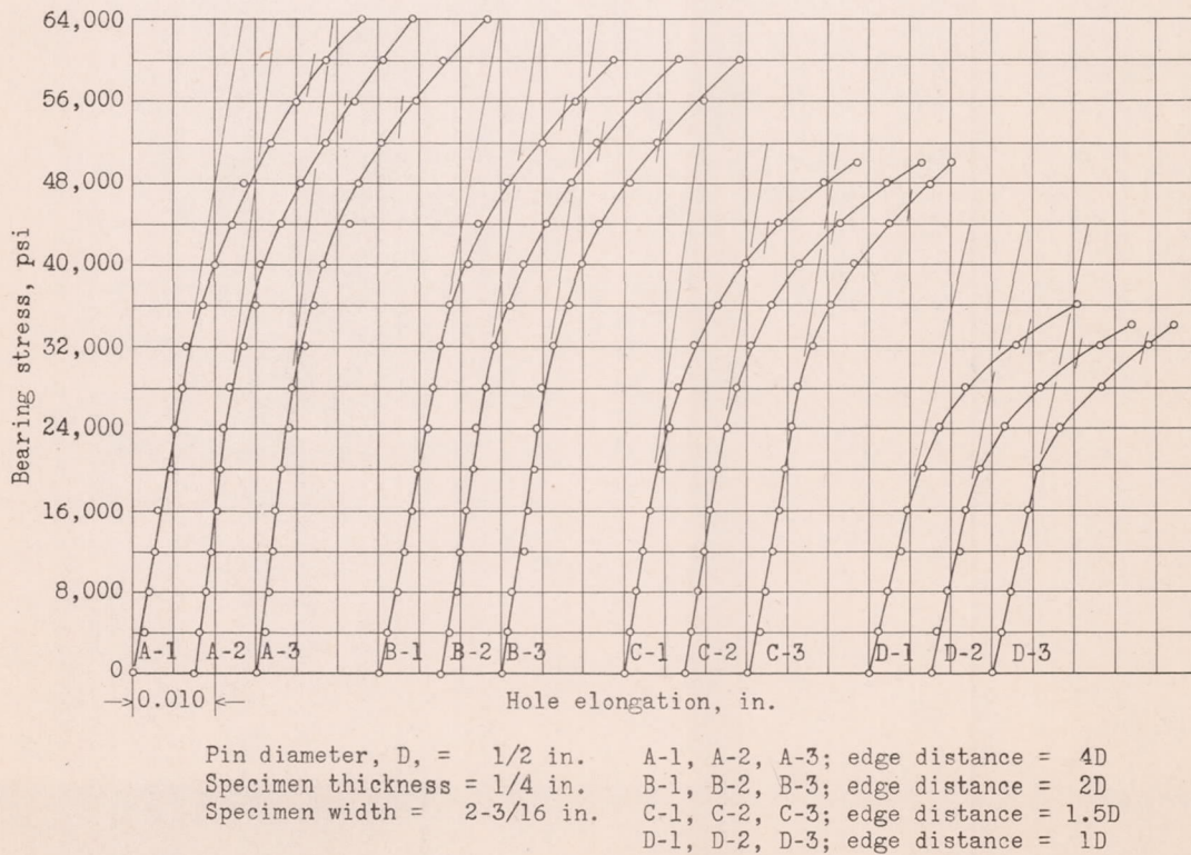
Figure 5.- Bearing stress - hole elongation curves for magnesium alloy castings, 265-T6.
