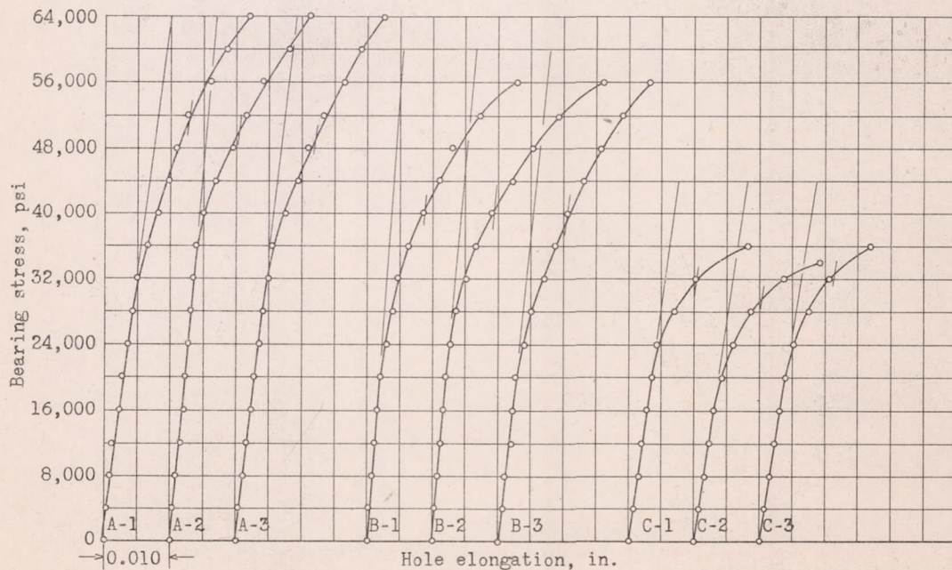
Figure 6.- Bearing stress - hole elongation curves for magnesium alloy castings, 403-C.
