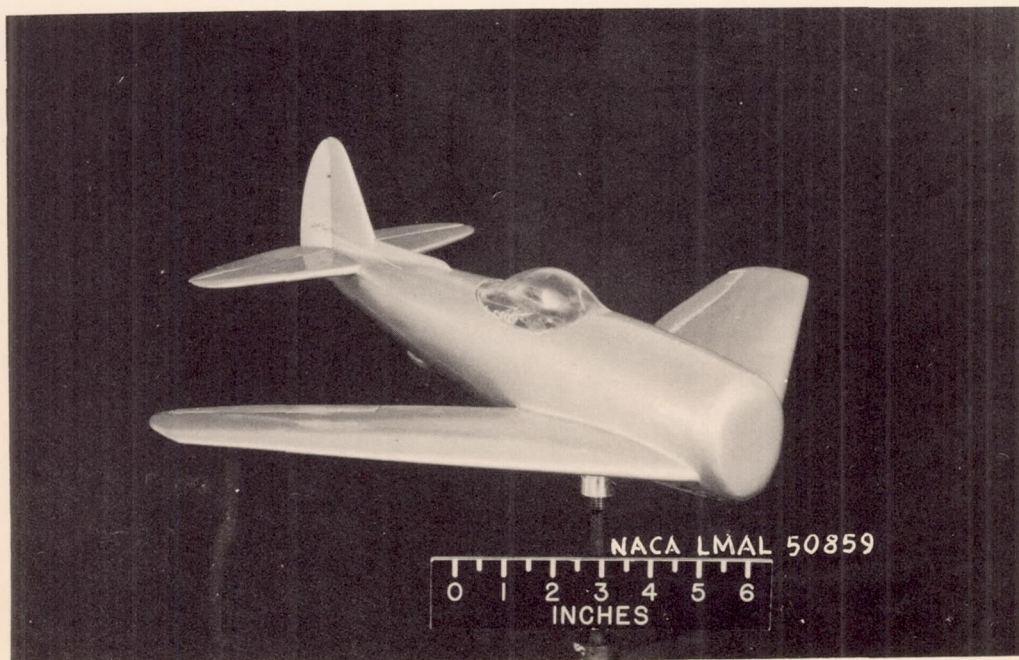
Figure 2.- Photographs of the model with the 0° swept-back wing (top) and of the model with the 40° swept-back wing (bottom).
