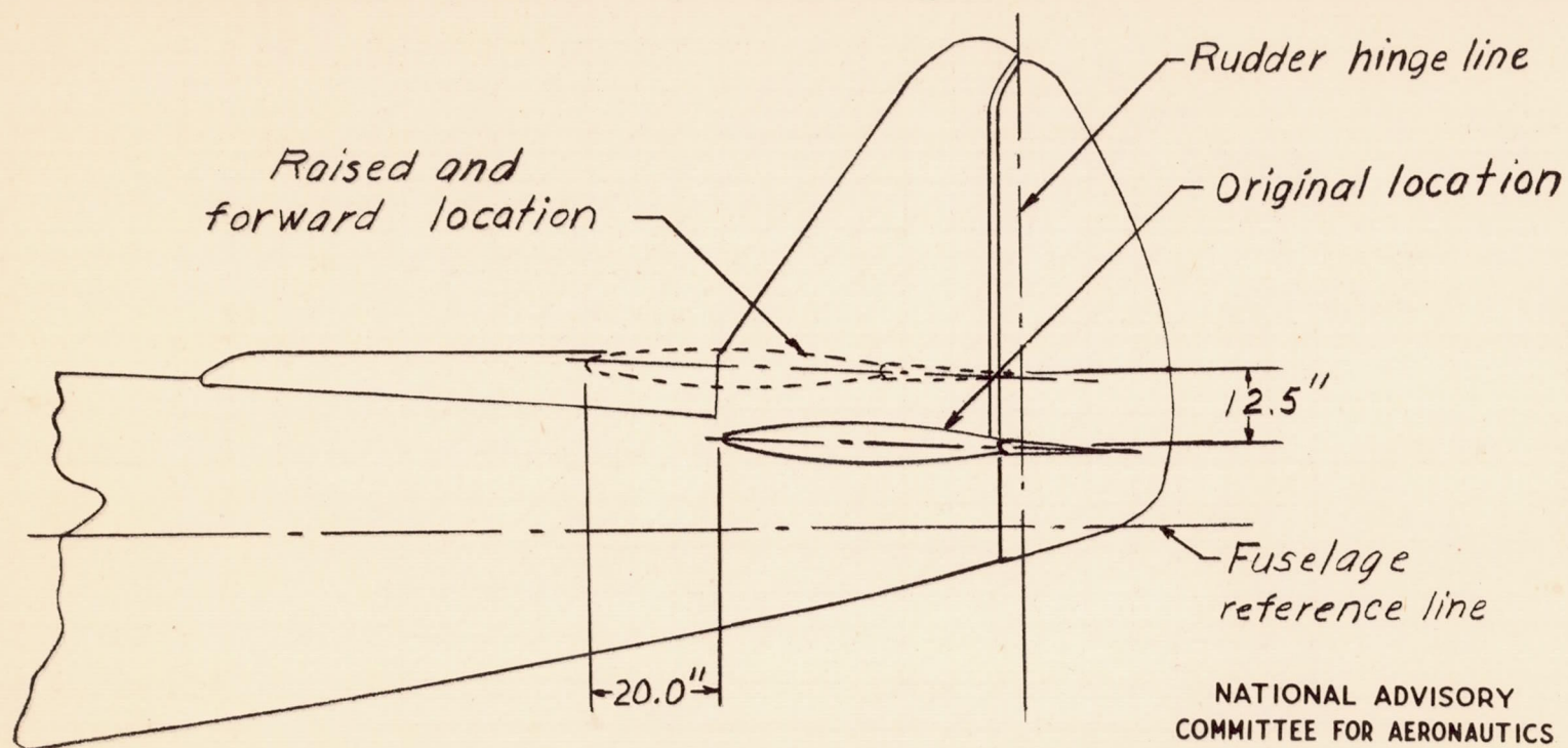
Figure 4.- Sketch showing the two locations of the horizontal tail tested on the model. (Dimensions are full scale.)
