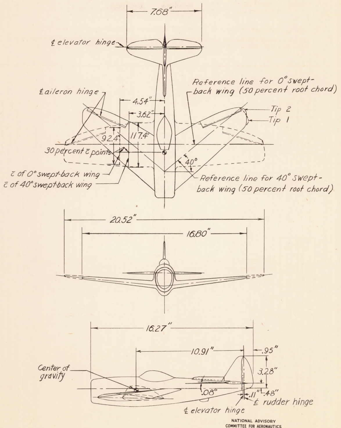
Figure 1.- Three-view drawing of the \frac{1}{25} -scale model of a typical fighter-type airplane. Center of gravity is shown for the basic loading condition.
