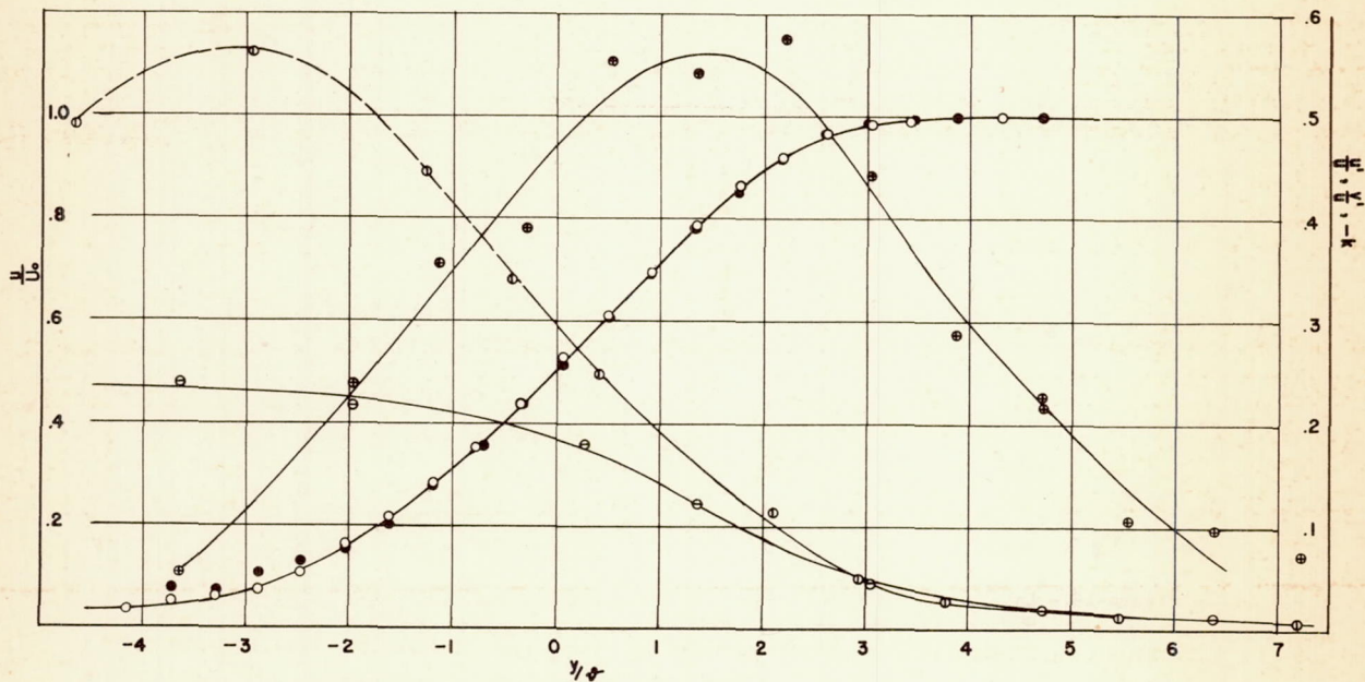
Figure 17.- Lateral distribution of mean and fluctuating velocities and correlation coefficient; x = 54.3 centimeters.
