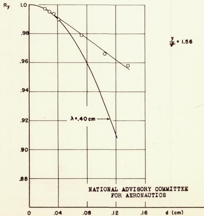
Figure 29.- R_y distribution at x = 90 centimeters.
