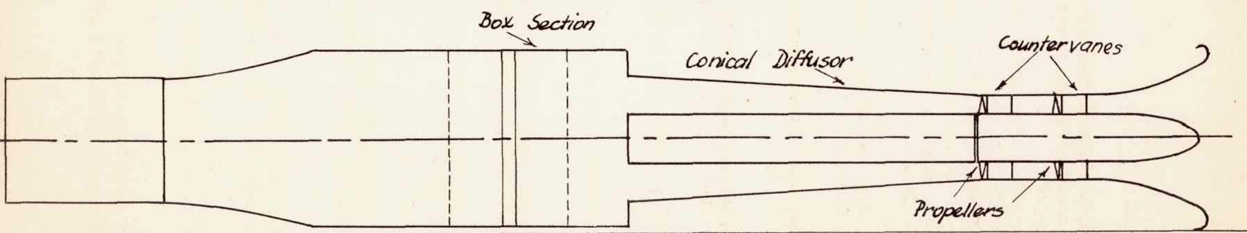
Figure 1.- Flow diagram of the two-dimensional tunnel.
