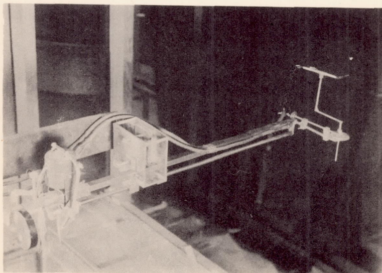
Figure 3.- Traversing mechanism.
