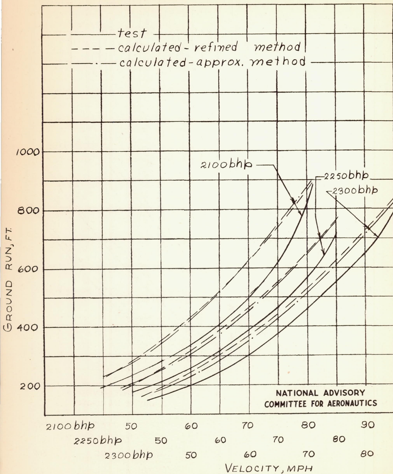
(g) Propeller E at 0.4375 gear ratio
