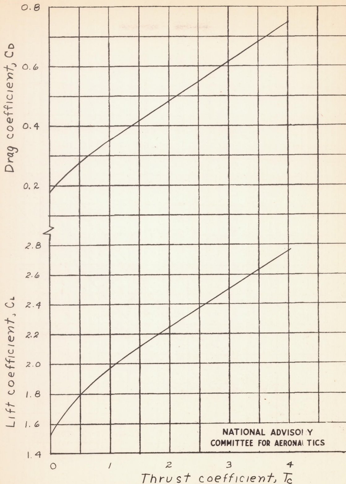
Figure 6.- Variation of lift and drag coefficients with thrust coefficient for the test airplane in the take-off configuration.
