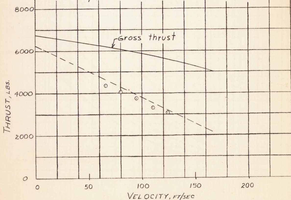
(b) Propeller D at 0.5625 gear ratio Figure 8.— Variation of calculated thrusts with airspeed for the test airplane at take-off power.
