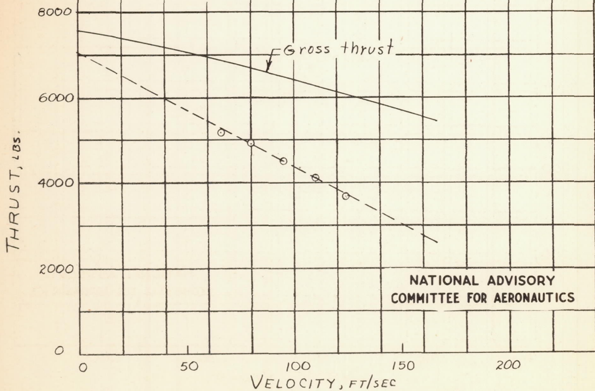
(d) Propeller C at 0.4375 gear ratio Figure 8.- Continued.
