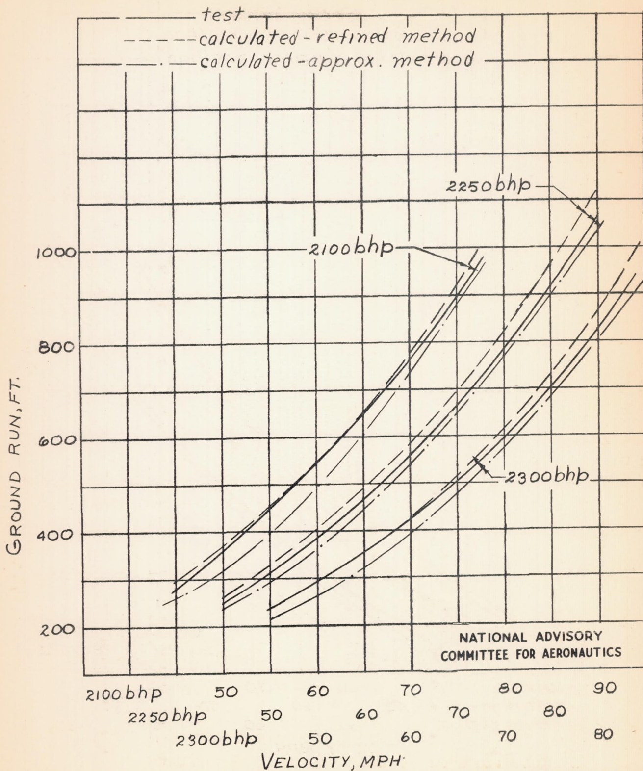
(b) Propeller D at 0.5625 gear ratio. Figure 7. - Continued
