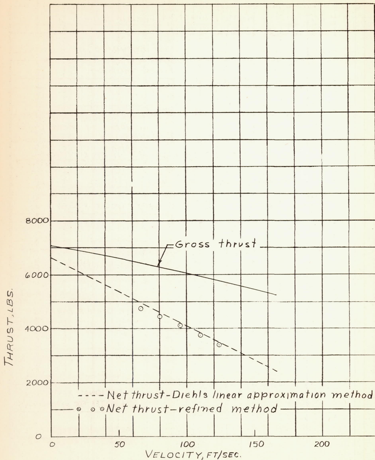
(g) Propeller Bat 0.4375 gear ratio Figure 8.— Concluded.
