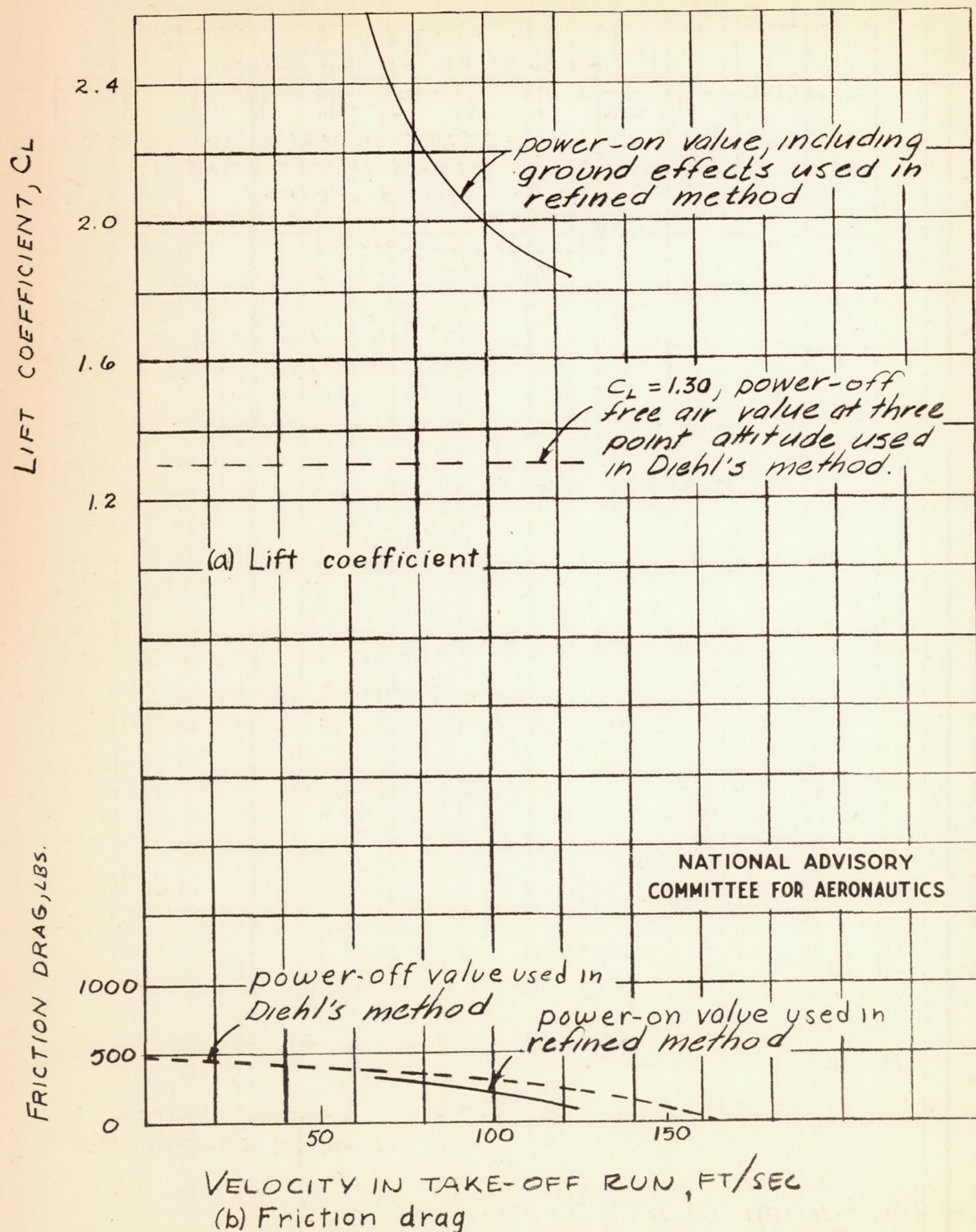
Figure 10.- Variation of lift coefficient and wheel friction drag with velocity in the take-off run.
