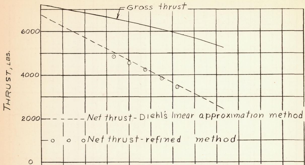
(c) Propeller F, at 0.4375 gear ratio
