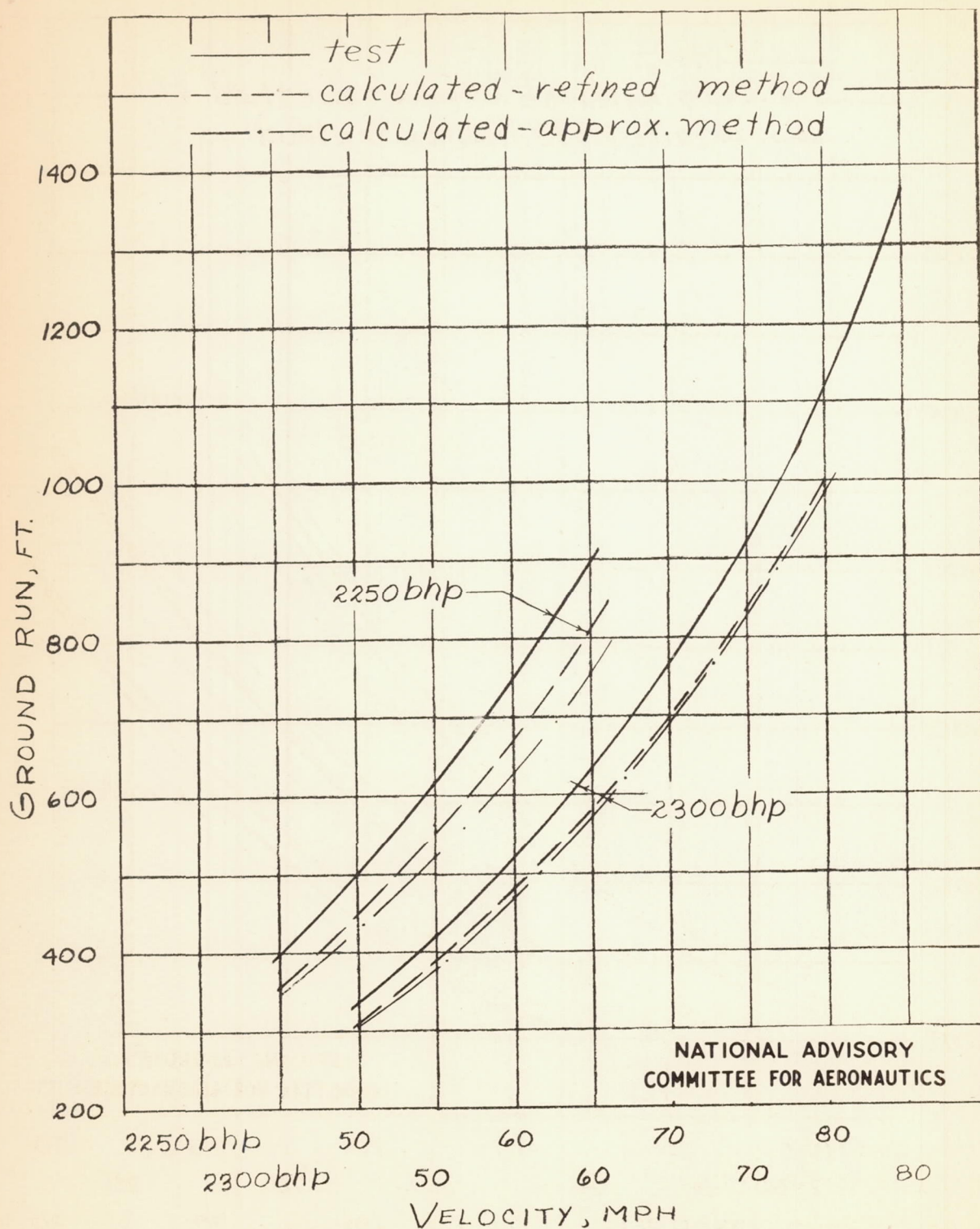
(e) Propeller D at 0.4375 gear ratio Figure 7. — Continued
