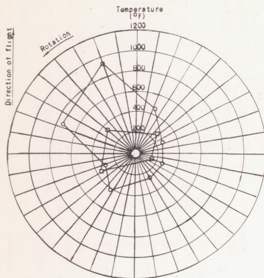
(a) Altitude, 14,600 feet; cruising power; nozzle-exit temperature, 1360^{\circ} F.
