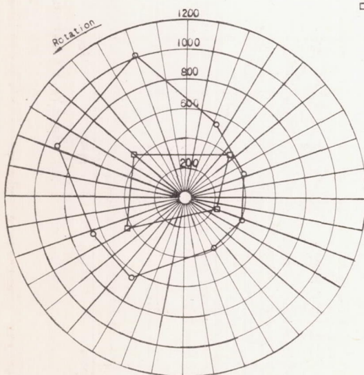
(c) Altitude, 24,000 feet; cruising power; nozzle-exit temperature, 1545^{\circ} F.
