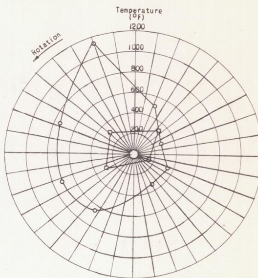
(b) Altitude, 14,600 feet; military power; nozzle-exit temperature, 1520^{\circ} F.
