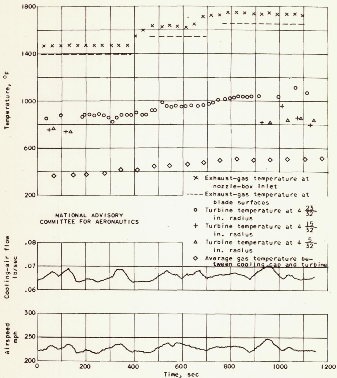
Figure 4. - Typical flight data. (See table I for other flight variables.)
