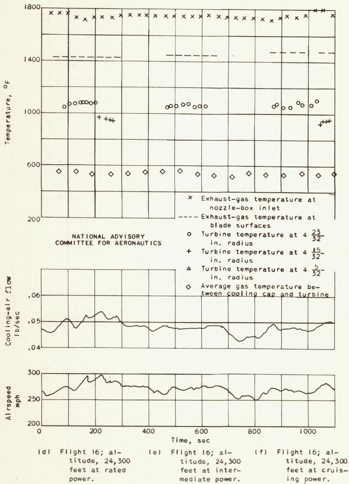
Figure 4. - Concluded. Typical flight data. (See table I for other flight variables.)
