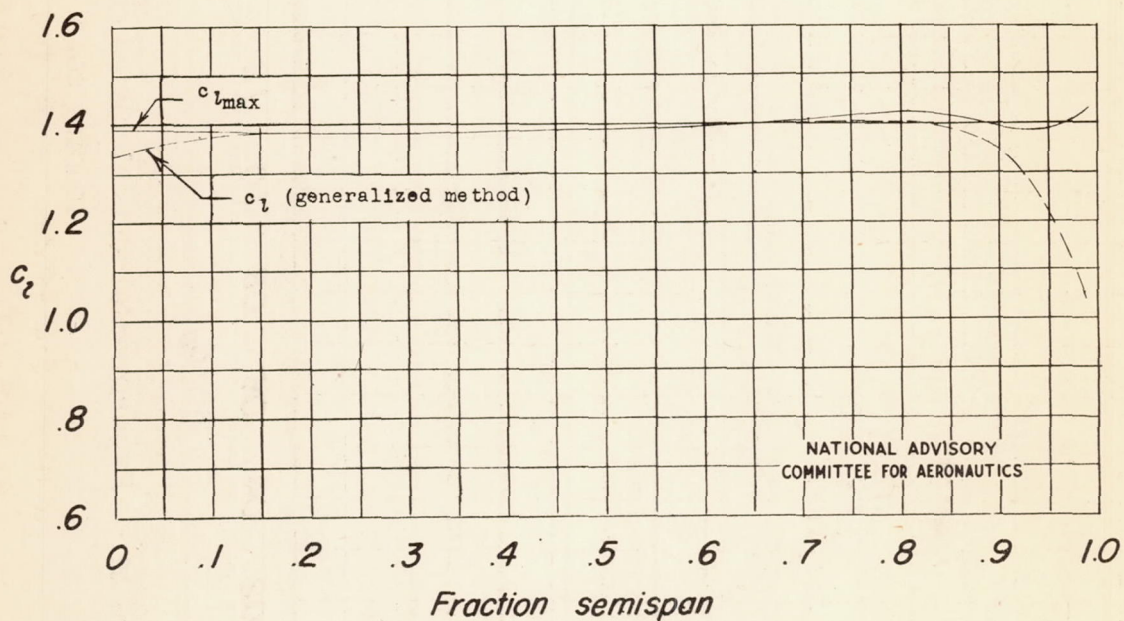
(b) Wing 3.5-12-44,22.1.
