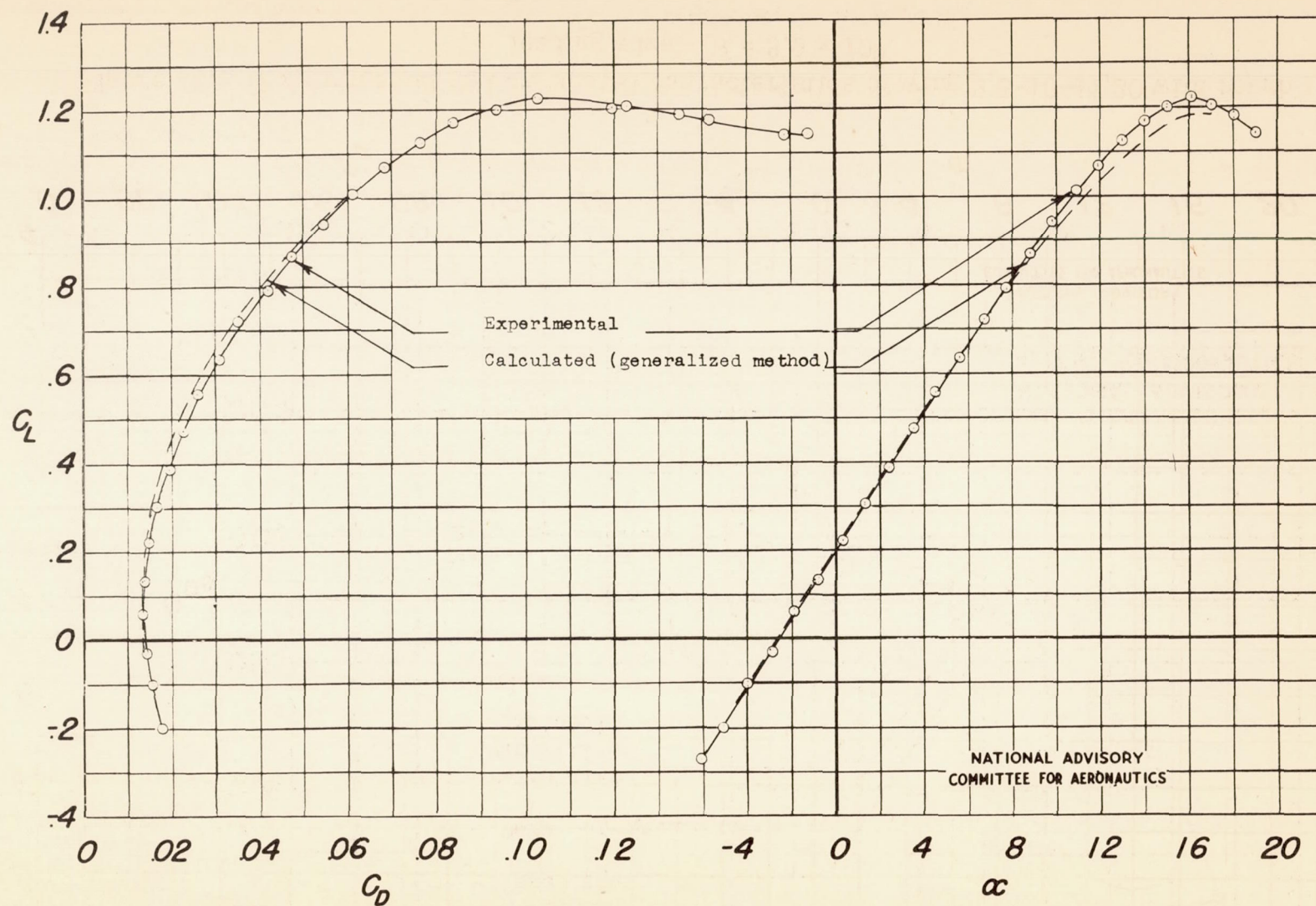
Figure 11.- Experimental and calculated characteristics of wing 2.5-8-44,16 with rough leading edge. R = 3.9 \times 10^6 .
