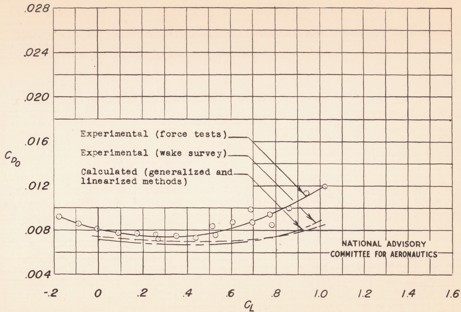
(b) C_{D0} against C_L .
