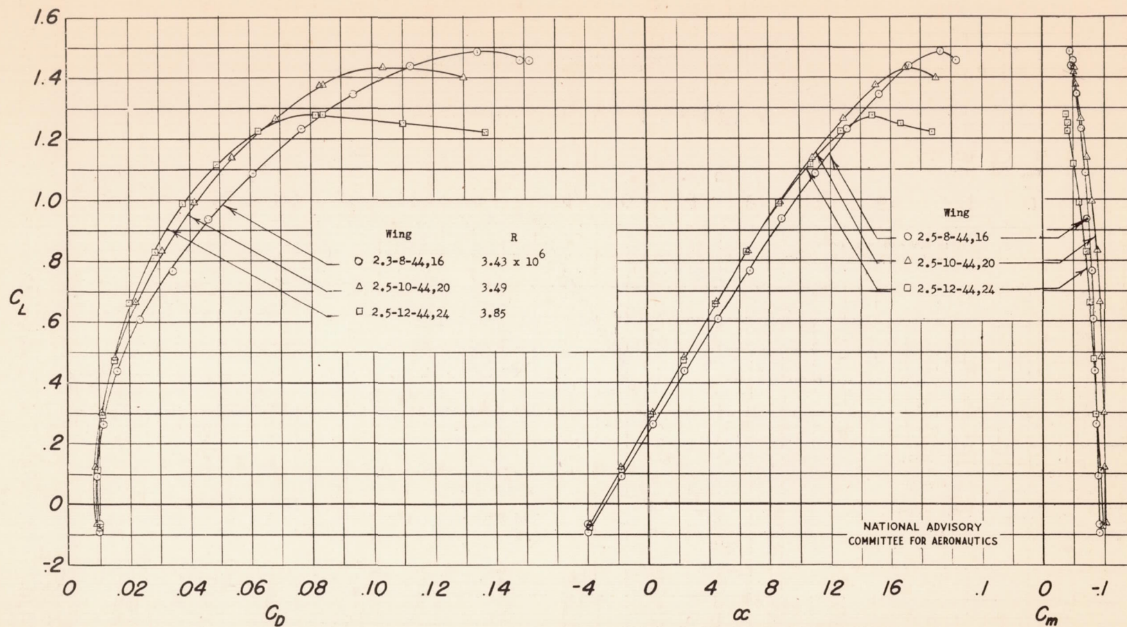
(a) Taper ratio 2.5; R \approx 3.6 \times 10^6 .
