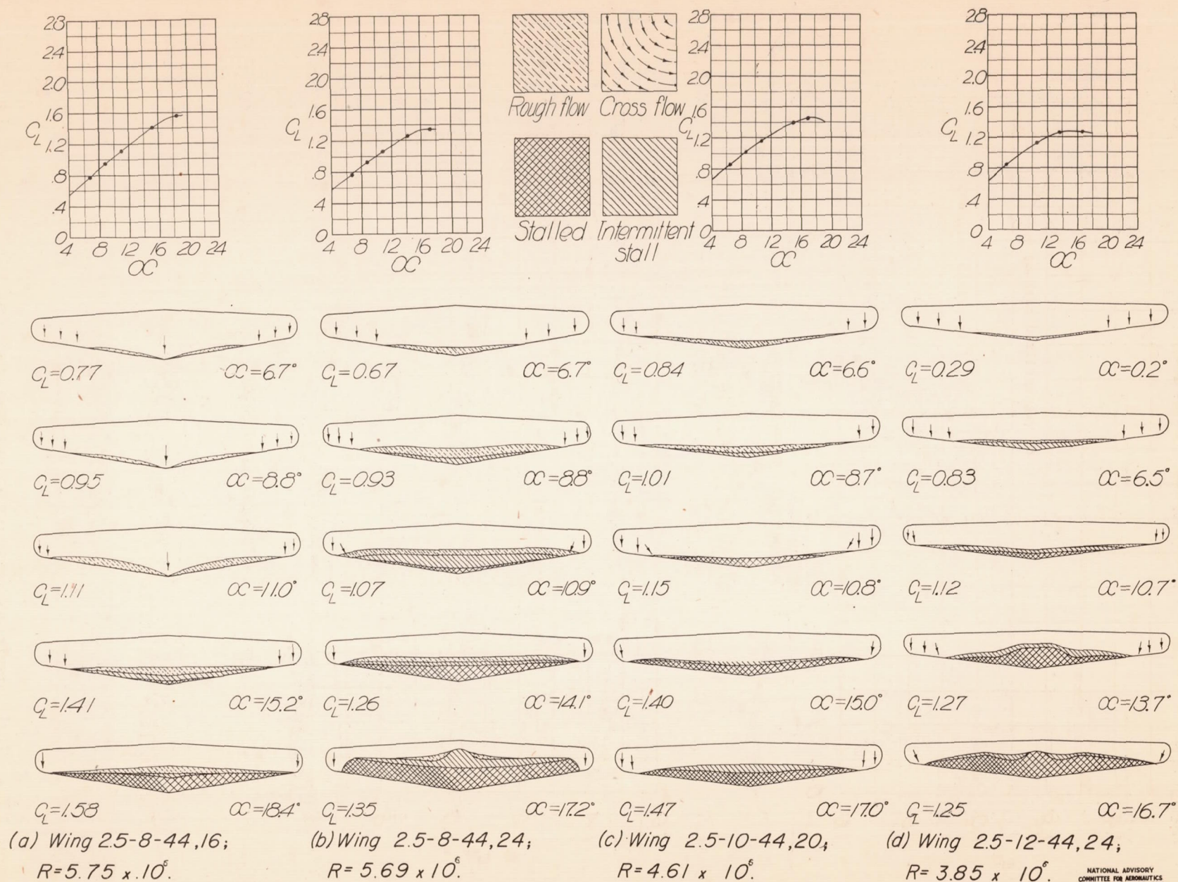
Figure 16.- Stall progression for wings of taper ratio 2.5.
