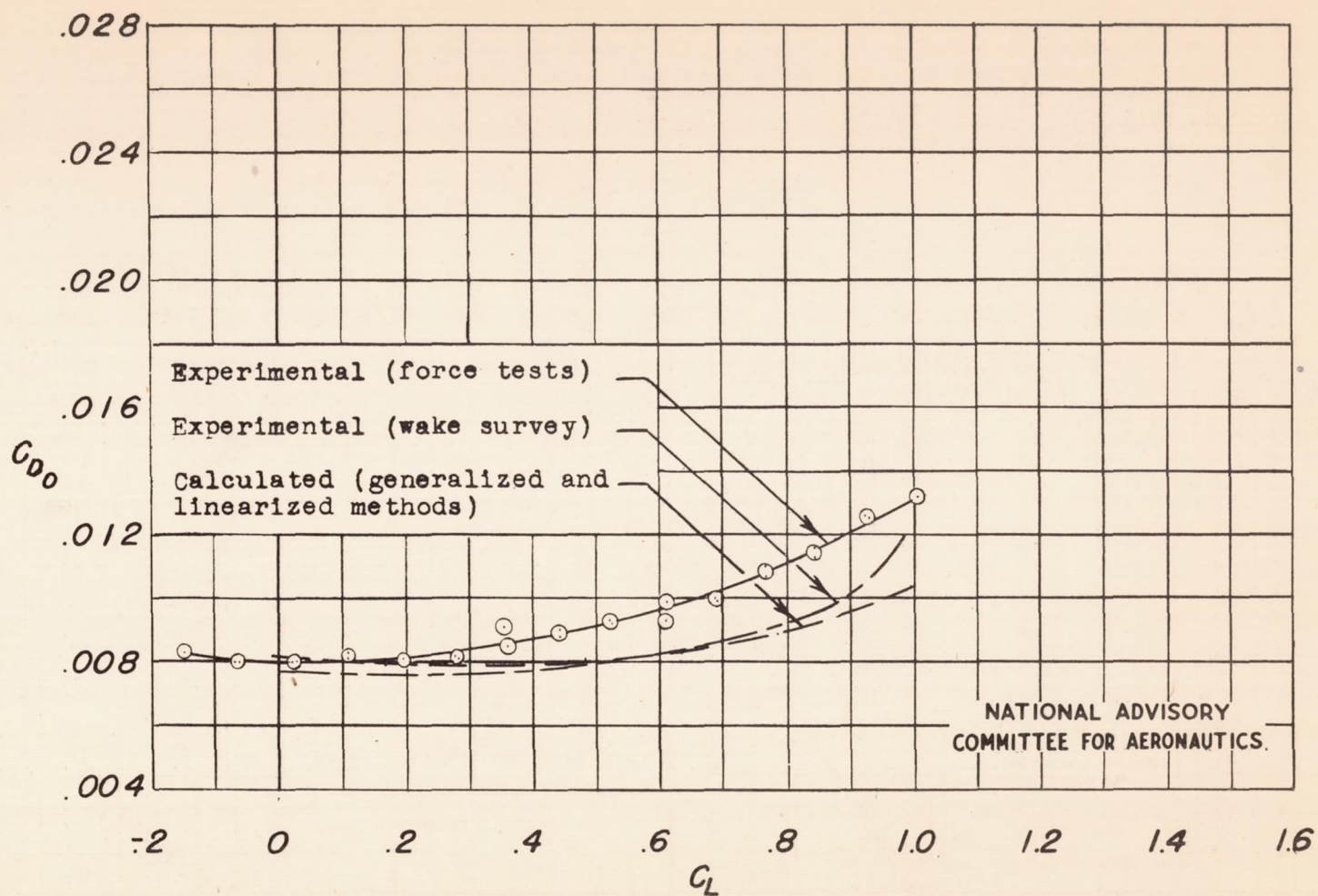
(b) C_{D0} against C_L .
