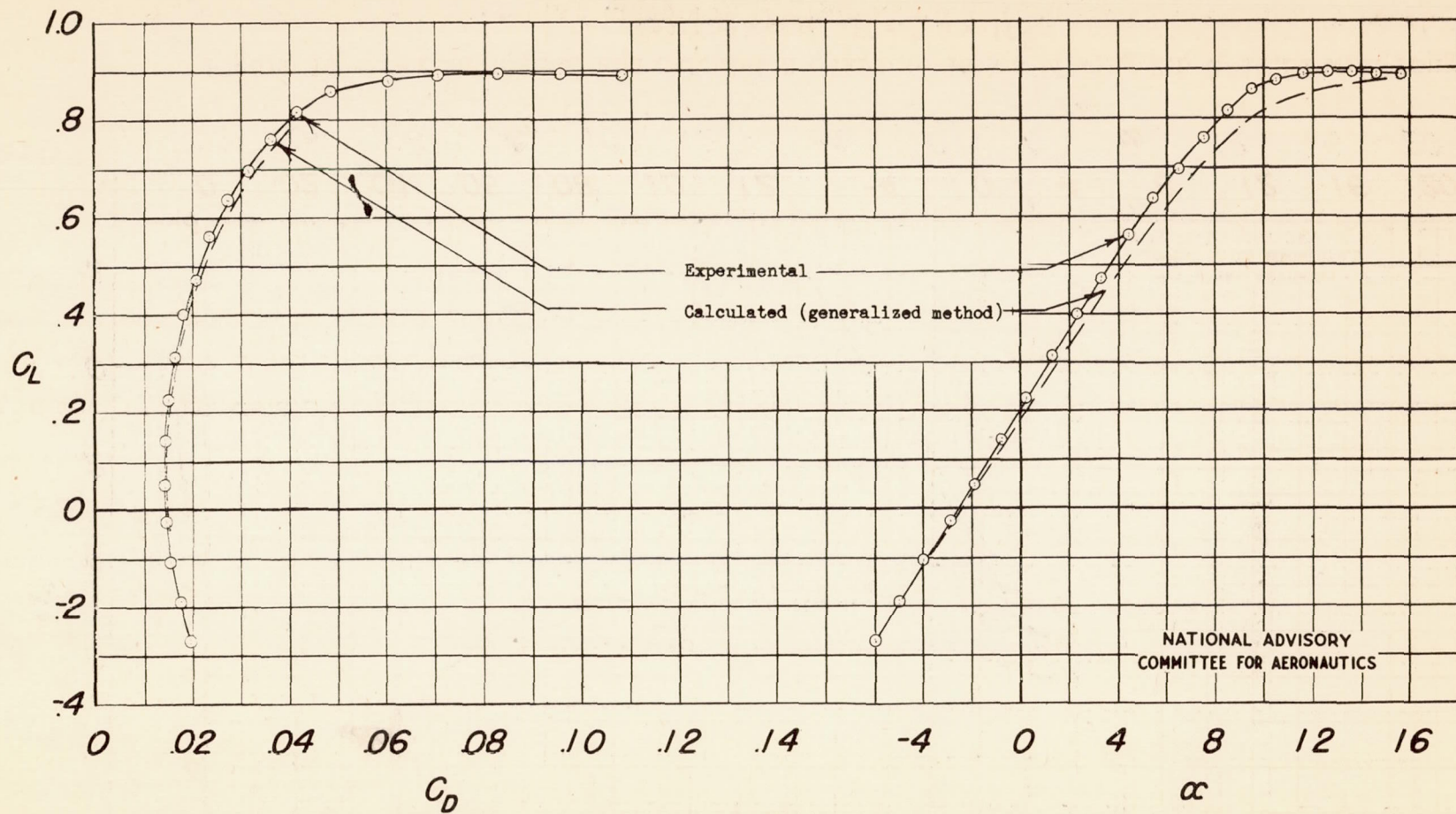
Figure 13.- Experimental and calculated characteristics of wing 2.5-12-44,24 with rough leading edge. R = 3.9 \times 10^6 .
