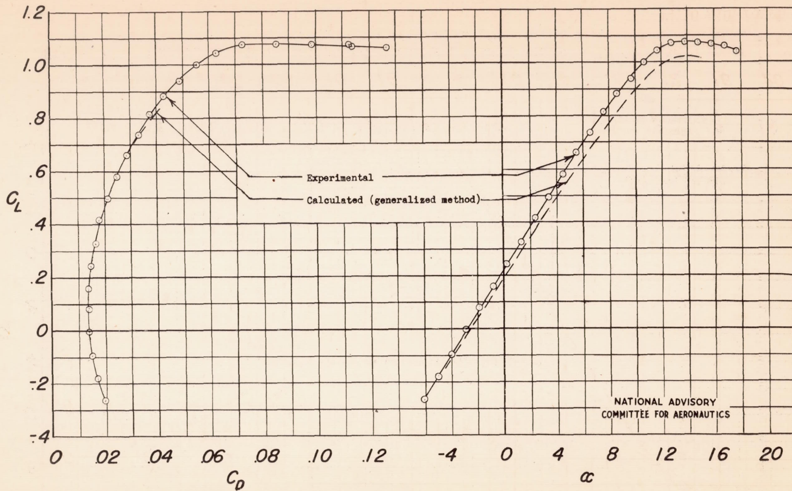
Figure 12.- Experimental and calculated characteristics of wing 2.5-10-44,20 with rough leading edge. R = 3.9 \times 10^6 .
