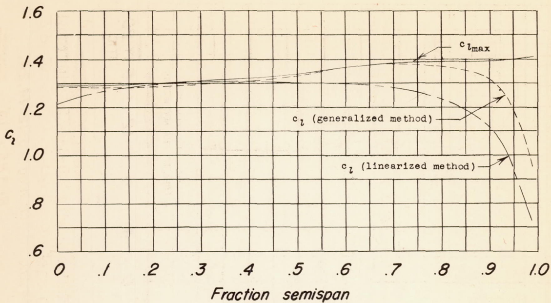
(a) Wing 2.5-12-44,24.
