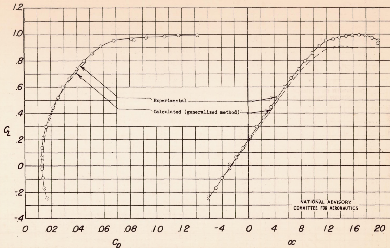
Figure 14.- Experimental and calculated characteristics of wing 2.5-8-44,24 with rough leading edge. R = 3.9 \times 10^6 .
