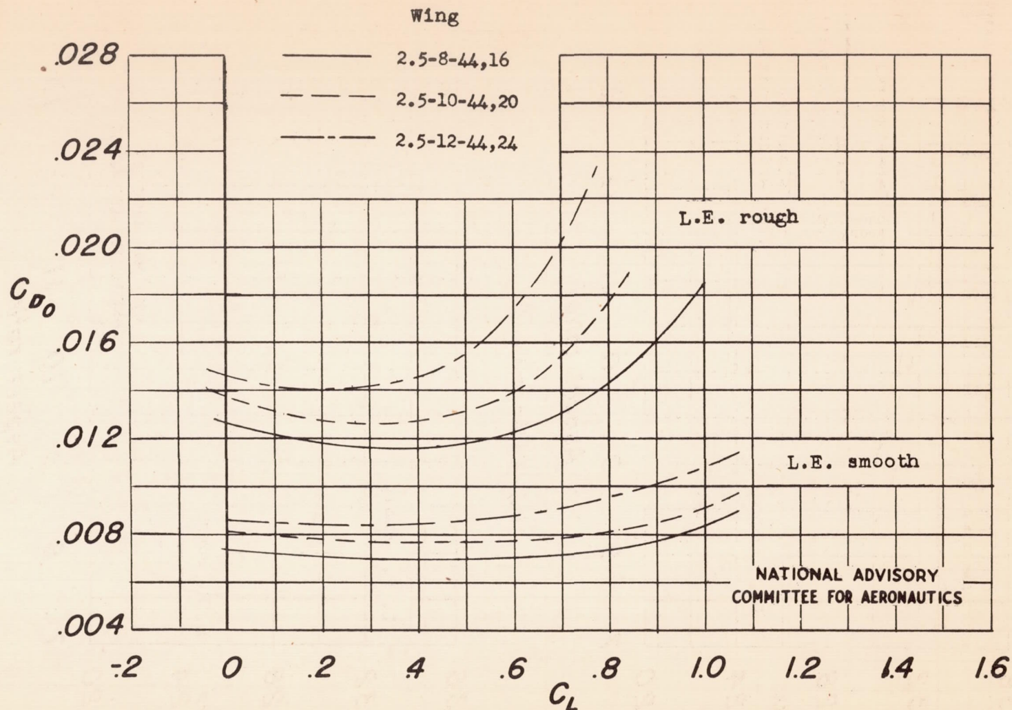
Figure 20.- Comparison of calculated profile-drag coefficients for smooth and rough wings.
