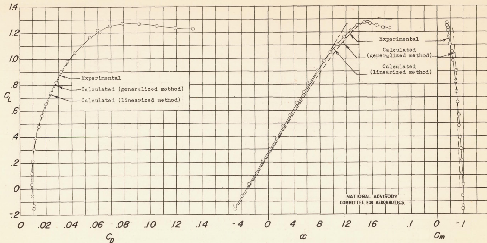
(a) C_L against C_D , \alpha , and C_m .
