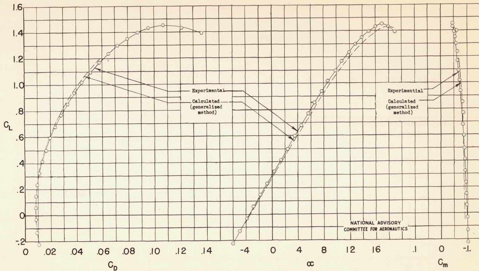
(a) C_L against C_D , \alpha , and C_m .
