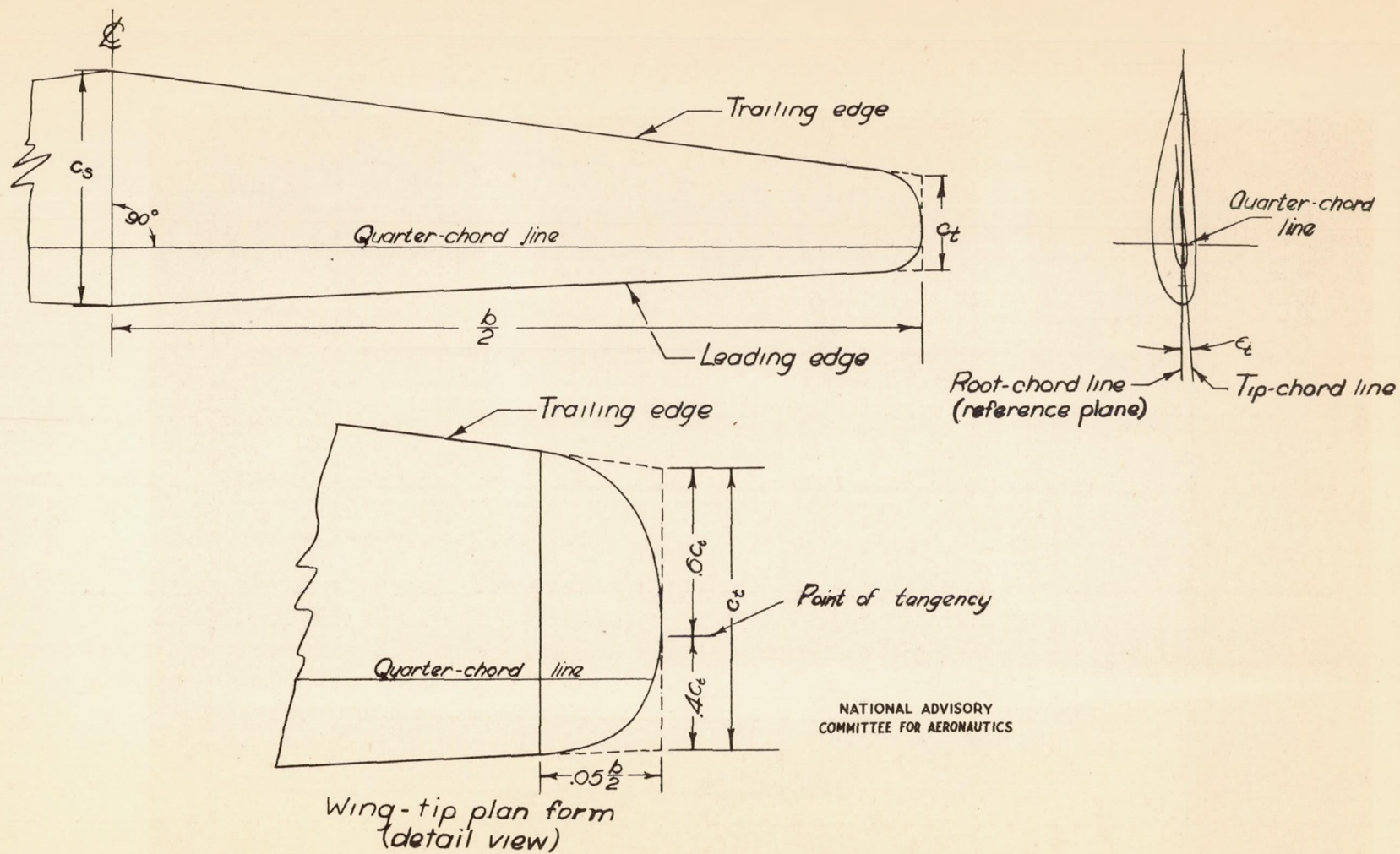
Figure 1.- Layout of typical tapered wing.
