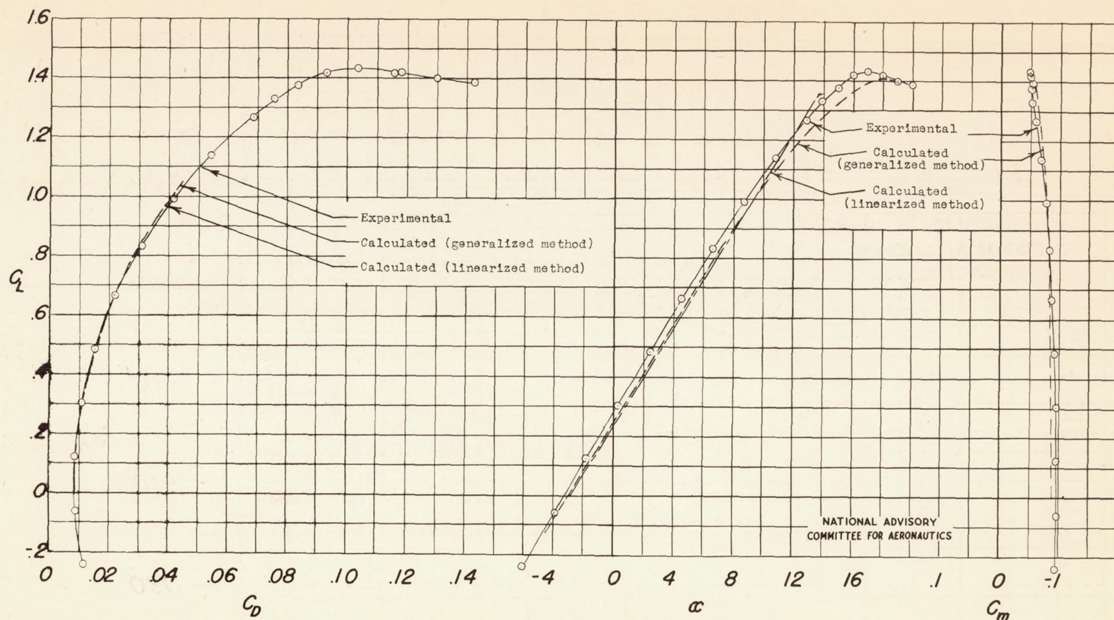
(a) C_L against C_D , \alpha , and C_m .
