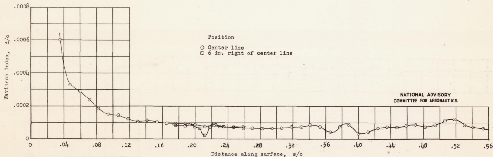
Figure 7.- Waviness measurements on NACA 65(215)-114 practical-construction airfoil section in "as-received" condition and with production finish.
