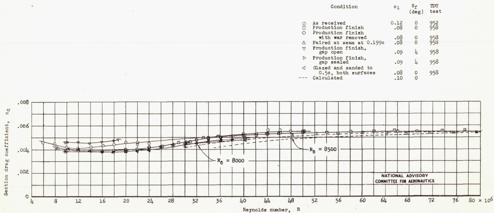
Figure 9.- Variation of section drag coefficient with Reynolds number for NACA 65(215)-114 practical-construction airfoil section with various surface conditions and flap deflections.
