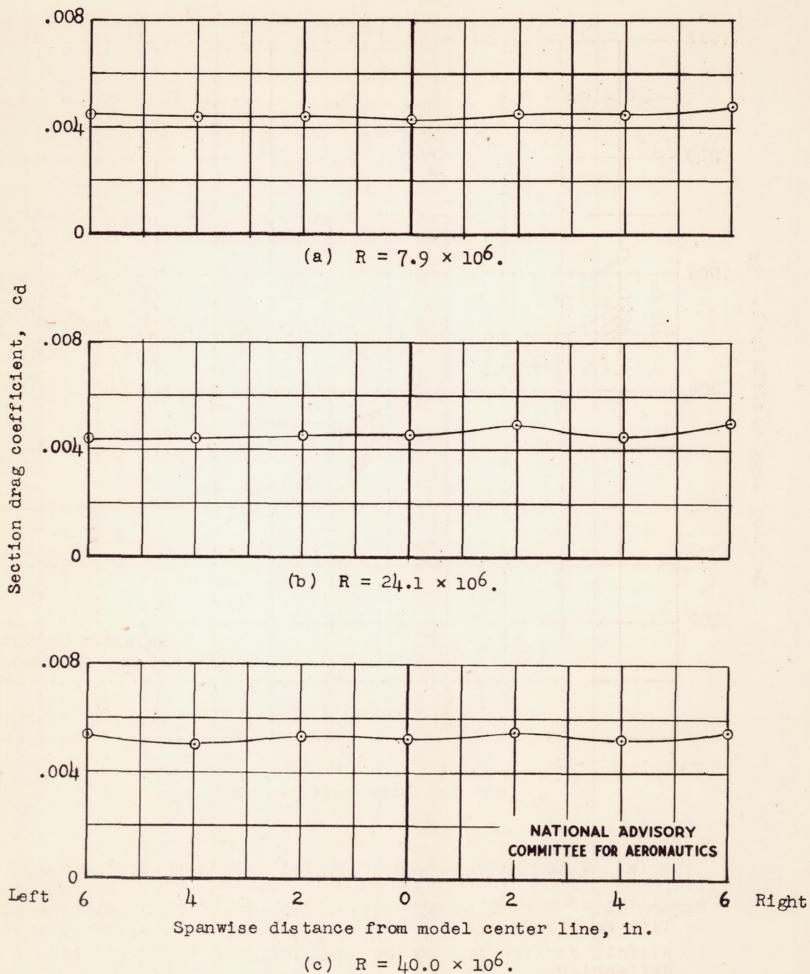
Figure 10.- Spanwise drag variation of NACA 65(215)-114 practical-construction airfoil section in as-received condition. c_l = 0.12 ; test, TDT 952.
