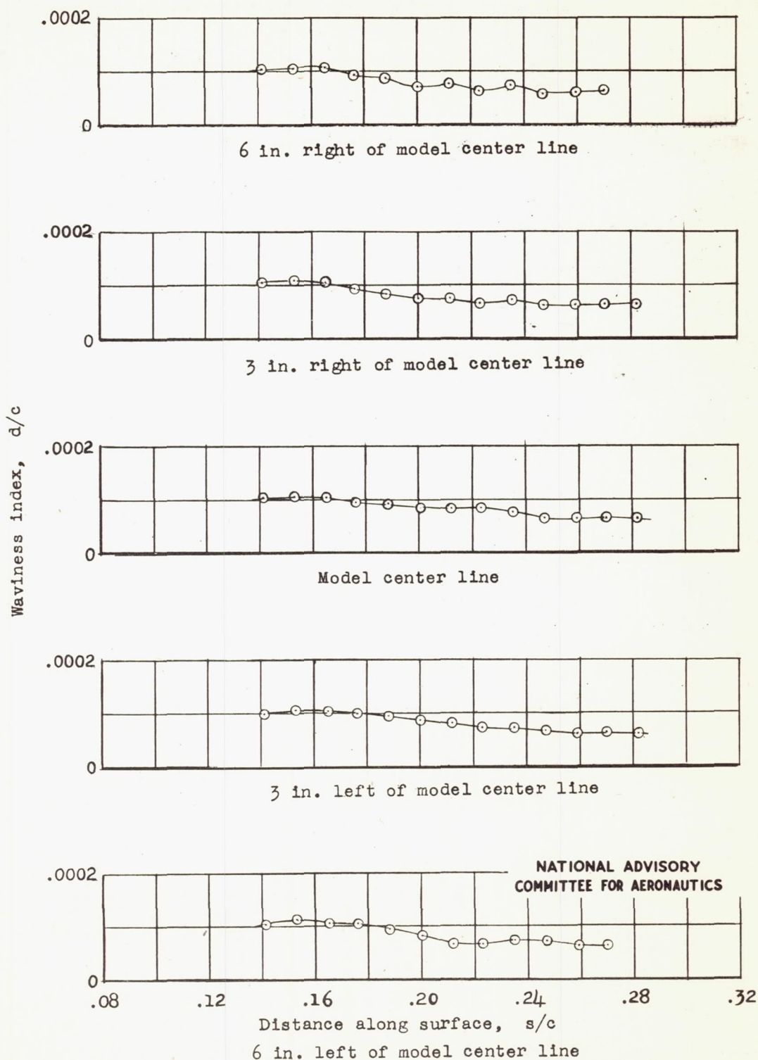
Figure 8.- Waviness measurements of NACA 65(215)-114 practical-construction airfoil section with wave faired at 0.199c.
