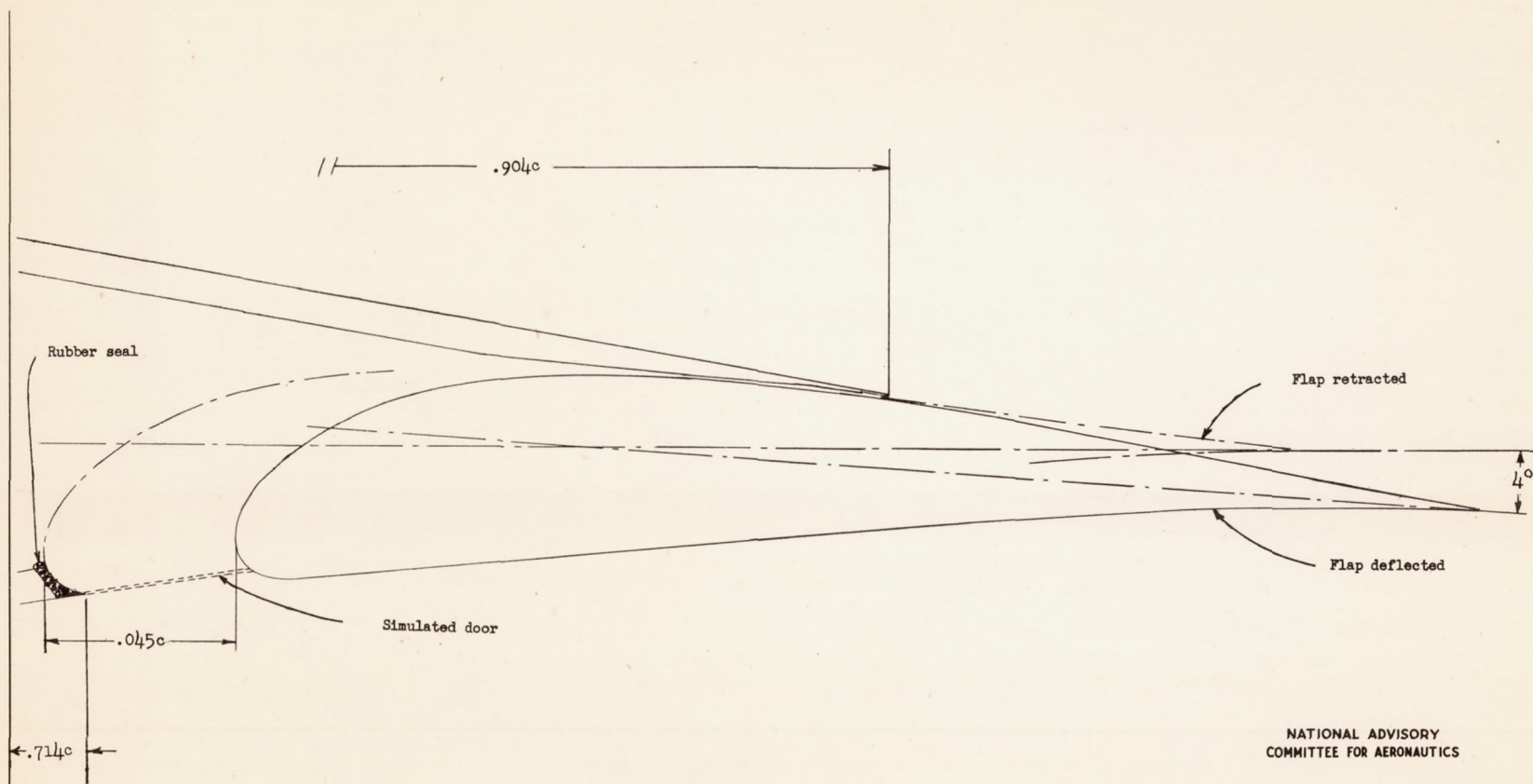
Figure 3.- Flap for NACA 65(215)-114 practical-construction airfoil section in retracted and deflected position.
