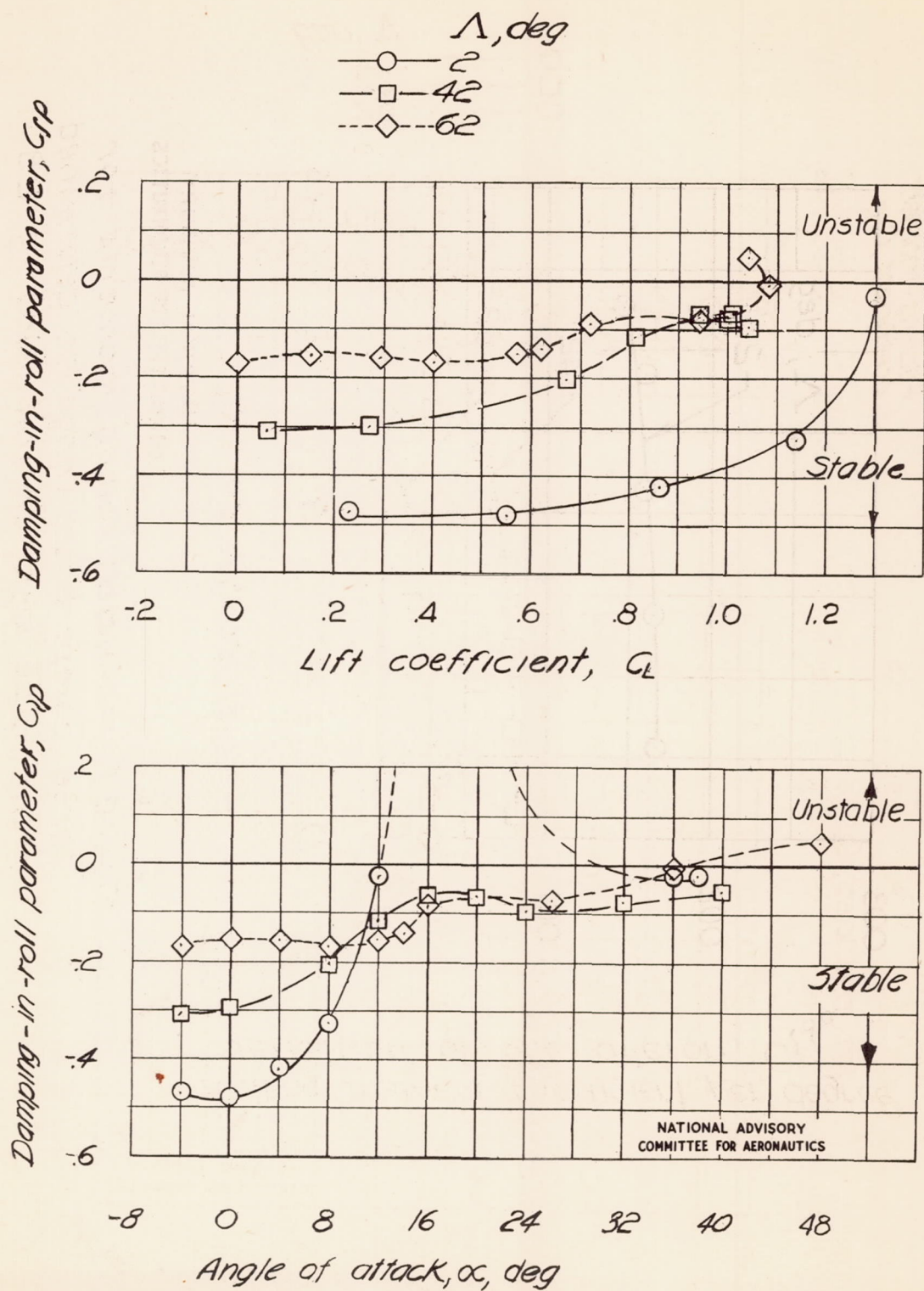
Figure 5.-Variation of the damping-in-roll parameter C_{rp} with angle of attack and lift coefficient as obtained from tests of wings having sweep back angles of 2^\circ , 42^\circ , and 62^\circ ; q=2.8 .
