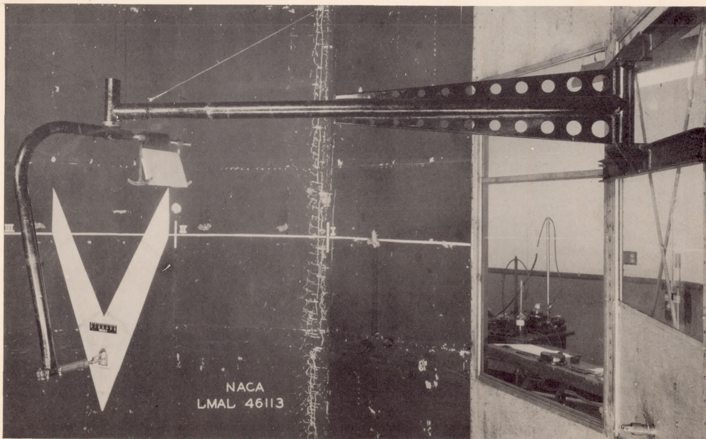
Figure 1.- Roll stand with model of wing with 62° sweepback attached, mounted in Langley 15-foot free-spinning tunnel.
