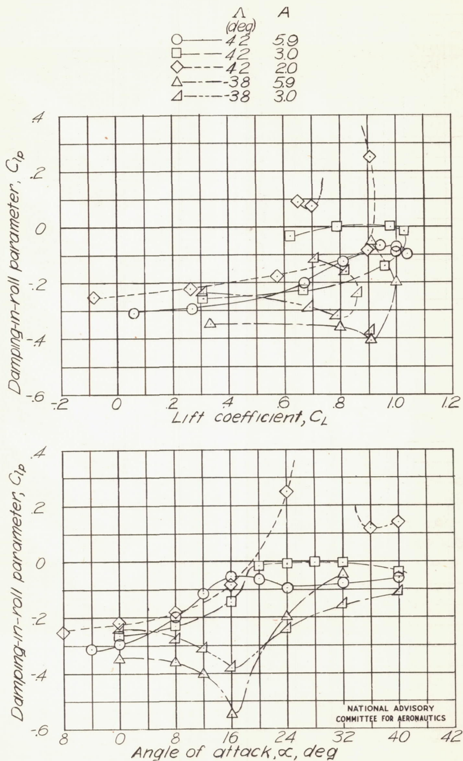
Figure 7.-Variation of the damping-in-roll parameter C_{lp} with angle of attack and lift coefficient for the wings tested.
