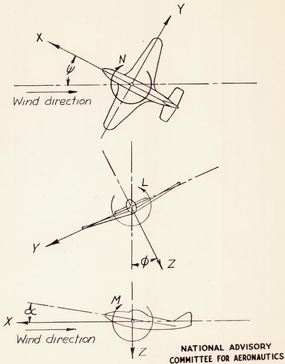
Figure 4.- The stability system of axes. Arrows indicate positive directions of moments and forces. This system of axes is defined as an orthogonal system having its origin at the center of gravity and in which the Z-axis is in the plane of symmetry and perpendicular to the relative wind, the X-axis is in the plane of symmetry and perpendicular to the Z-axis, and the Y-axis is perpendicular to the plane of symmetry.
