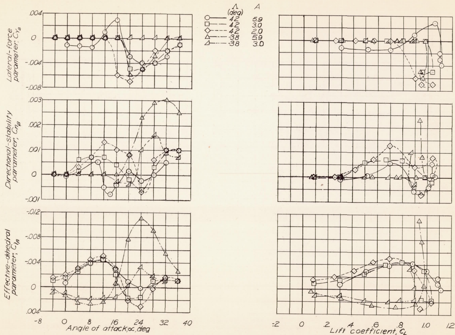
Figure 6. - Variation of the lateral-stability parameters C_{Y_{\delta}} , C_{N_{\delta}} , and C_{L_{\delta}} with angle of attack and lift coefficient for the wings tested.
