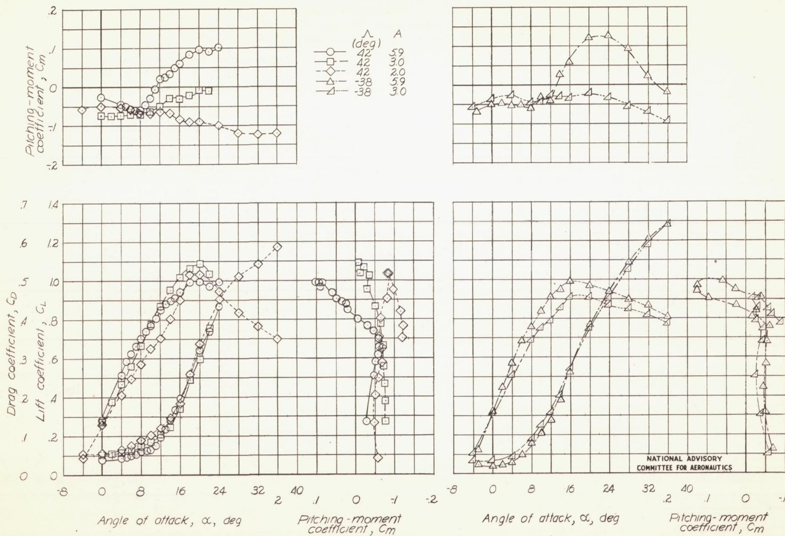
Figure 5- Variation of the lift, drag, and pitching-moment characteristics with angle of attack for the wings tested. q = 3.0 .
