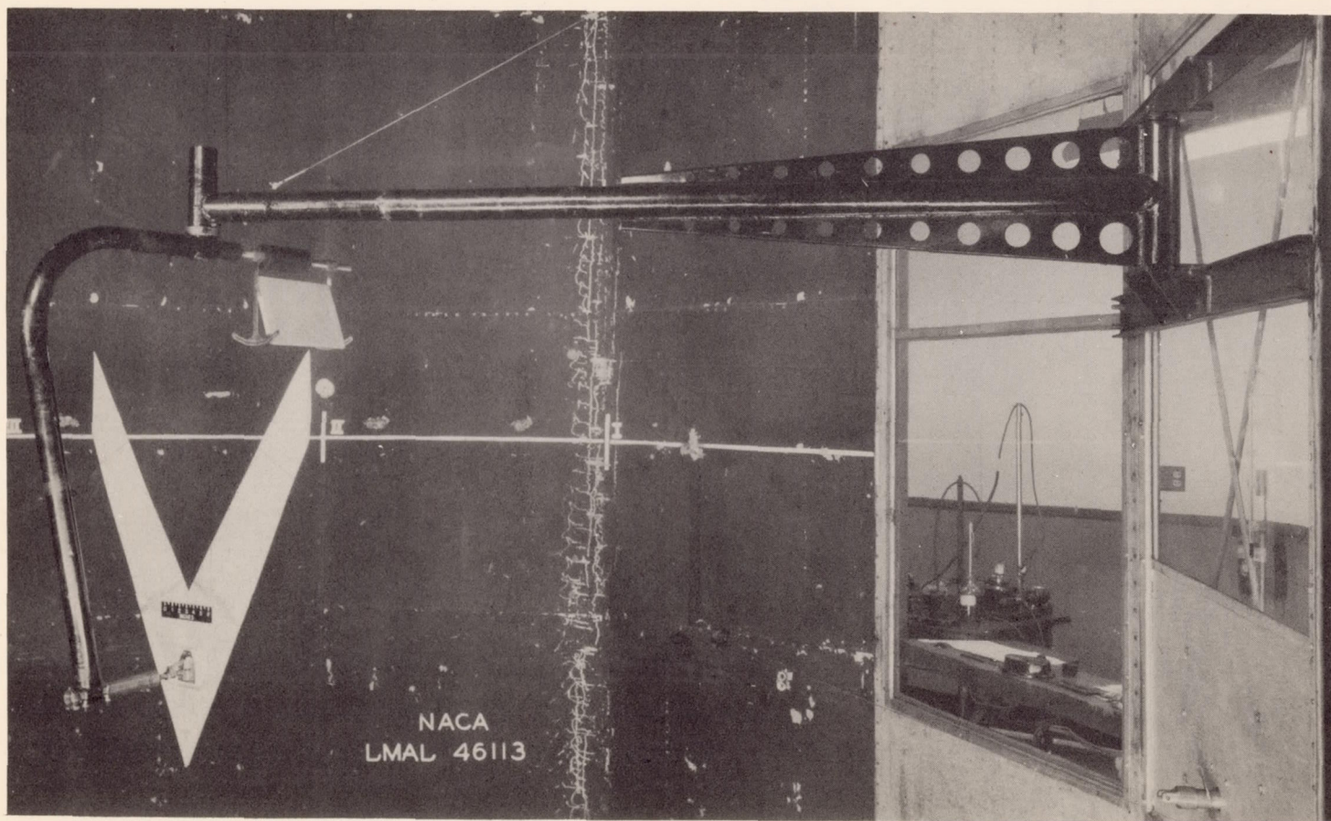
Figure 2.- Roll stand with model of swept-back wing attached, mounted in Langley 15-foot free-spinning tunnel.
