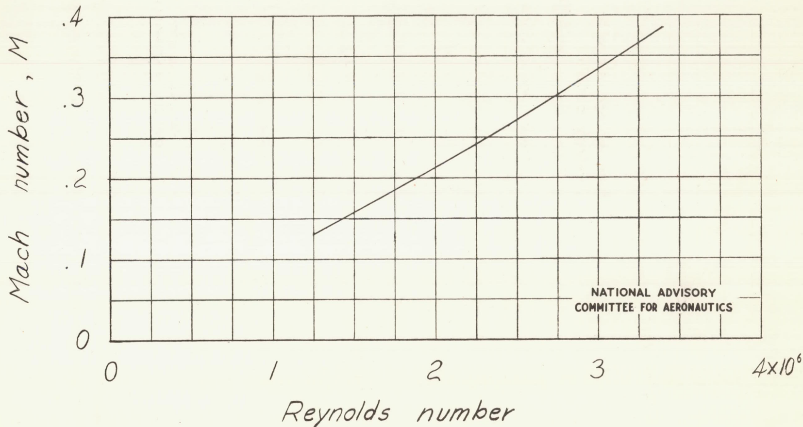
Figure 7.- Variation of Mach number with Reynolds number of the \frac{1}{10} -scale hulls of a hypothetical flying boat.
