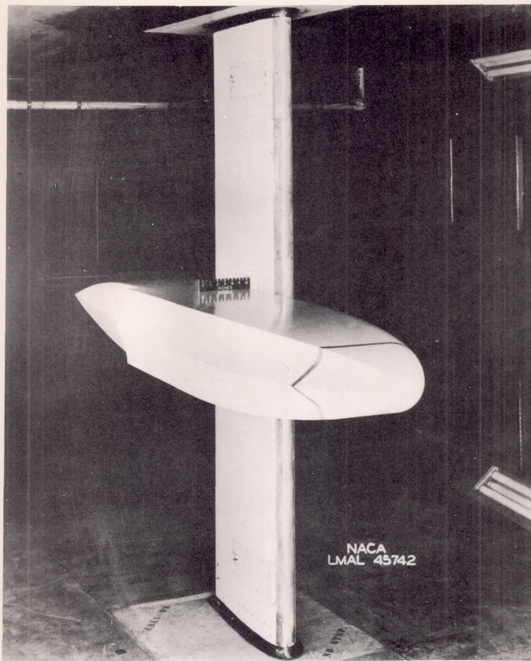
(b) Hull 203 \left(\frac{L}{b} = 9\right) with wing.
