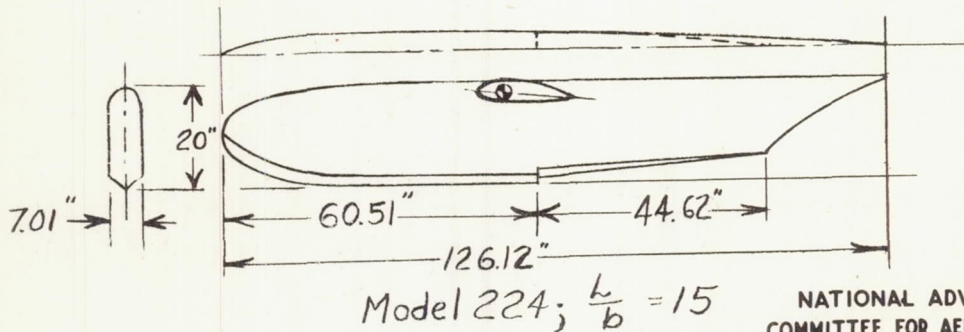
Figure 1.—Lines of Langley tank models 203, 213, 214, and 224.
