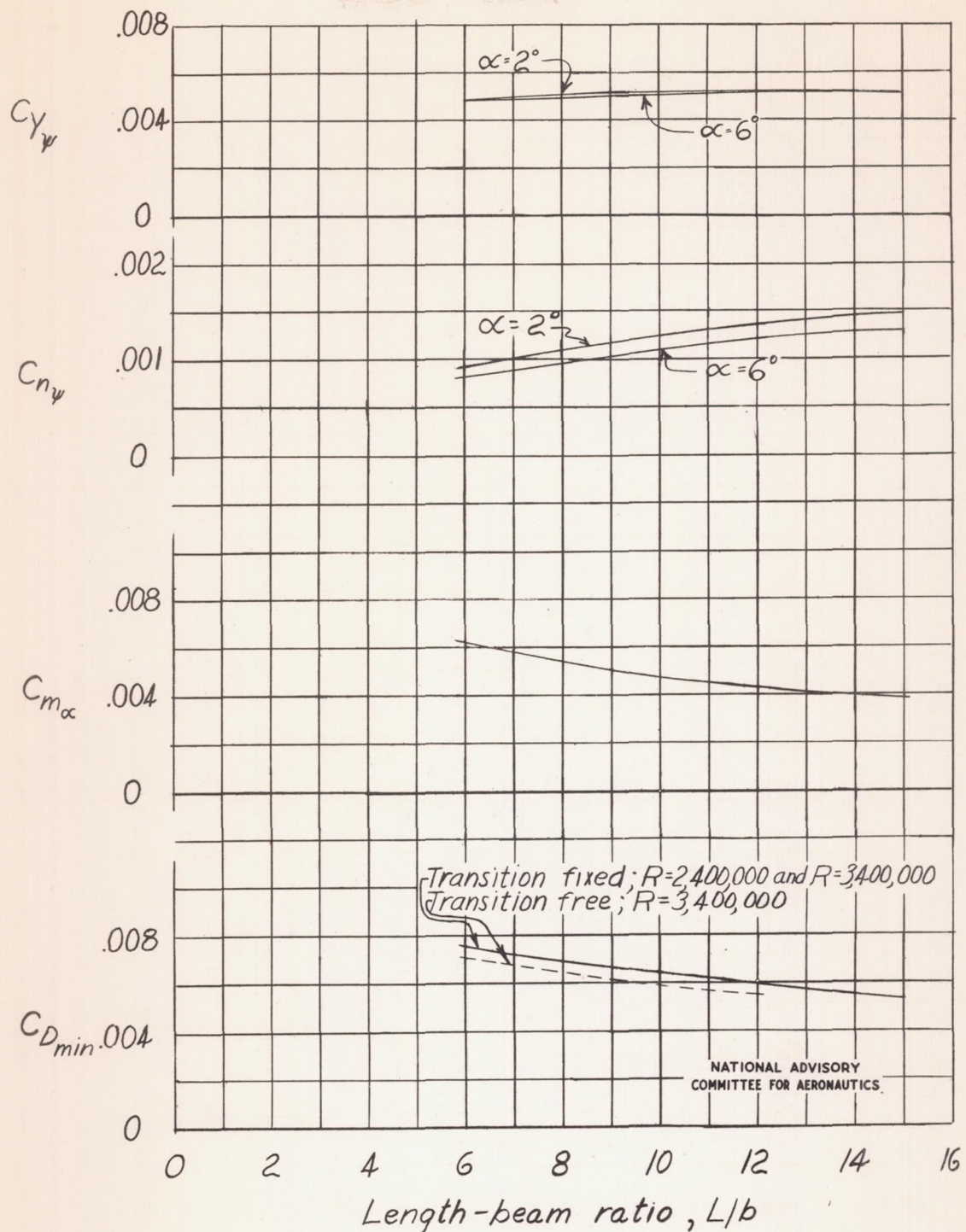
Figure 11.- Effect of length-beam ratio on C_{Dmin} and the parameters C_{m\alpha} , C_{n\psi} , C_{Y\psi} for the \frac{1}{10} -scale hulls of a hypothetical flying boat.
