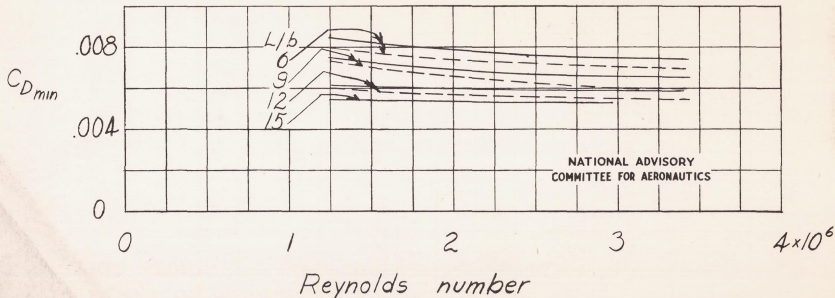
Figure 13.- Effect of Reynolds number on C_{D_{min}} for the \frac{1}{10} -scale hulls of a hypothetical flying boat.
