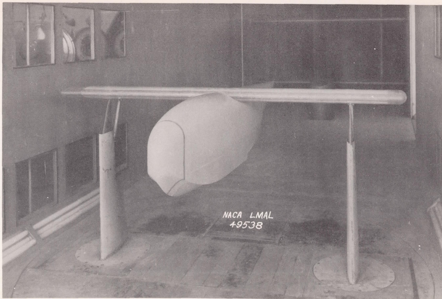
Figure 7.- Langley tank model 203 with bow chines rounded 7 percent of hull length mounted in the Langley 300 MPH 7- by 10-foot tunnel.
