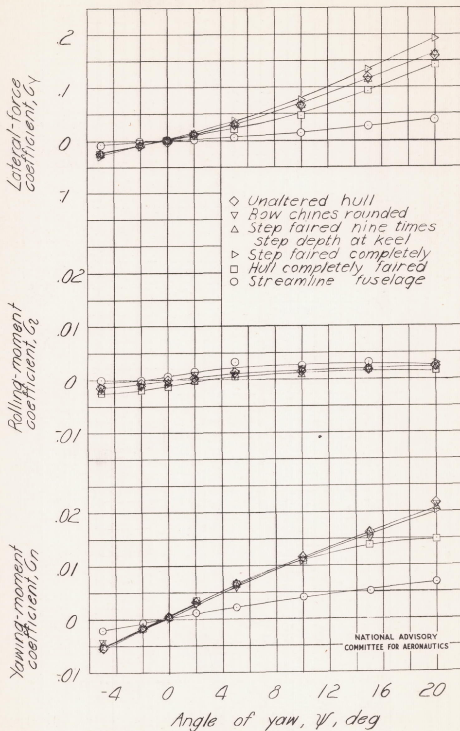
Figure 9.- Effect of aerodynamic refinement on the aerodynamic characteristics in yaw of Langley tank model 203. R \approx 1.2 \times 10^6 ; \alpha = 2^\circ .
