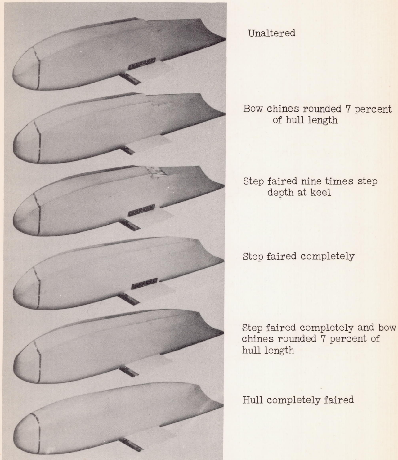
Figure 5.- Langley tank model 203 unaltered and with aerodynamic refinements.
