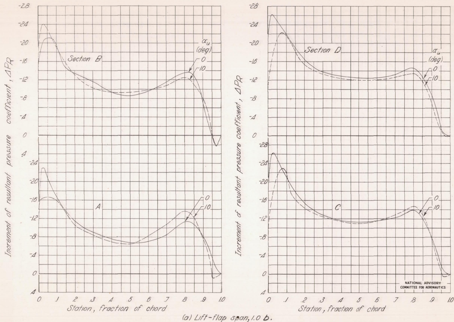
Figure 13.-Increment of resultant pressure coefficient at different spanwise sections caused by a 0.20c-chord lift flap hinged at 0.80c. \delta f_L = 60^\circ ; R = 1.76 \times 10^6 . (Section locations are shown in fig. 1.)
