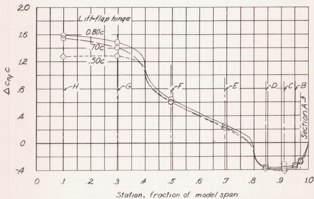
Figure 19. - Variation of the incremental spanwise loading caused by varying the hinge location of a 0.20c -chord lift flap with a 0.20c -chord trim flap hinged in the normal position. b_{f_L} = 0.40 b ; b_{f_T} = 0.20 b ; \delta_{f_L} = 60^\circ ; \delta_{f_T} = 60^\circ .
