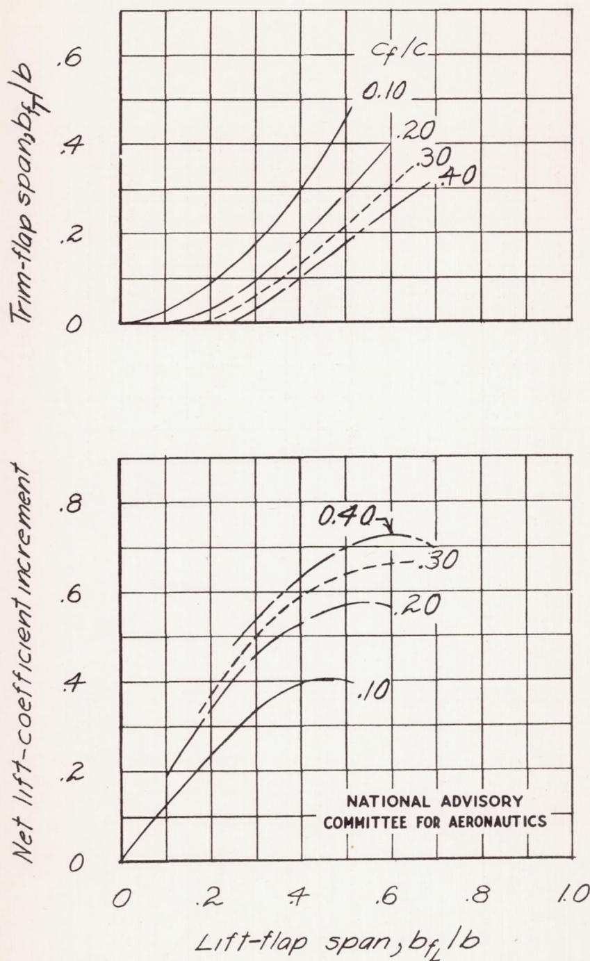
Figure 24. - Effect of lift-flap span on the net lift-coefficient increment and trim-flap span for various-chord lift and trim flaps. \alpha = 10^\circ ; \Delta C_m = 0 ; \delta_{f_L} = 60^\circ ; \delta_{f_T} = 60^\circ .
