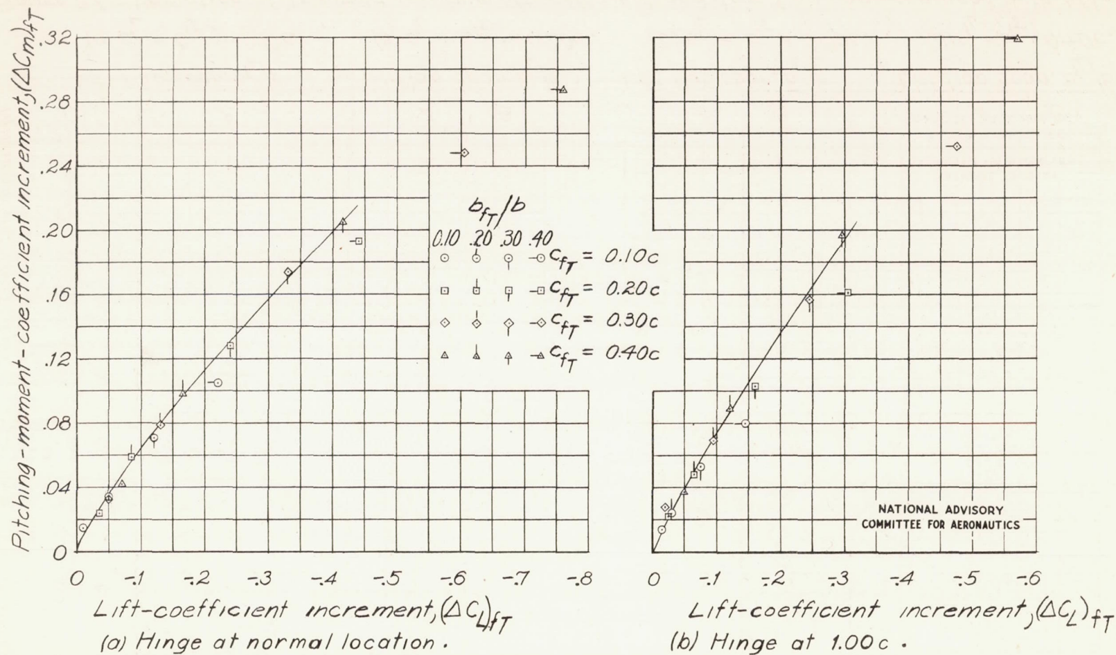
Figure 26.-Variation of pitching-moment-coefficient increment with lift-coefficient increment of trim flaps. \alpha = 10^\circ ; \delta_{fT} = 60^\circ .
