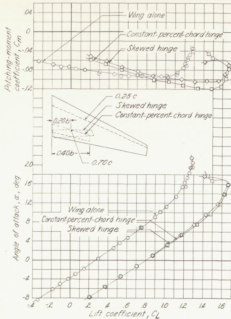
Figure 12. - Lift, drag, and pitching-moment coefficients of wing with 0.20c -chord lift flap with the hinge line coinciding with and skewed relative to 0.70c of wing. Lift-flap span, 0.40b ; \delta f_L = 60^\circ ; R = 1.78 \times 10^6 .
