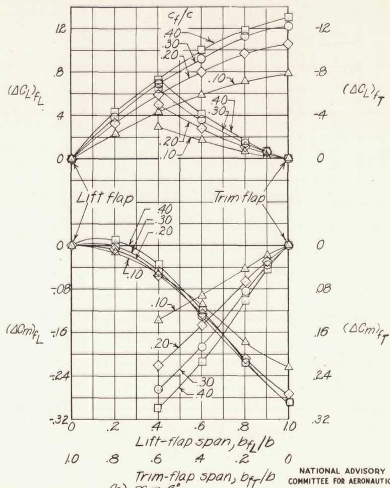
Figure 22.—Effect of lift-flap span and trim-flap span on the increment of lift coefficient and increment of pitching-moment coefficient of various-chord lift and trim flaps. \delta_L = 60^\circ ; \delta_T = 60^\circ .
