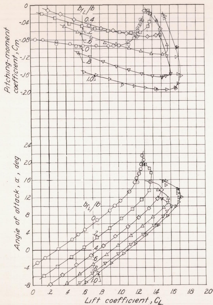
Figure 5. — Lift, drag, and pitching-moment coefficients of wing with 0.20c -chord lift flap for various flap spans. \delta f_L = 60^\circ ; R = 1.78 \times 10^6 .
