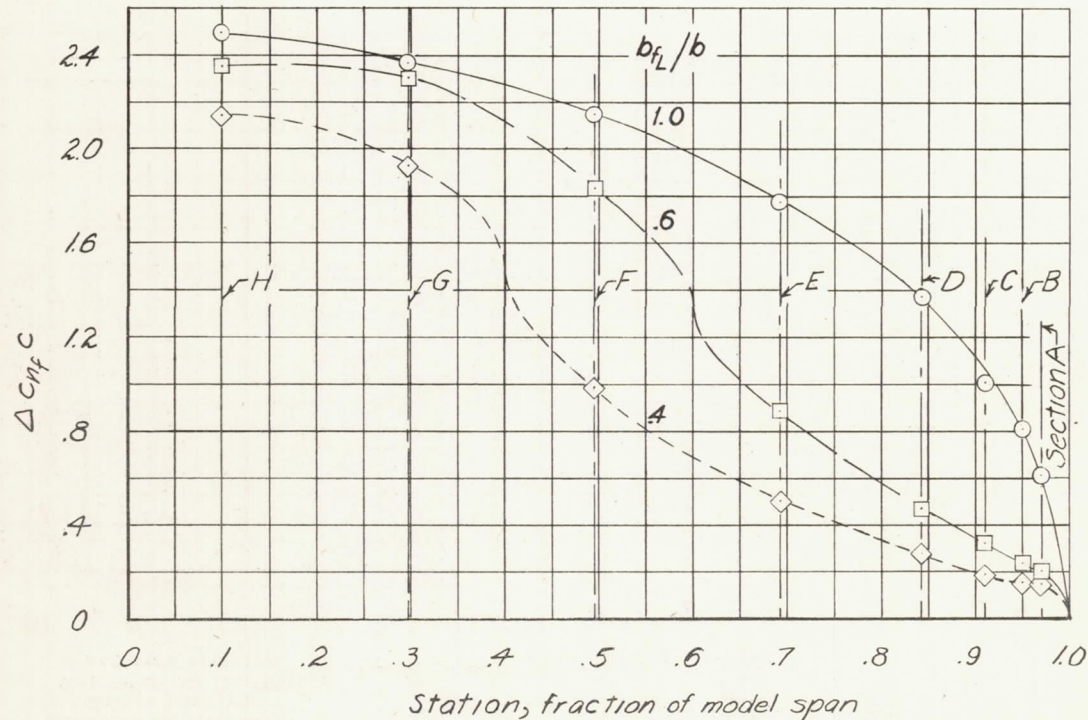
Figure 18. - Variation of the incremental spanwise loading caused by a 0.40c-chord lift flap of various spans. \delta_{fL} = 60^\circ .
