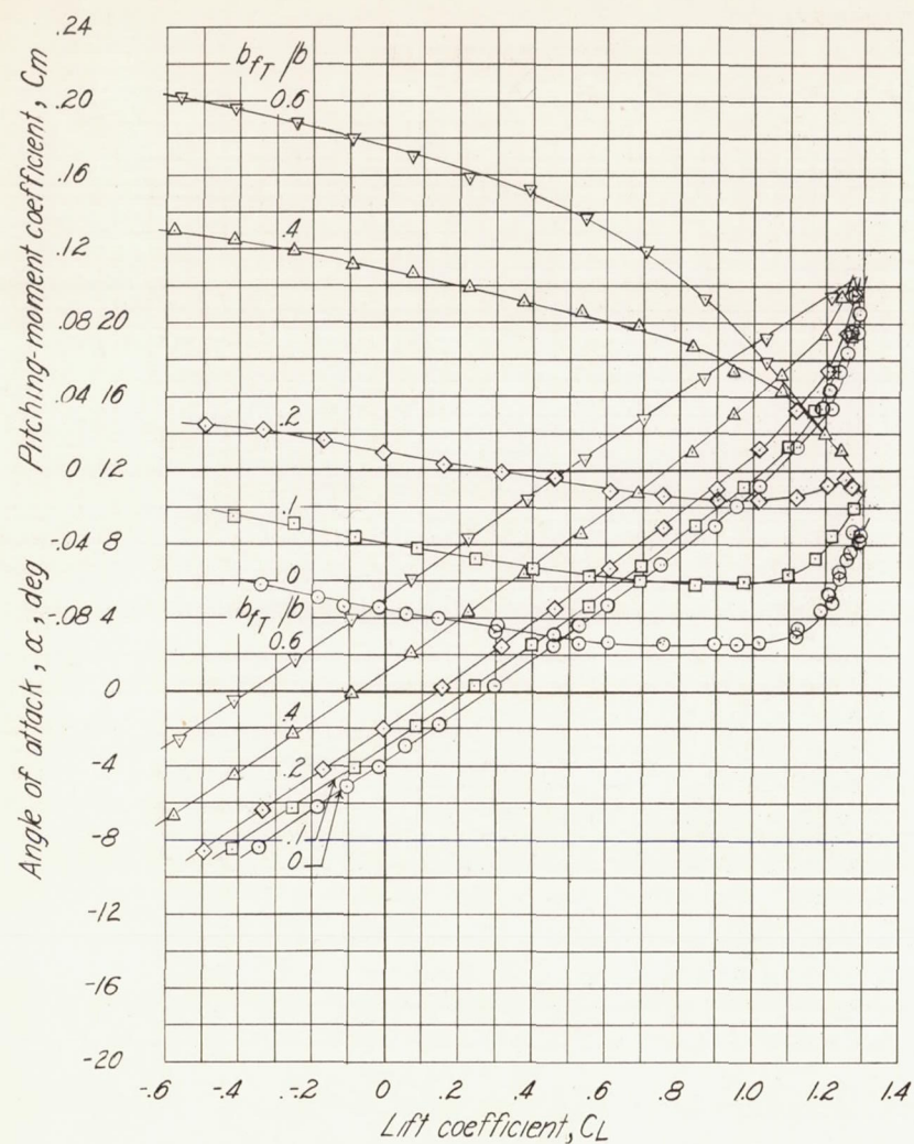
(a) Trim-flap hinge, 0.70c. Figure 10. — Lift, drag, and pitching-moment coefficients of wing with 0.30c-chord trim flap for various flap spans. \delta f_T = 60^\circ ; R = 1.78 \times 10^6 .
