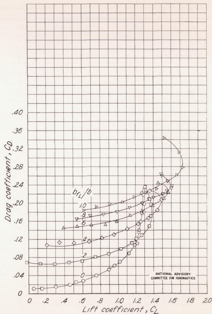
Figure 5. — Lift, drag, and pitching-moment coefficients of wing with 0.20c -chord lift flap for various flap spans. \delta f_L = 60^\circ ; R = 1.78 \times 10^6 .
