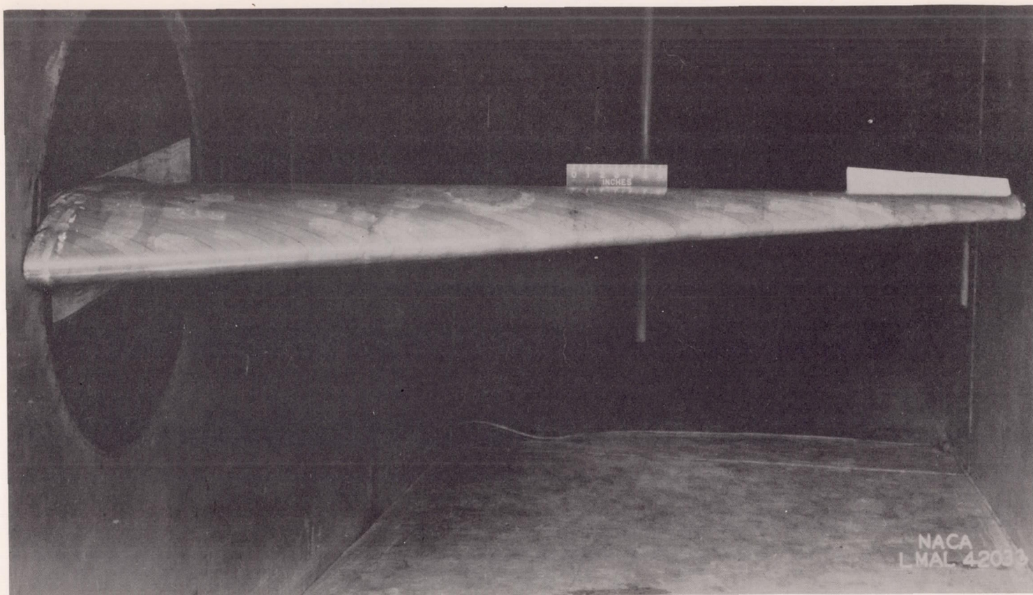
(b) Front view of swept-back wing with a 0.20c-chord 0.20b-span trim flap.
