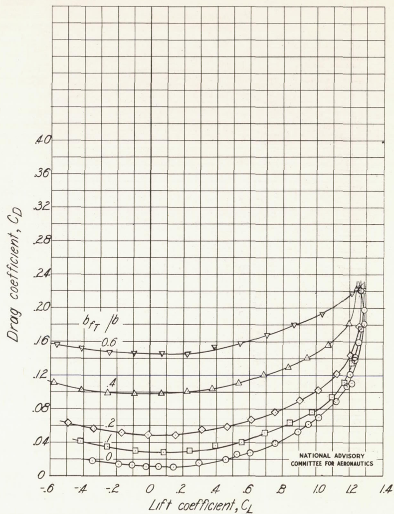
(a) Trim-flap hinge, 0.70c. Figure 10. — Lift, drag, and pitching-moment coefficients of wing with 0.30c-chord trim flap for various flap spans. \delta f_T = 60^\circ ; R = 1.78 \times 10^6 .
