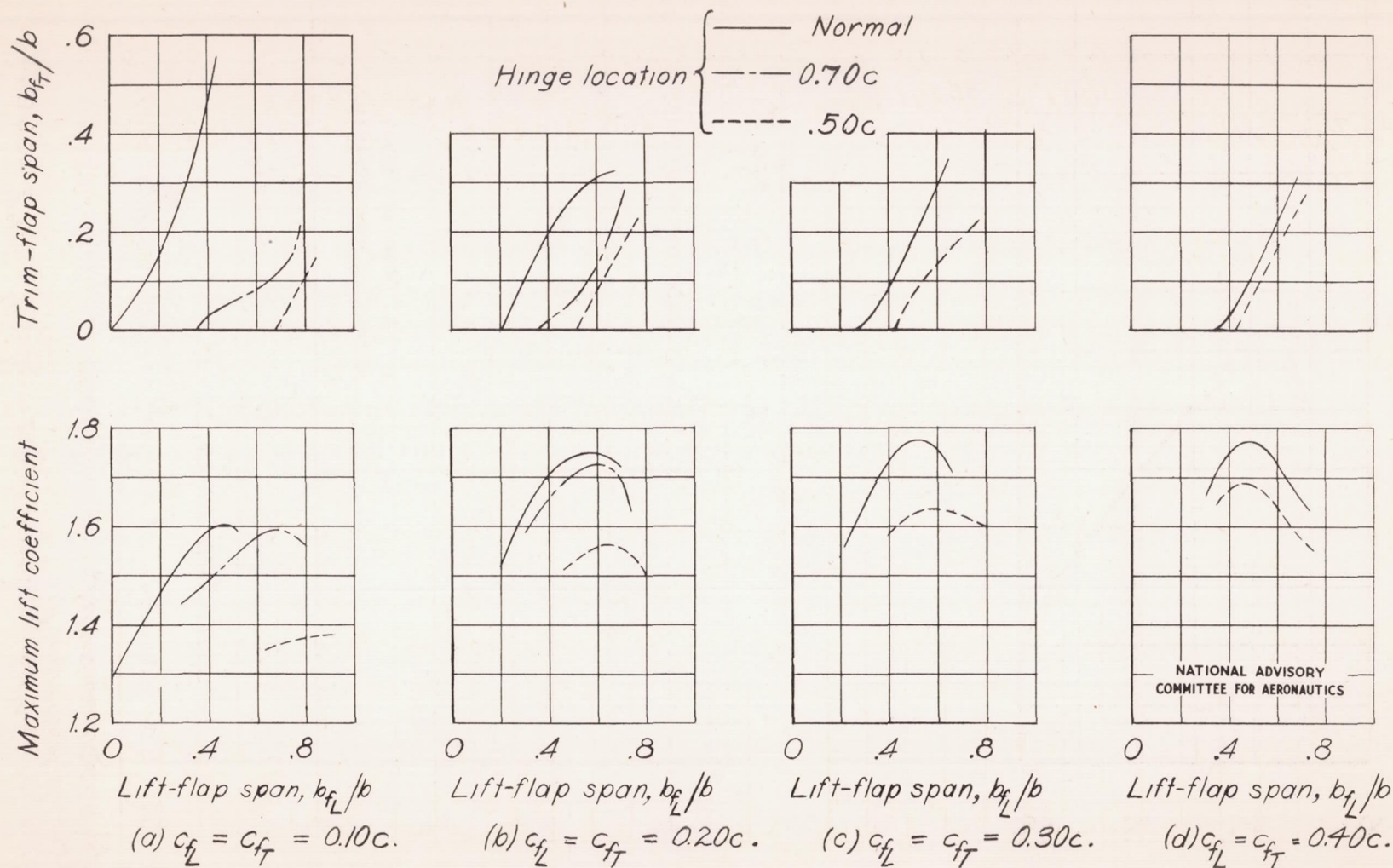
Figure 27. - Variation of trimmed maximum lift coefficient and trim-flap span required with lift-flap span for various lift-flap hinge locations.
