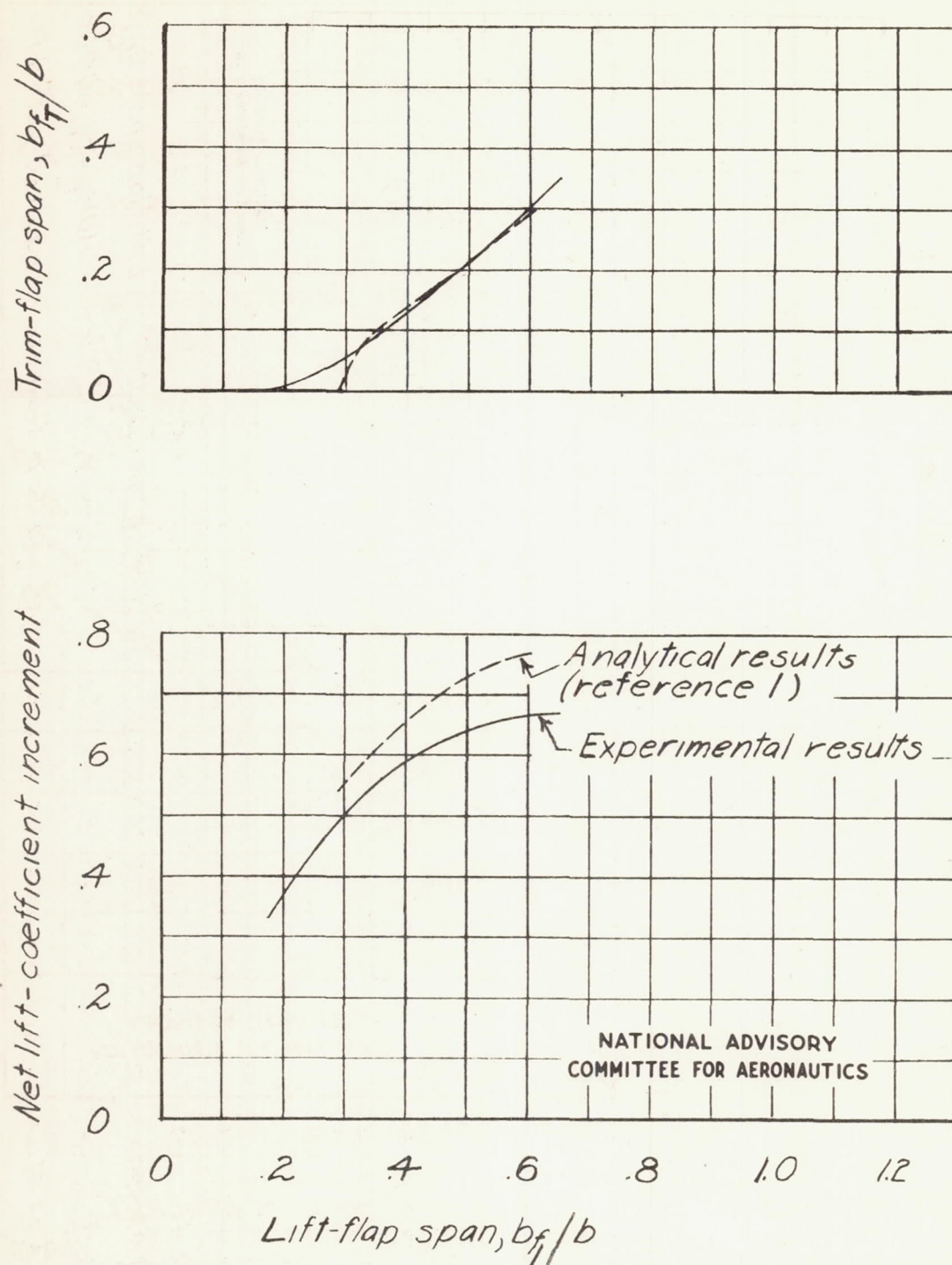
Figure 28.- Comparison of experimental results with results based on analytical methods of reference 1. Sweepback of quarter-chord line 23^\circ ; c_{fL} = c_{fT} = 0.30c .
