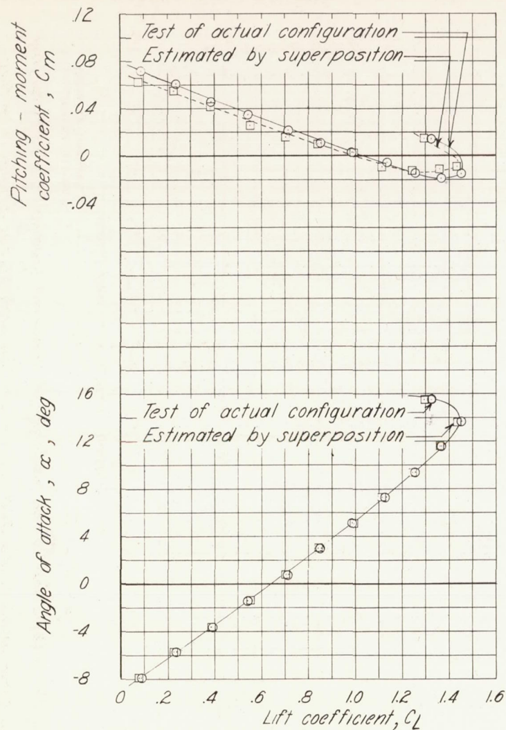
(a) Lift-flap hinge, 0.50c ; trim-flap hinge, 0.80c . Figure 20. - Lift, drag, and pitching-moment coefficients of wing with 0.20c -chord lift and trim flaps. Lift-flap span, 0.40b ; trim-flap span, 0.20b ; \delta_{fl} = 60^\circ ; \delta_{ft} = 60^\circ ; R = 1.78 \times 10^6 .
