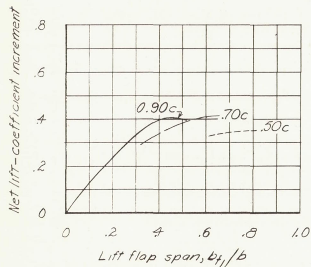
Figure 25.—Effect of lift-flap span on the net lift-coefficient increment and trim-flap span for various locations of the lift flap hinge. Trim flap hinged in normal location. \Delta C_m = 0 ; \delta_{f_L} = 60^\circ ; \delta_{f_T} = 60^\circ ; \alpha = 10^\circ .
