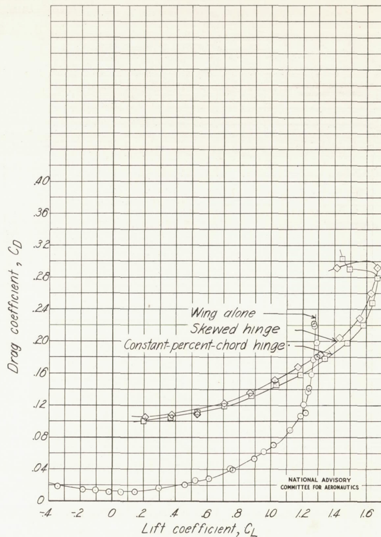
Figure 12. - Lift, drag, and pitching-moment coefficients of wing with 0.20c -chord lift flap with the hinge line coinciding with and skewed relative to 0.70c of wing. Lift-flap span, 0.40b ; \delta f_L = 60^\circ ; R = 1.78 \times 10^6 .
