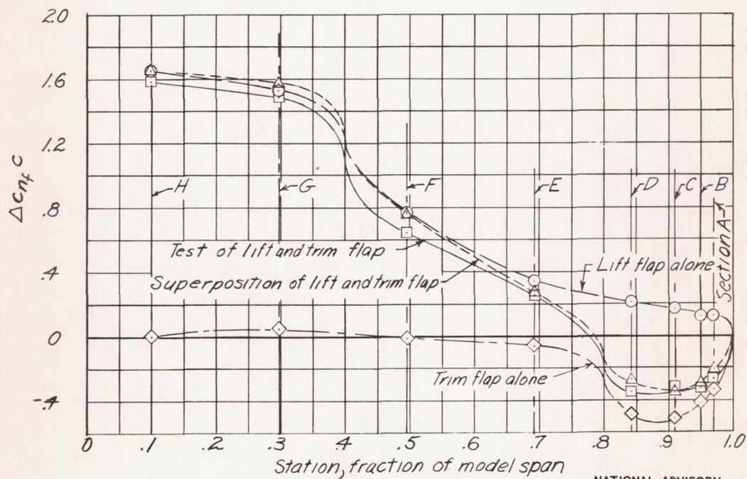
Figure 21. - Comparison of the incremental spanwise loading obtained from tests of a lift flap and a trim flap with that obtained by a superposition of the loadings obtained with each flap tested separately. Hinge location normal, c_{f_L} = 0.20c ; c_{f_T} = 0.20c ; b_{f_L} = 0.40b ; b_{f_T} = 0.20b ; \delta_{f_L} = 60^\circ ; \delta_{f_T} = 60^\circ .
