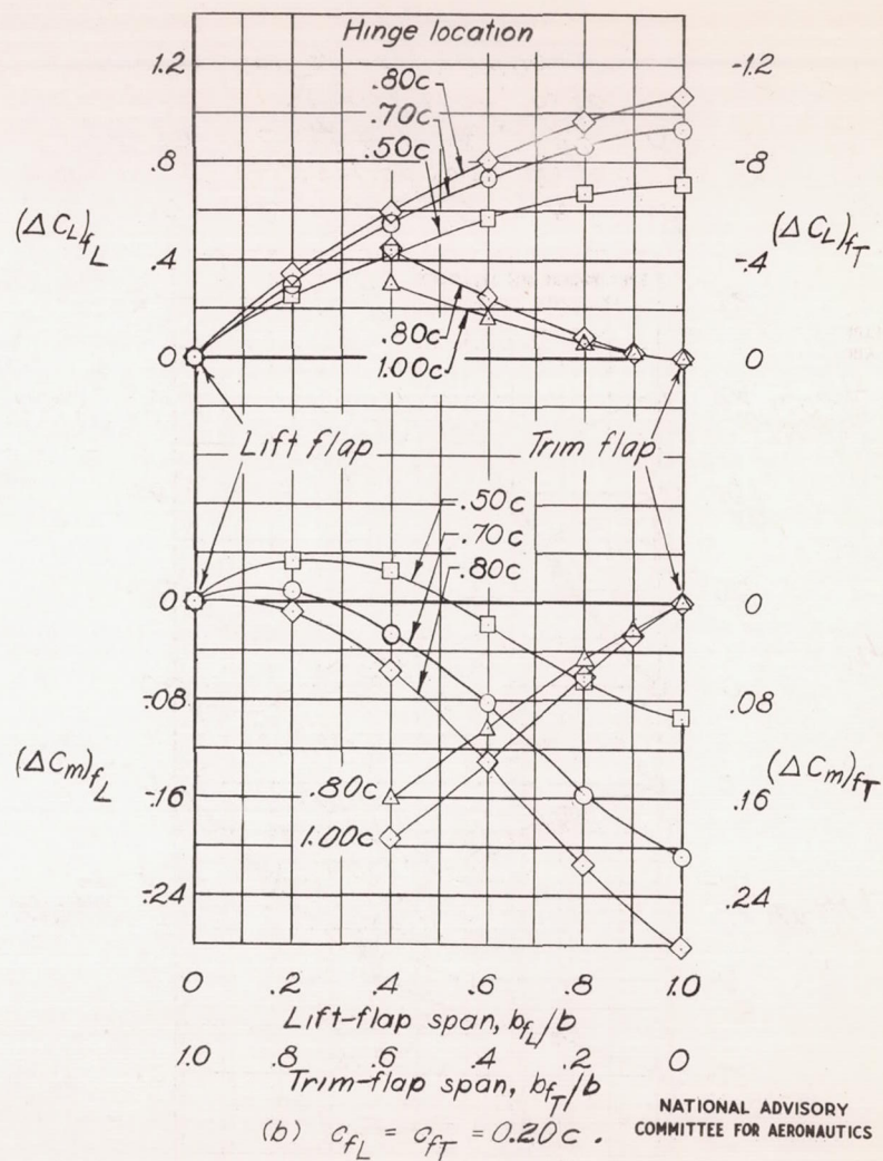
Figure 23.—Effect of lift-flap span and trim-flap span on the increment of lift coefficient and increment of pitching-moment coefficient for various hinge locations of lift and trim flaps. \alpha = 10^\circ ; \delta_{FL} = \delta_{FT} = 60^\circ .
