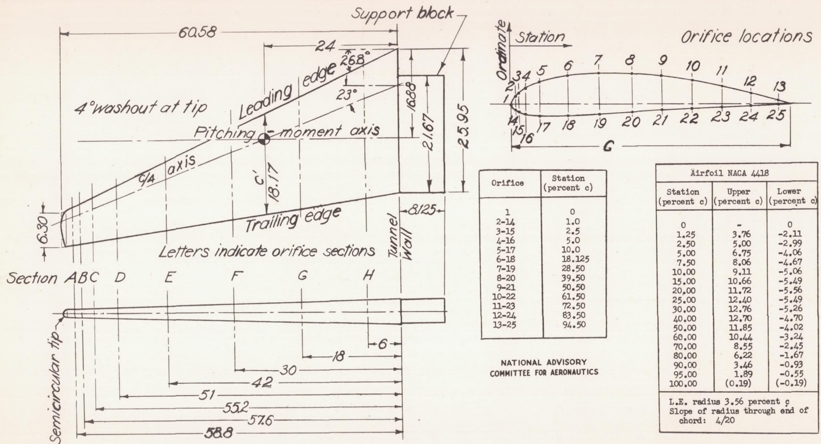
Figure 1.-Details of the swept-back wing model. Area (complete wing) 13.550 square feet; aspect ratio 7.51; taper ratio 0.243. All dimensions are in inches.
