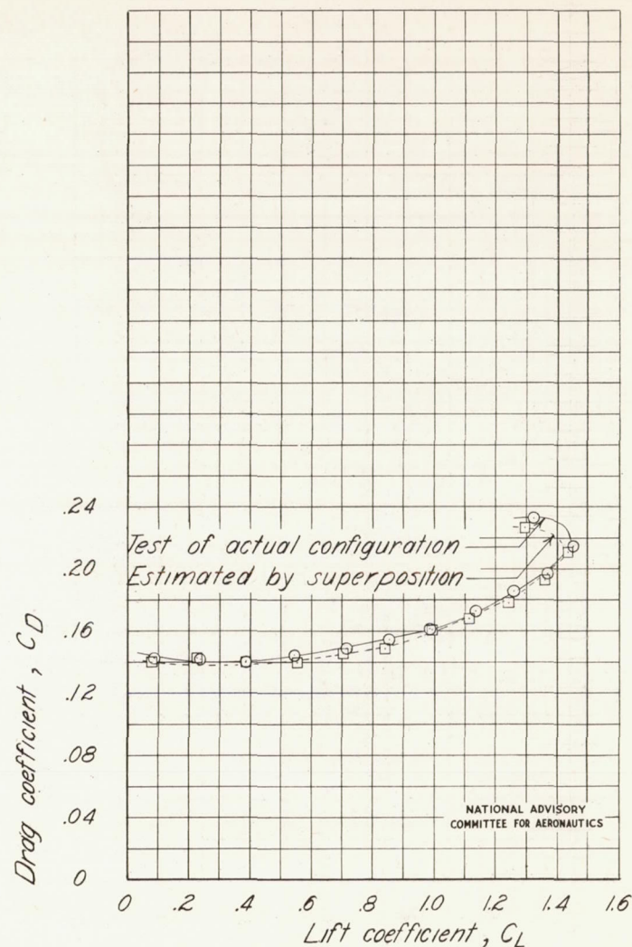
(a) Lift-flap hinge, 0.50c ; trim-flap hinge, 0.80c . Figure 20. - Lift, drag, and pitching-moment coefficients of wing with 0.20c -chord lift and trim flaps. Lift-flap span, 0.40b ; trim-flap span, 0.20b ; \delta_{fl} = 60^\circ ; \delta_{ft} = 60^\circ ; R = 1.78 \times 10^6 .
