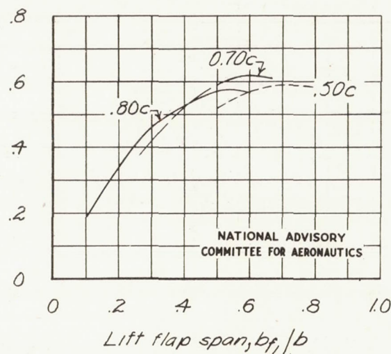
Figure 25.—Effect of lift-flap span on the net lift-coefficient increment and trim-flap span for various locations of the lift flap hinge. Trim flap hinged in normal location. \Delta C_m = 0 ; \delta_{f_L} = 60^\circ ; \delta_{f_T} = 60^\circ ; \alpha = 10^\circ .
