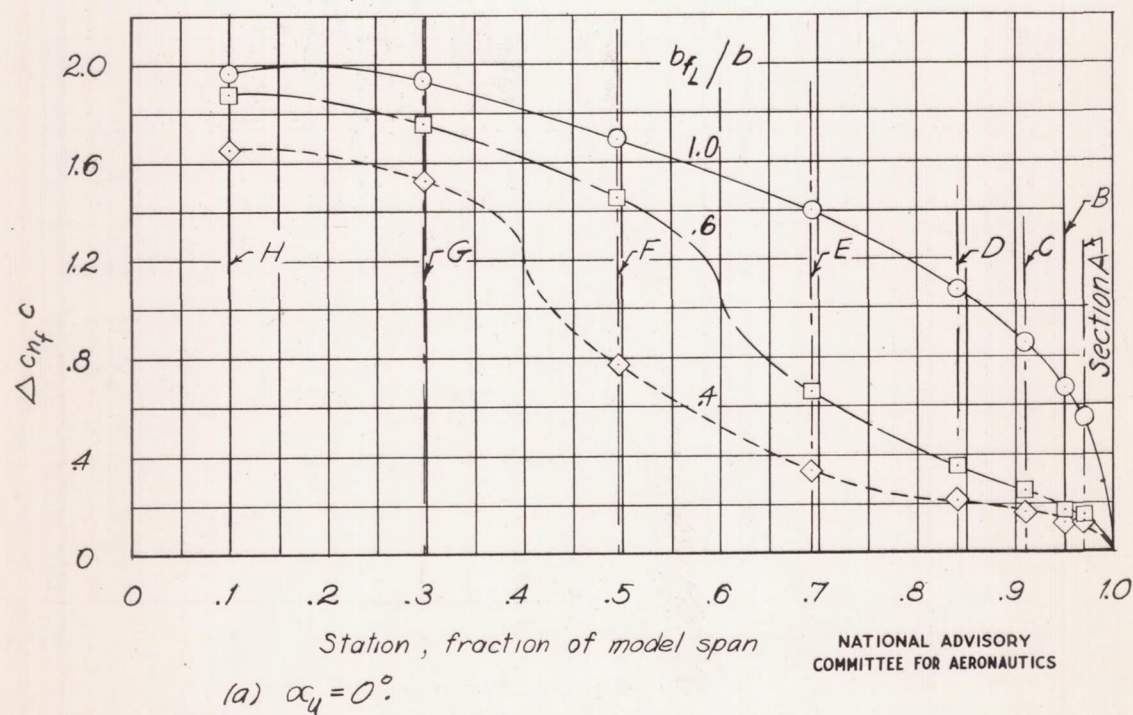
Figure 17. - Variation of the incremental spanwise loading caused by a 0.20c-chord lift flap of various spans. \delta_{fL} = 60^\circ .
