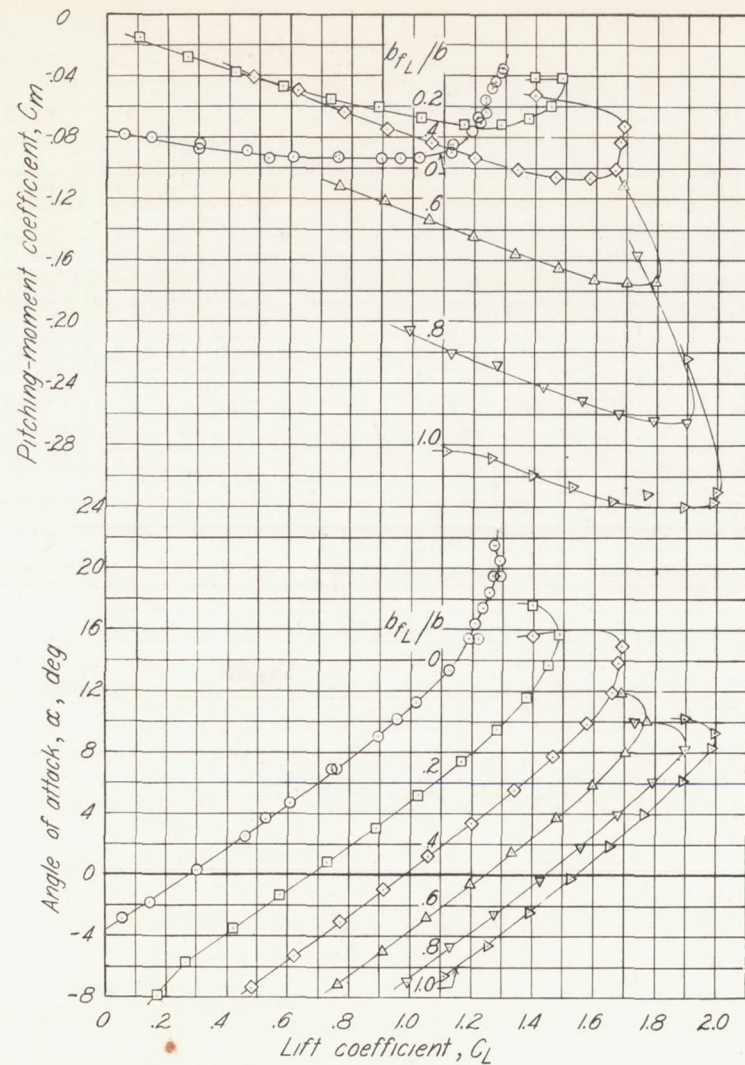
Figure 7. -Lift, drag, and pitching-moment coefficients of wing with 0.40c-chord lift flap for various flap spans. \delta f_L = 60^\circ ; R = 1.78 \times 10^6 .
