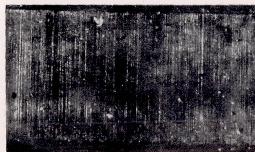
Figure 31.—Photomicrographs of surface replicas of cast-iron rings used in runs D, E, and F. (25×).
