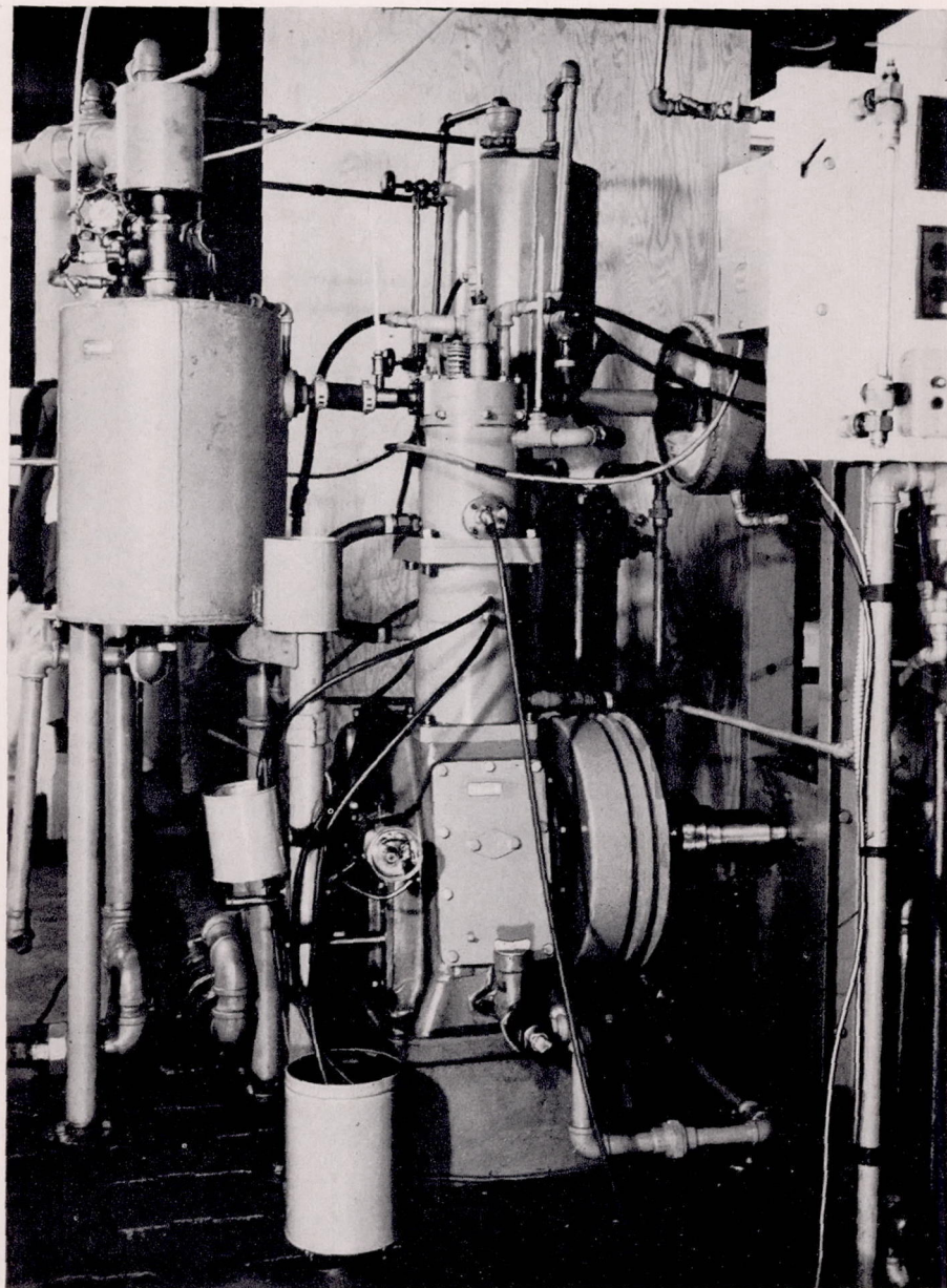
Figure 2.—General view of engine.
