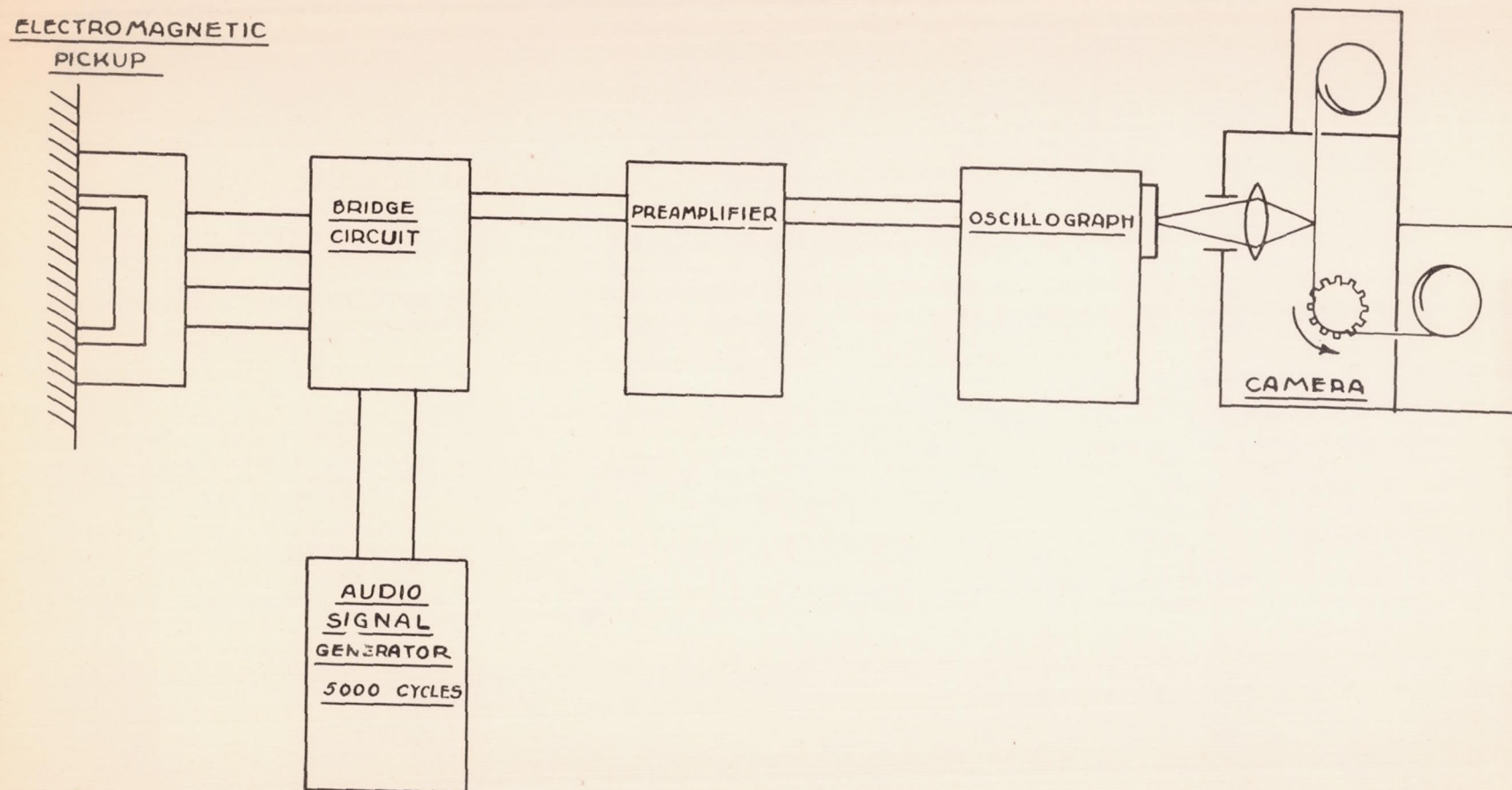
Figure 6.- Schematic diagram of sleeve-motion measuring apparatus.
