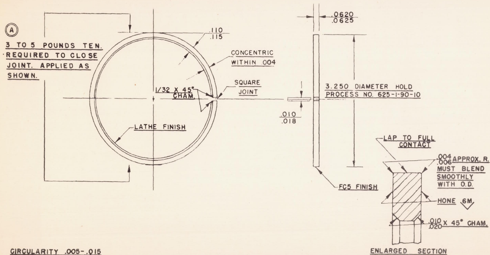
Figure 7.- Plain compression ring used in the tests.
