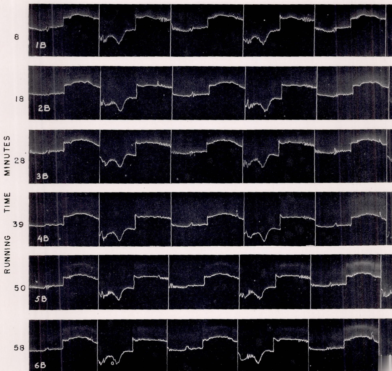
FIGURE 13.—Friction records for the run-in test with SAE 4140 barrel and chrome-plated top ring. (Records have been outlined for clearness.)
