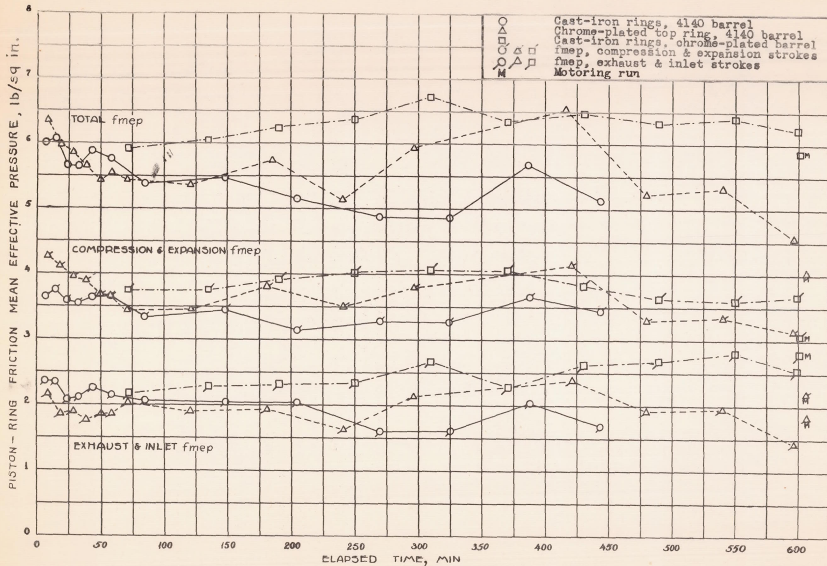
Figure 10.- Effect of running time on piston-ring friction mean effective pressure.
