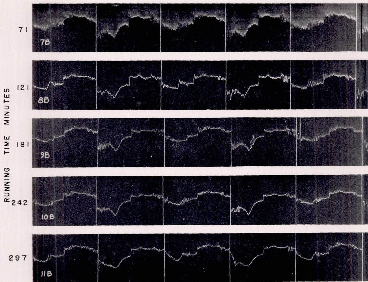
FIGURE 14.—Friction records for the run-in test with SAE 4140 sleeve and chrome-plated top ring. (Records 8B to 11B have been outlined for clearness.)
