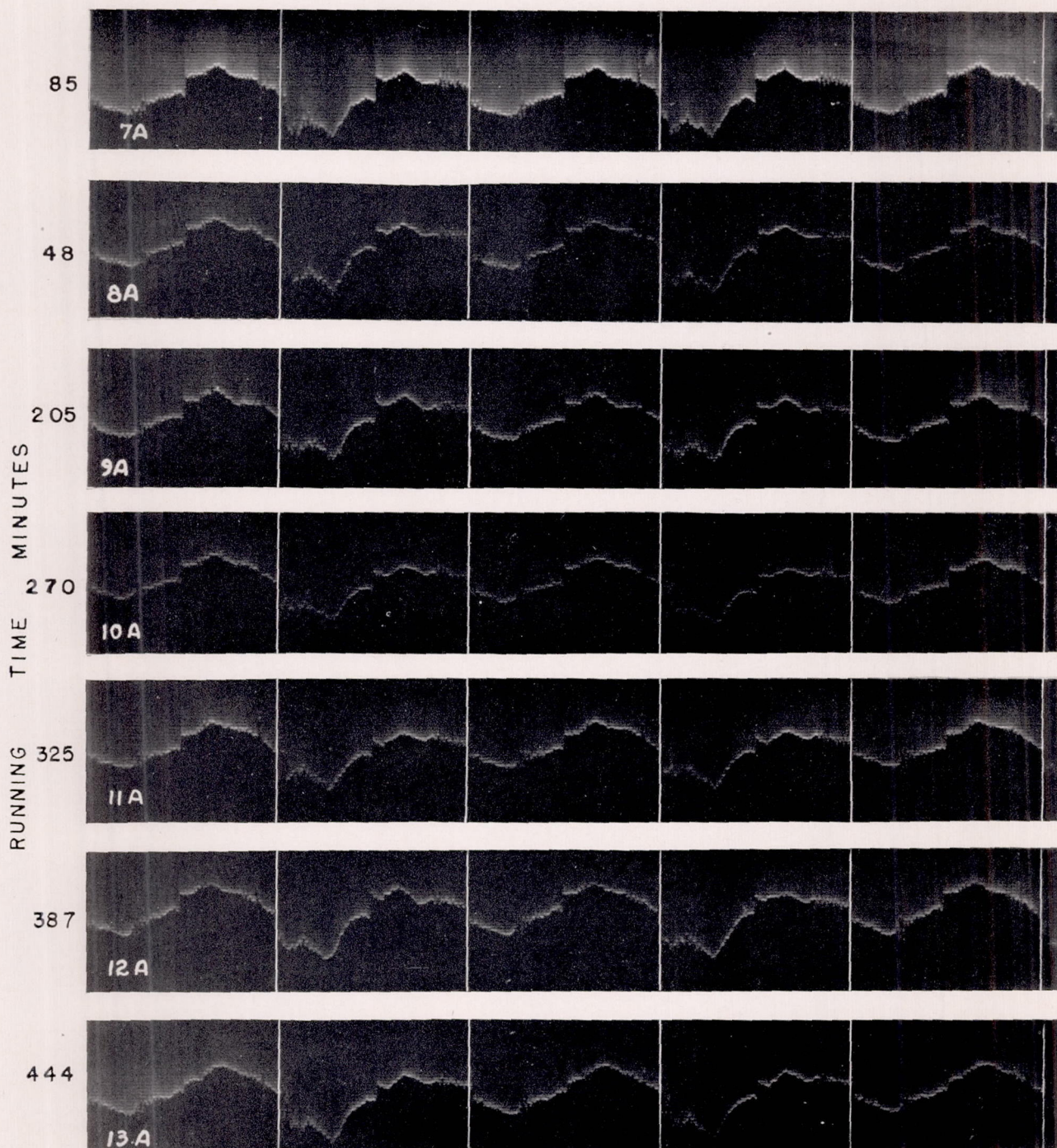
Figure 12.—Friction records for the run-in test with SAE 4140 sleeve and cast-iron rings.
