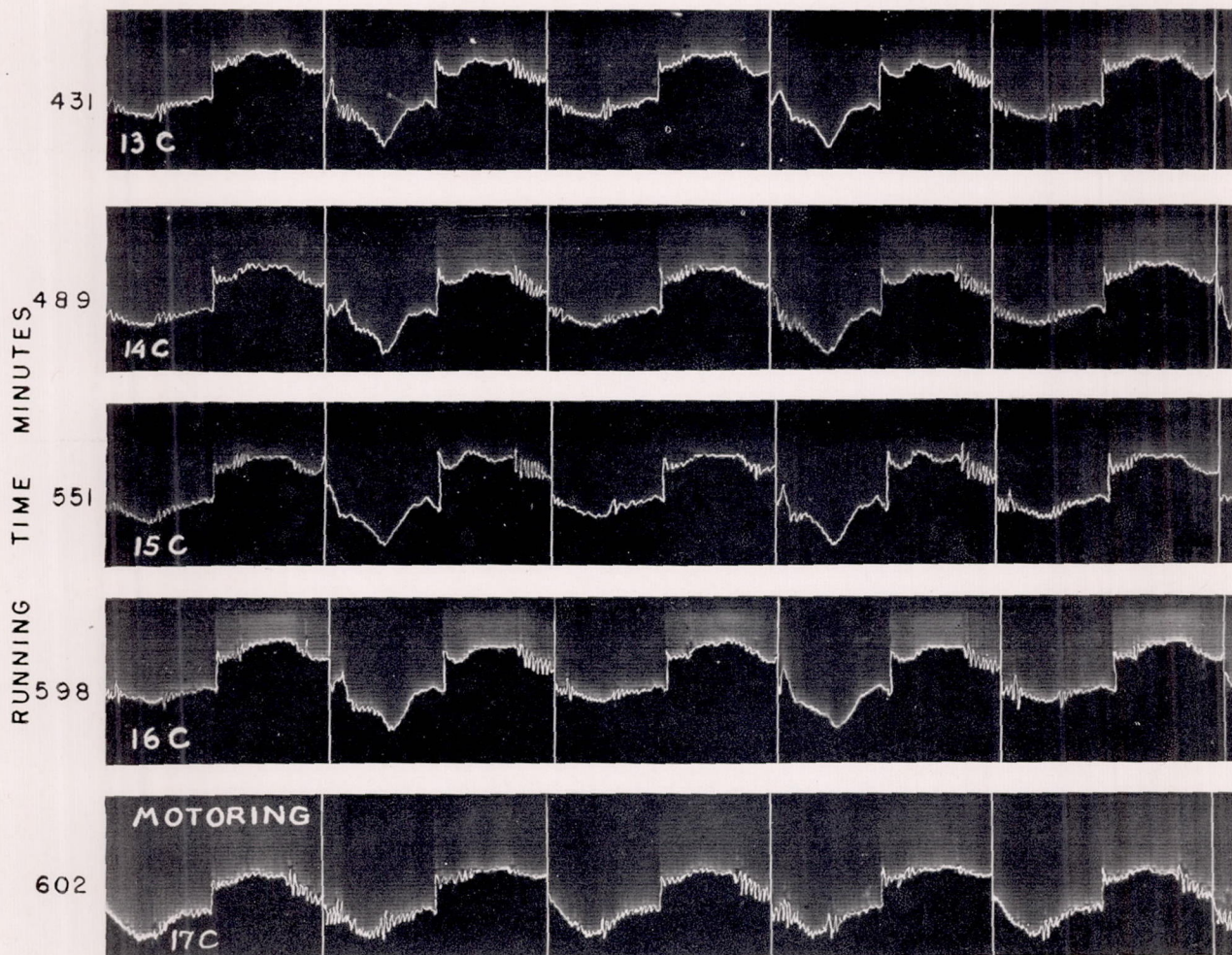
FIGURE 18.—Friction records for the run-in test with porous chrome-plated sleeve and cast-iron rings. (Records have been outlined for clearness.)
