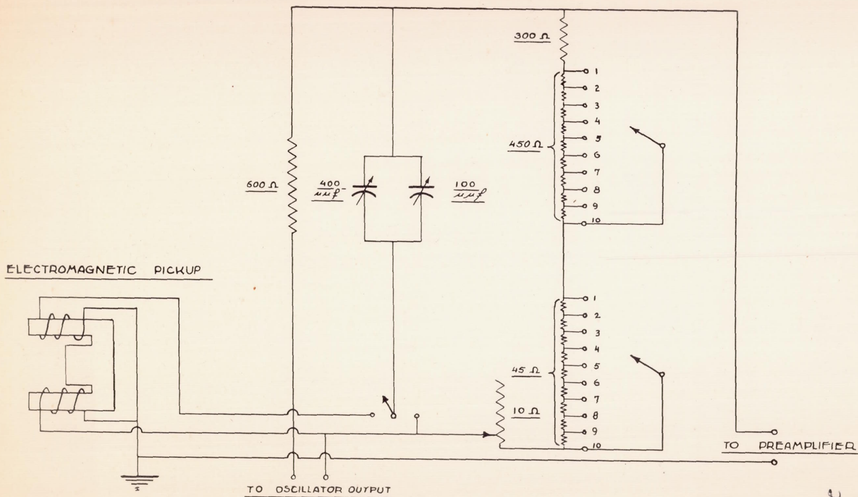
Figure 5.- Electrical diagram of bridge circuit.
