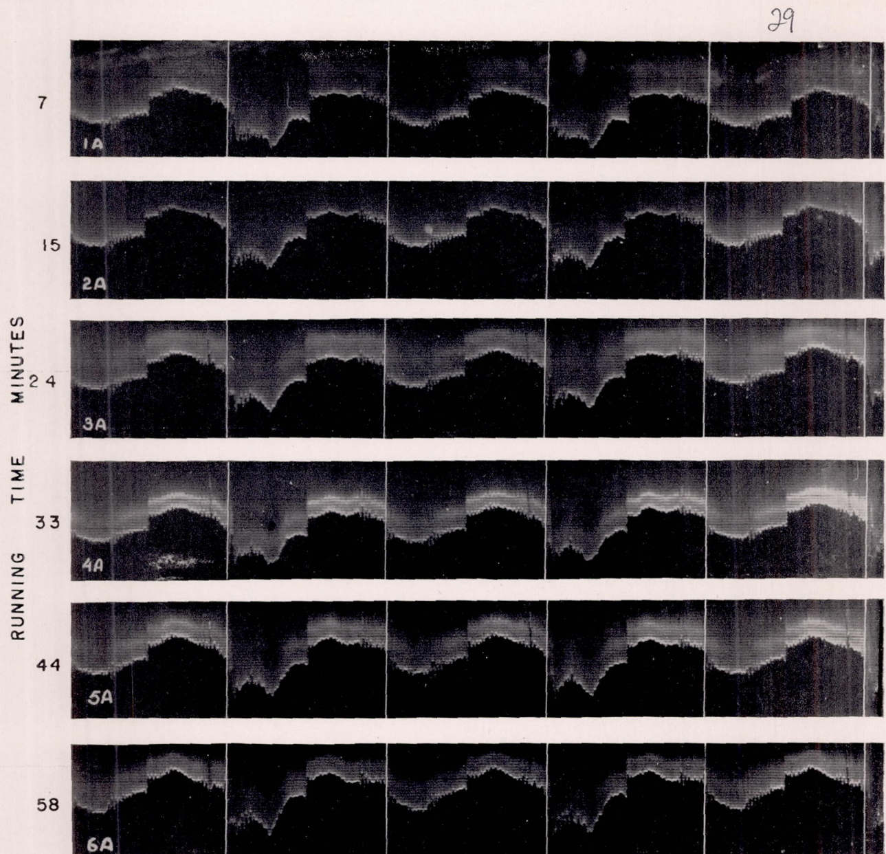
Figure 11.—Friction records for the run-in test with SAE 4140 sleeve and cast-iron rings.
