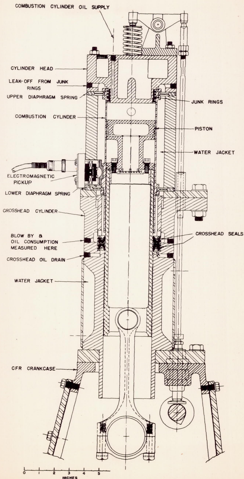
Figure 1.- Engine, showing crosshead and spring-mounted combustion cylinder.
