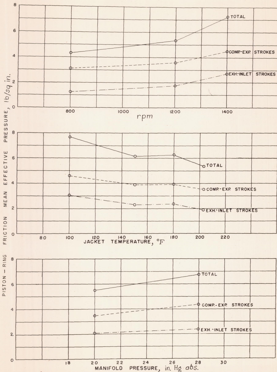
Figure 23.- The effect of engine speed, jacket temperature, and manifold pressure on piston-ring friction mean effective pressure.
