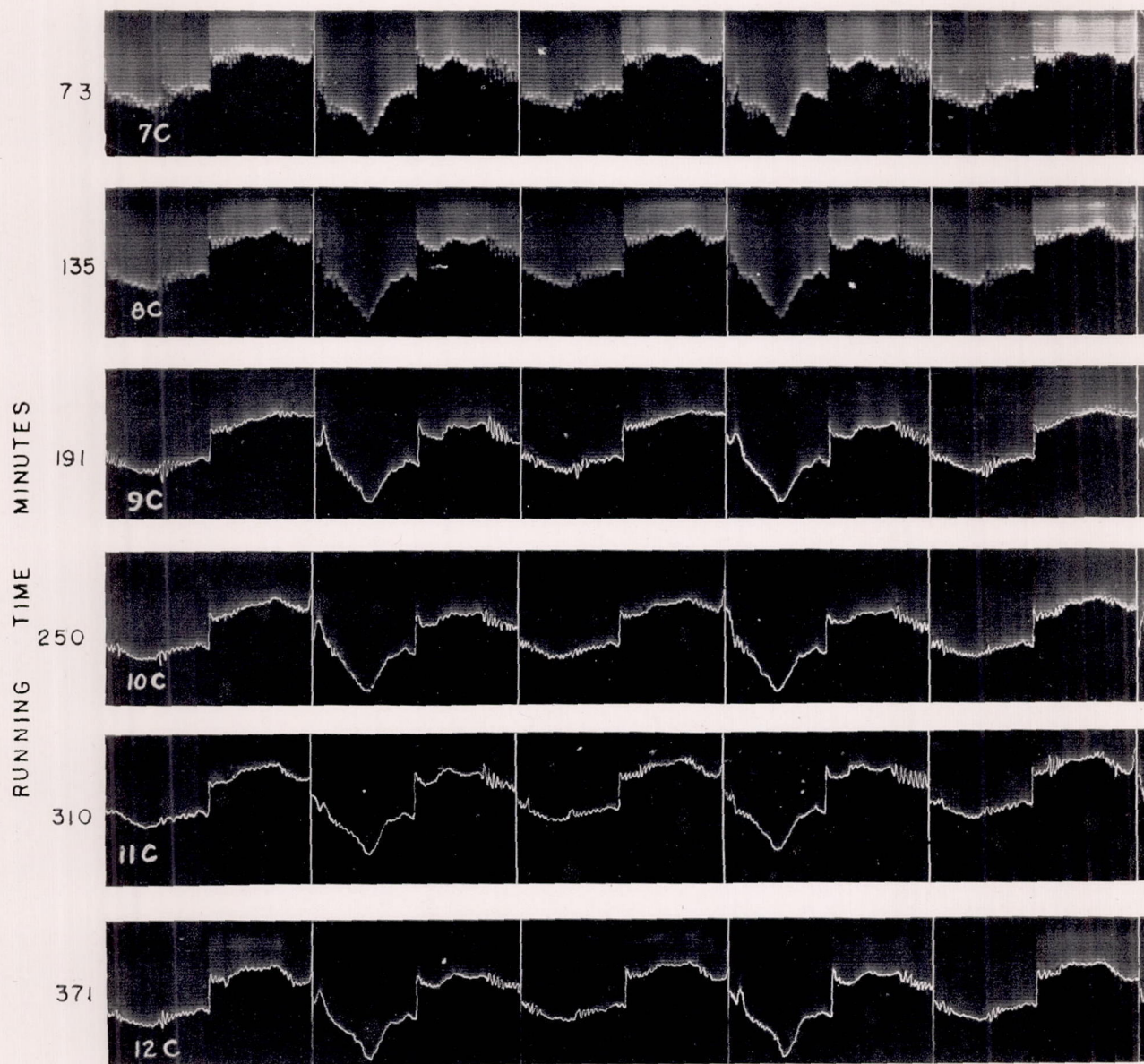
FIGURE 17.—Friction records for the run-in test with porous chrome-plated sleeve and cast-iron rings. (Records 9C to 12C have been outlined for clearness.)
