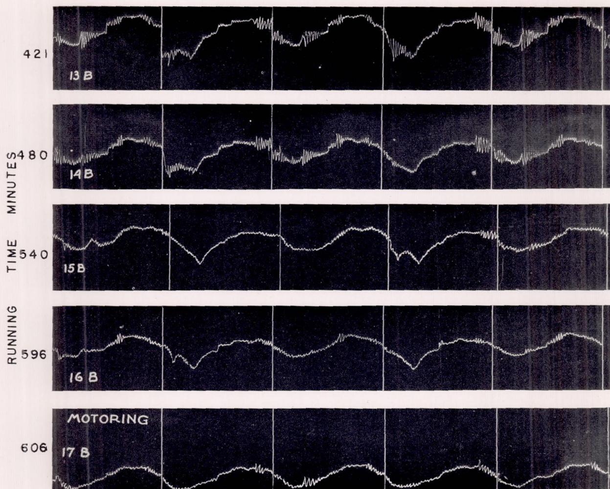
FIGURE 15.—Friction records for the run-in test with SAE 4140 sleeve and chrome-plated top ring. (Records have been outlined for clearness.)
