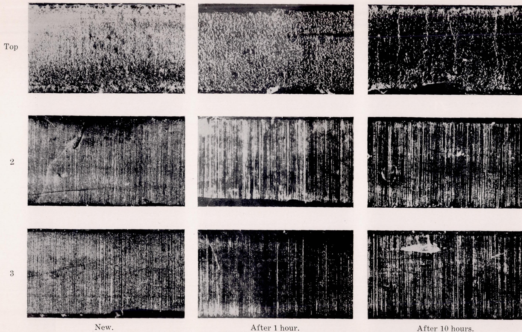
Figure 27.—Photomicrographs of surface replicas of rings used in run B. Top ring is porous chrome-plated. (25×).
