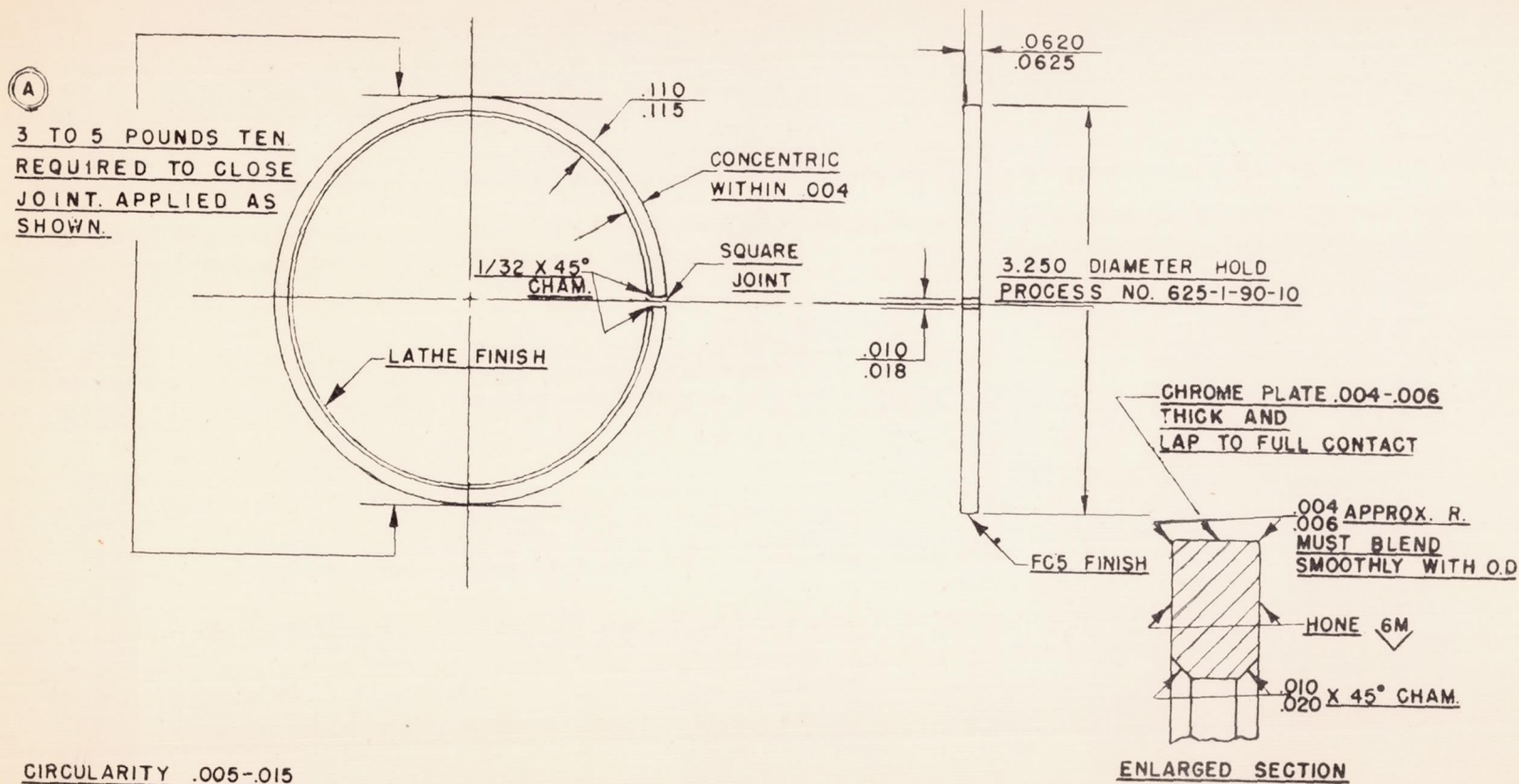
Figure 9.- Porous chrome-plated compression ring used in tests.
