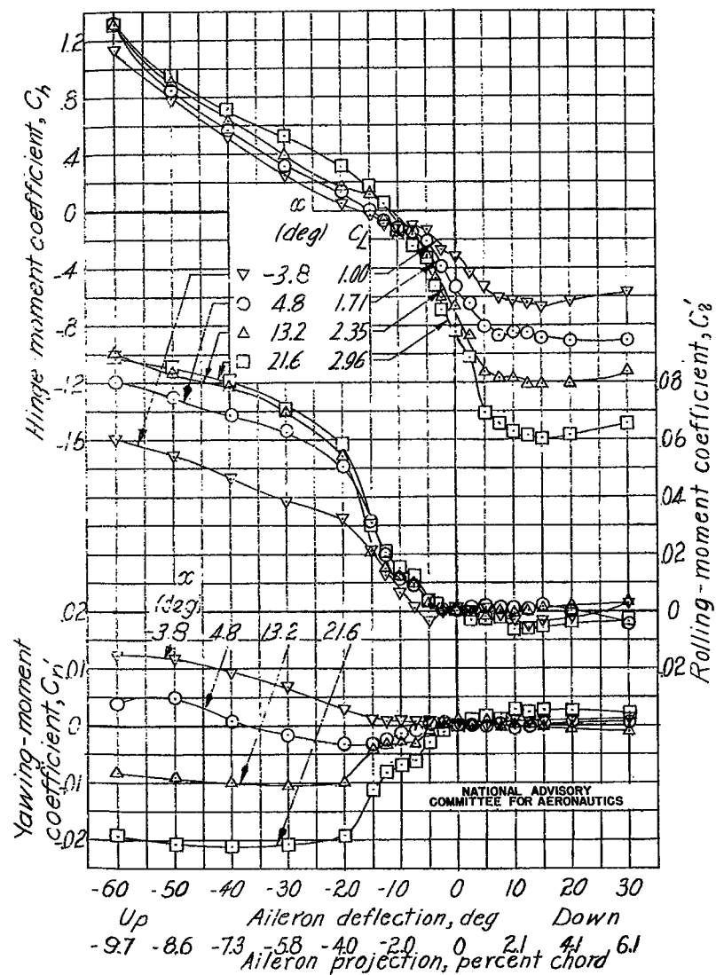
(c) Flap deflected 40°.
