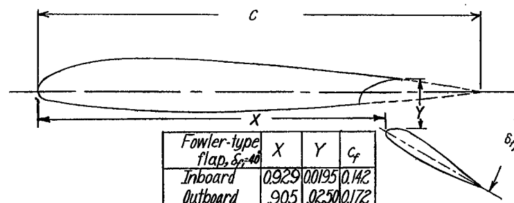
(a) Cross section of the Fowler-type flap.
