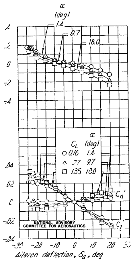
Figure C11.- Aerodynamic characteristics of a 0.15c by 0.37 b/2 sealed aileron with 0.35c a balance on an NACA 23-12 wing with a 0.33c by 0.63 b/2 inboard Fowler flap ( f_1 ) and a 0.23c by 0.37 b/2 outboard retractable balanced split flap ( f_2 ).
