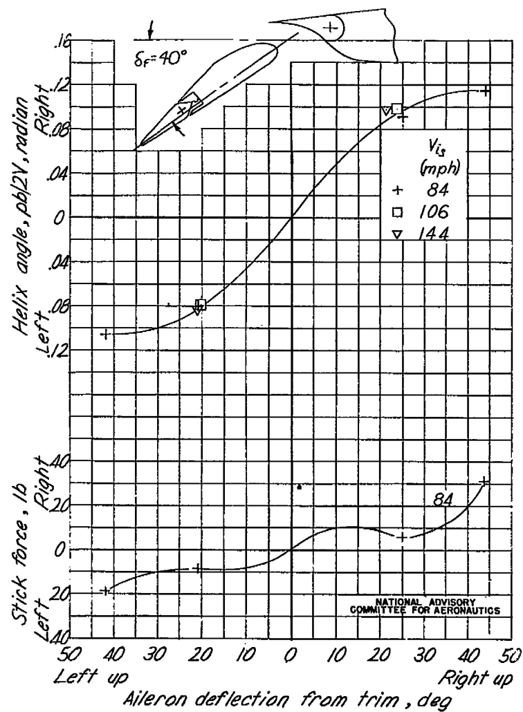
(c) Flap selector setting, 40^\circ .
