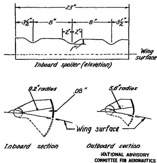
Figure B90.- Front elevation and sections of the spoiler tested on the airplane.
