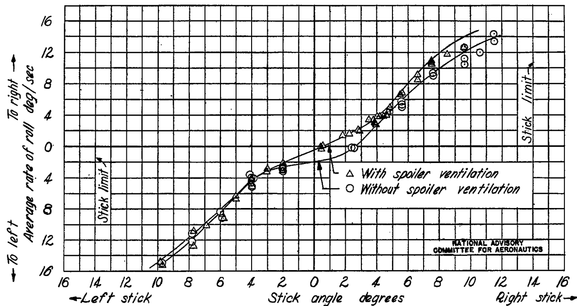
Figure B95.- Variation of average rate of roll due to spoiler deflection with stick angle for the airplane. Flaps full down and ailerons drooped 29^\circ , 11.5 miles per hour above stall.
