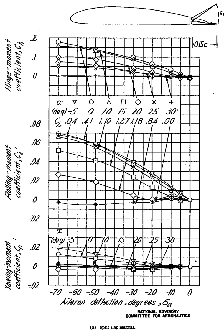
Figure B16.- Aileron characteristics of the 0.15c upper-surface aileron on the Clark Y wing.
