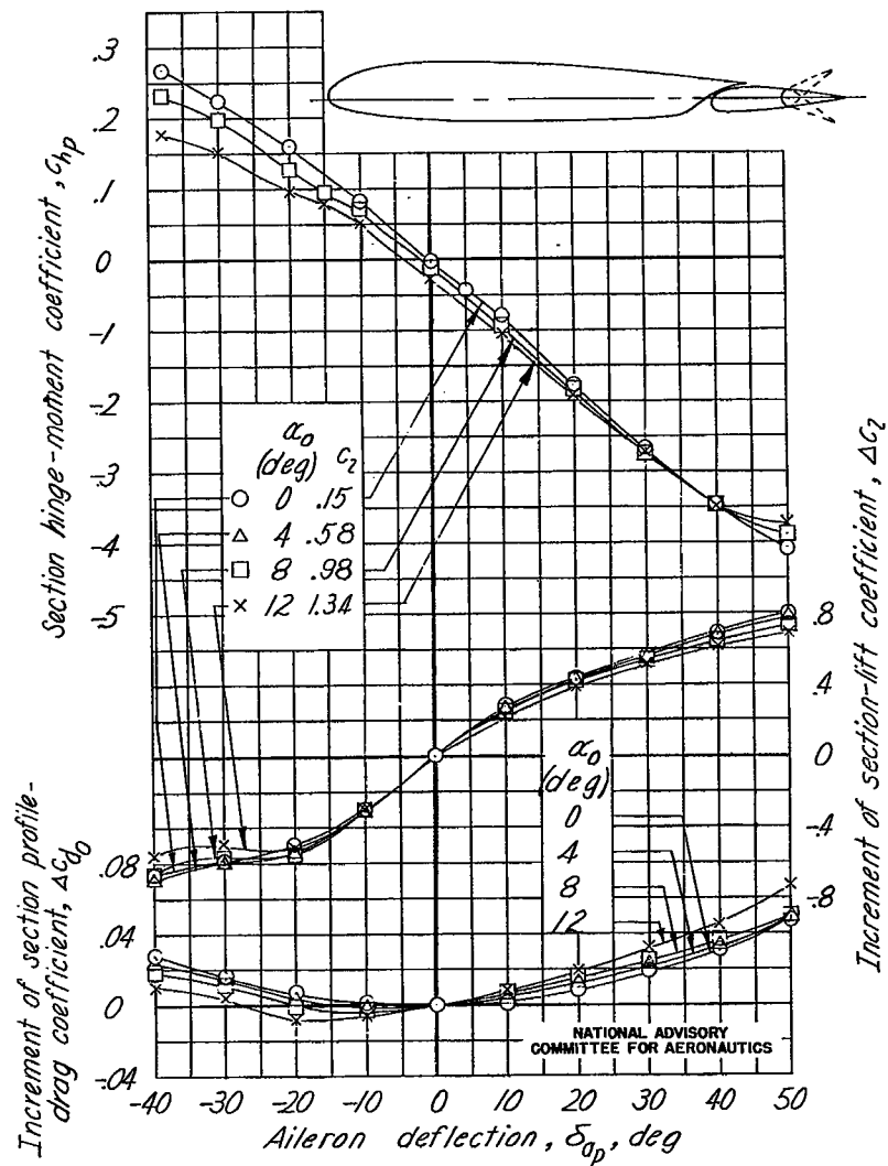
(a) \delta_p, 0^\circ . Figure A3.- Effect of plain aileron deflection on the section aerodynamic characteristics of an NACA 23012 airfoil equipped with a full-span slotted flap.
