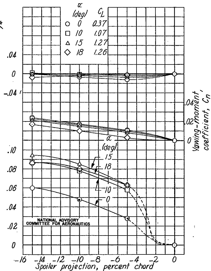
Figure B19.- Rolling-, yawing-, and pitching-moment characteristics of the Clark Y wing due to retractable spoiler projection. Flap retracted.
