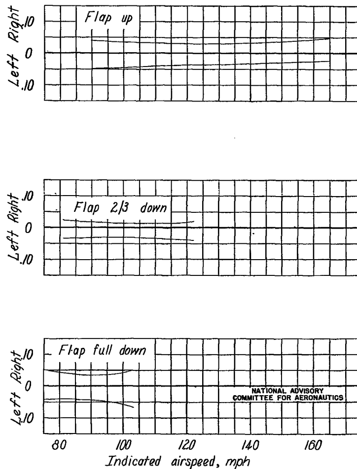
Figure B102.- Variation of the helix angle pb/2V with airspeed for a lateral stick force of 30 pounds or less, power-off conditions.
