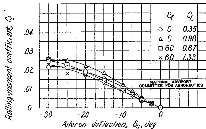
Figure B23.- Variation of rolling-moment coefficient with plain sealed aileron deflection on the Clark Y-15 airfoil.
