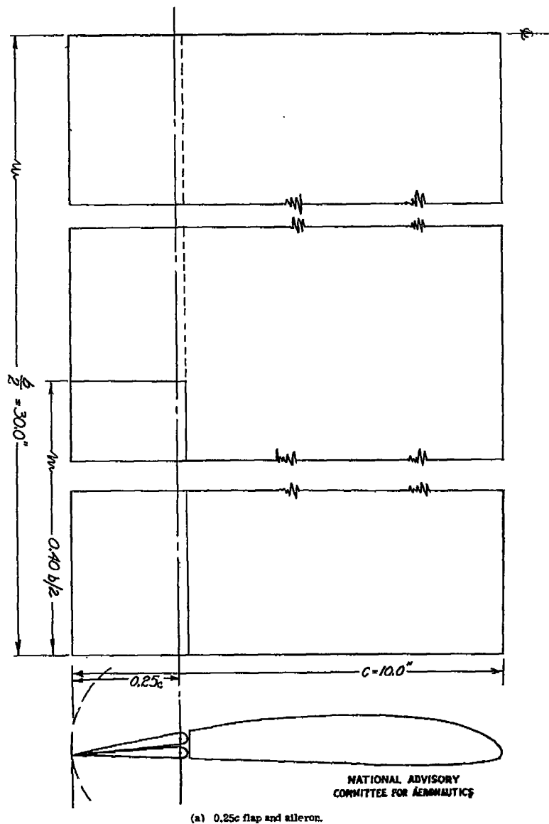
(a) 0.25c flap and aileron.
