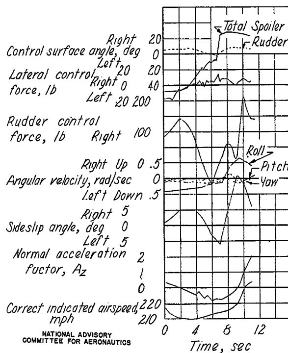
Figure B128.- Time history of a maneuver showing the spoiler effectiveness in approximately inverted flight. Ailerons fixed in neutral position, climb condition (power on, flaps up).
