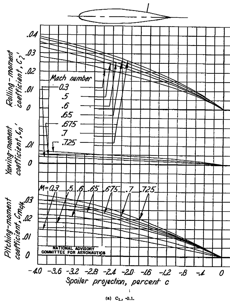
Figure B69.- Variation of rolling-, yawing-, and pitching-moment characteristics with spoiler projection for the wing of a fighter-type airplane.
