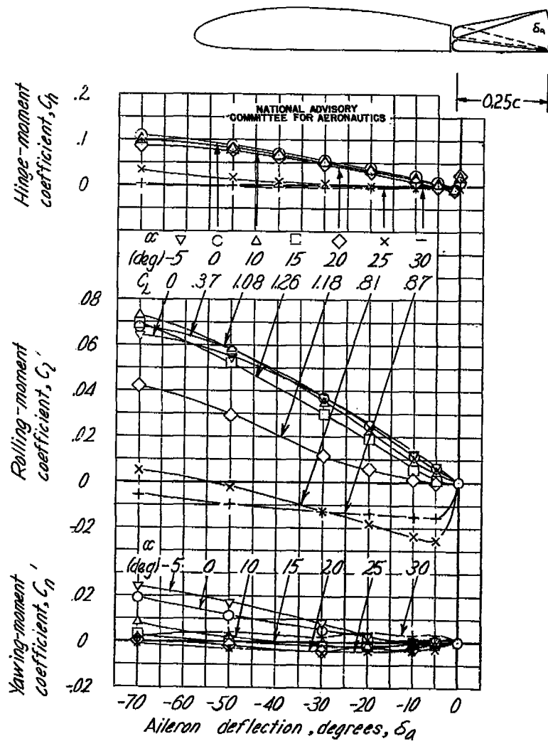
(a) Split flap neutral.
