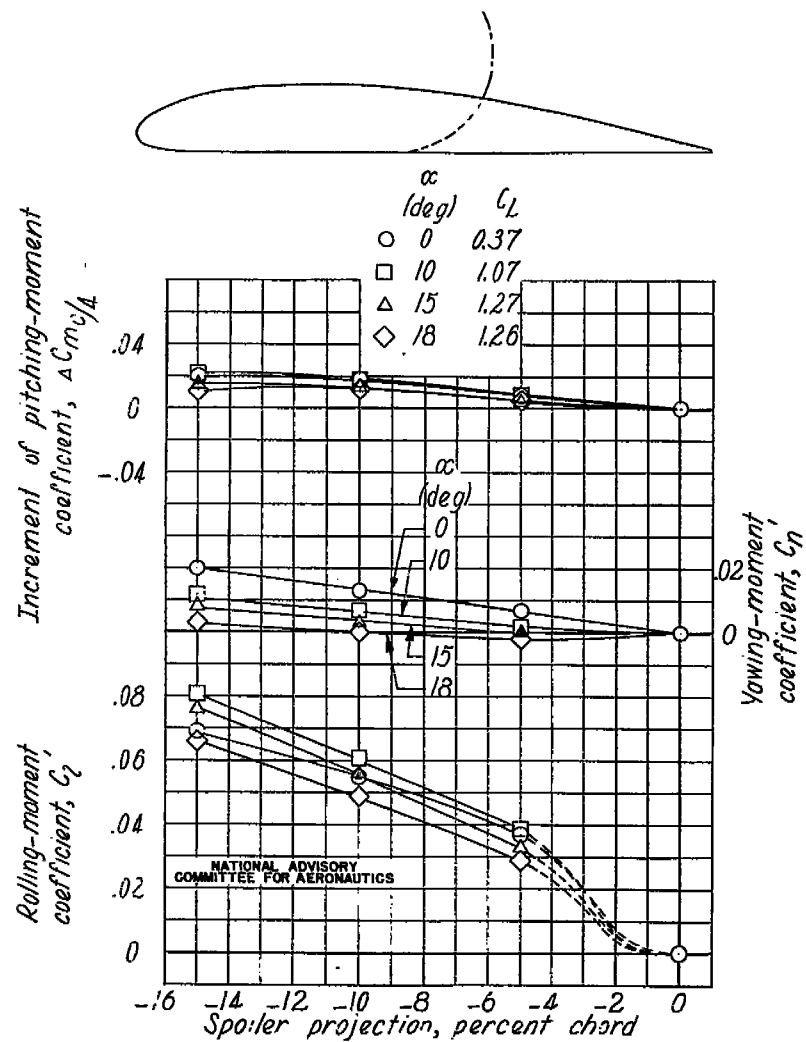
(b) Spoiler located at 0.80c. Figure B19.- Continued.
