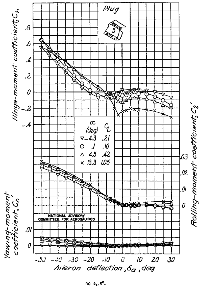
Figure B59.- Rolling-, yawing-, and hinge-moment coefficients due to aileron deflection at various angles of attack for the tapered-wing model with a full-span flap and plug aileron 5; \delta_f, 0^\circ .
