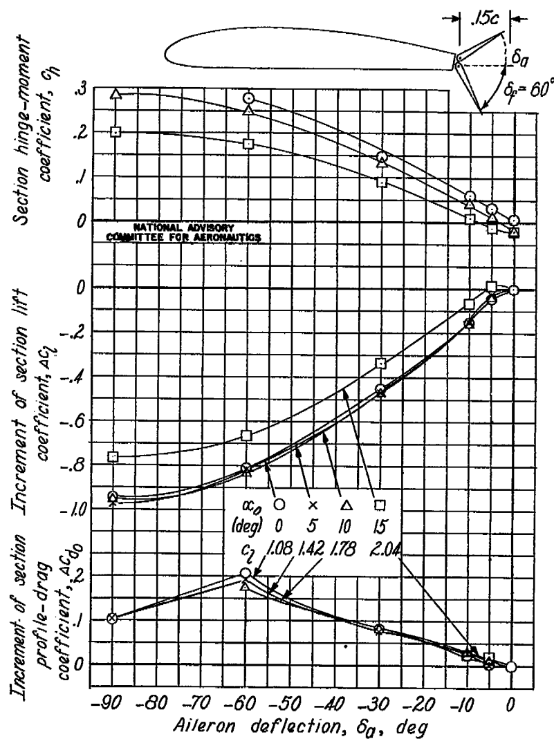
(b) Flap down 60^\circ .
