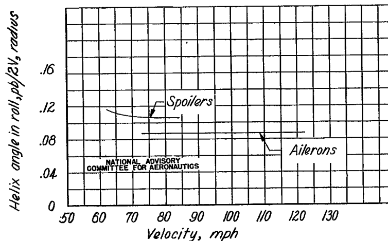
Figure B107.- Variation of helix angle in roll with velocity for a full stick displacement.
