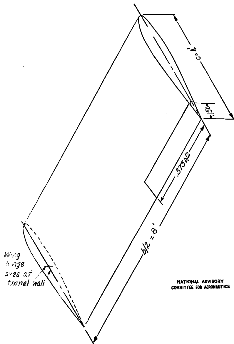
Figure B30.- Schematic diagram of the 4- by 8-foot wing model as tested in the Langley 7- by 10-foot tunnel. Span of all lateral-control devices, 3 feet.
