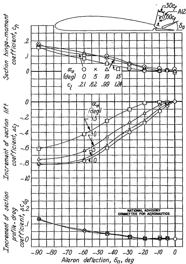
Figure B4.- Characteristics of the balanced upper-surface aileron at axis A12 on the Clark Y airfoil.
