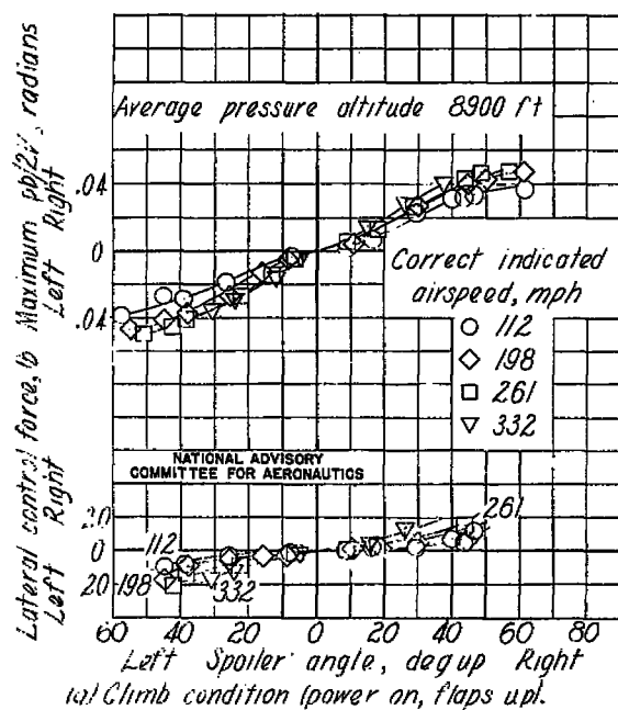
Figure B131.- Variation of the maximum heux angle pb/2v and control-wheel force with spoiler angle in abrupt rudder-fixed rolls. (Ailerons fixed in neutral position).
