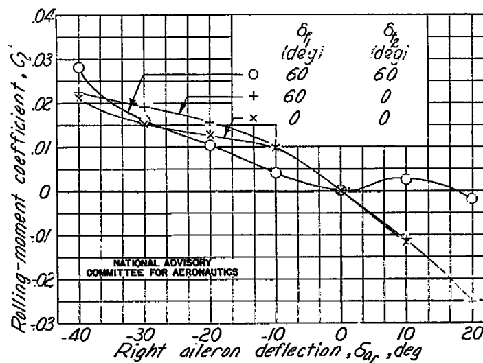
Figure C32.- Effect of flap deflection on the lateral control of the full-span flap model. \alpha = 10^\circ .
