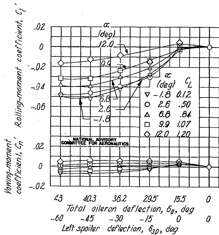
(a) \delta_a, 0^\circ . Figure B73.- Effect of spoiler and aileron deflection on the rolling- and yawing-moment characteristics of the 0.08-scale airplane model.
