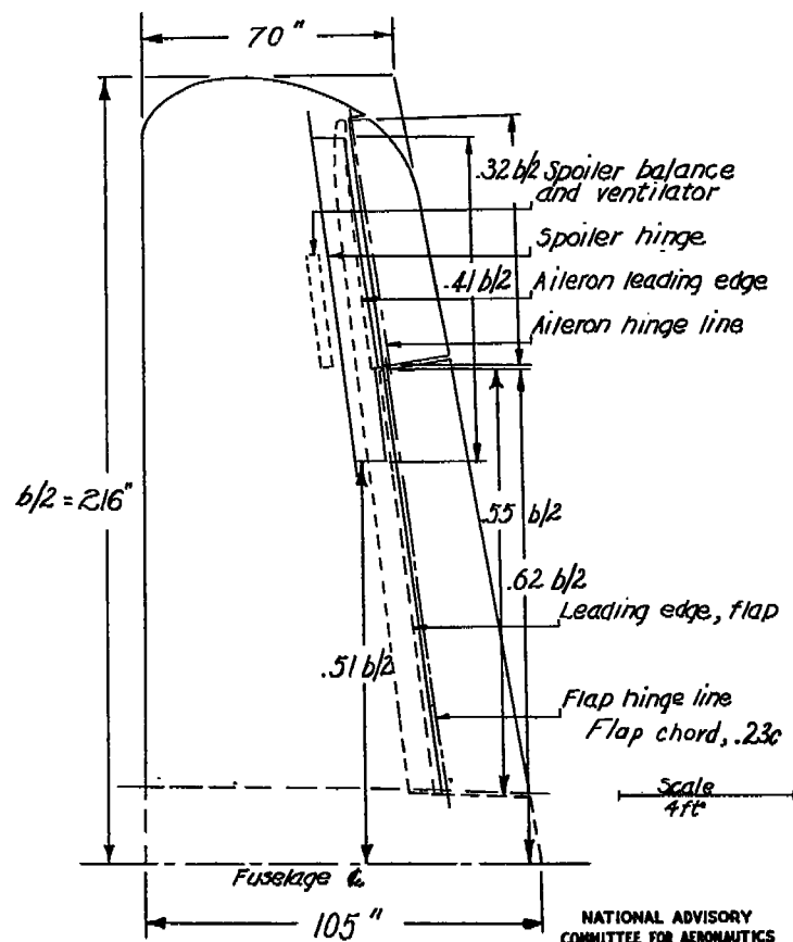
Figure B92.- Plan form of the semispan wing of a scout-observation-type airplane tested in flight by Vought-Sikorsky Aircraft.
