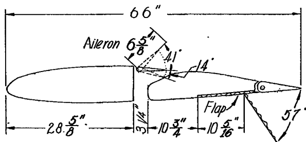
Section with slot-lip aileron at 0.45c
