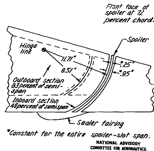
Figure B125.- Cut-away view of spoiler-slot arrangement on the wing of the fighter-type airplane.
