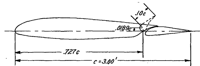
Slot-lip-aileron configuration
