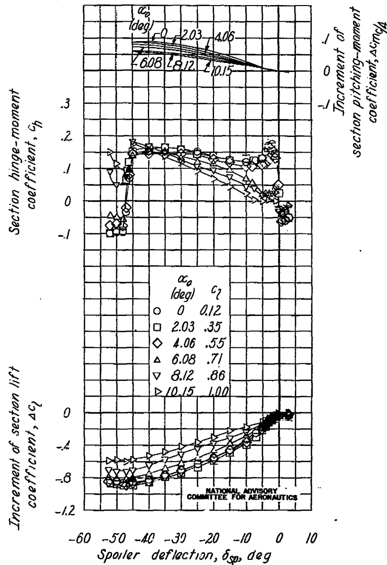
Figure B14.- Effect of spoiler deflection on the section lift, pitching-moment, and hinge-moment characteristics of the NACA 60(215)-216 airfoil. Spoiler thickness, 0.0028c; forward gap, 3.0013c; rear gap, 0.1100c; spoiler beveled 17° on both faces. Roughness on upper surface.
