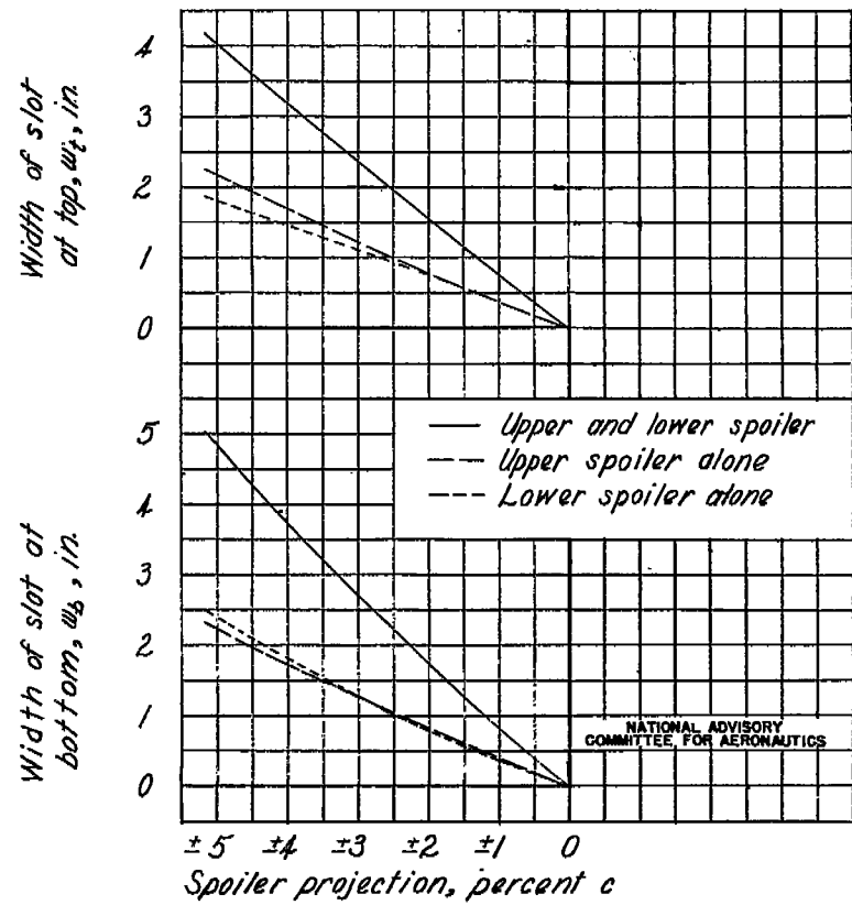
Figure B22.- Variation of spoiler-slot width with spoiler projection.
