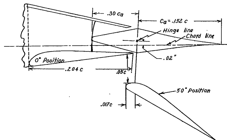
(b) Cross section and dimensions of sealed aileron and balanced split flap.
