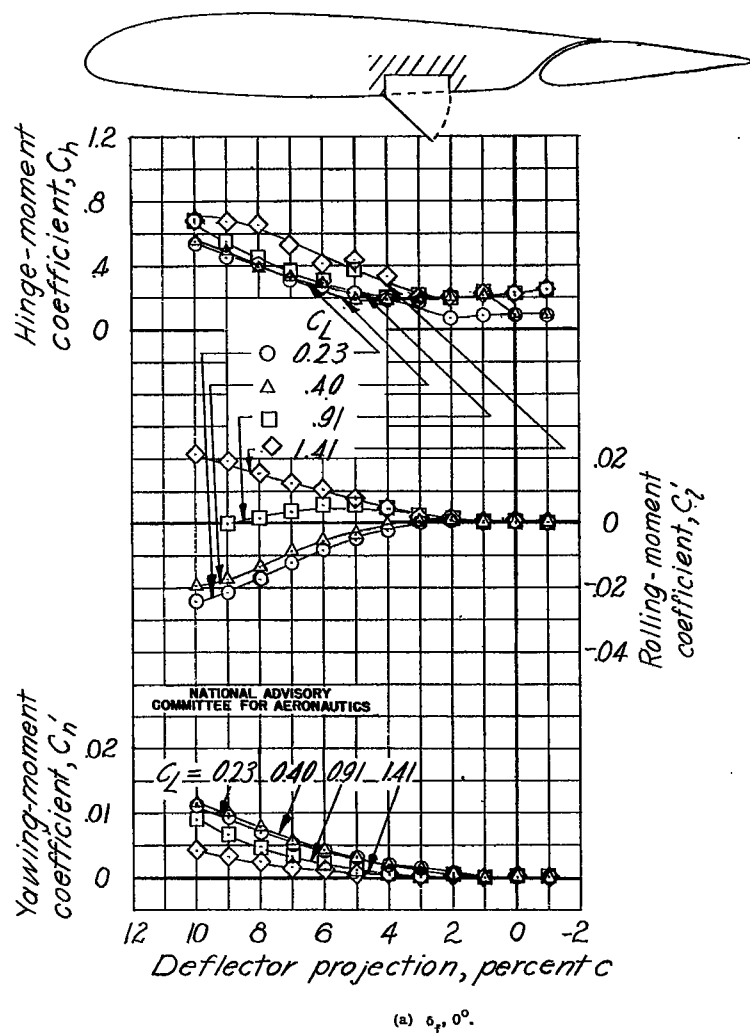
Figure B35.- Aileron characteristics of a 0.10c deflector hinged at 0.50c on an NACA 23012 wing with a 0.2566c full-span slotted flap.
