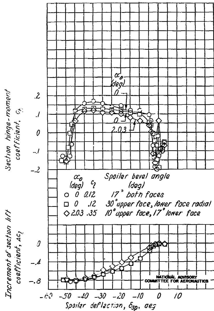
Figure B13.- Effect of spoiler deflection and spoiler bevel angle on the section lift and hinge-moment characteristics of the NACA 60(215)-216 airfoil. \delta_p , 3°. Spoiler thickness, 0.0028c; spoiler upper face smooth.
