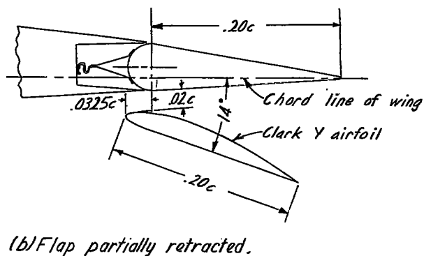
Figure C48.- Sections of internally balanced aileron and balanced split-flap arrangement as tested on a personal-type airplane.
