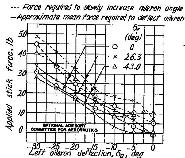
Figure B78.- Stick forces required to deflect the left aileron with the flap in various positions. Approximate test speed, 28 miles per hour. Langley full-scale wind tunnel.
