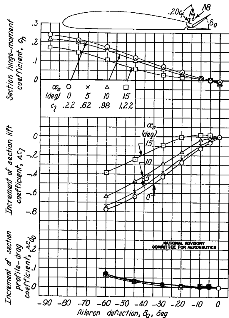
Figure B5.- Characteristics of the balanced upper-surface aileron at axis A 8 on the Clark Y airfoil.
