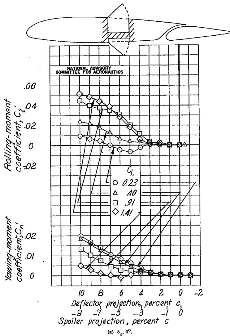
Figure B37.- Aileron characteristics of a 0.10c spoiler and a 0.10c deflector on an NACA 23012 wing with a 0.2568c full-span slotted flap; spoiler and deflector hinged at 0.50c.
