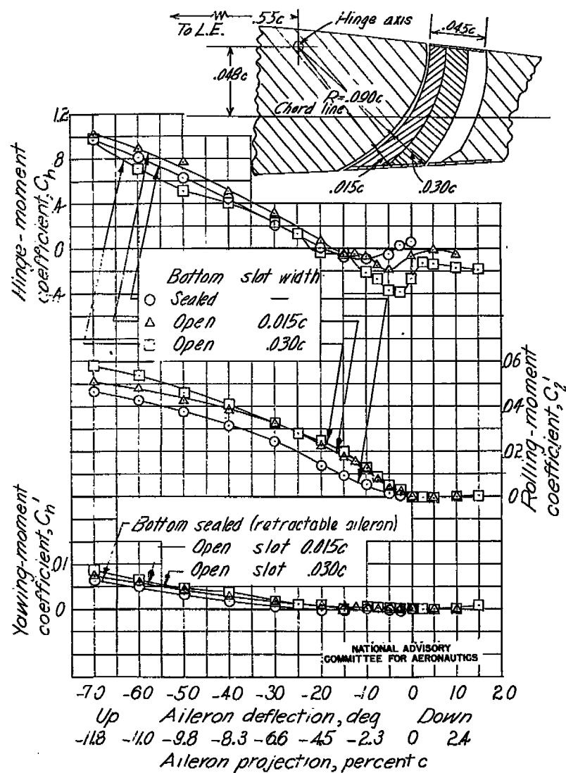
(a) Flap neutral; \alpha , 8.7^\circ ; C_L , 0.77.
