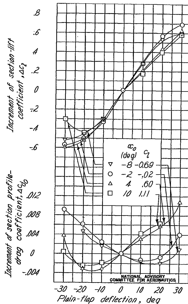
(a) Slotted flap retracted, \delta_f = 0^\circ .
