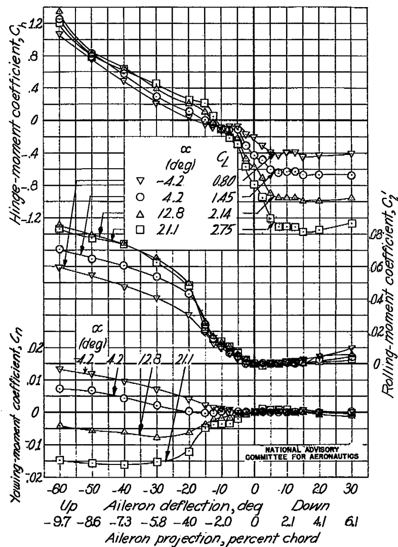
(b) Flap deflected 30^\circ .
