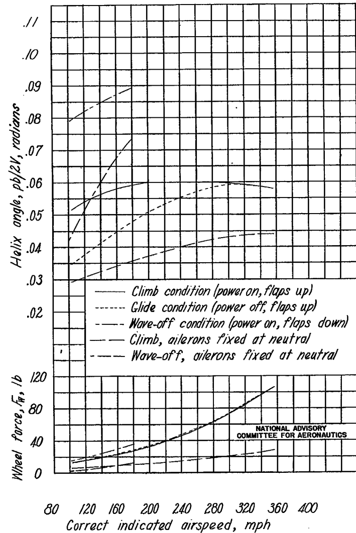
Figure B133.- Variation of maximum helix angle and wheel force with airspeed. Spoiler deflected 40° up. (Spoilers and ailerons deflected unless otherwise indicated.)
