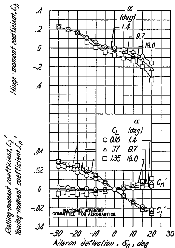
Figure C8.- Aerodynamic characteristics of a 0.15c by 0.37 b/2 sealed aileron with 0.30c balance on an NACA 23012 wing with a 0.30c by 0.63 b/2 inboard Fowler flap ( f_1 ) and a 0.30c by 0.37 b/2 outboard retractable plain split flap ( f_2 ).
