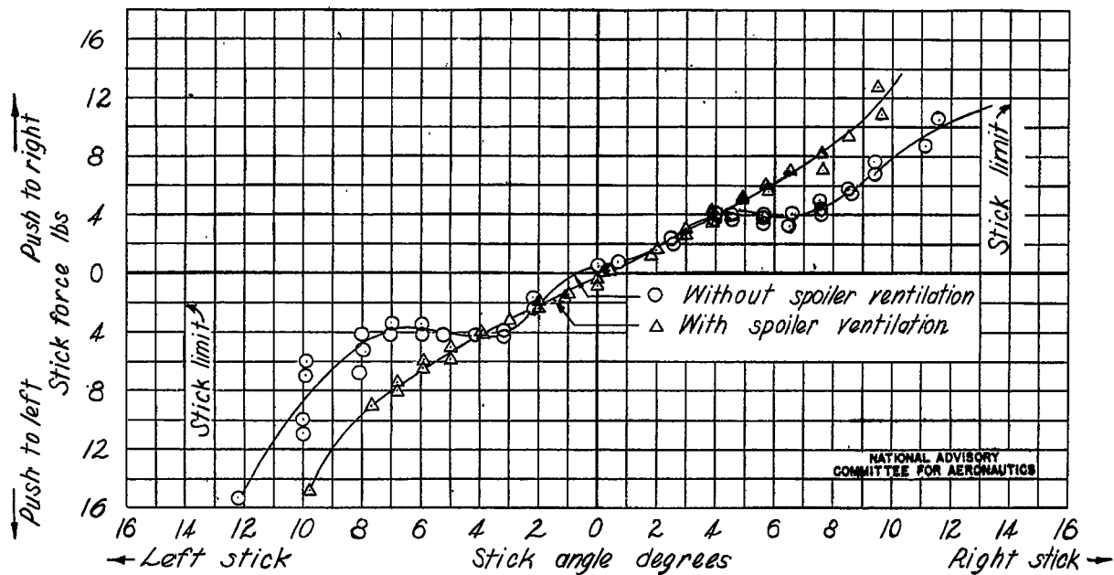
Figure B96.- Variation of stick force with stick angle for the airplane. Flaps full down and ailerons drooped 29^\circ , 11.5 miles per hour above stall.
