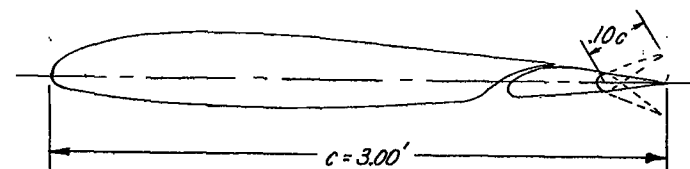
Plain-aileron configuration
