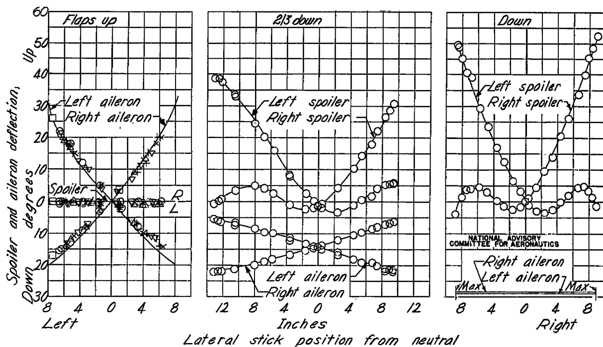
Figure B98.- Variation of aileron and spoiler angles with stick position as measured on the ground with no load on the surfaces.
