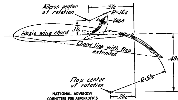
Figure B109.- Cross-sectional drawing of the wing showing the aileron and flap extended and retracted.
