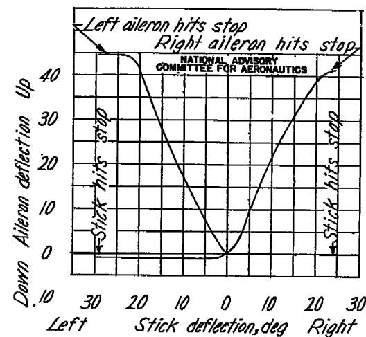
Figure B77.- Variation of aileron deflection with control-stick deflection.
