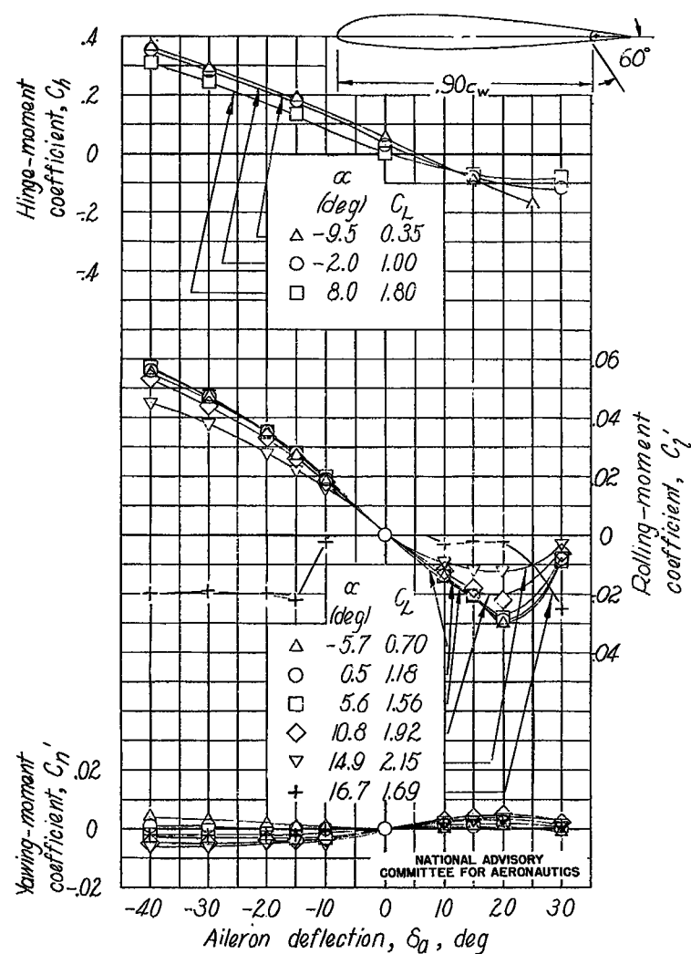
(b) Flap deflection, 60^\circ .
