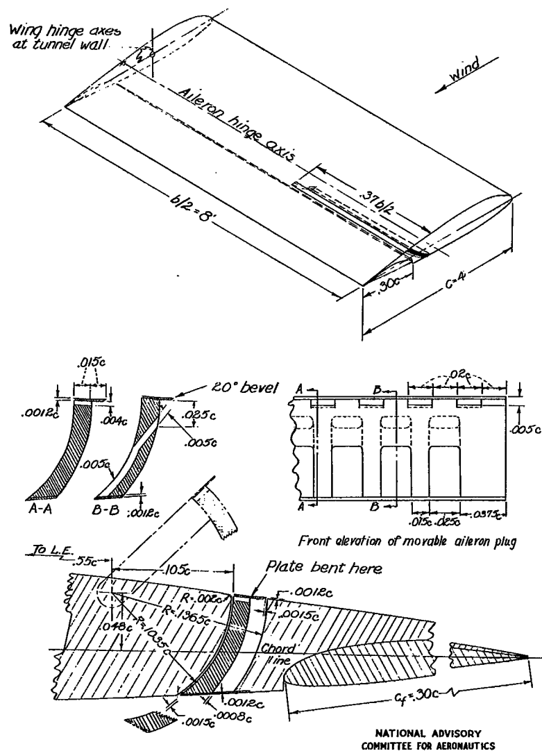
Figure B51.- Schematic diagram of model setup and details of the 0.37 b/2 plug-type aileron on a 4- by 8-foot semispan NACA 23012 wing with a 0.30c full-span Fowler flap.
