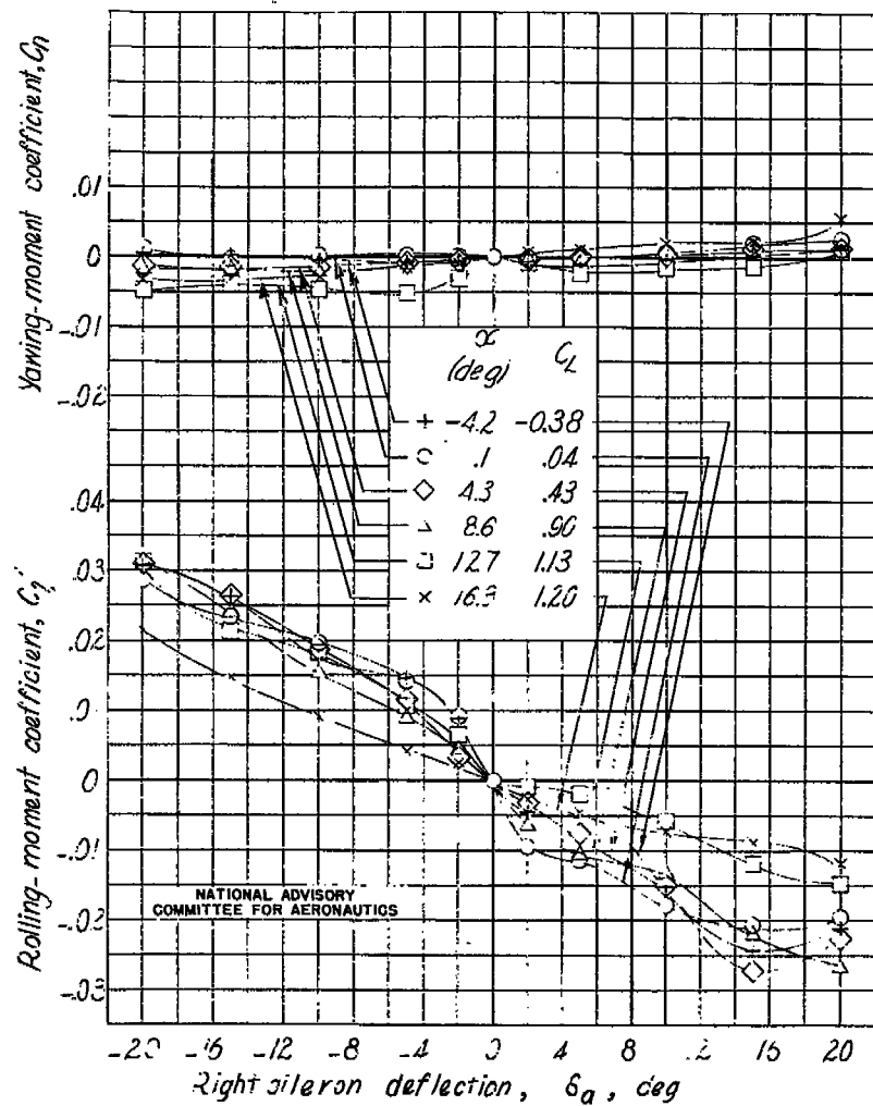
Figure 24(b). Variation of the rolling and yawing moment coefficients with aileron deflection on the \frac{1}{2} -scale model.
