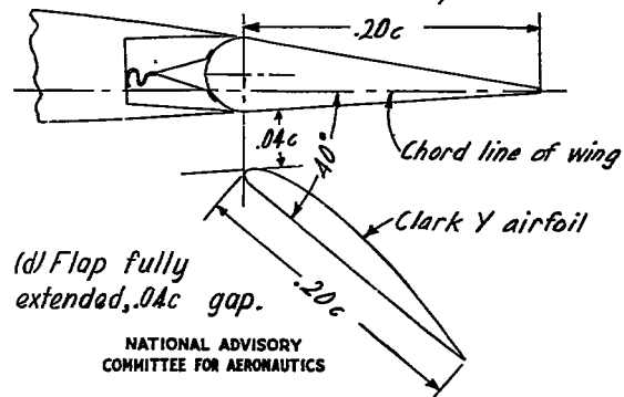
Figure C48.- Sections of internally balanced aileron and balanced split-flap arrangement as tested on a personal-type airplane.
