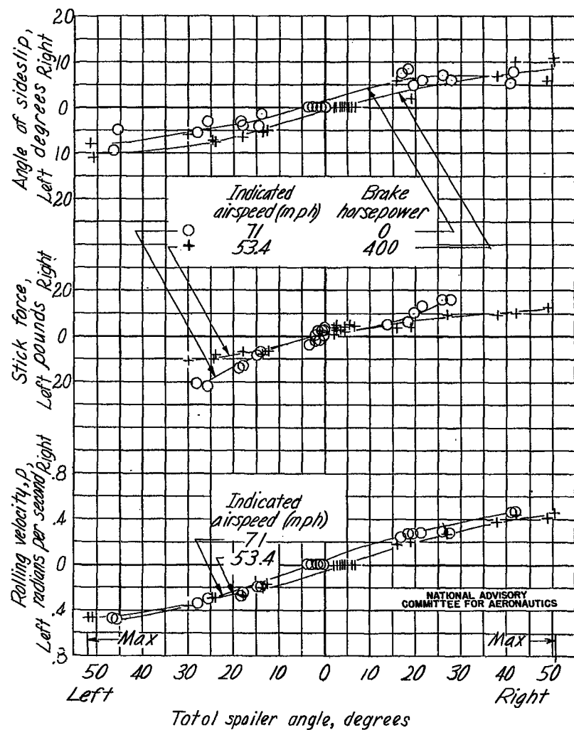
(c) Flaps down. Figure B101.- Concluded.
