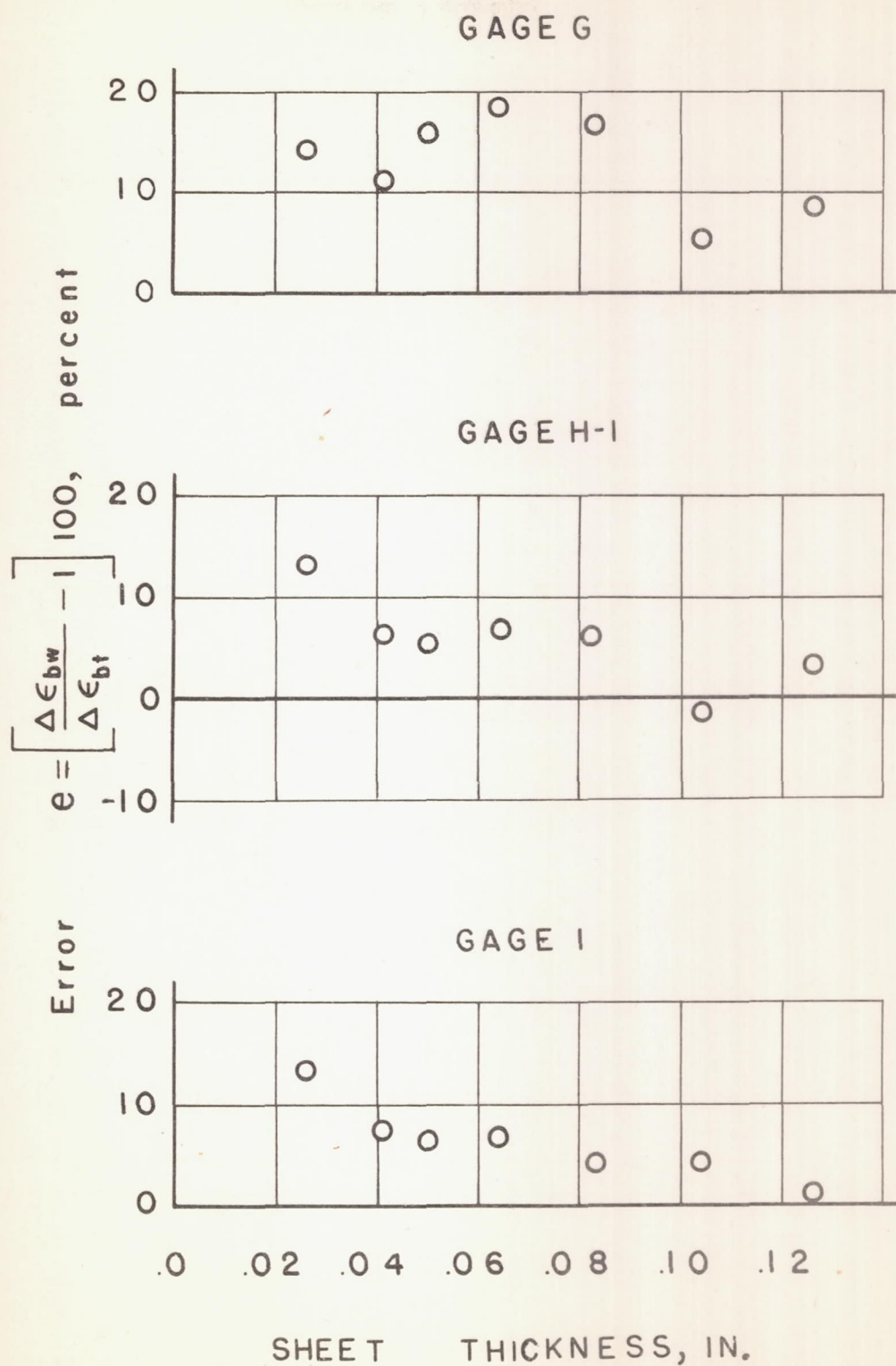
Figure 4.- Average error in the extreme-fiber strain, indicated by wire gages G, H-1, and I, plotted against sheet thickness.
