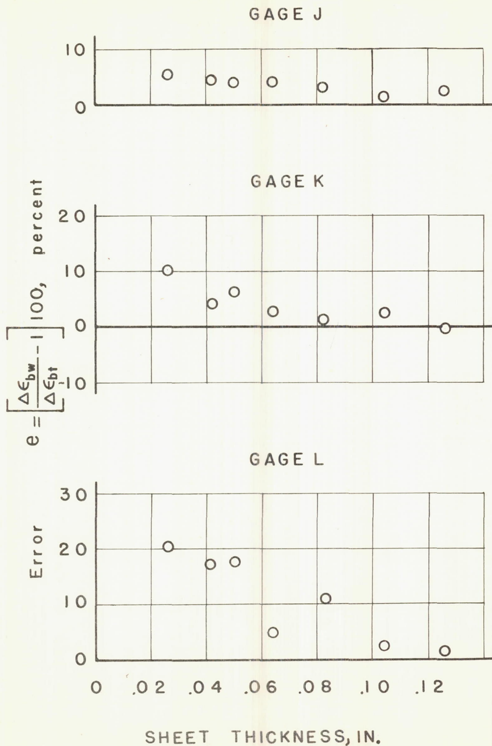
Figure 5.- Average error in the extreme-fiber strain, indicated by wire gages J, K, and L, plotted against sheet thickness.
