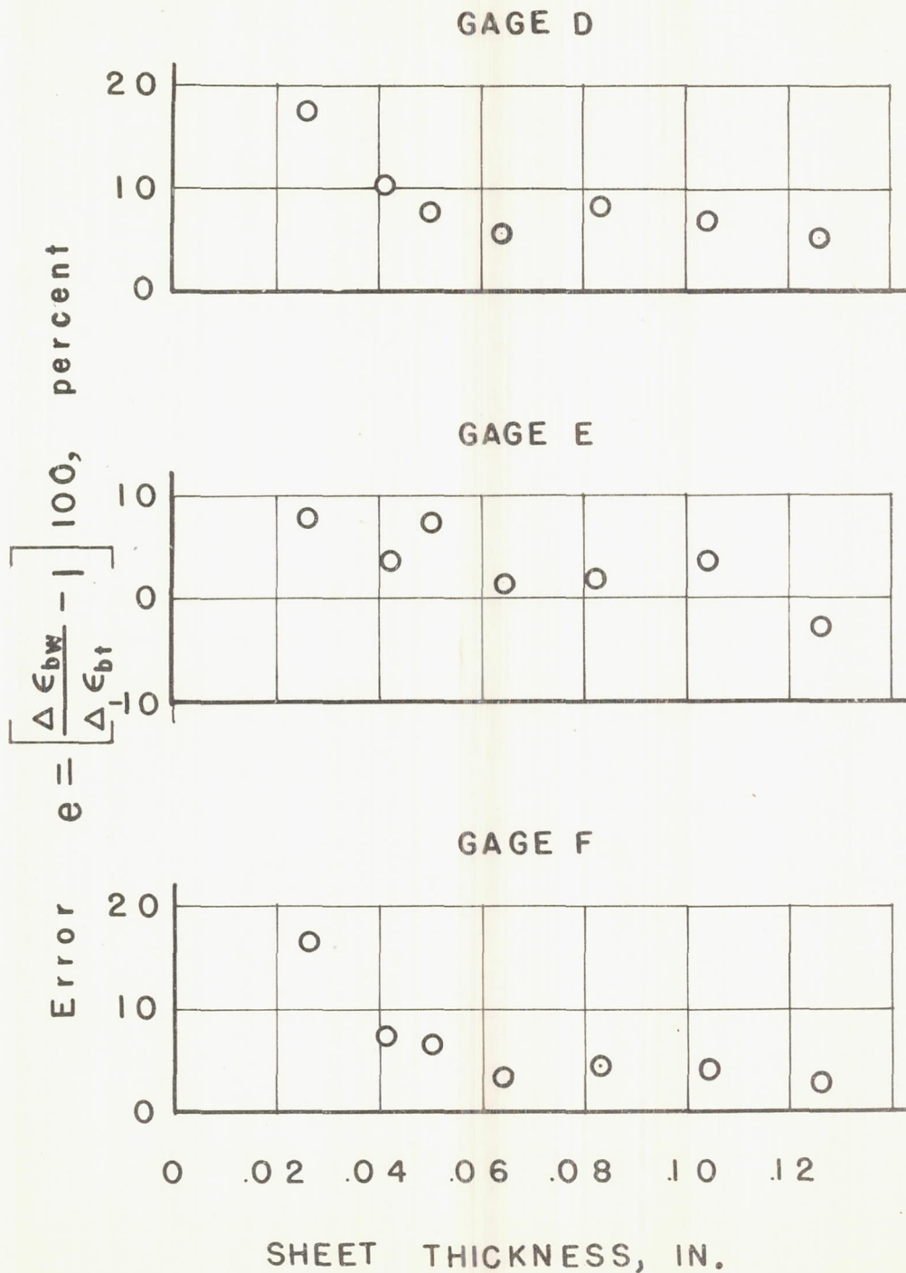
Figure 3.- Average error in the extreme-fiber strain, indicated by wire gages D, E, and F, plotted against sheet thickness.
