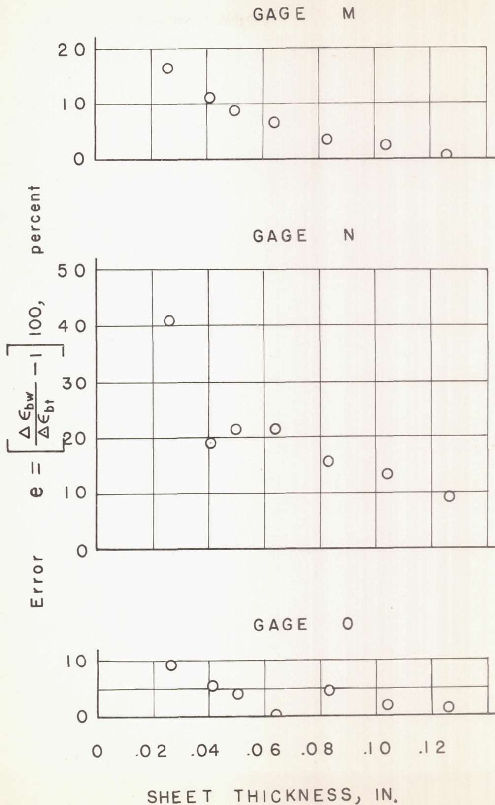
Figure 6.- Average error in the extreme-fiber strain, indicated by wire gages M, N, and O, plotted against sheet thickness.
