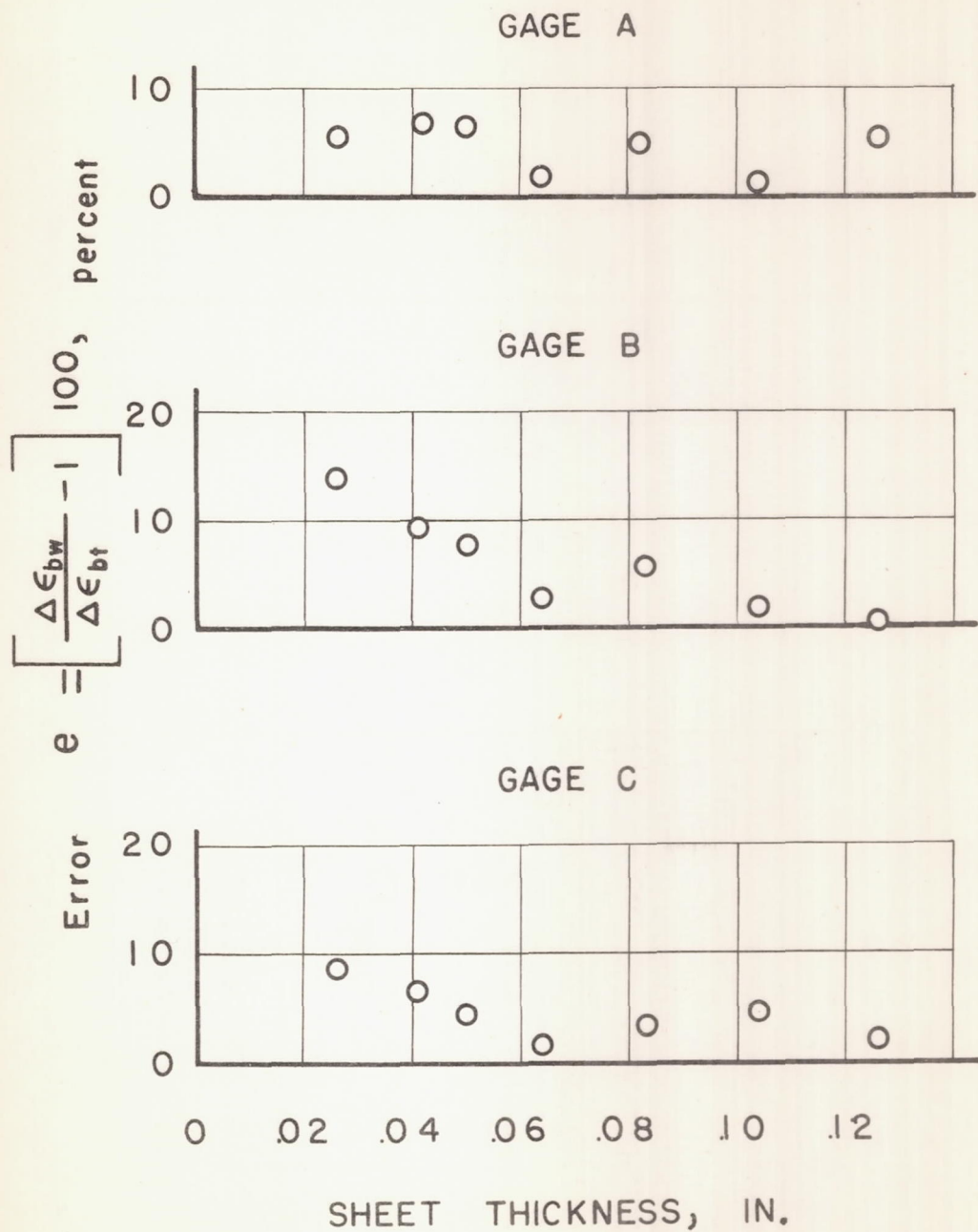
Figure 2.- Average error in the extreme-fiber strain, indicated by wire gages A, B, and C, plotted against sheet thickness.
