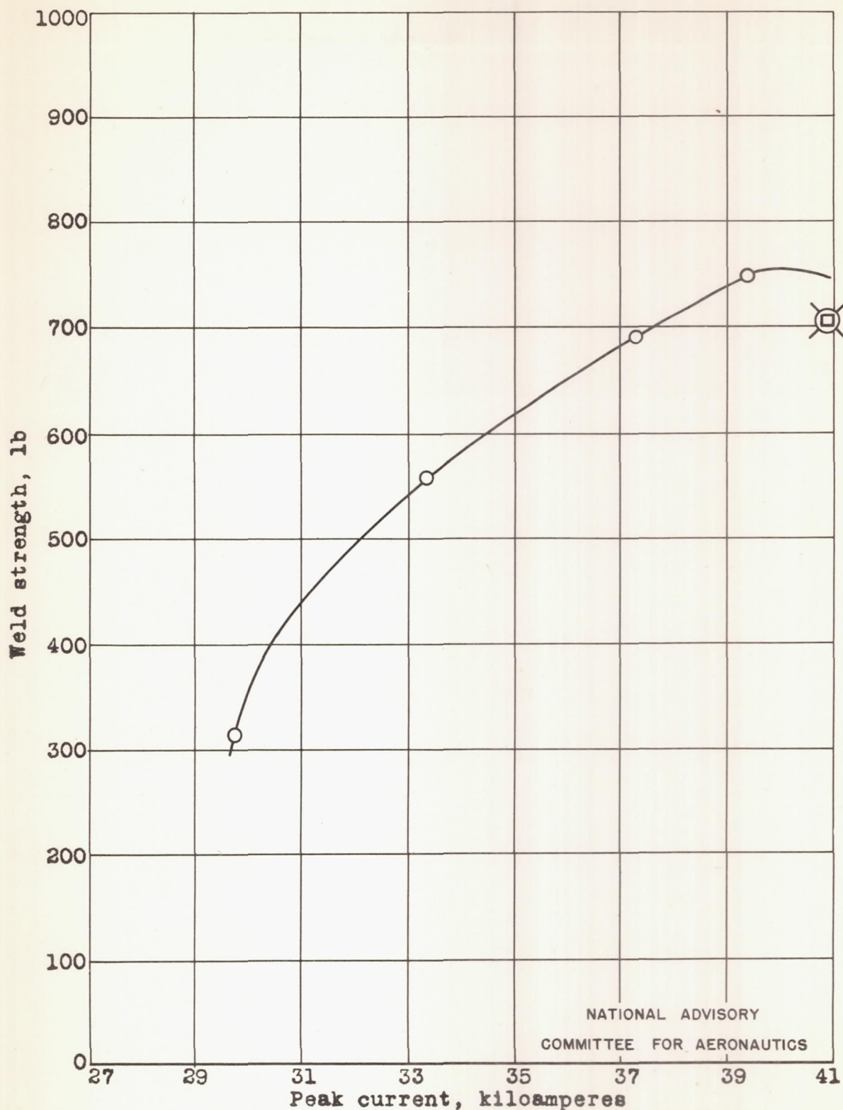
Figure 18.- Strength-current characteristic of clad XB75S-T to bare XB75S-T. Thickness of both alloys, 0.040 inch; electrode dome-tip radius, 4 inches; electrode force, 1200 pounds (weld), 2000 pounds (forge); forge timing, 38 milliseconds; average rate of current rise, 3120 amperes per millisecond.
