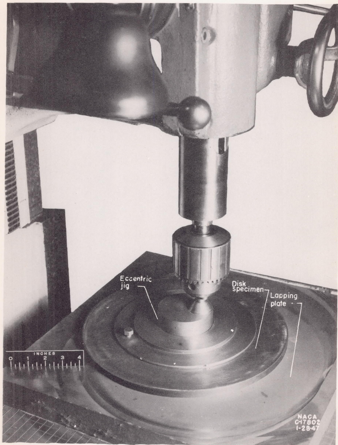
Figure 3. - Lapping apparatus used in preparation of disk specimen.
