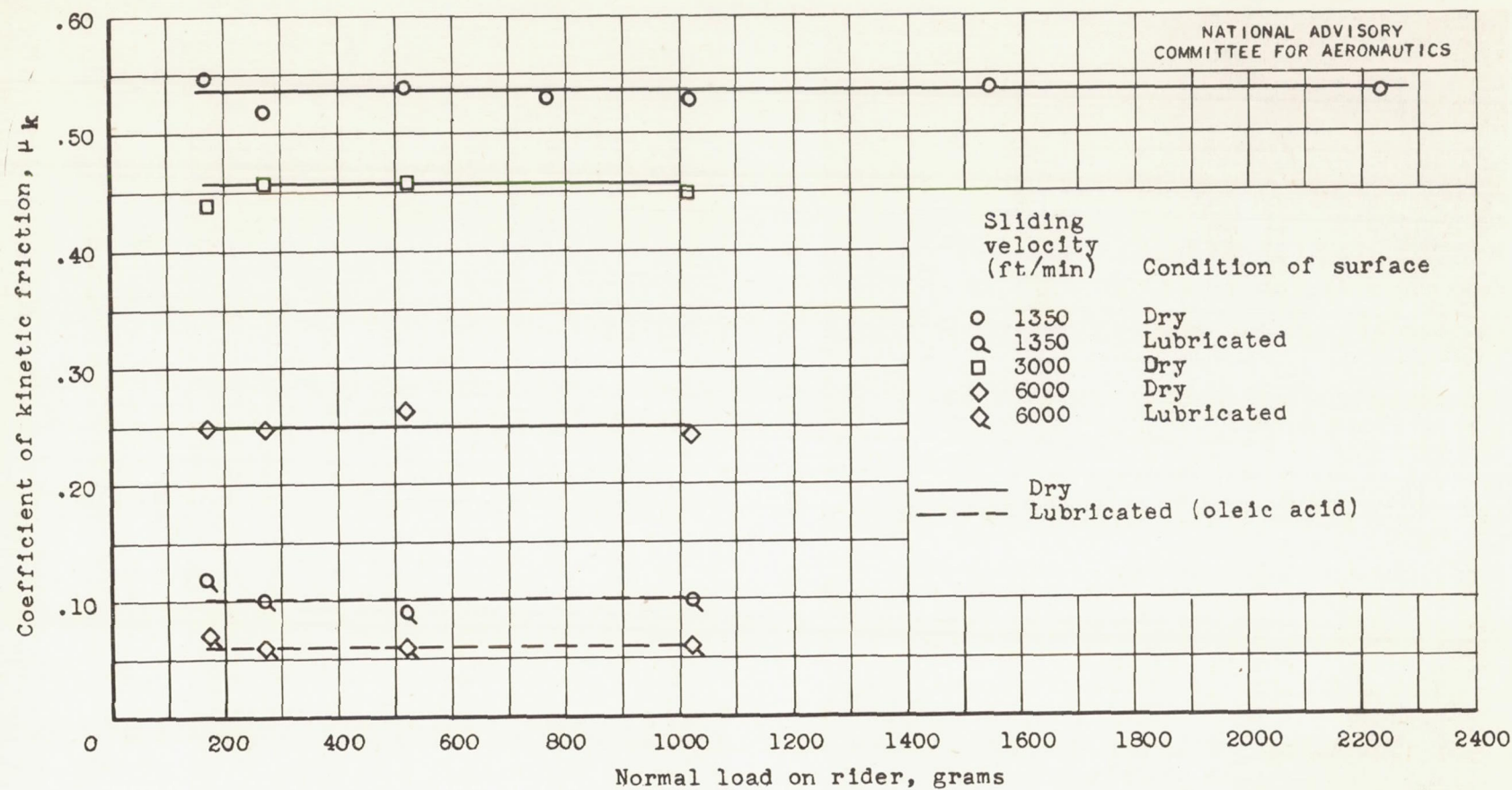
Figure 8. - Effect of load on kinetic friction for dry and boundary-lubricated steel surfaces at various sliding velocities.
