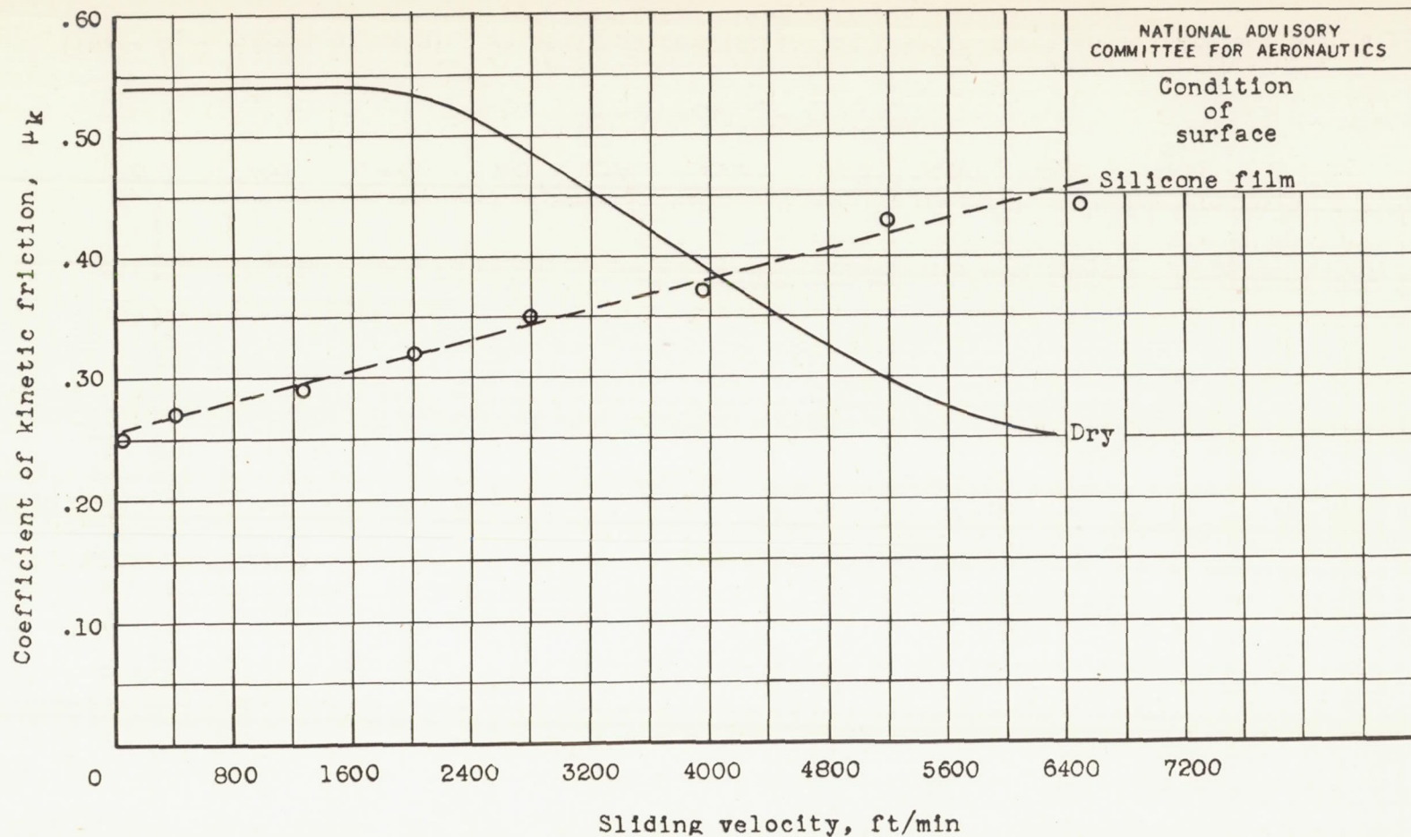
Figure 6. - Comparison of sliding friction of a steel surface having a silicone film with that of a dry steel surface at various velocities. Load, 269 grams. (Curve for dry surface taken from fig. 5.)
