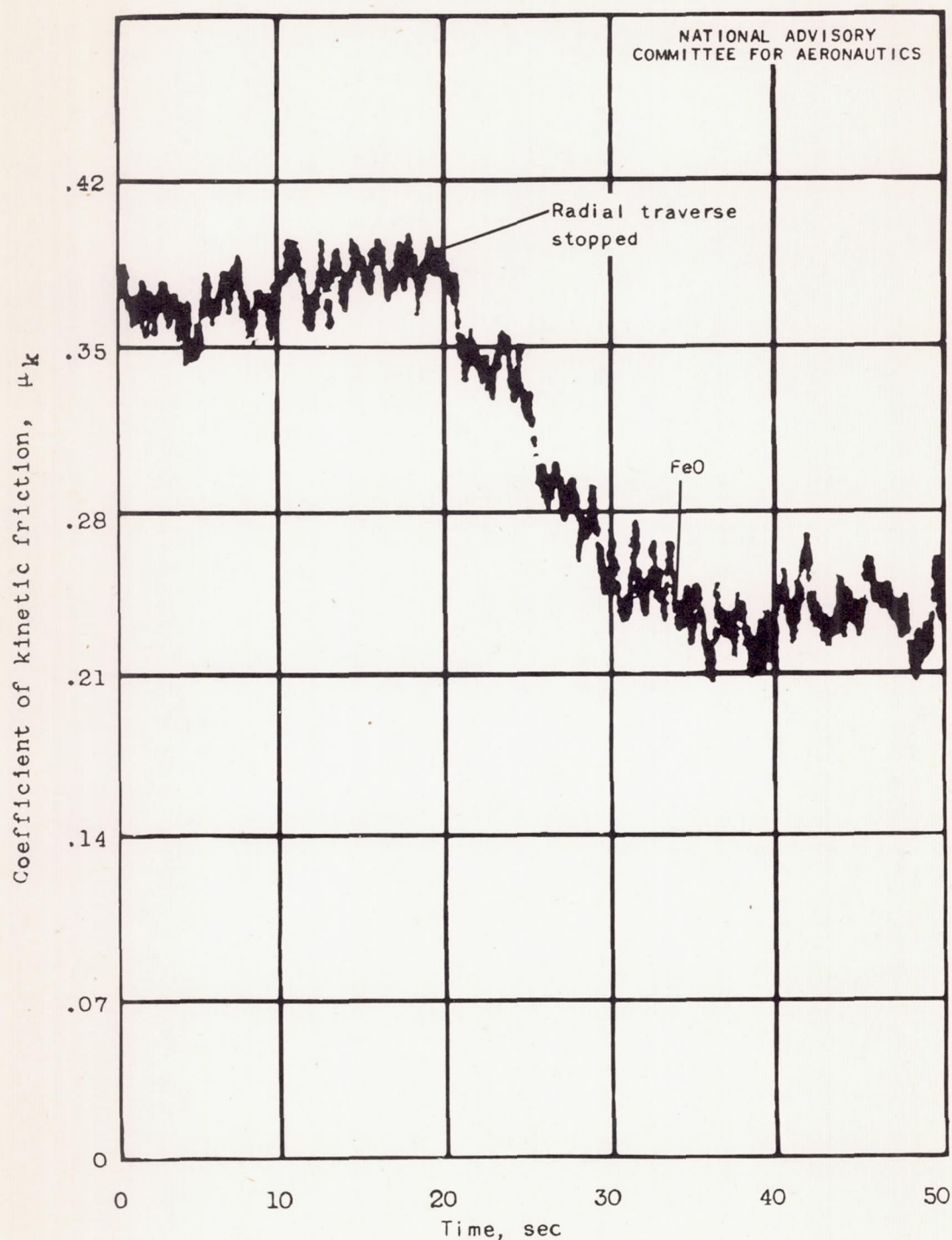
Figure 12. - Recording-potentiometer data showing effect of high-velocity sliding over a continuous path (without radial traverse) on coefficient of kinetic friction. Ferrous oxide (FeO) was visibly present as the decreasing friction trend began to stabilize. Dry steel; load, 269 grams; sliding velocity, 4000 feet per minute.
