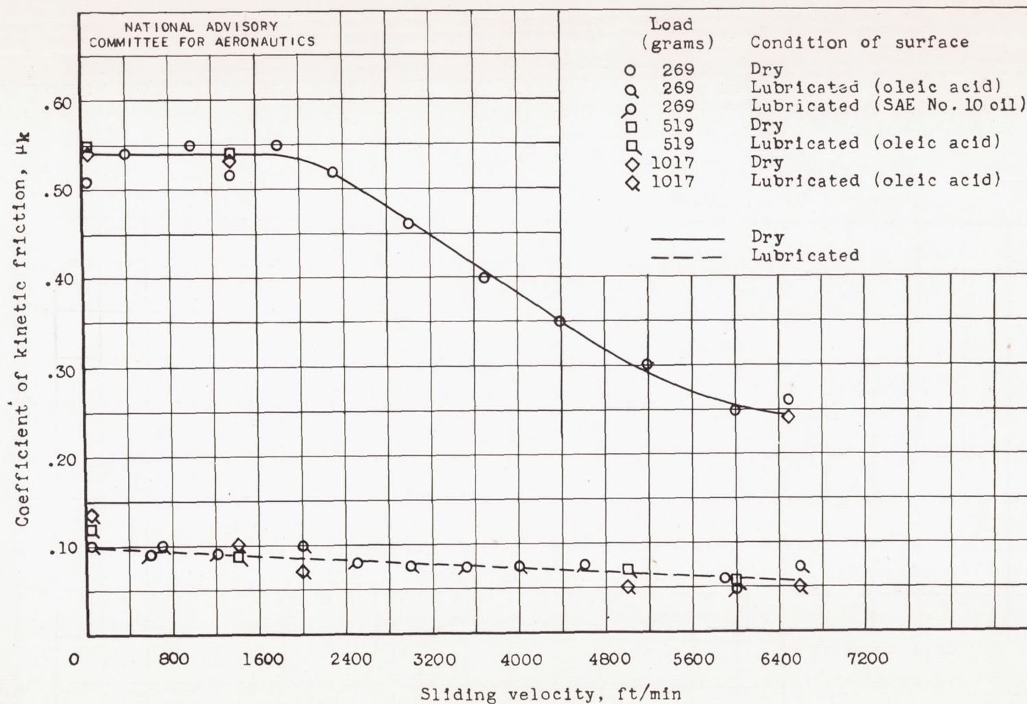
Figure 5. - Effect of sliding velocity on coefficient of kinetic friction for dry and boundary-lubricated steel surfaces.
