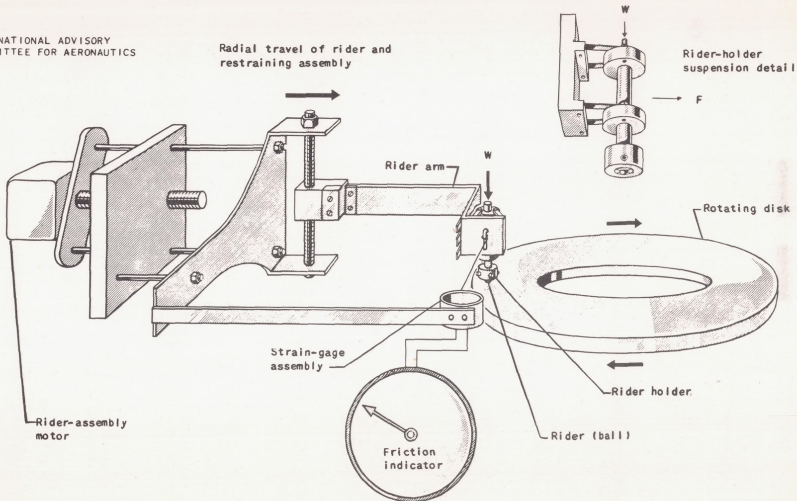
Figure 1. - Schematic diagram of sliding-friction apparatus.
