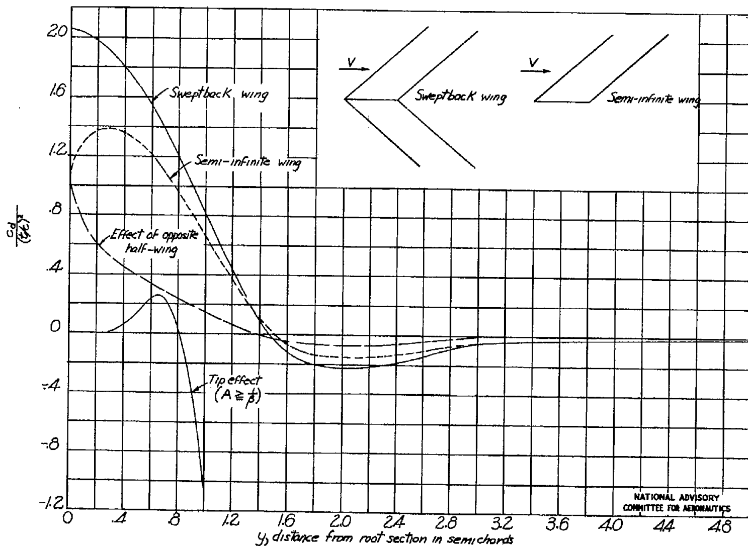
Figure 10.- Section wave-drag distribution for wing of constant chord (taper ratio 1.0). Mach number, 1.414; sweepback angle, 60^\circ .
