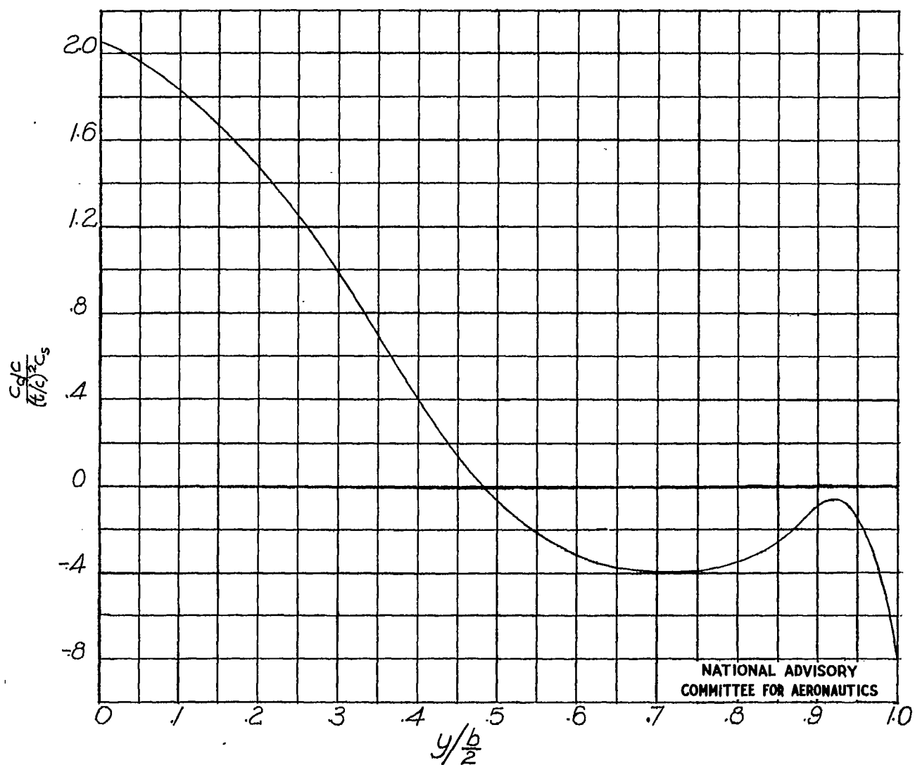
Figure 9.- Section wave-drag distribution for taper ratio 0.5. Mach number, 1.414; aspect ratio, 3.26; sweepback angle, 60^\circ .
