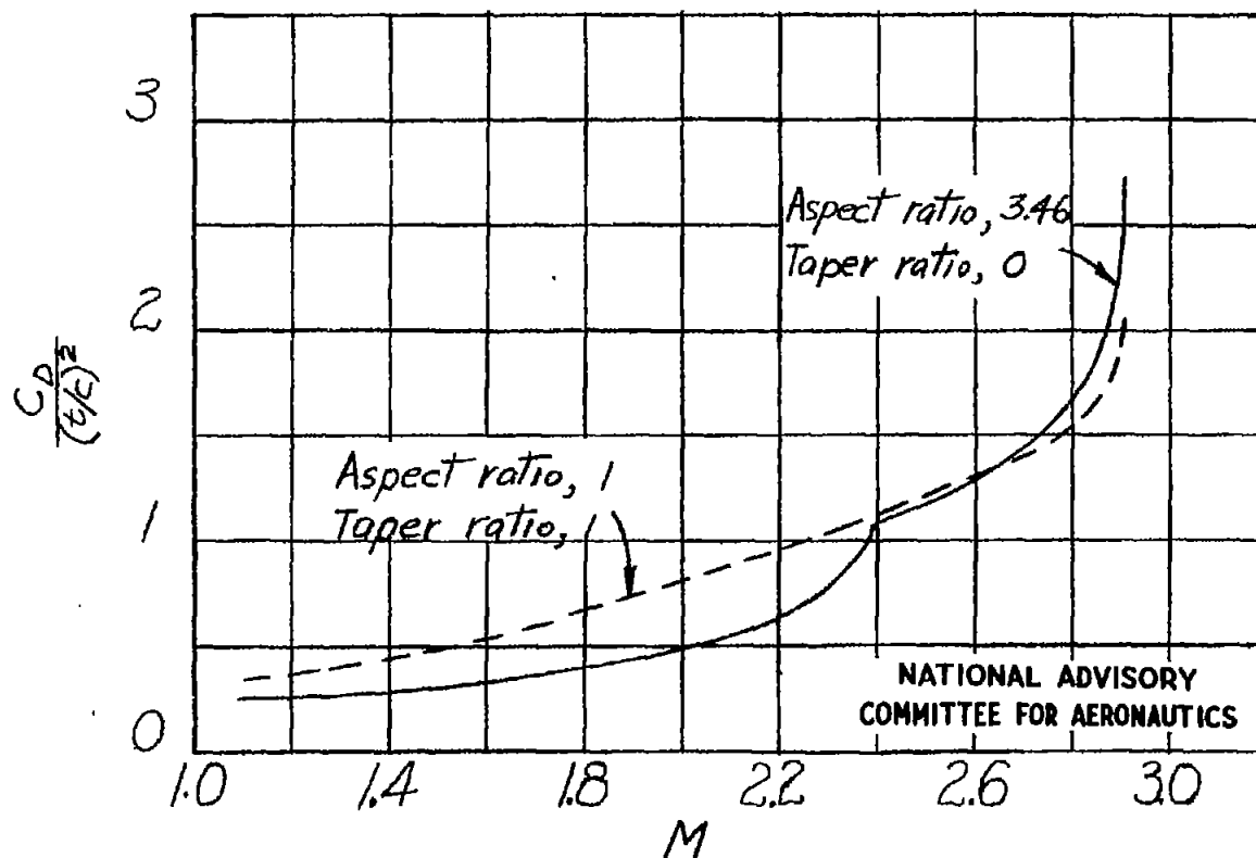
Figure 13.- Variation of wing wave-drag coefficient with Mach number. Sweepback angle, 70^\circ .
