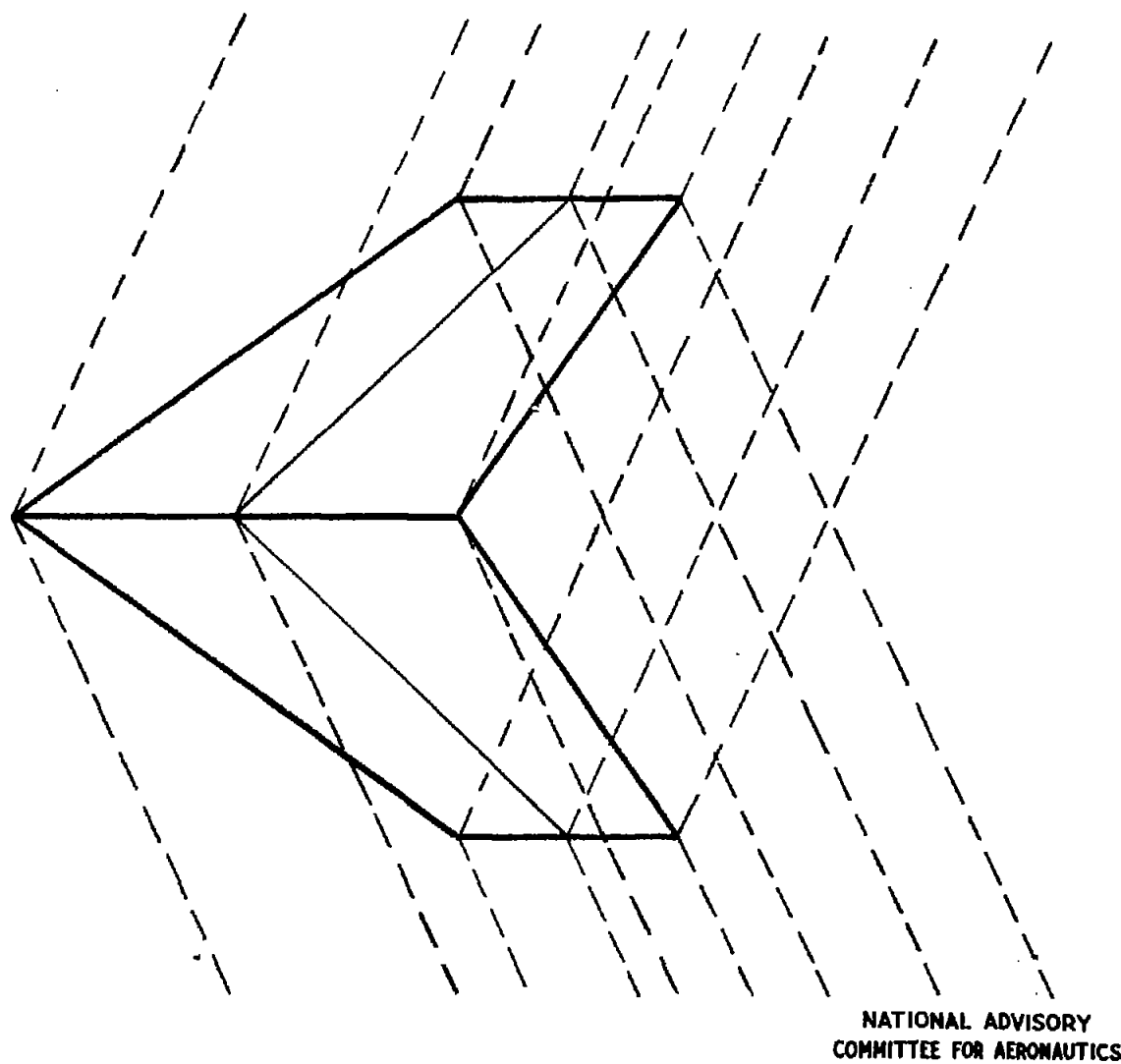
Figure 2.- Mach line configuration for a tapered plan form.
