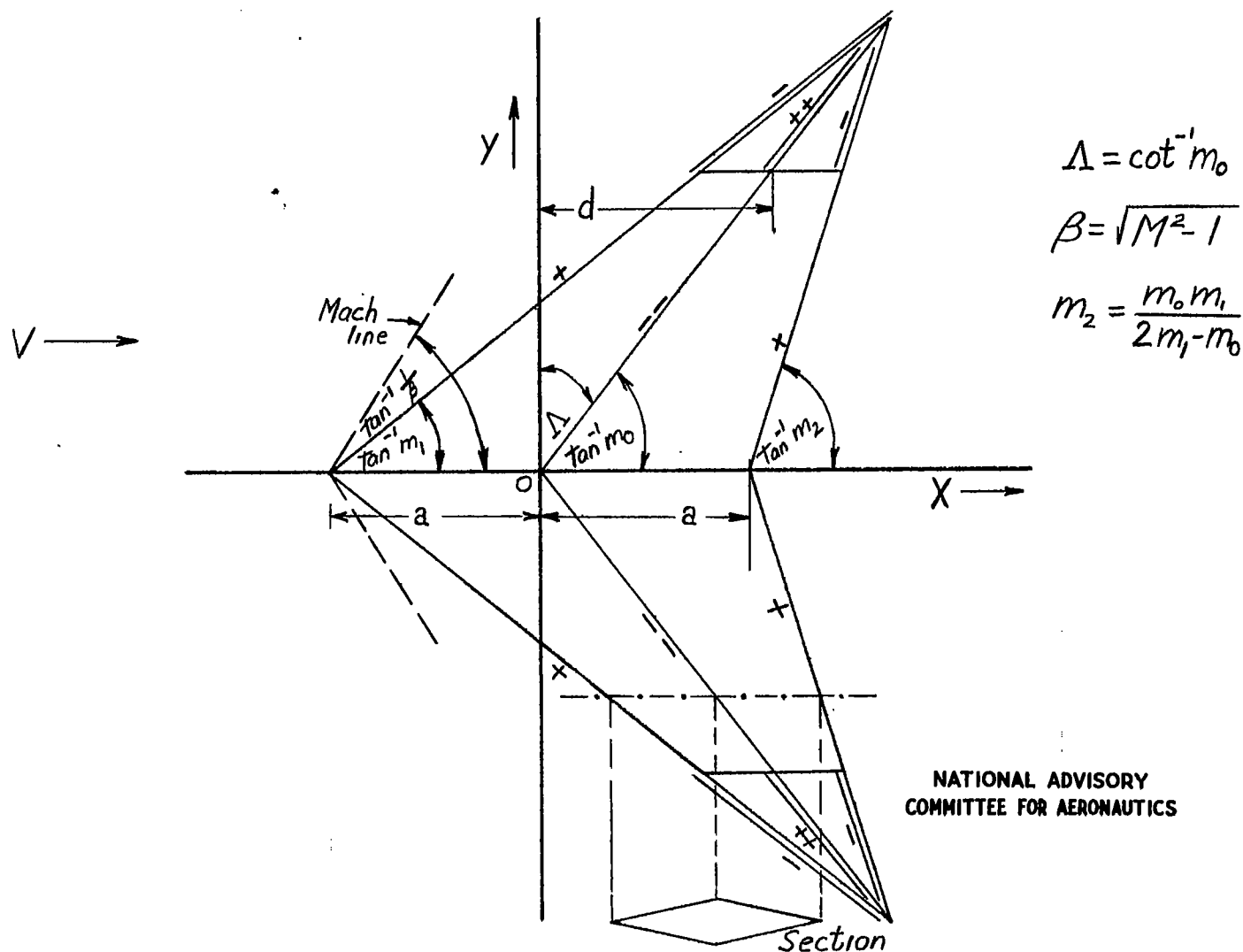
Figure 1.- Symbols and distributions of sinks and sources for a tapered wing.
