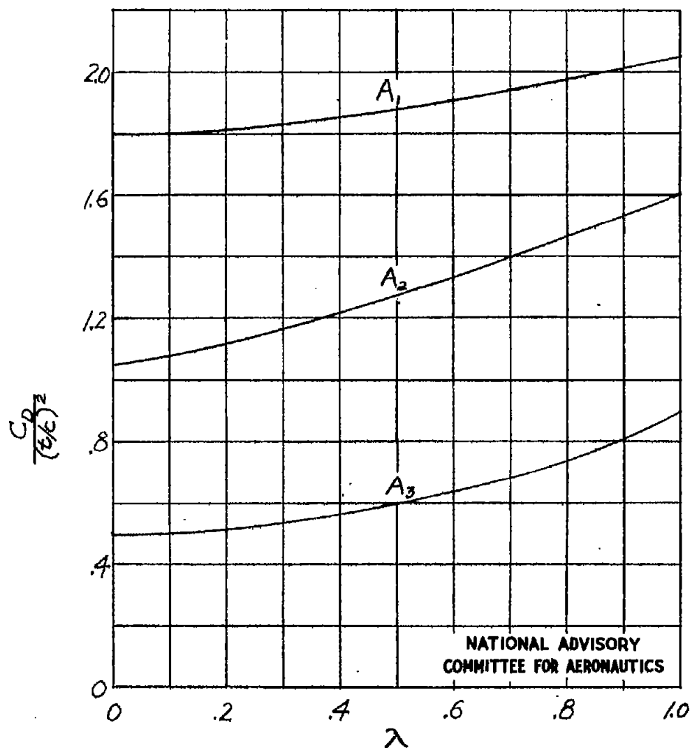
Figure 15.- Variation of wing wave-drag coefficient with taper ratio for three families of wing plan forms. Mach number, 1.414; sweepback angle, 60^\circ .
