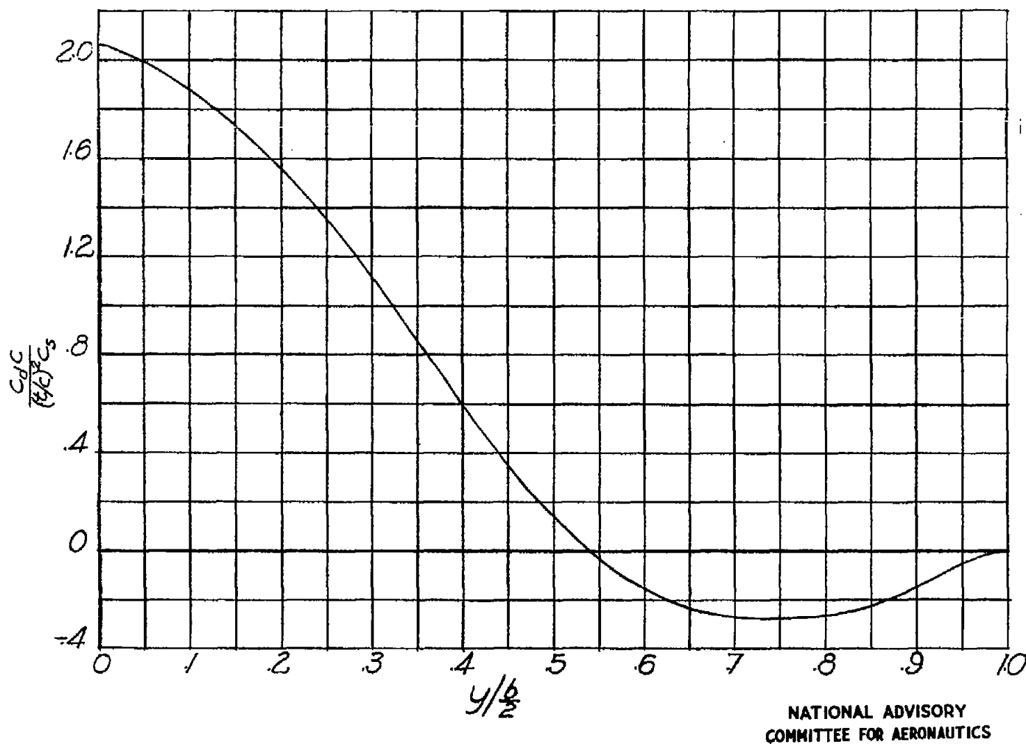
Figure 6.- Section wave-drag distribution for wing of taper ratio 0. Mach number, 1.414; aspect ratio, 3.46; sweepback angle, 60^\circ .
