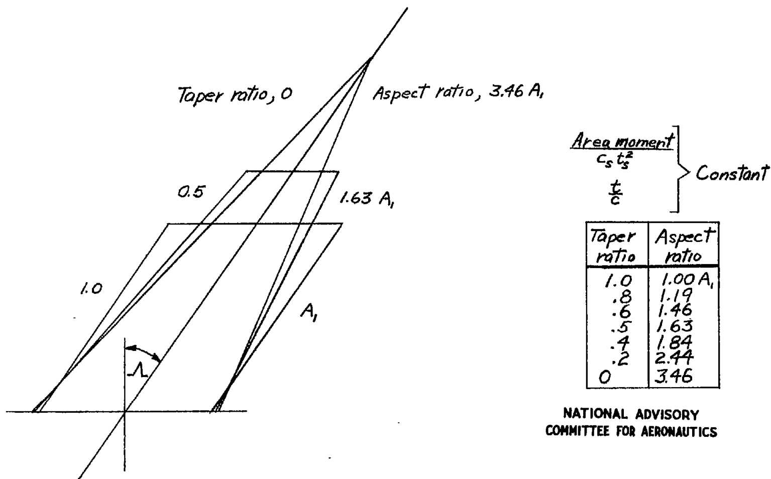
Figure 5.- Family of tapered plan forms used for calculations. Plan forms shown have same area.
