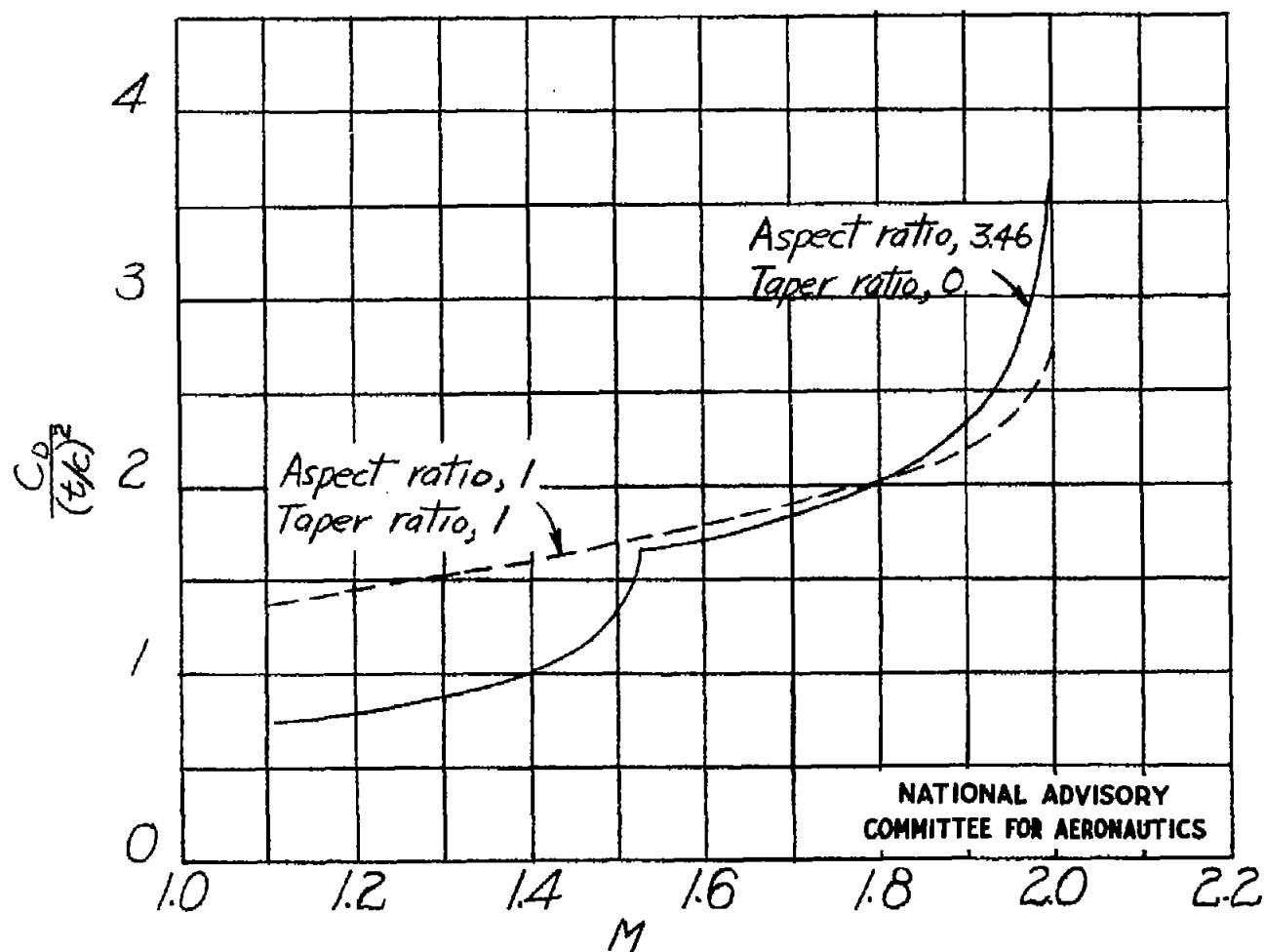
Figure 12.- Variation of wing wave-drag coefficient with Mach number. Sweepback angle, 60^\circ .
