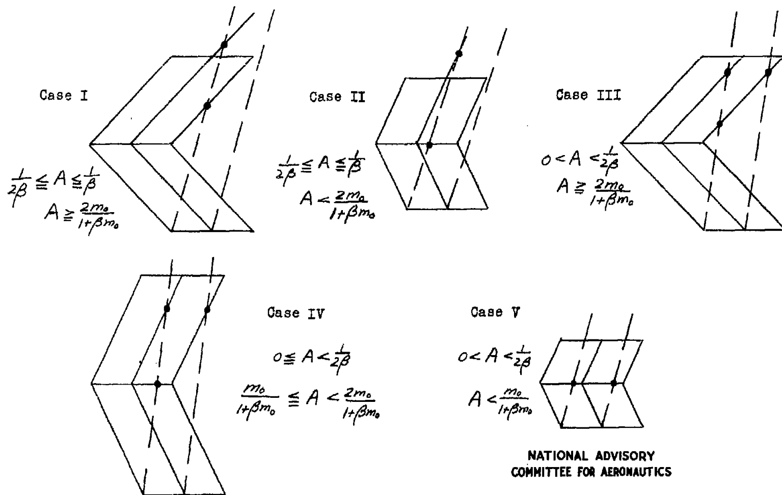
Figure 4.- Additional tip effects for wing of constant chord (taper ratio 1.0).
