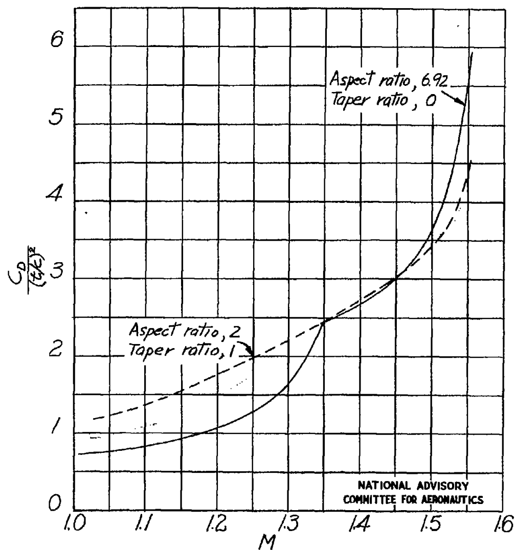
Figure 11.- Variation of wing wave-drag coefficient with Mach number. Sweepback angle, 50^\circ .
