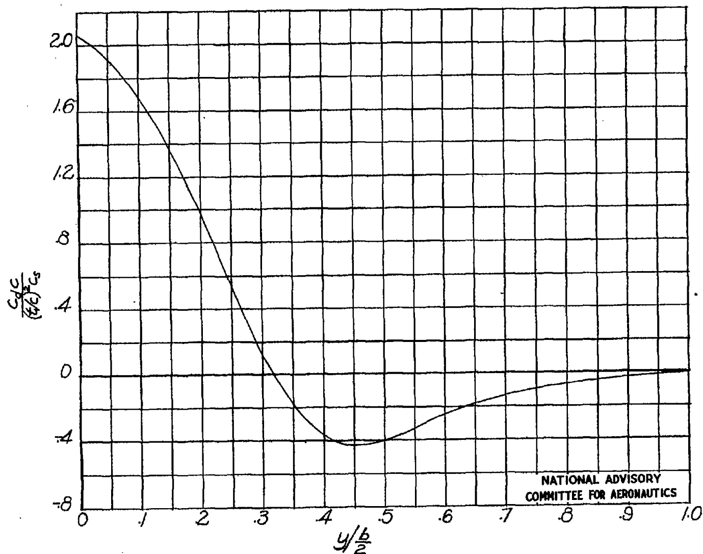
Figure 7.- Section wave-drag distribution for wing of taper ratio 0. Mach number, 1.414; aspect ratio, 6.92; sweepback angle, 60^\circ .
