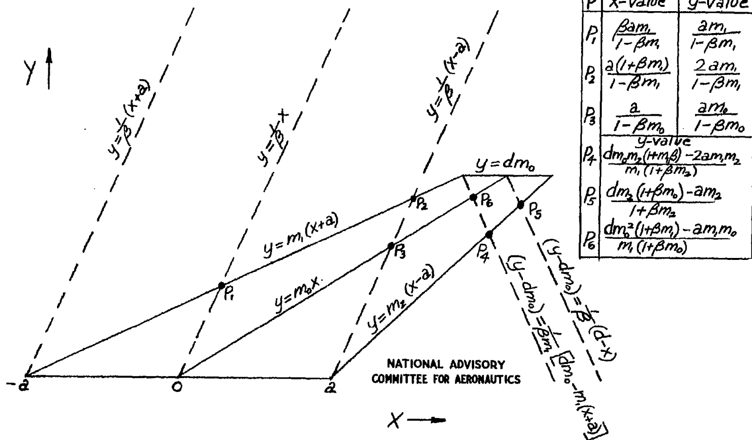
Figure 3.- Information pertinent to integration limits in equations (5) and (7).
