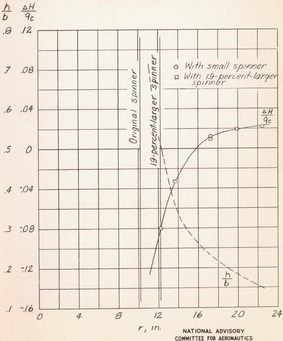
Figure 7.- Comparison between total-pressure loss due to shanks for original and 19-percent-larger spinner. M = 0.67 ; C_p per blade = 0.13; J = 2.83 .
