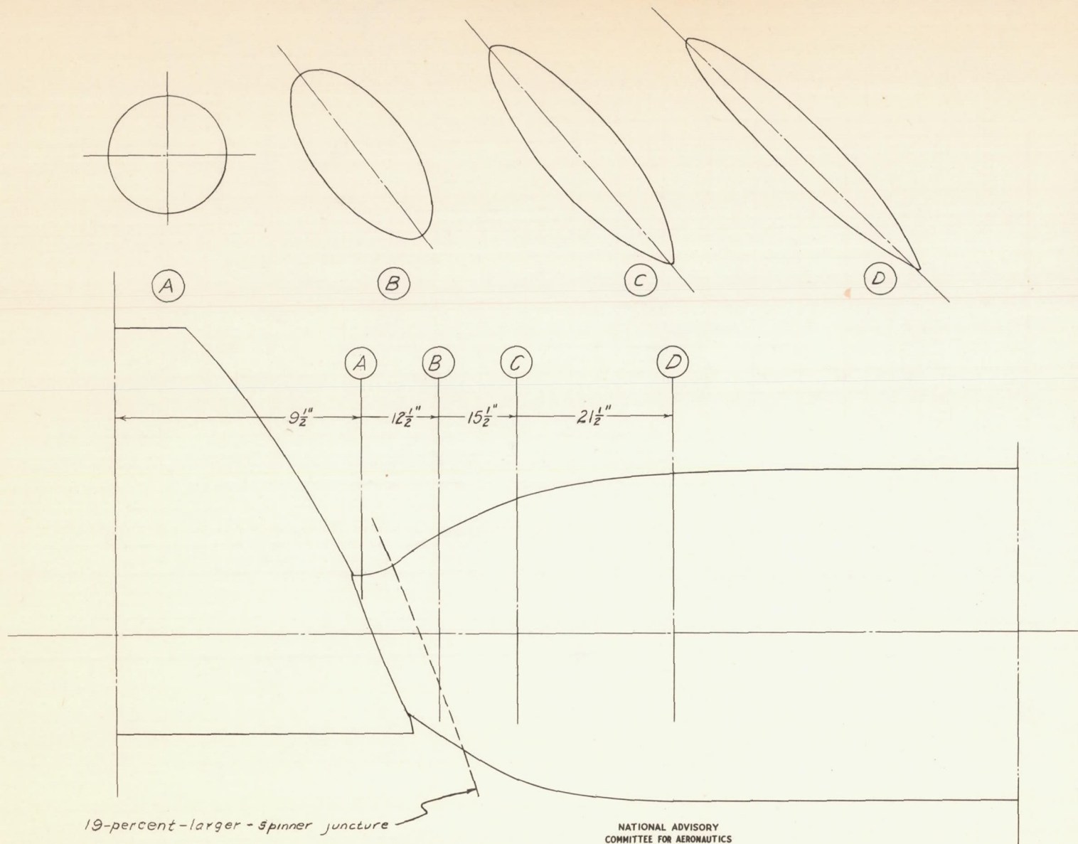
Figure 3.- Details of shank sections and spinner juncture.
