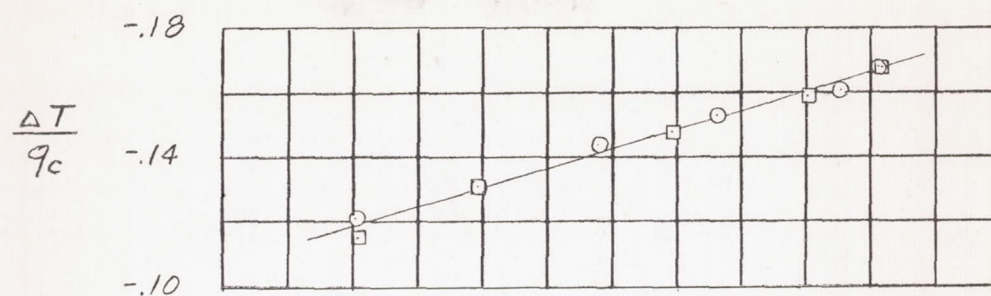
(a) Shank losses in terms of \frac{\Delta T}{q_c} .
