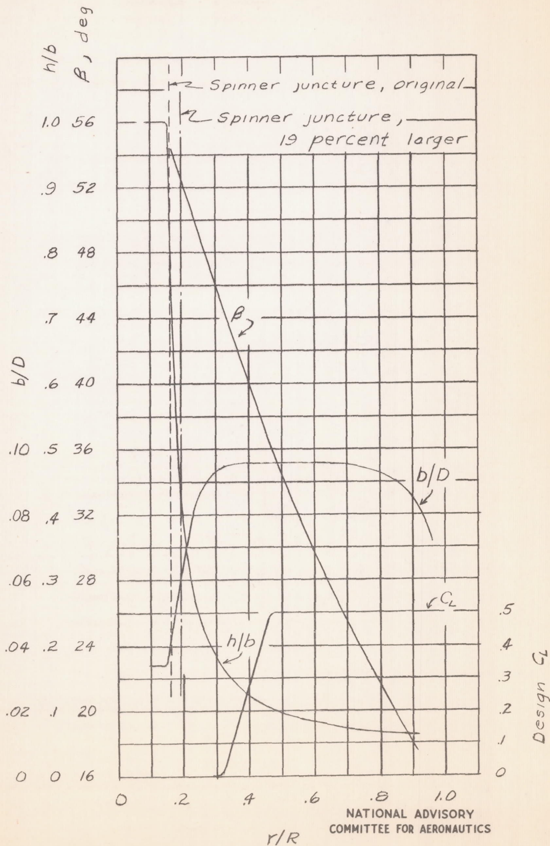
Figure 2.- Blade-form curves for propeller tested.
