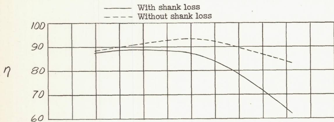
(a) C_P per blade = 0.07 at 1120 rpm.
