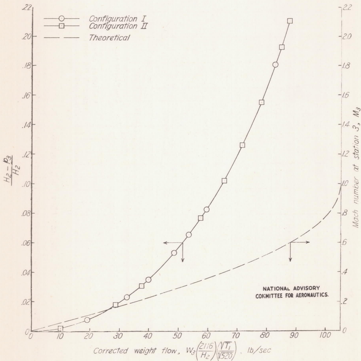
Figure 7.- Calibration curve for approach section and curve of theoretical relation of Mach number to weight flow.
