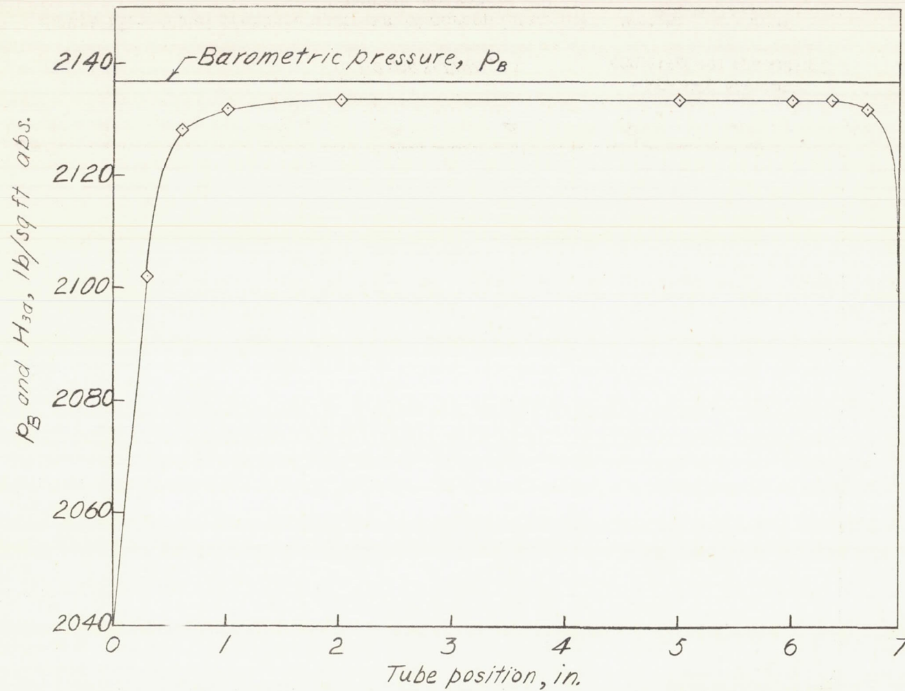
Figure 12.- Total pressure upstream of screen (station 3). Weight flow, 82.15 pounds per second.
