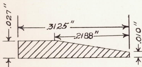
(b) Typical vane cross section of configuration I.
