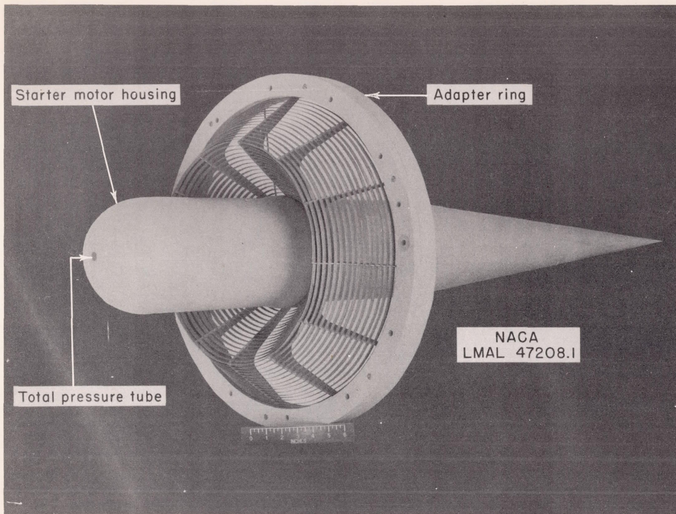
Figure 1.- Turbojet inlet screen and starter-motor housing.
