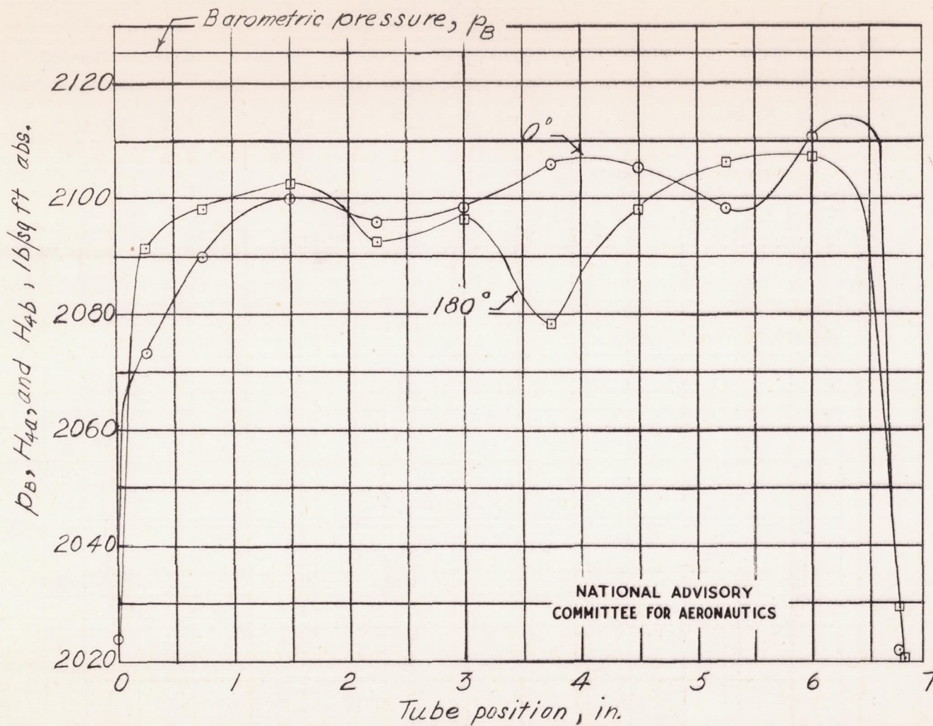
(c) Circumferential position, 0^\circ and 180^\circ ; weight flow, 59.35 pounds per second.
