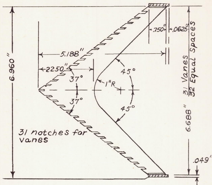
(a) View of screen showing strut detail and vane location.
