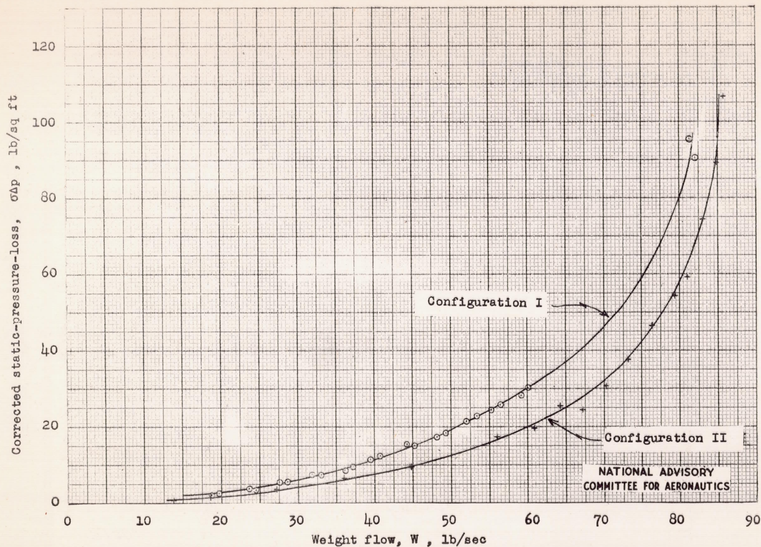
Figure 9.- Corrected static-pressure-loss plotted against weight flow.
