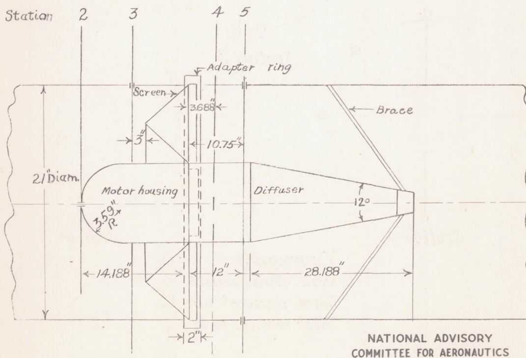
(b) Detail location of measuring stations.
