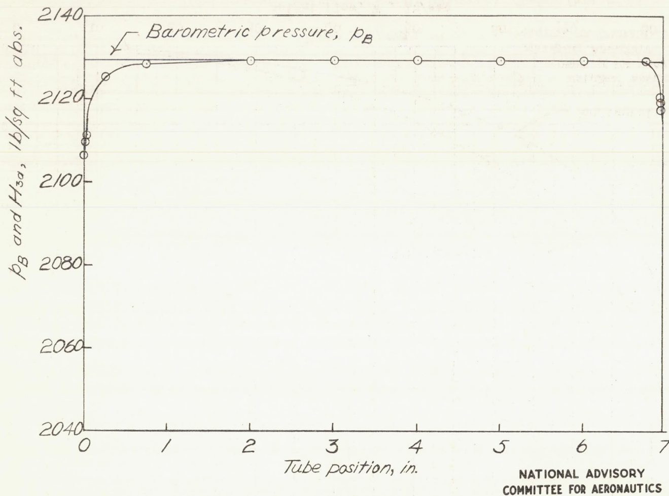
Figure 10.- Total pressure upstream of screen (station 3). Weight flow, 28.24 pounds per second.
