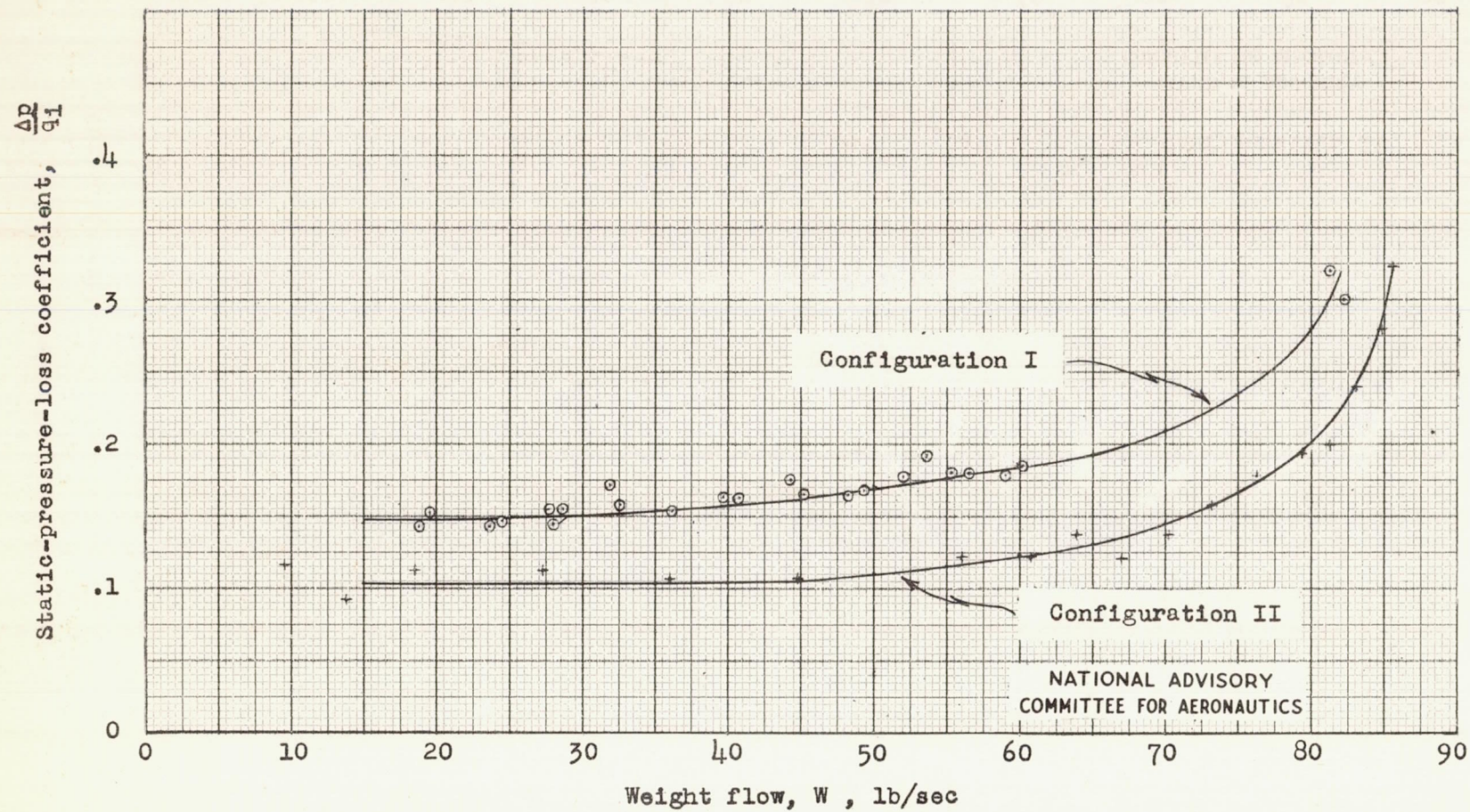
Figure 8.- Static-pressure-loss coefficient plotted against weight flow.
