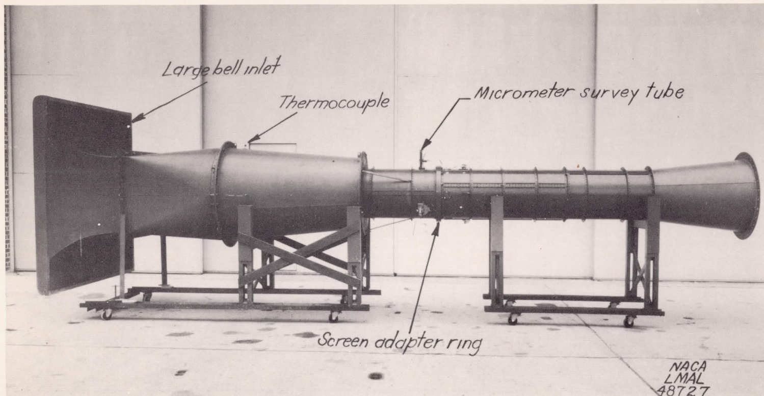
Figure 3.- General view of ducting and apparatus.
