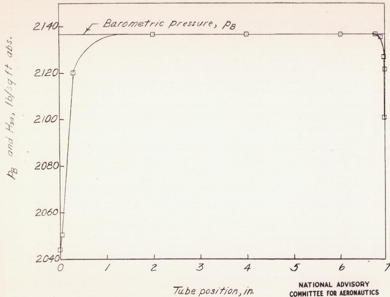
Figure 11.- Total pressure upstream of screen (station 3). Weight flow, 56.81 pounds per second.
