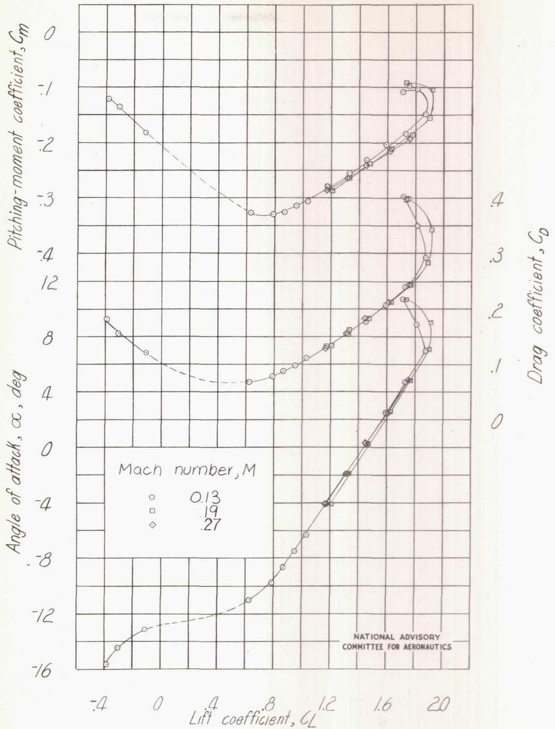
Figure 7.- Variation of aerodynamic characteristics with Mach number of wing with full-span slotted flap deflected 45°. Flap nose in normal location.
