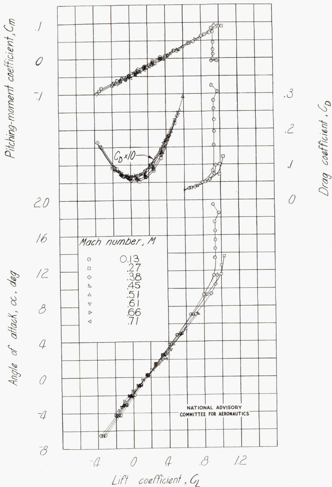
Figure 6.- Variation of plain-wing aerodynamic characteristics with Mach number.
