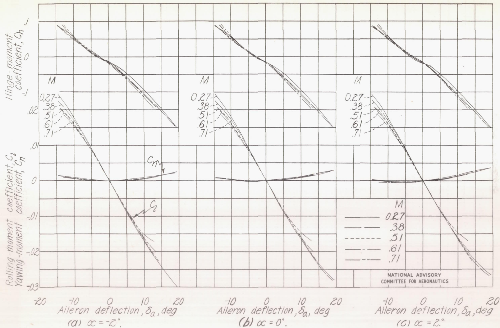
Figure 12.- Variation of lateral-control characteristics of complete wing with aileron deflection and Mach number. \delta_f = 0^\circ .
