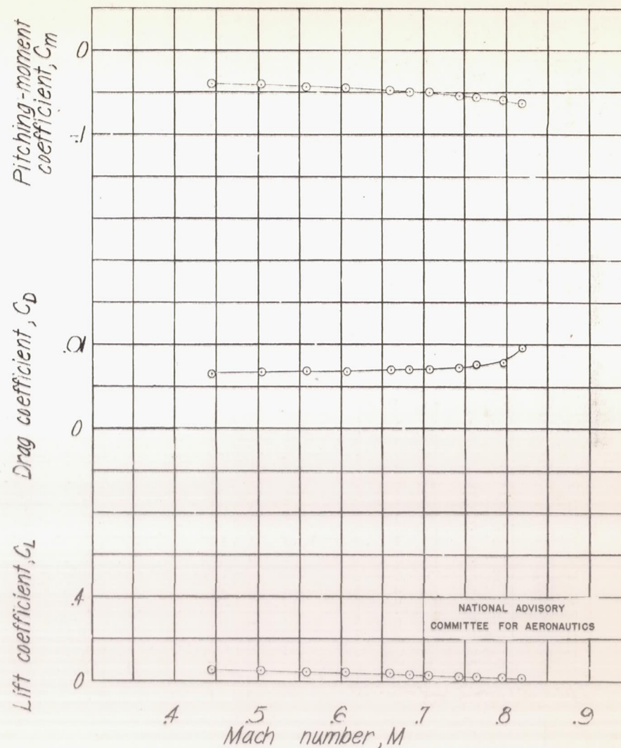
Figure 10.- Variation with Mach number of plain-wing characteristics. \alpha = -1.45^\circ .
