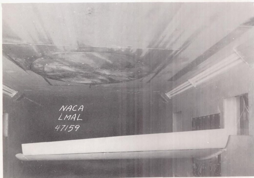
Figure 1.- Reflection-plane model in inverted position with full-span flap deflected.
