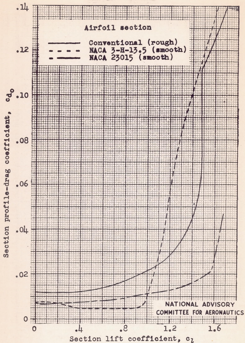
Figure 19.- Airfoil section profile-drag coefficient c_{d_0} against section lift coefficient c_l for the airfoil sections of figure 1 from reference 3.
