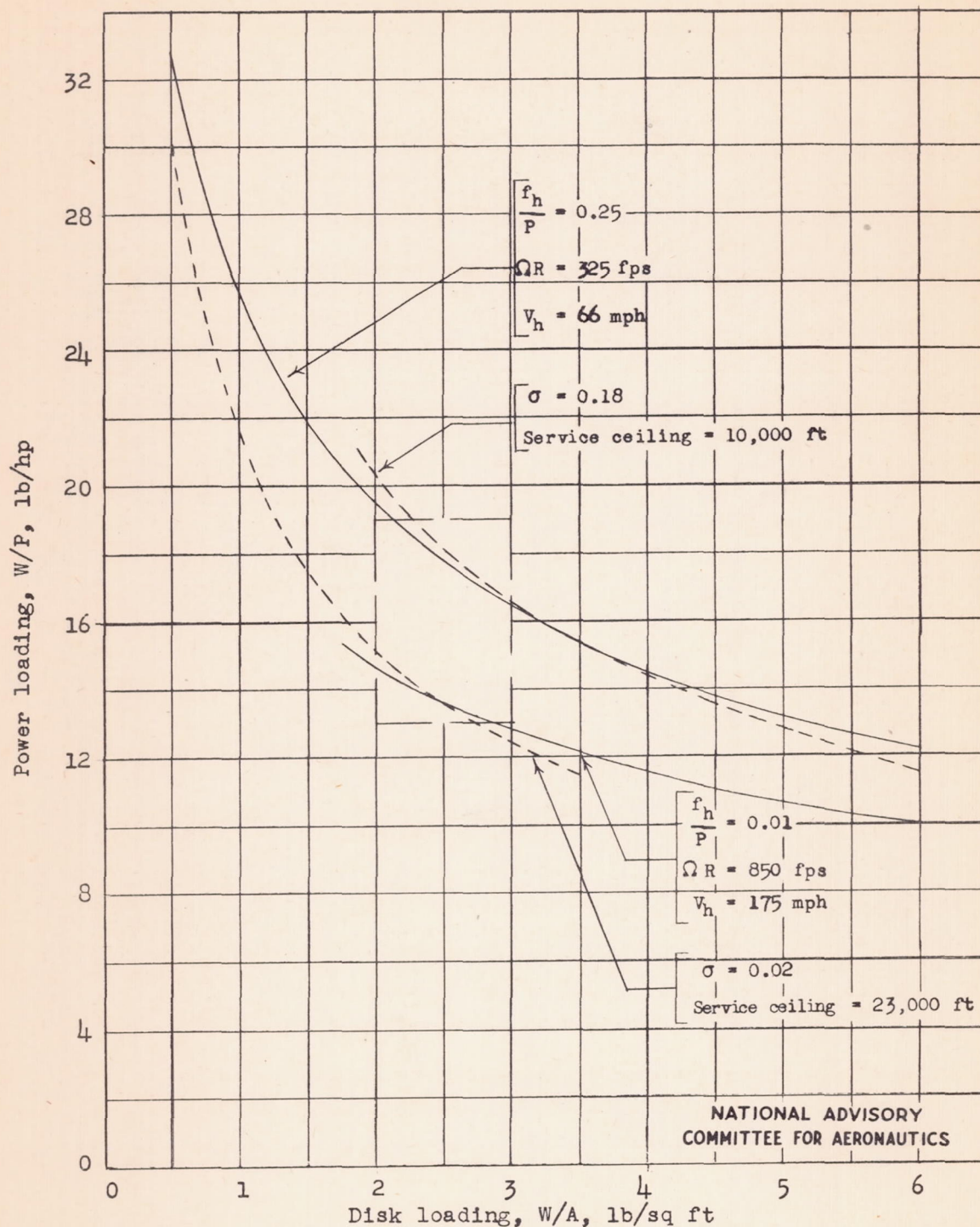
Figure 17.- Power-loading disk-loading performance chart for sea level for helicopters with power just sufficient to hover.
