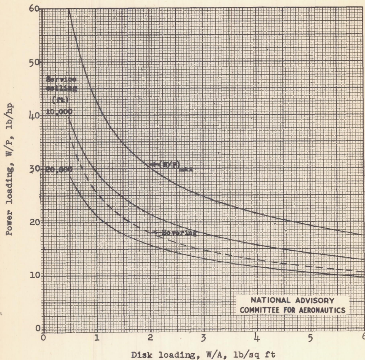
Figure 3.- Service ceiling for the conditions of figure 1.
