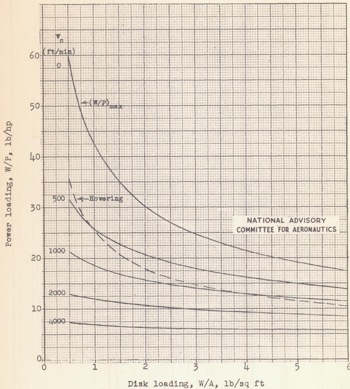
Figure 2.- Maximum rate of climb for the conditions of figure 1.
