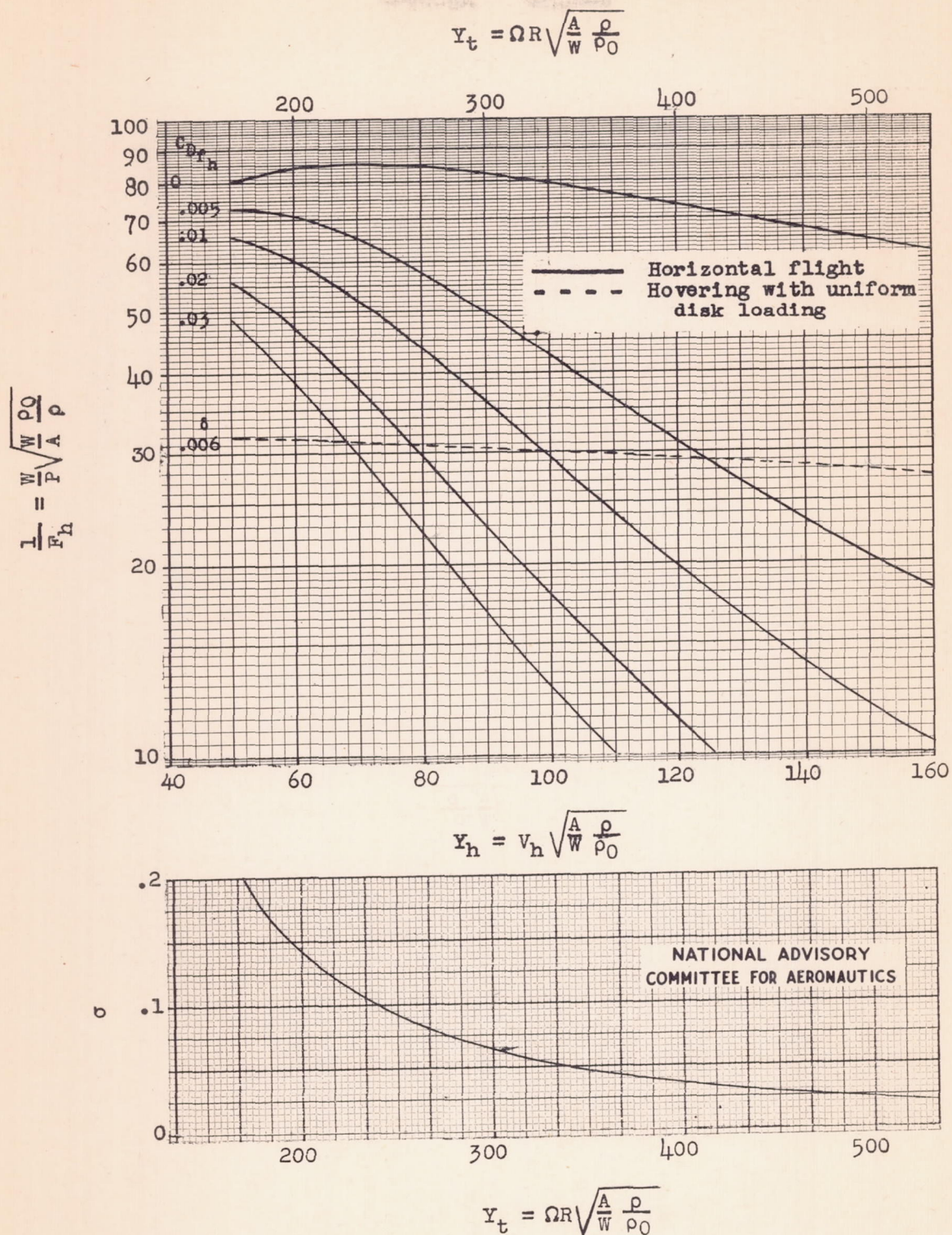
Figure 5.- Generalized performance chart for horizontal flight and hovering. \mu = 0.3 ; \delta = 0.006 ; \sigma Y_t^2 = 5740 .
