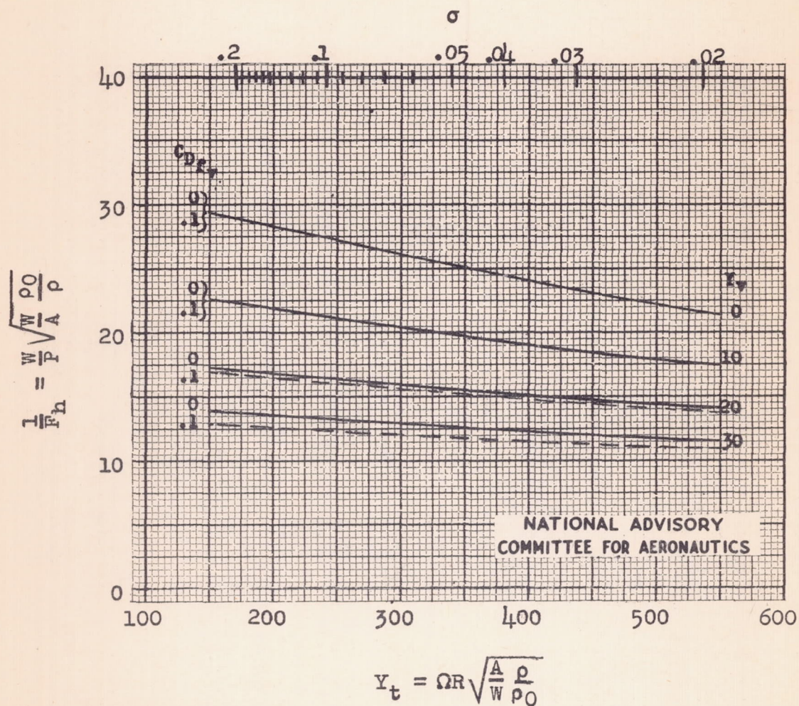
Figure 9.- Generalized performance chart for constant values of the rate-of-vertical-climb parameter Y_v at sea level. \delta = 0.012 ; \sigma Y_t^2 = 5740 .
