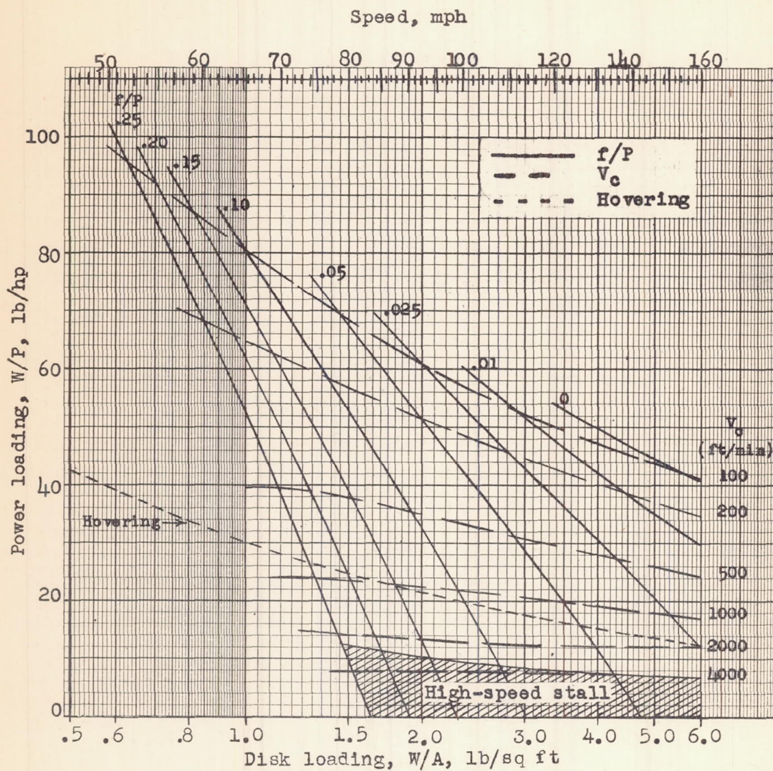
Figure 12.- Power-loading disk-loading performance chart for sea level. \mu = 0.3 ; \delta = 0.006 ; \sigma = 0.056 ; \sigma Y_t^2 = 5740 .
