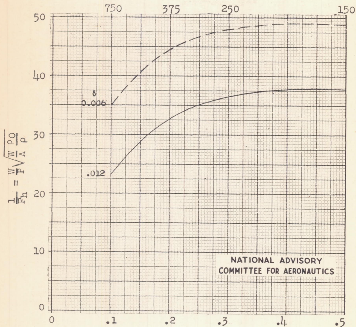
Figure 6.- Variation of \frac{1}{F_h} with \mu . \sigma Y_t^2 = 5740 ; Y_h = 75 ; C_{D_{f_h}} = 0.01 .
