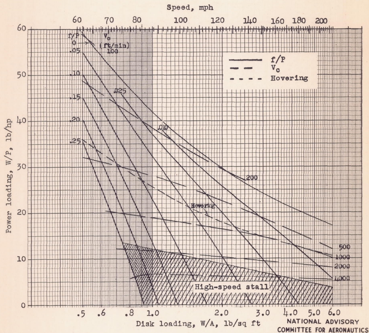
Figure 15.- Power-loading disk-loading performance chart for sea level.
