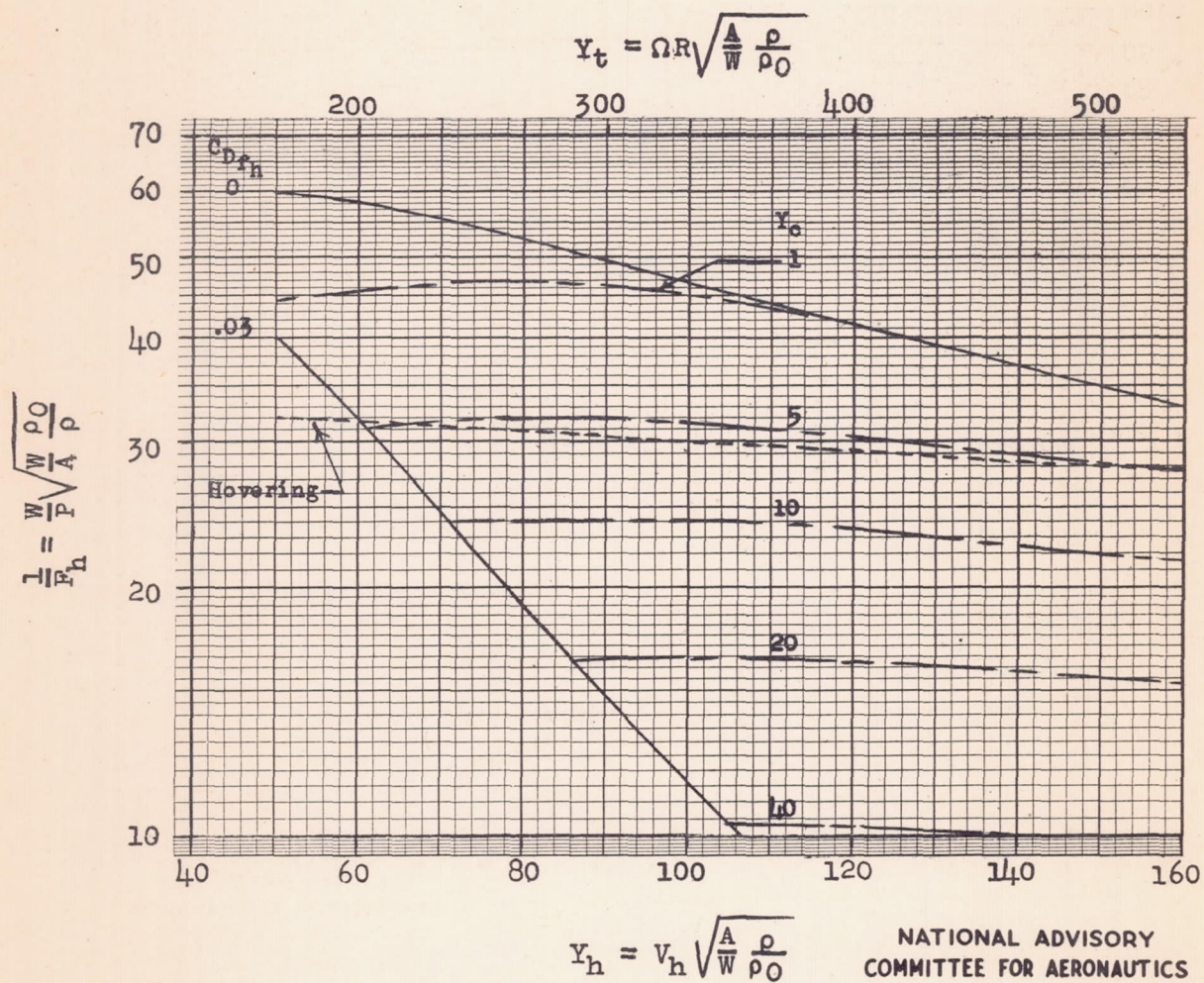
Figure 7.- Generalized performance chart for maximum rate of climb for the conditions of figure 4. \delta = 0.012 . ( V_h is the maximum speed, i.e. for Y_c = 0 .)
