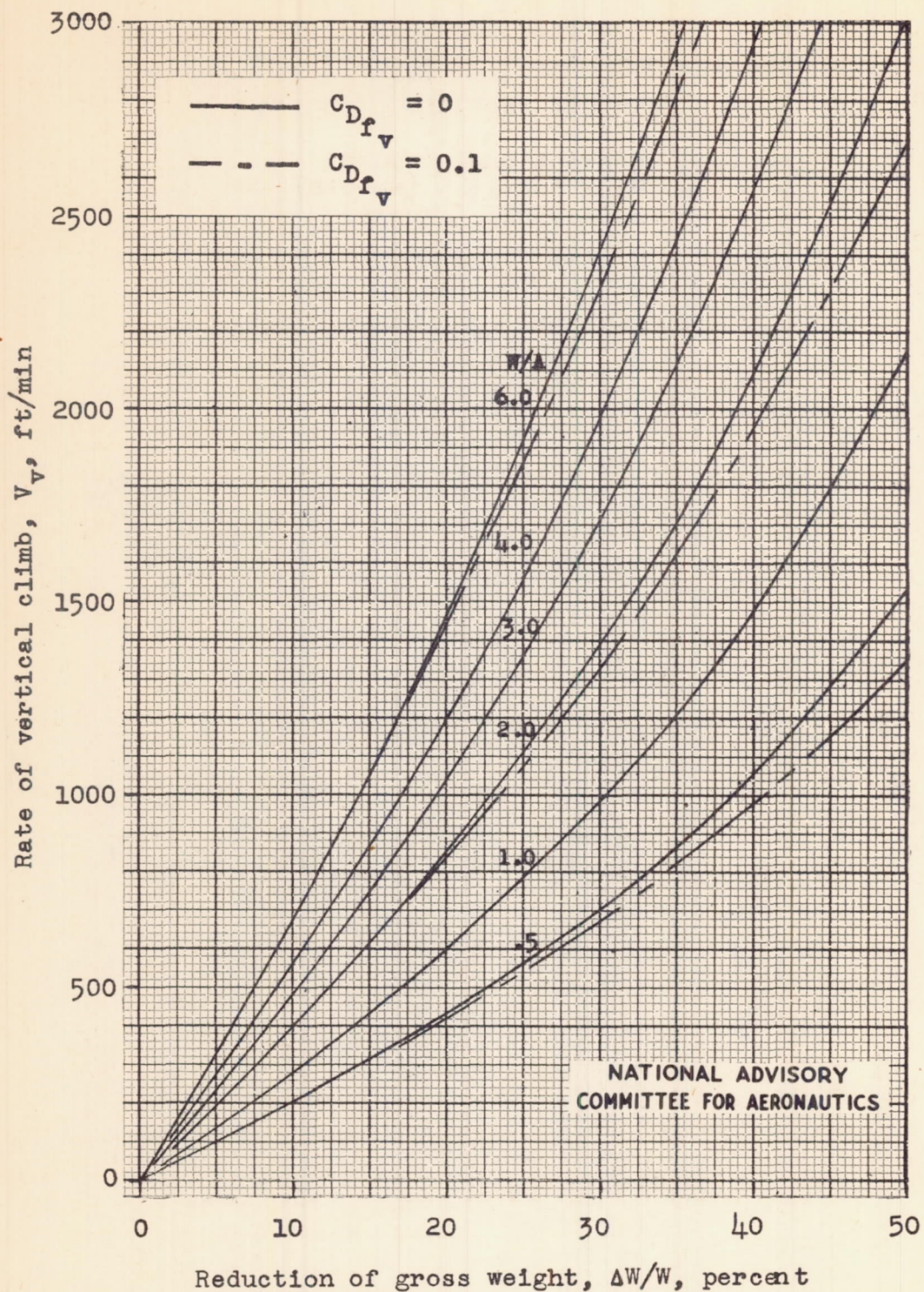
Figure 20.- Rate of vertical climb obtainable by reduction in gross weight of helicopters with power just sufficient to hover.
