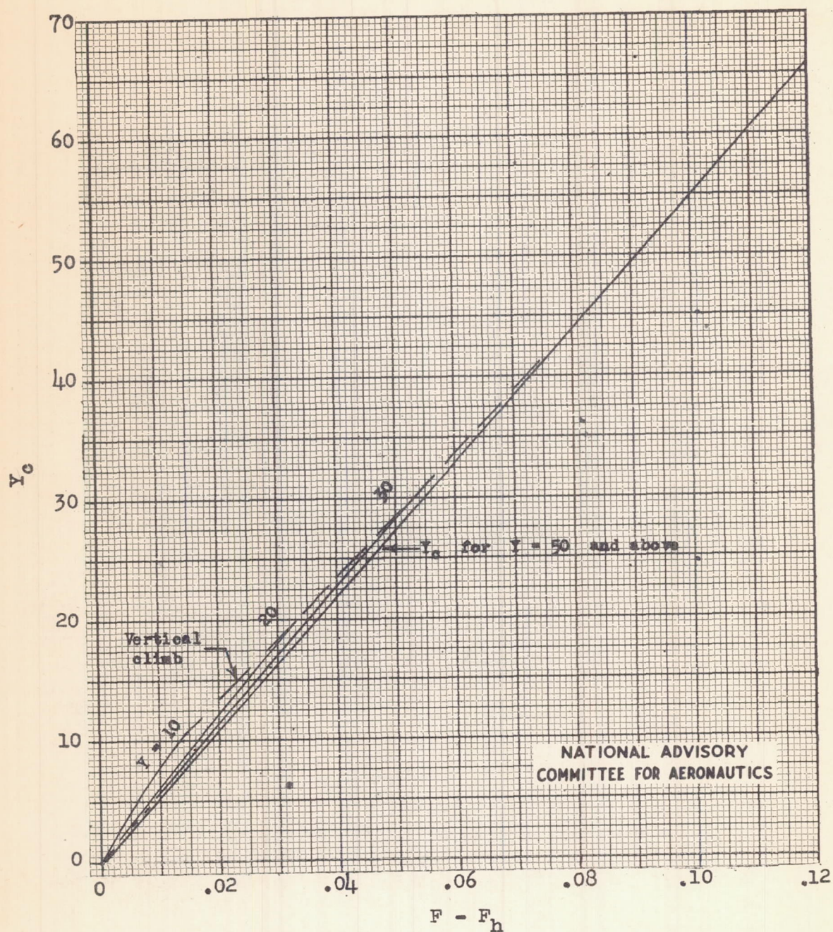
Figure 10.- Chart for finding the rate-of-forward-climb parameter Y_c .
