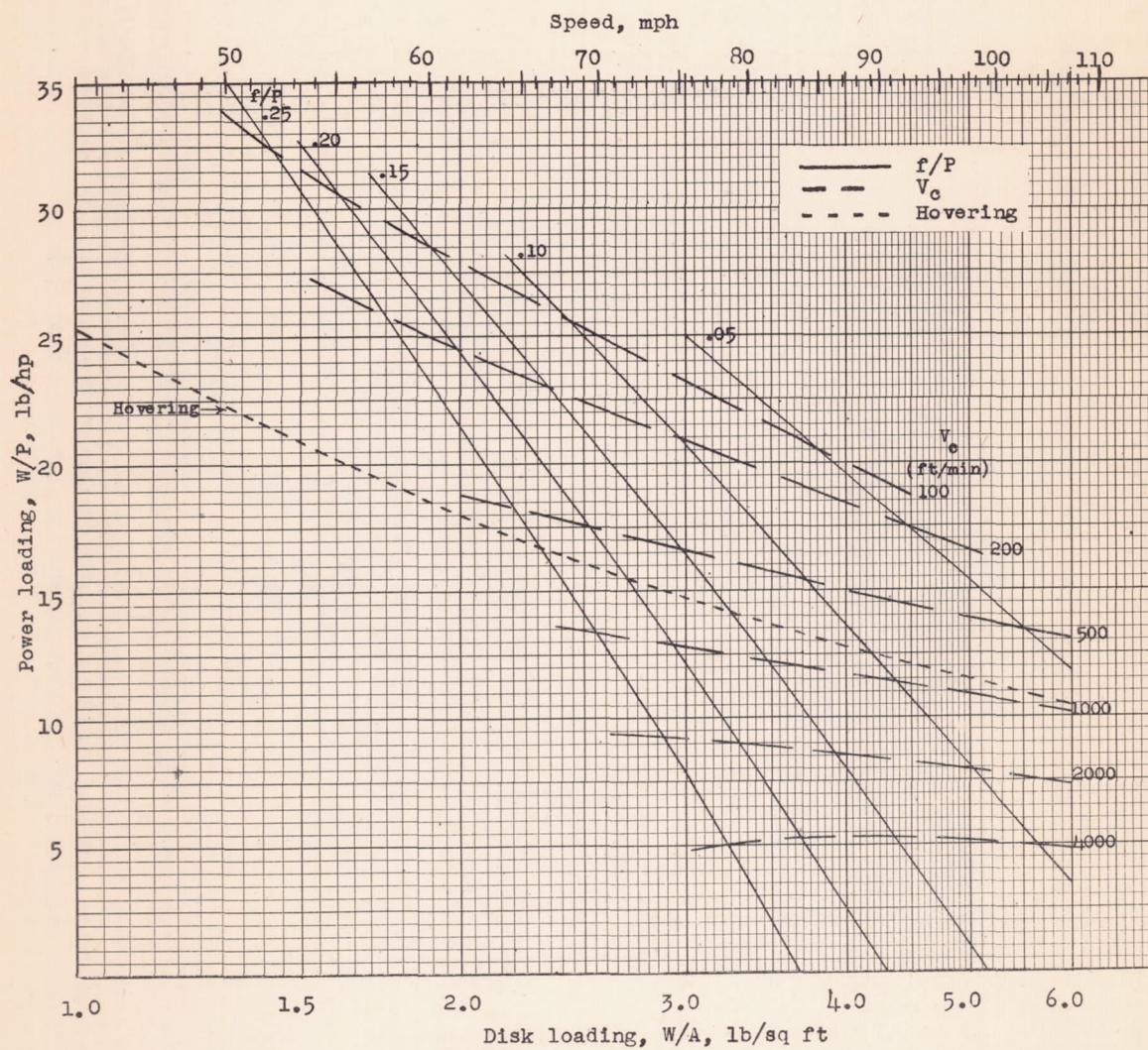
Figure 13.- Power-loading disk-loading performance chart for sea level. \mu = 0.2 ; \delta = 0.012 ; \sigma = 0.056 ; \sigma Y_t^2 = 5740 .
