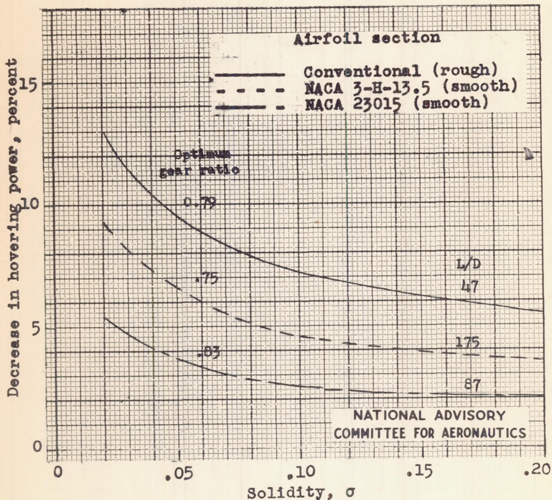
Figure 22.- Decrease in the power required for hovering by use of a rotor-speed-reduction gear.
