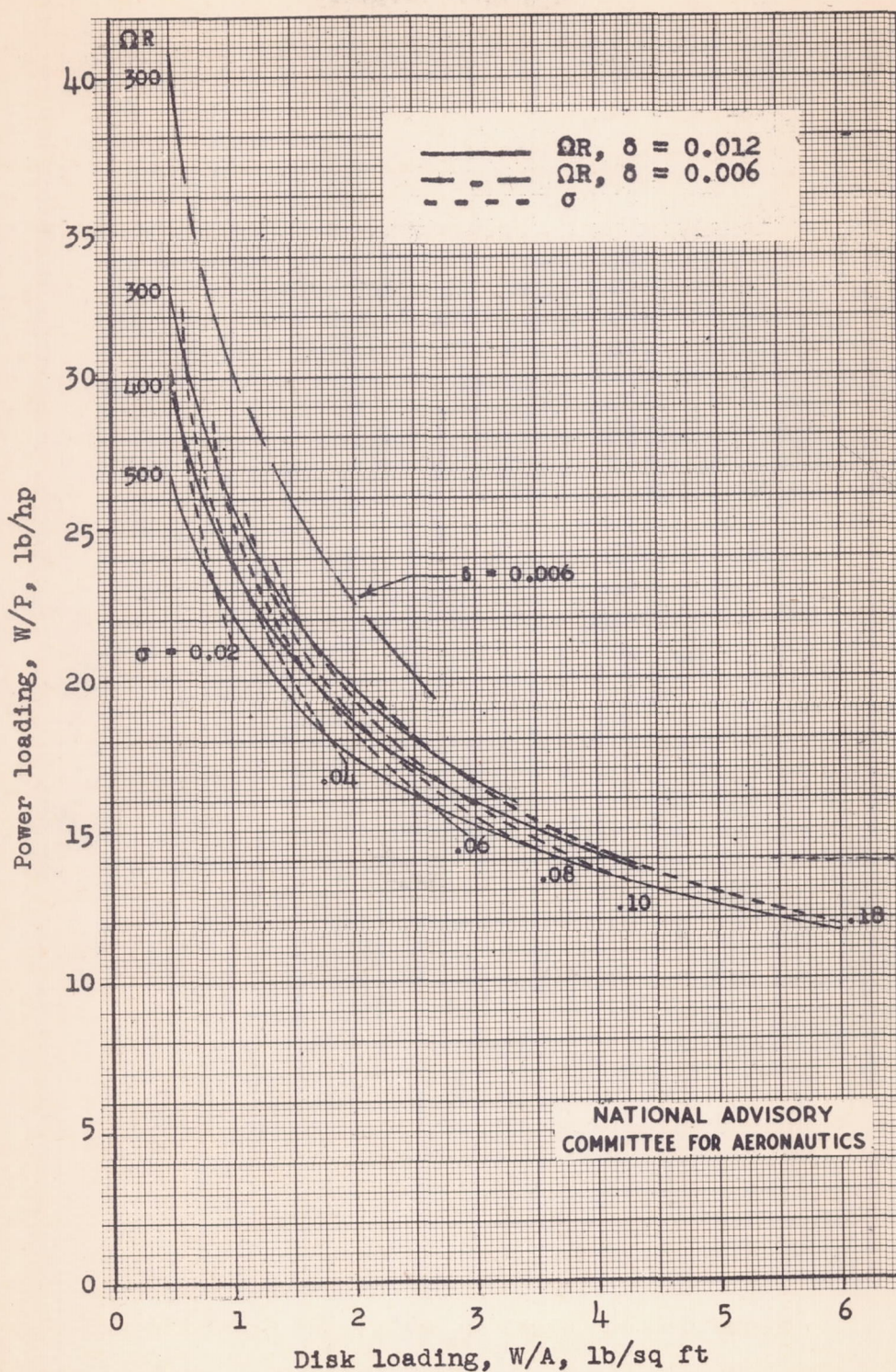
Figure 21.- Power-loading disk-loading performance chart for hovering helicopters at sea level with \sigma Y_t^2 = 5740 .
