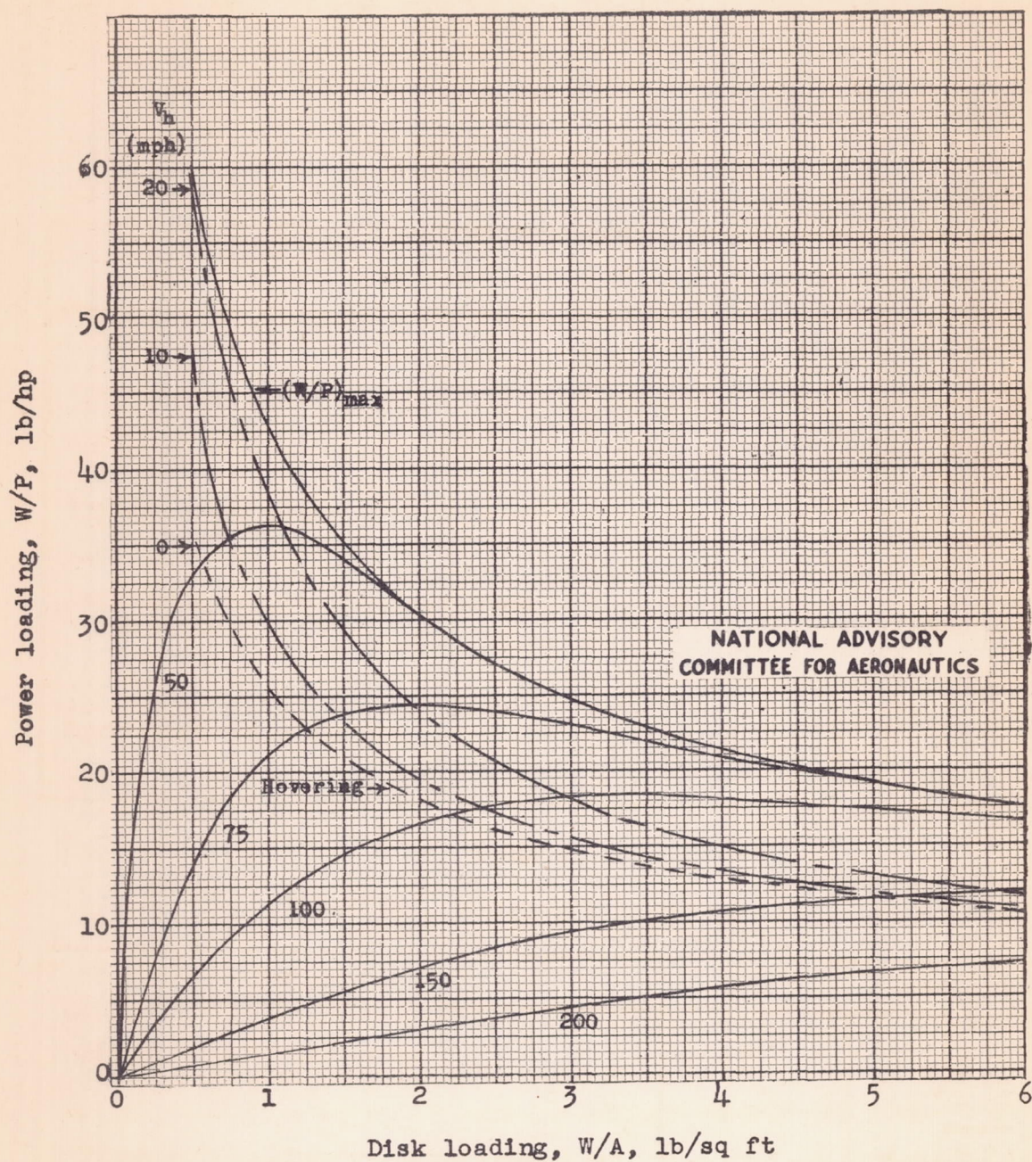
Figure 1.- Specialized selection chart for horizontal flight and hovering. \rho = 0.002378 slug per cubic foot; \delta = 0.012 ; \sigma = 0.056 ; Y_t = 320 ; R = 19.0 feet; f = 10.0 square feet.
