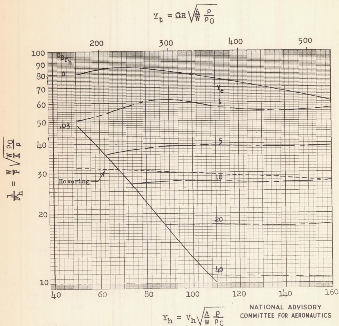
Figure 8.- Generalized performance chart for maximum rate of climb for the conditions of figure 5. \delta = 0.006 . ( V_h is the maximum speed, i.e. for Y_c = 0 .)
