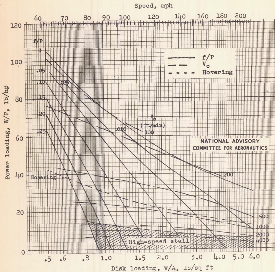
Figure 16.- Power-loading disk-loading performance chart for sea level. \mu = 0.4 ; \delta = 0.006 ; \sigma = 0.056 ; \sigma V_t^2 = 5740 .
