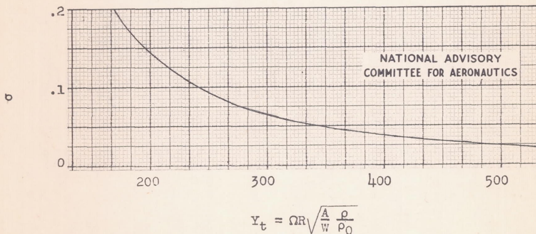
Figure 4.- Generalized performance chart for horizontal flight and hovering. \mu = 0.3 ; \delta = 0.012 ; \sigma Y_t^2 = 5740 .
