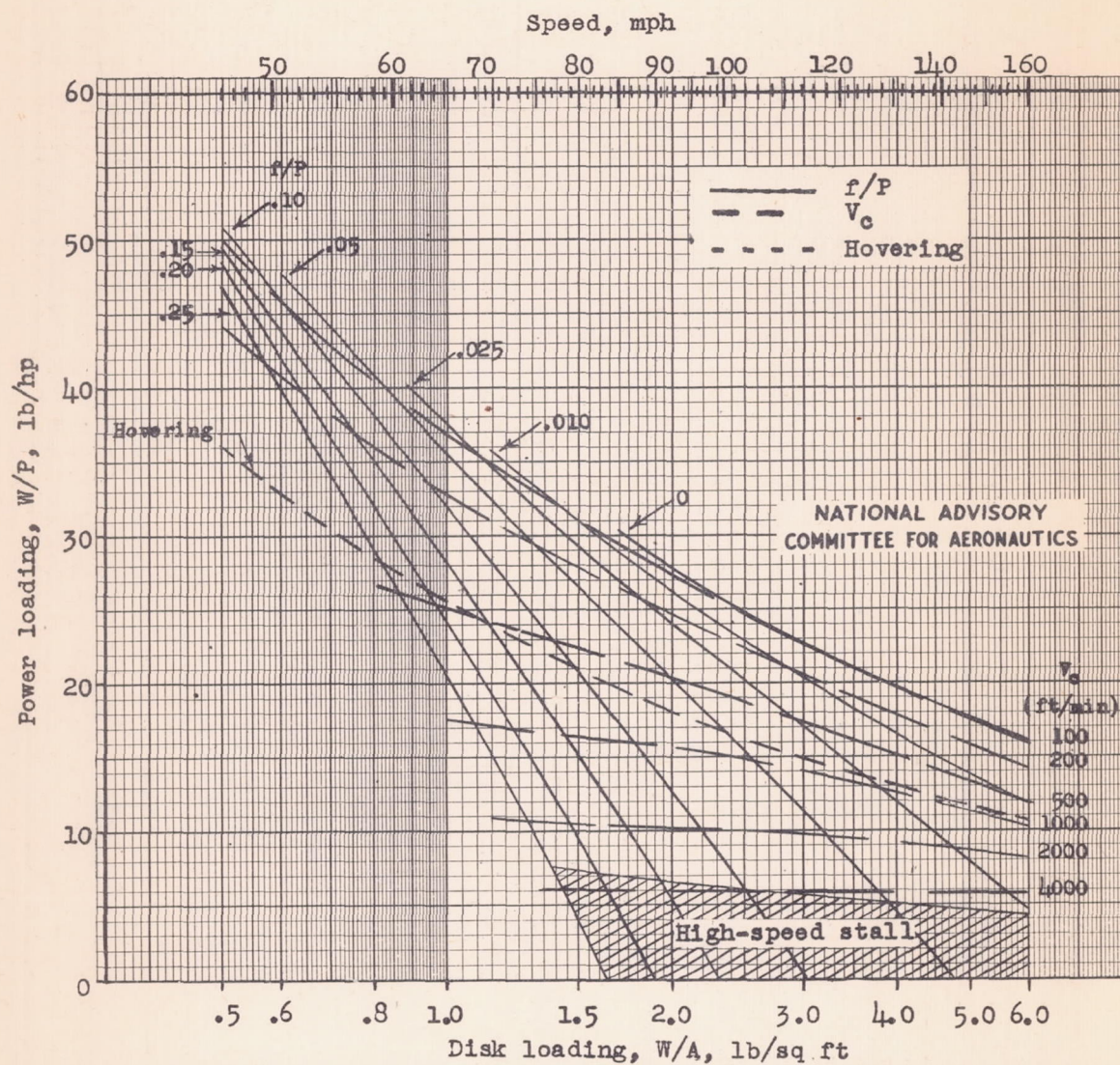
Figure 11.- Power-loading disk-loading performance chart for sea level. \mu = 0.3 ; \delta = 0.012 ; \sigma = 0.056 ; \sigma V_t^2 = 5740 .
