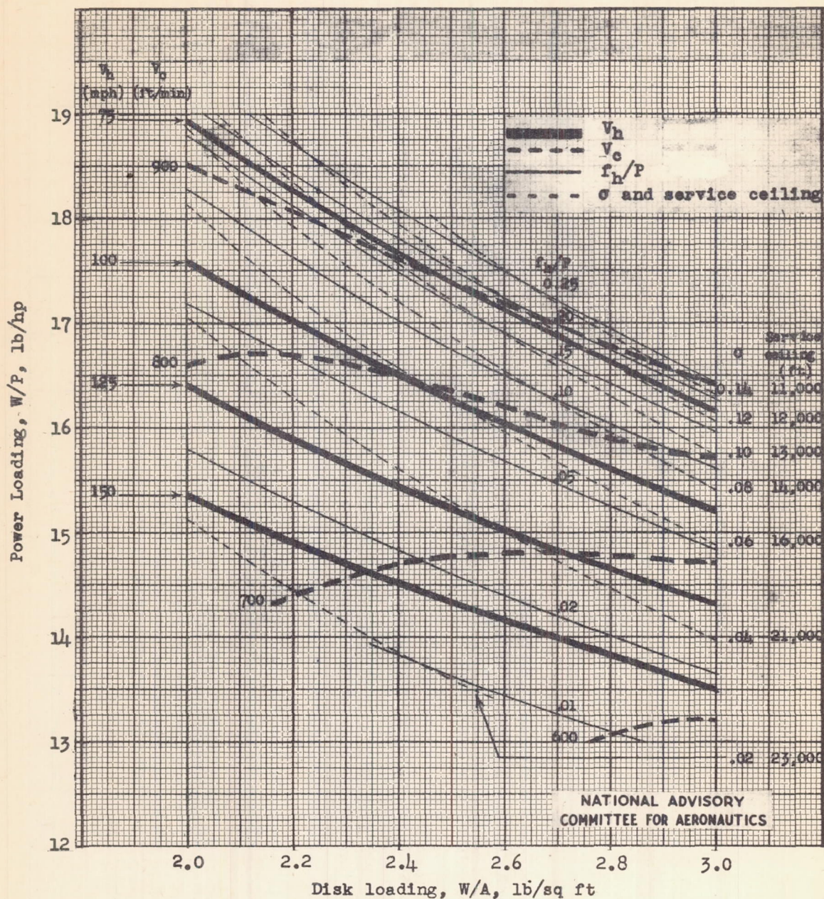
Figure 18.- Enlarged power-loading disk-loading performance chart for sea level for helicopters with power just sufficient to hover. \mu = 0.3 ; \delta = 0.012 ; \sigma Y_t^2 = 5740 .
