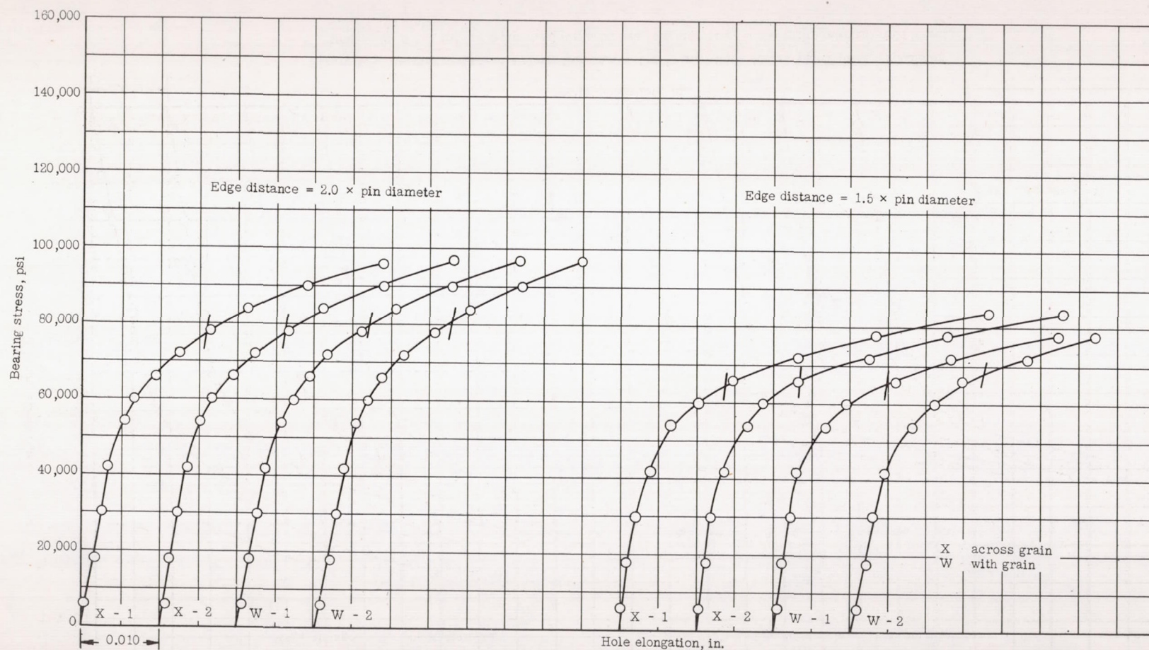
Figure 4.- Bearing stress-hole elongation curves for \frac{1}{4} -inch-thick Alclad 14S-W plate. Specimen thickness, 0.250 inch; specimen width, 2 inches; pin diameter, 0.500 inch; bearing-yield offset, 0.02 \times \text{pin diameter} .
