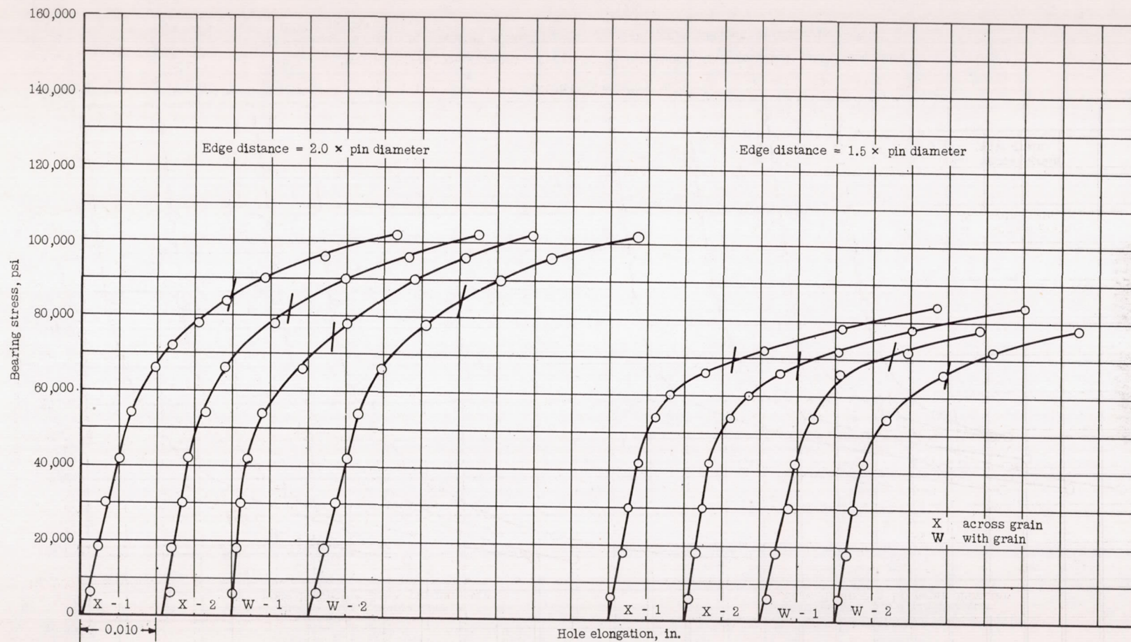
Figure 6.- Bearing stress-hole elongation curves for \frac{3}{4} -inch-thick 14S-W (nonclad) plate. Specimen thickness, 0.250 inch; specimen width, 2 inches; pin diameter, 0.500 inch; bearing-yield offset, 0.02 \times pin diameter.
