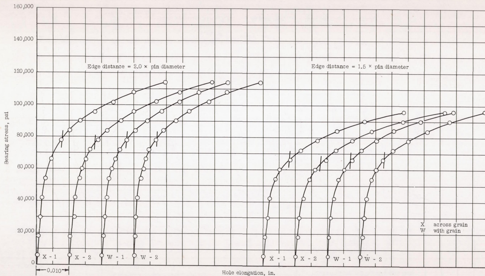
Figure 2.- Bearing stress-hole elongation curves for 0.064-inch-thick Alclad 14S-W sheet. Specimen thickness, 0.064 inch; specimen width, 2 inches; pin diameter, 0.250 inch; bearing-yield offset, 0.02 \times pin diameter.
