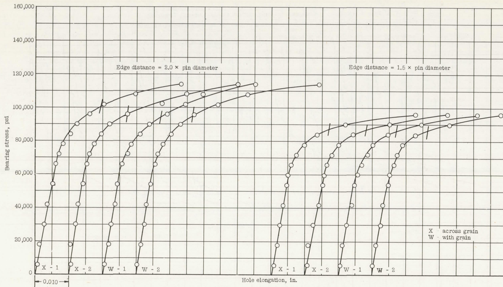
Figure 5.- Bearing stress-hole elongation curves for \frac{1}{4} -inch-thick Alclad 14S-T plate. Specimen thickness, 0.250 inch; specimen width, 2 inches; pin diameter, 0.500 inch; bearing-yield offset, 0.02 \times pin diameter.
