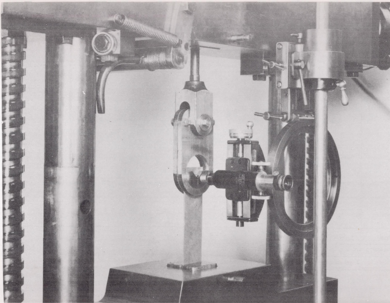
Figure 1.- Arrangement for bearing tests. Microscope used for measurement of hole elongations.
