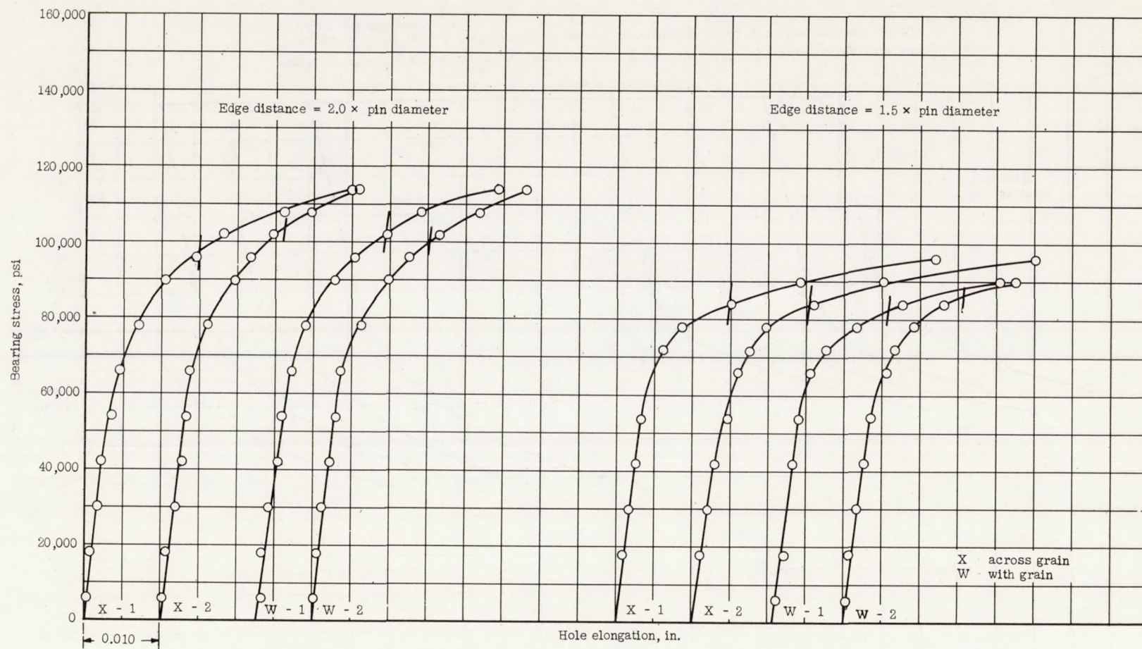
Figure 7.- Bearing stress-hole elongation curves for \frac{3}{4} -inch-thick 14S-T (nonclad) plate. Specimen thickness, 0.250 inch; specimen width, 2 inches; pin diameter, 0.500 inch; bearing-yield offset, 0.02 \times pin diameter.
