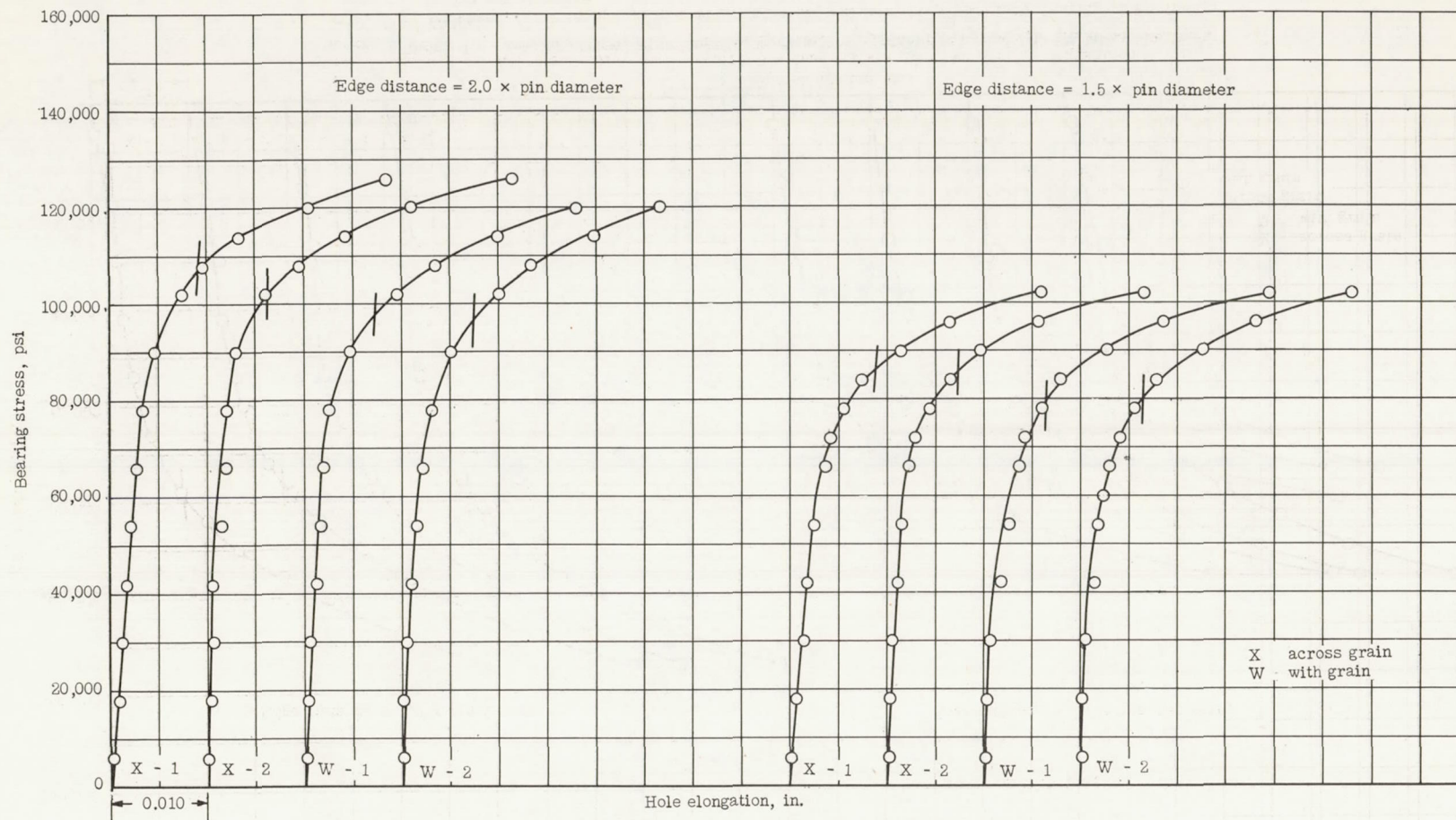
Figure 3.- Bearing stress-hole elongation curves for 0.064-inch-thick Alclad 14S-T sheet. Specimen thickness, 0.064 inch; specimen width, 2 inches; pin diameter, 0.250 inch; bearing-yield offset, 0.02 \times pin diameter.
