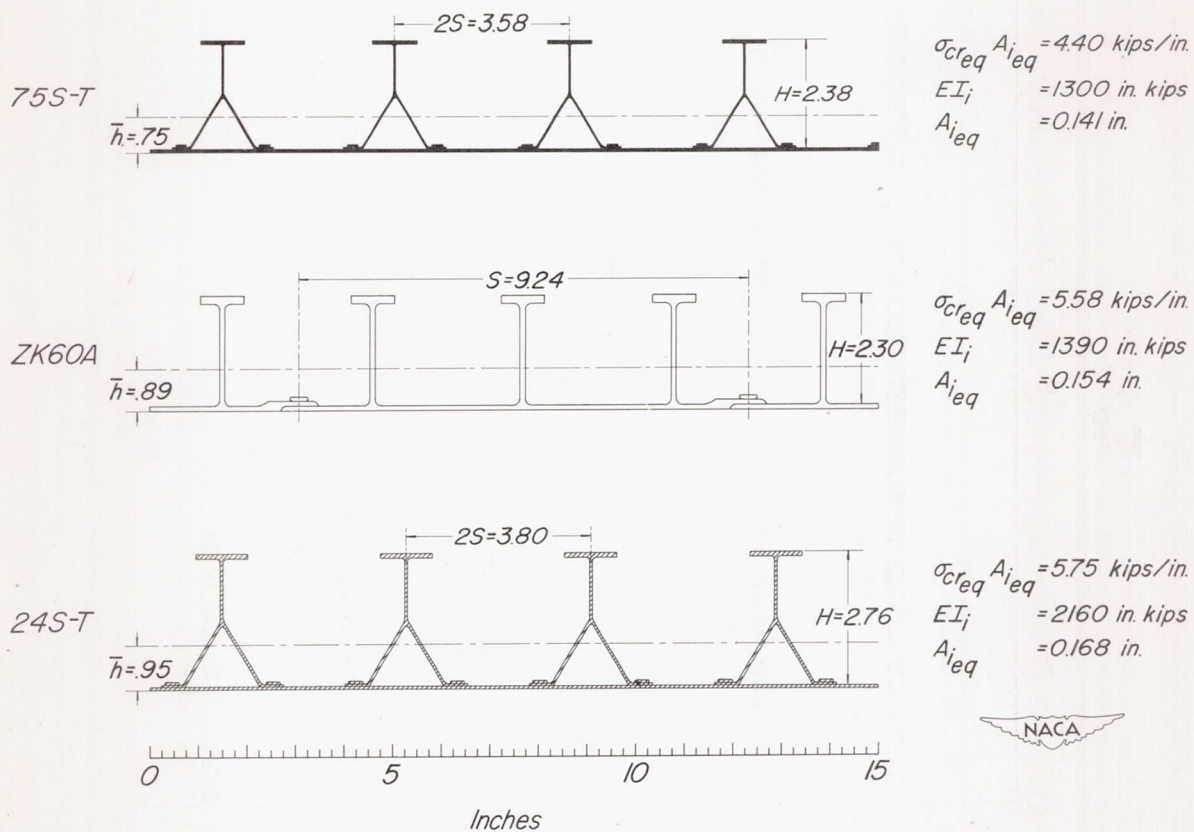
Figure 7.—Comparison of characteristics of the ZK60A extruded panel and 24S-T and 75S-T Y-stiffened panel designs for P_i = 5.75 kips per inch, t_{seq} = 0.064 inch, and \frac{L}{\sqrt{C}} = 39.2 inches.
