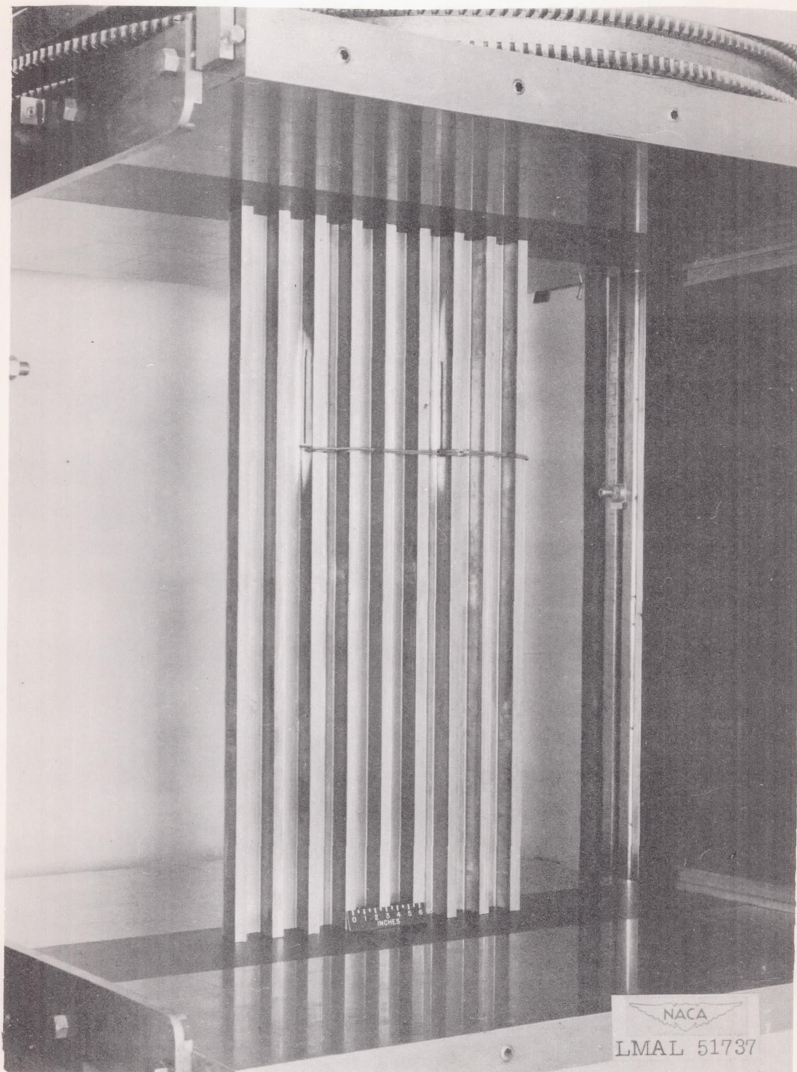
Figure 4.- Test specimen in testing machine. \frac{L}{p} = 55 .
