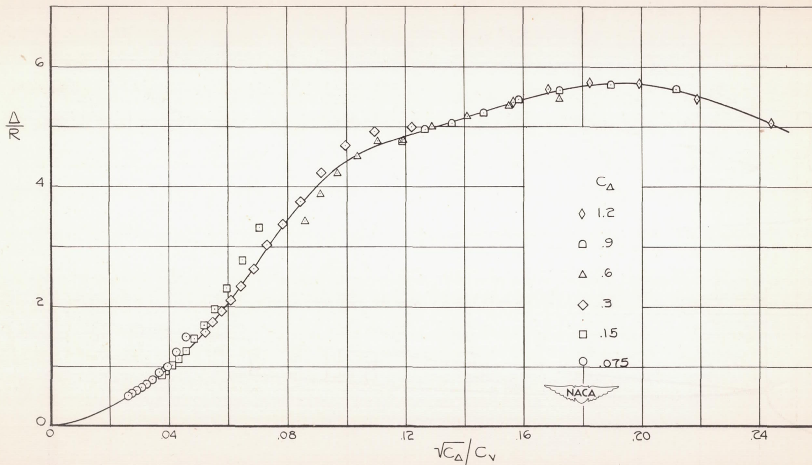
Figure 8.- Chart for estimation of resistance of NACA model 57-B-5 float at high speed and load coefficients. Trim, 6^\circ .
