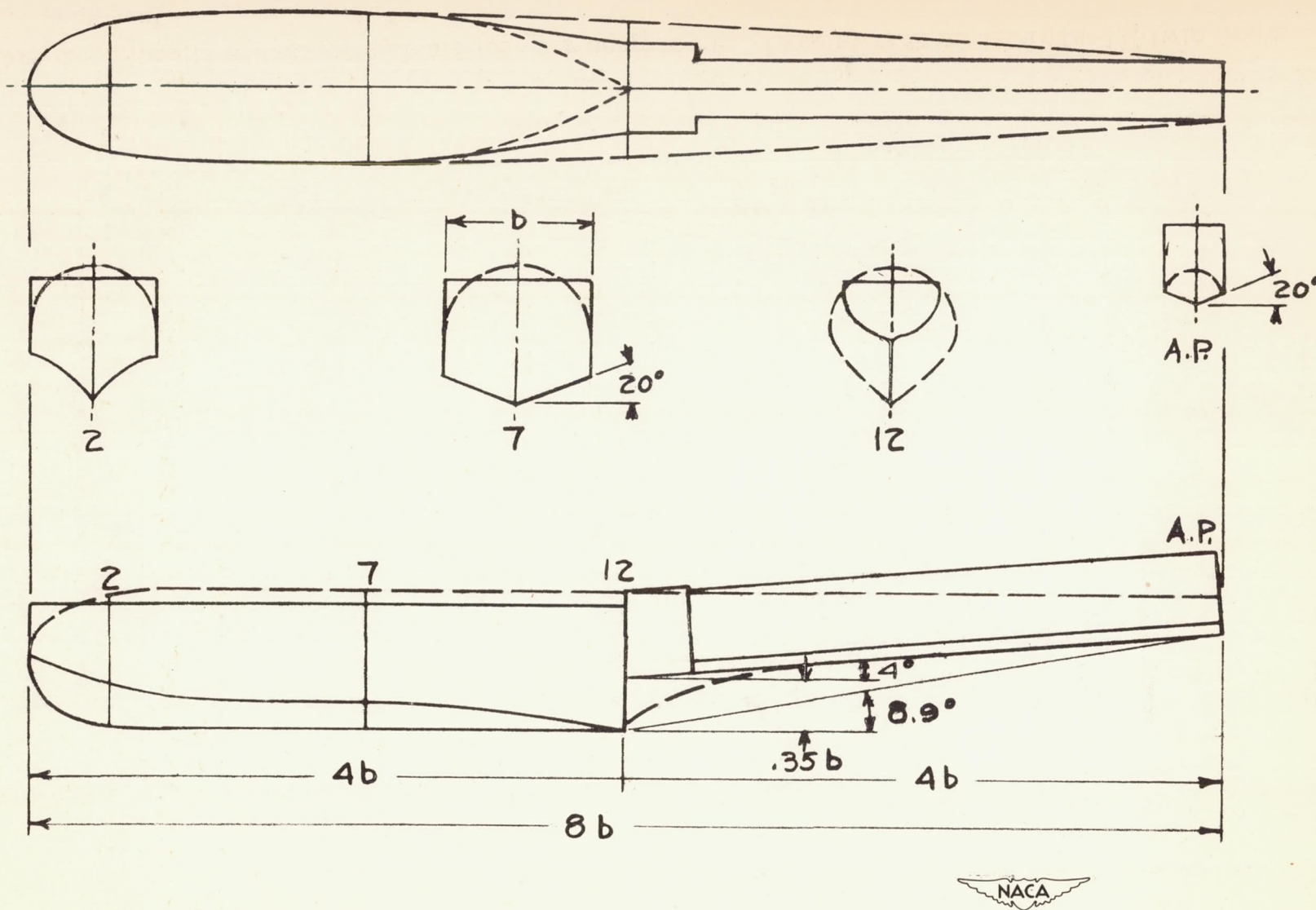
Figure 5.- Langley tank model 163A-11 planing-tail hull. Possible form of float shown by dashed lines.
