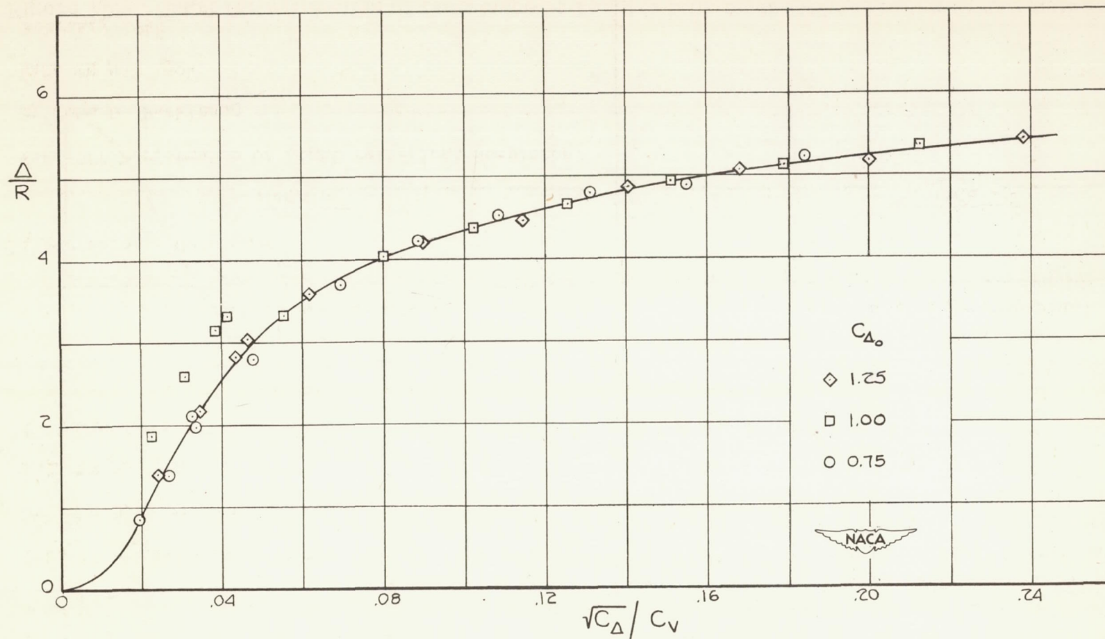
Figure 11.- Chart for estimation of resistance of Langley tank model 163A-11 planing-tail hull at high speed and load coefficients. Trim, 8^\circ .
