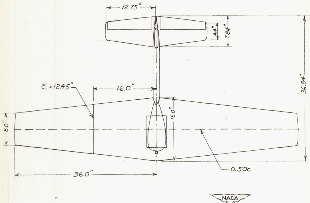
Figure 4.- Equivalent straight-wing model.
