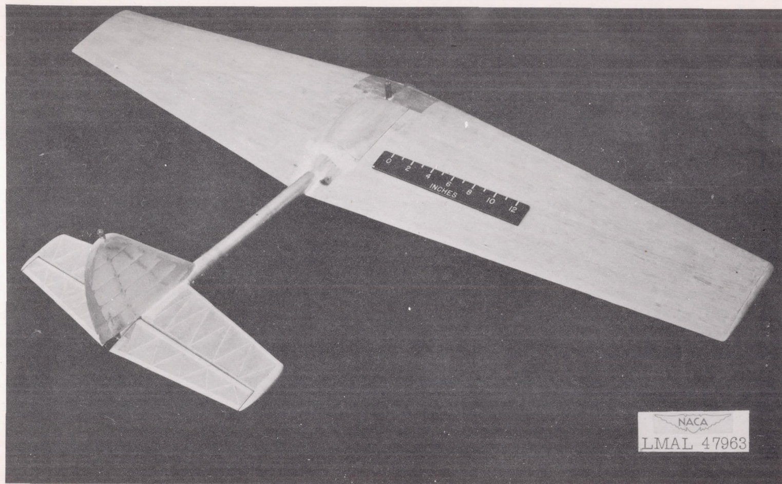
Figure 2.- Equivalent straight-wing model.
