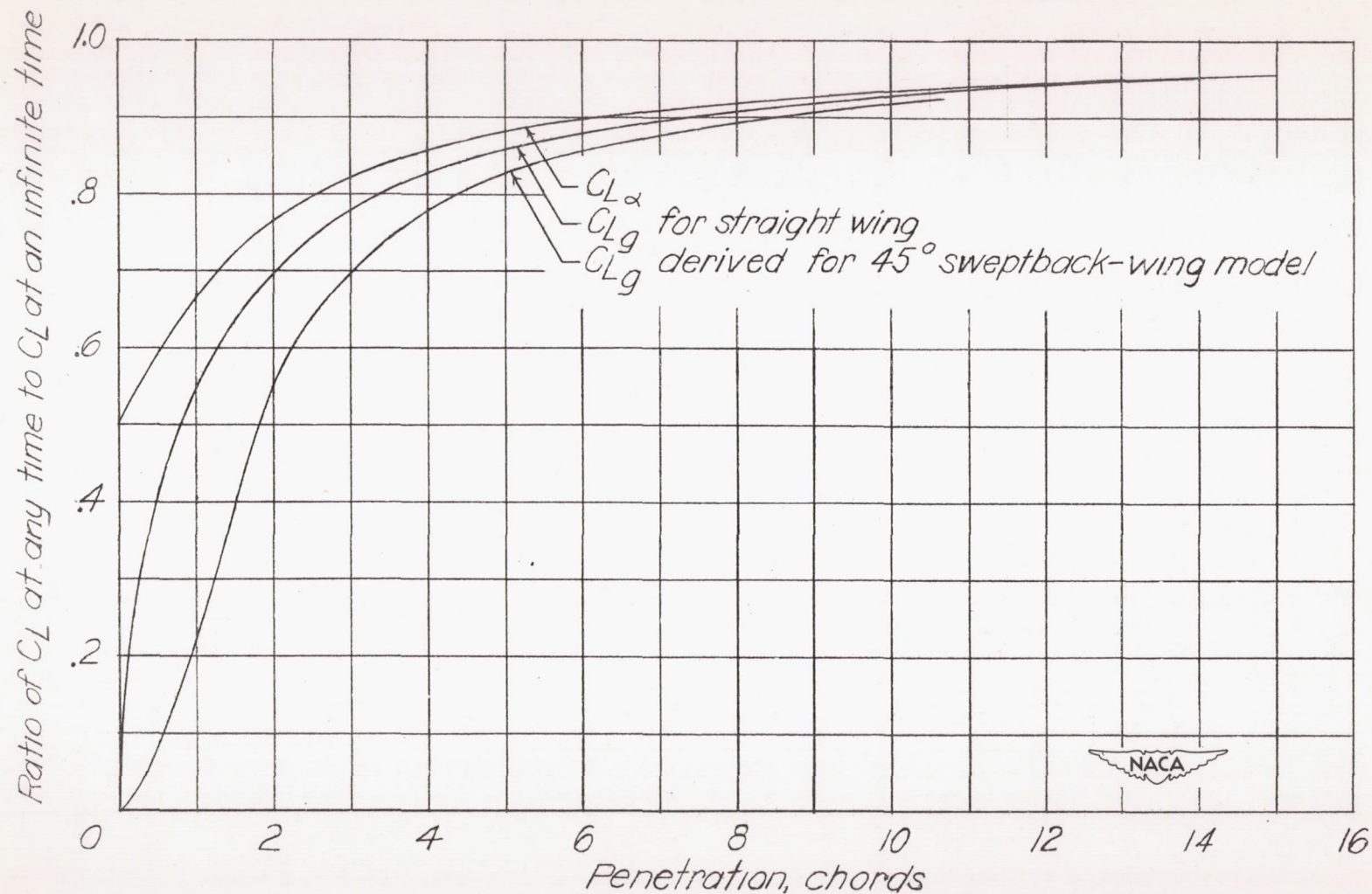
Figure 9 - Curves of C_{Lg} and C_{L\alpha} for infinite aspect ratio based on Jones' unsteady-lift functions (reference 5).
