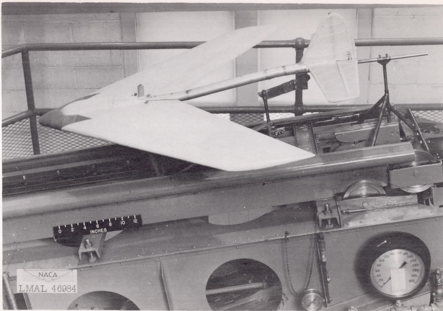
Figure 1.- Sweptback-wing model without fuselage.
