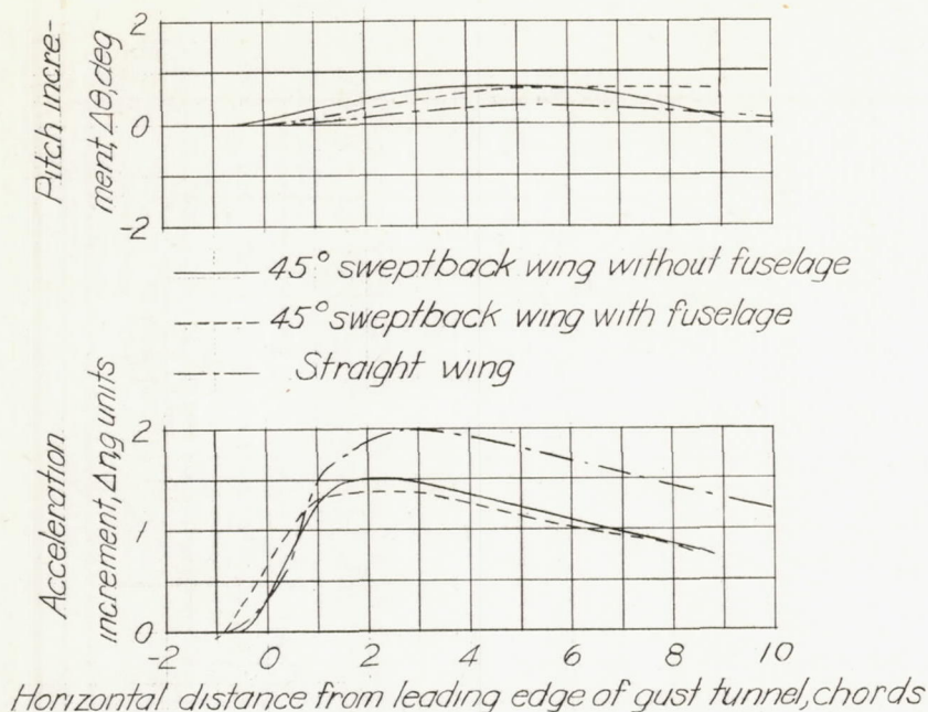
(a) Sharp-edge gust.
