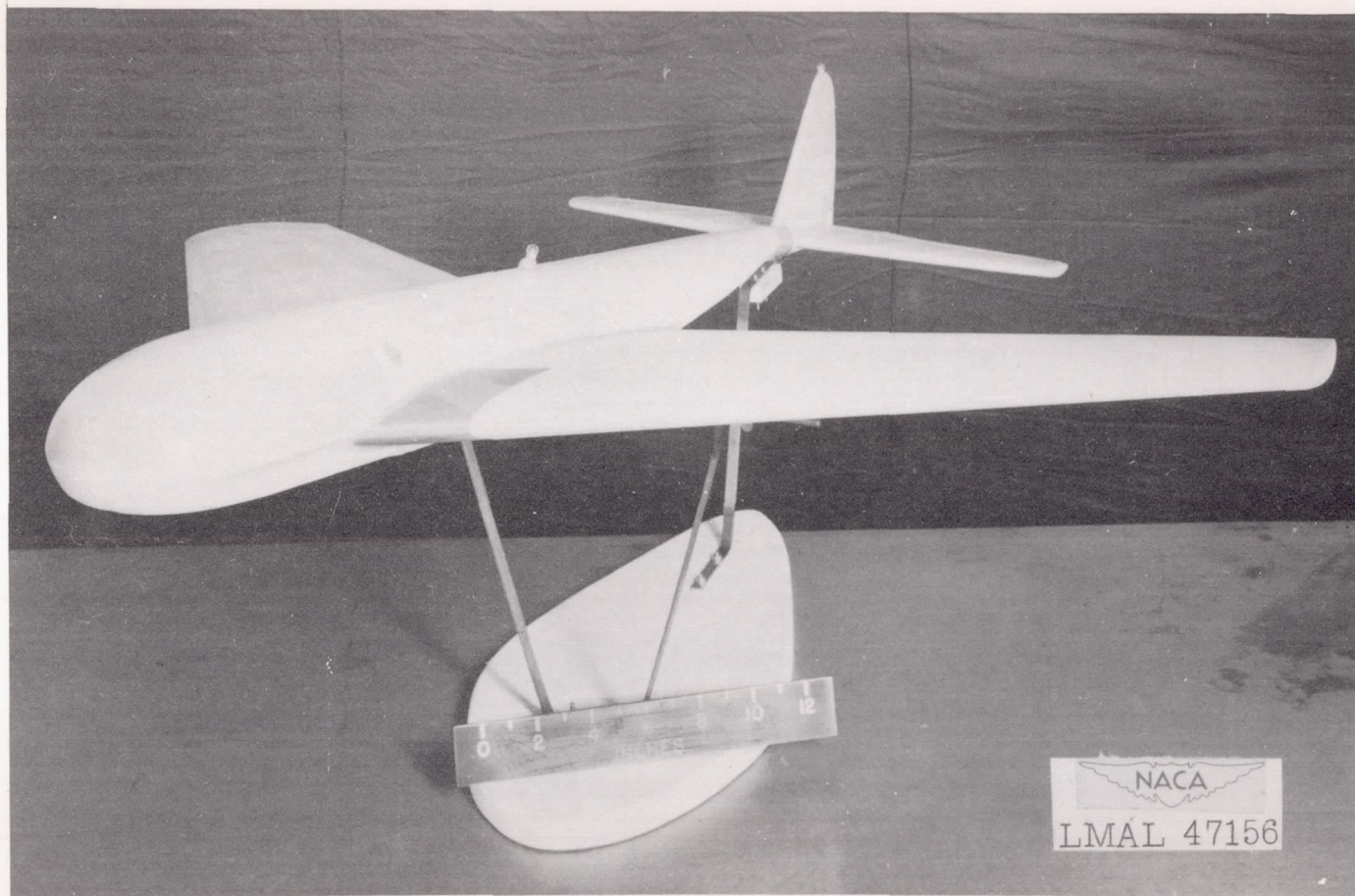
Figure 5.- Sweptback-wing model with fuselage.
