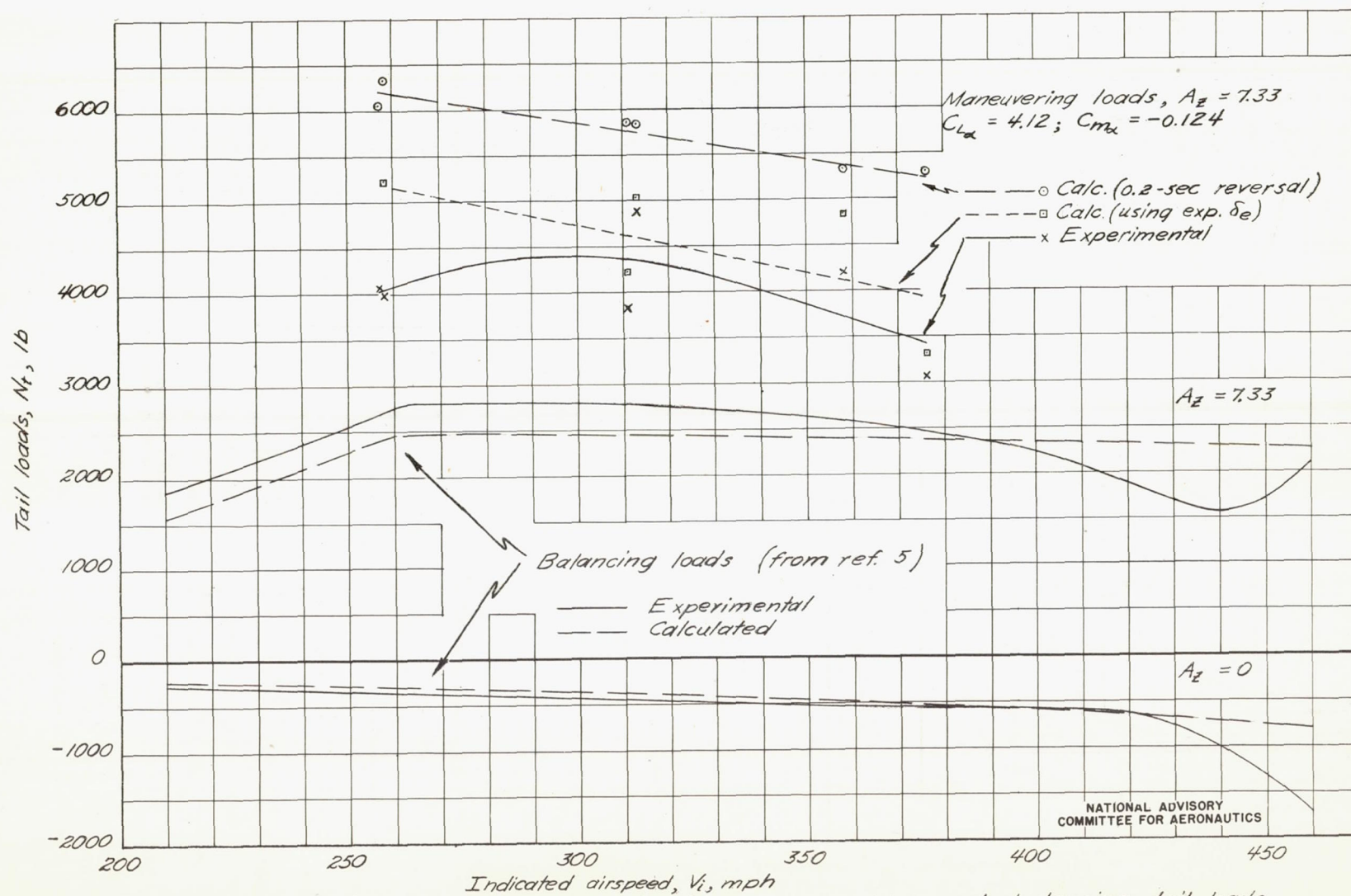
Figure 10. — The variation with indicated airspeed of the maneuvering and balancing tail loads.
