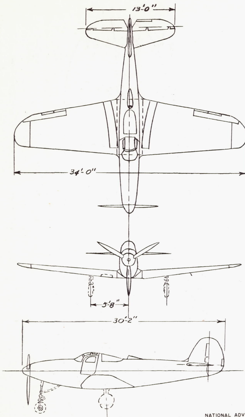
Figure 3. - Three-view drawing of the test airplane.
