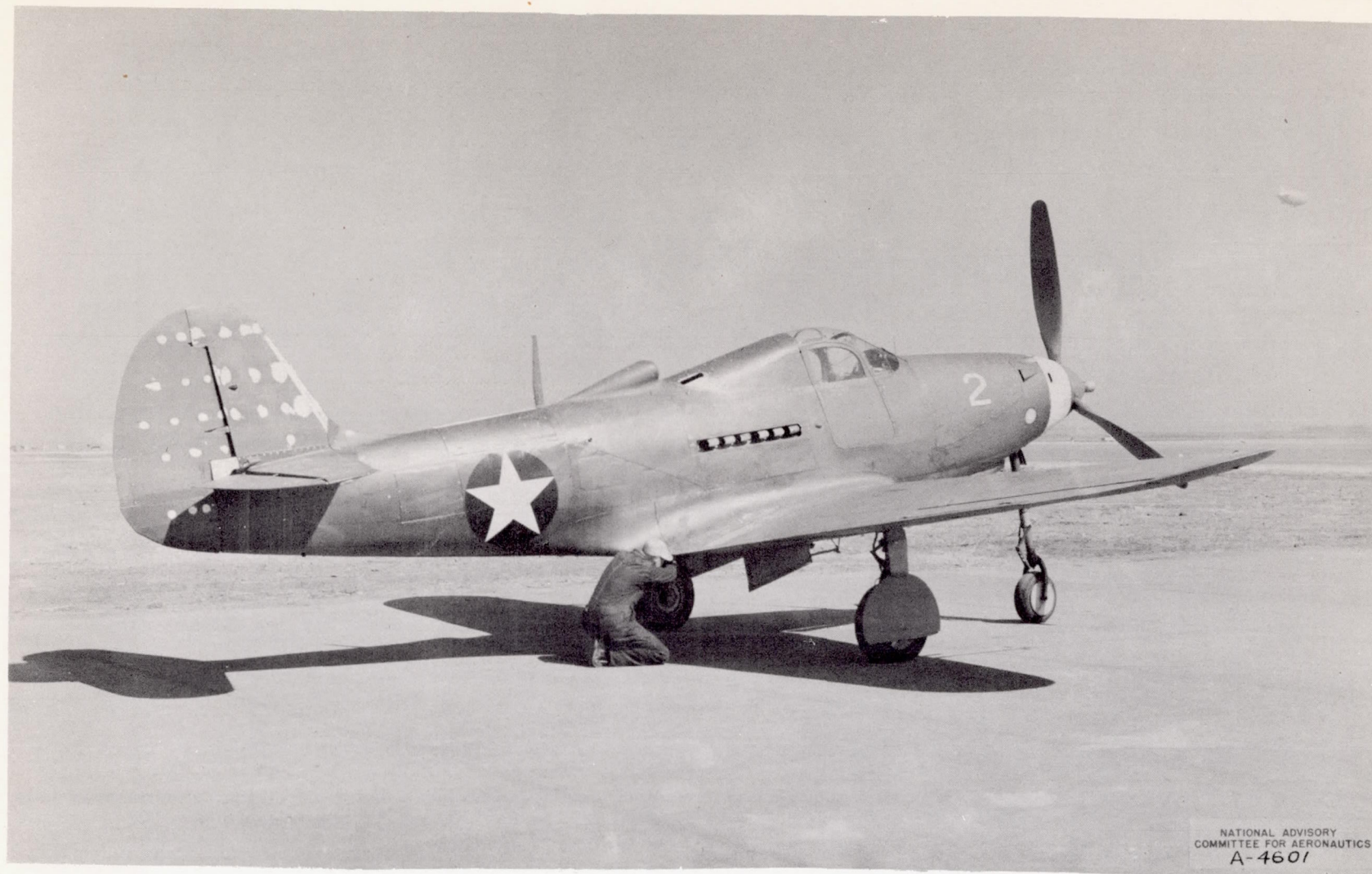
Figure 1.- Three-quarter rear view of test airplane as instrumented for tail-load flight tests.
