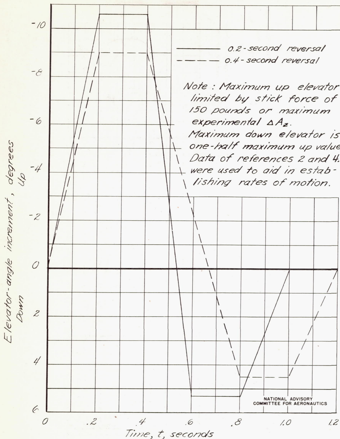
Figure 5. — Typical computed linear elevator motions used to determine the maneuvering tail-load increments by the tabular method.
