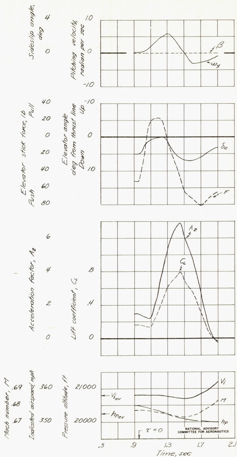
Figure 6. - Time histories of basic flight data.
