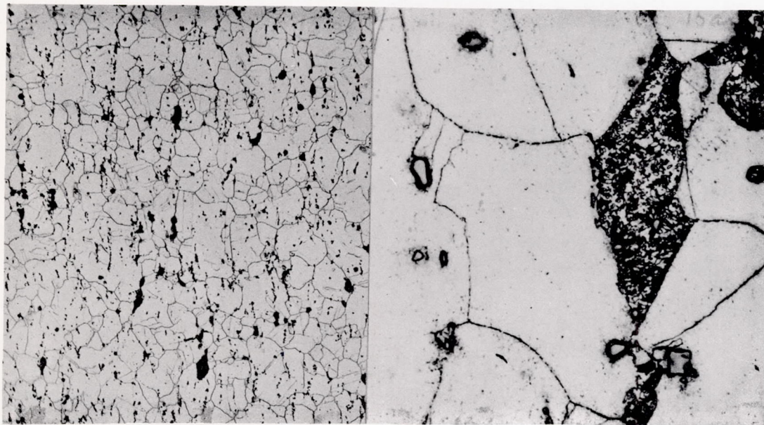
100X 1000X (a) Creep specimen 1Z; 1129 hours under 30,000 psi.
