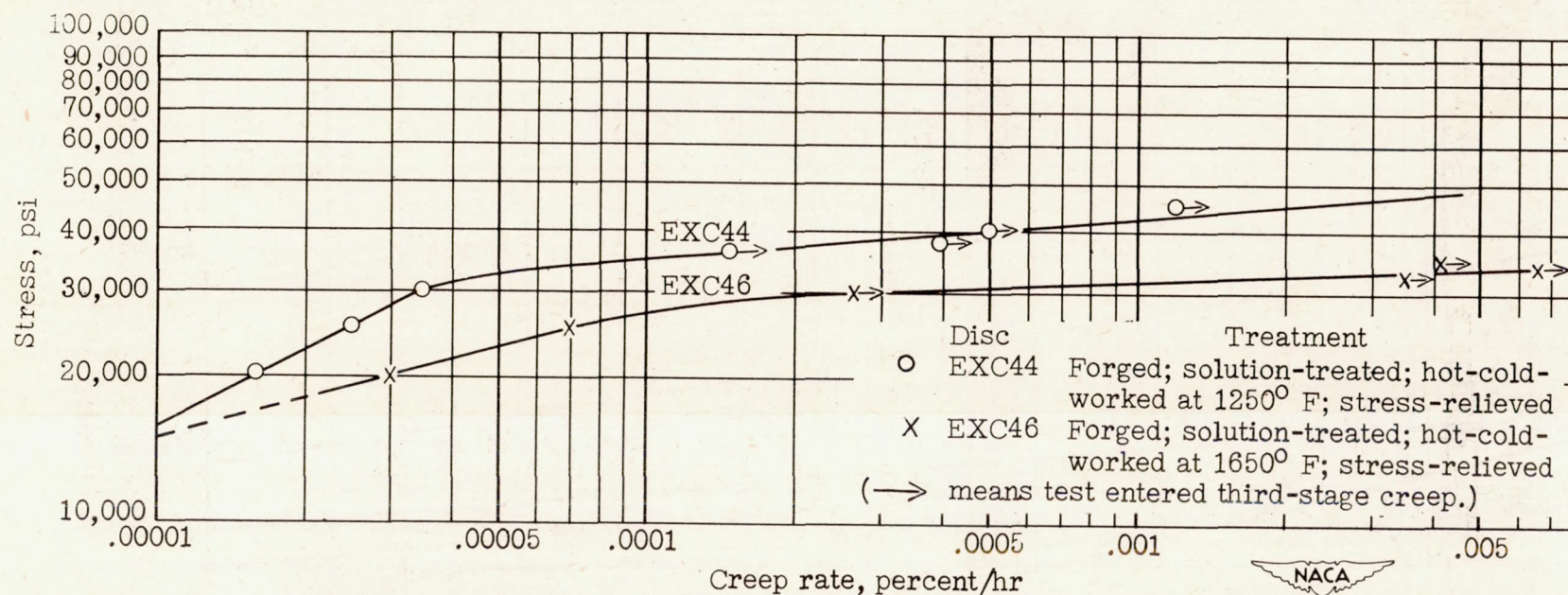
Figure 9.- Curves of stress against creep rate at 1200° F for contour discs of 19-9DL alloy. All data at stresses above 30,000 psi from rupture tests.
