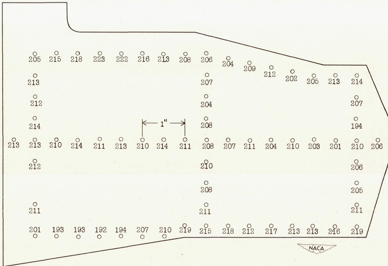
Figure 5.- Hardness survey on a half section of contour disc EXC46 or 19-9DL alloy. Brinell hardness; disc section 8.
