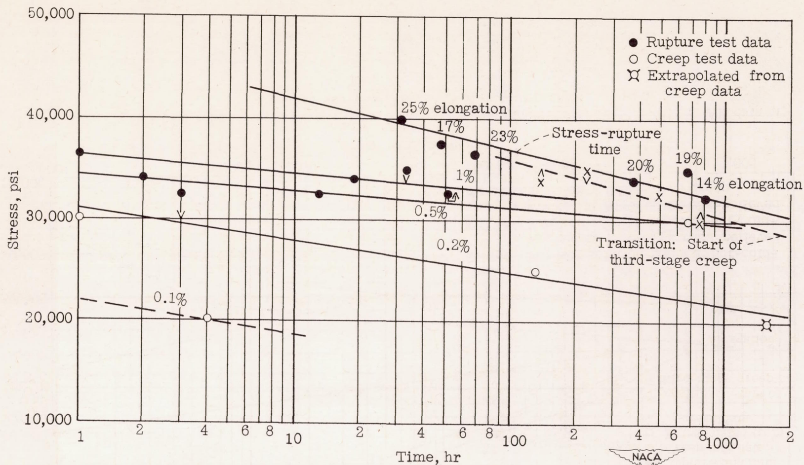
Figure 8.- Curves of stress against time for total deformation at 1200° F for contour disc EXC46 of 19-9DL alloy. (Treatment: Forged; solution-treated; hot-cold-worked at 1650° F; stress-relieved.)
