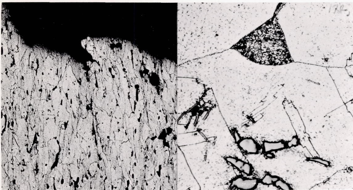
(a) Creep specimen 1Z; 1124 hours under 30,000 psi.
