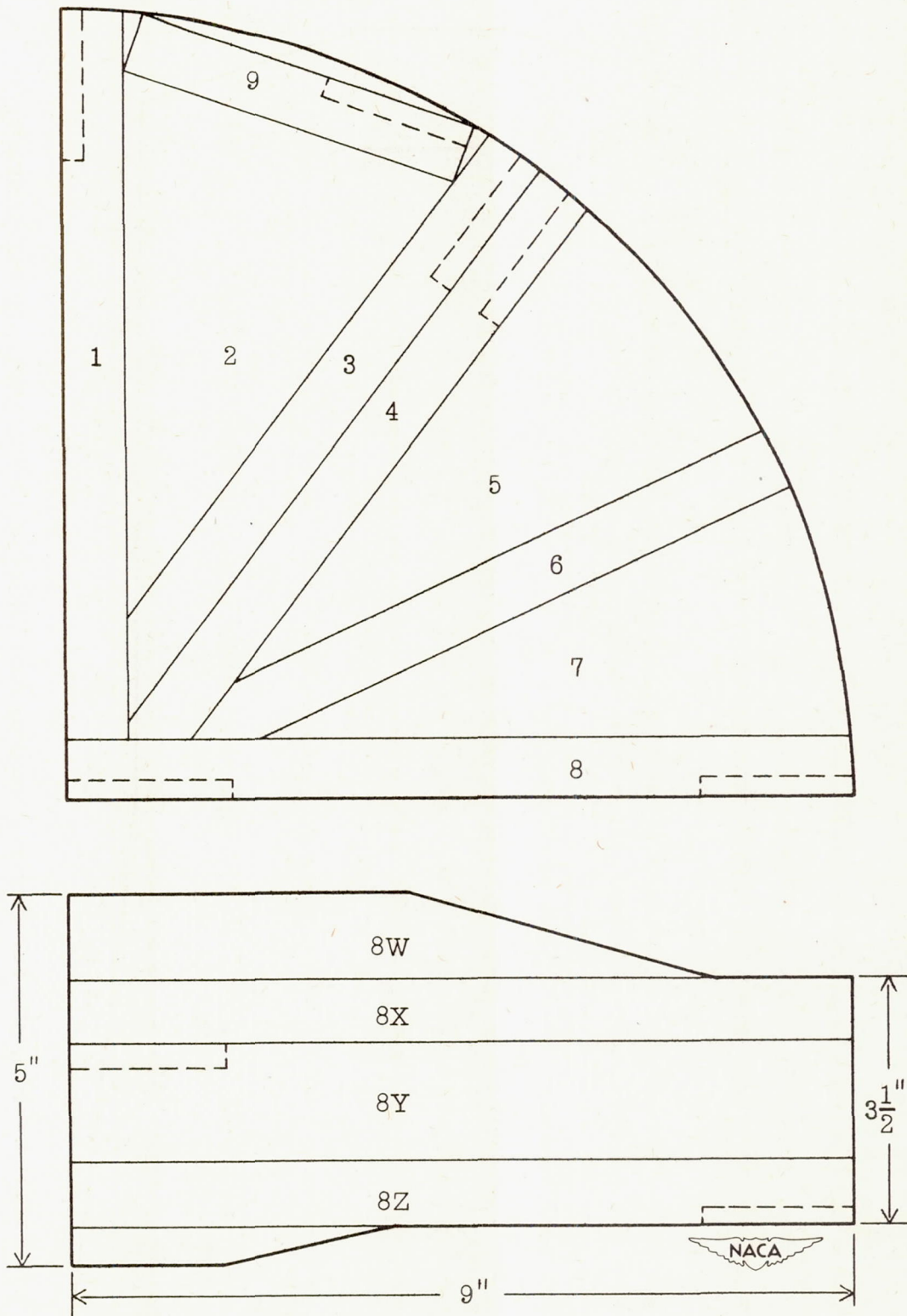
Figure 3.- Diagram showing location of test coupons in quarter sections of contour discs EXC44 and EXC46 of 19-9DL alloy.
