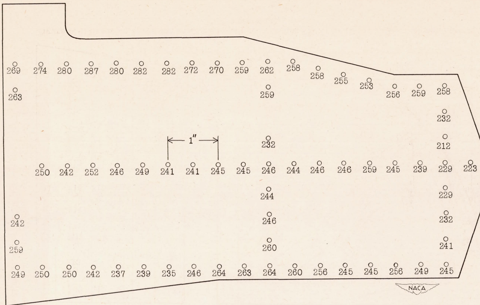
Figure 4.- Hardness survey on a half section of contour disc EXC44 of 19-9DL alloy. Brinell hardness; disc section 8.
