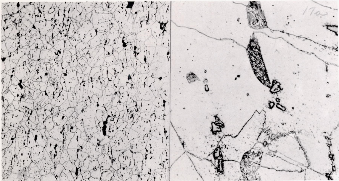
(a) Creep specimen 1Z; 1124 hours under 30,000 psi.
