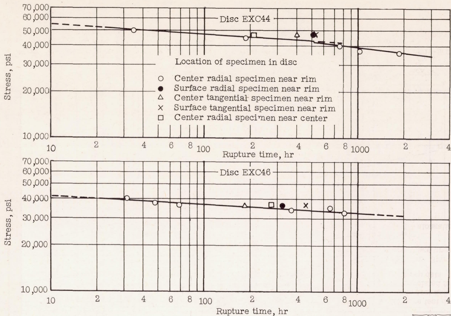
Figure 6.- Curves of stress against rupture time at 1200° for contour discs of 19-9DL alloy.
