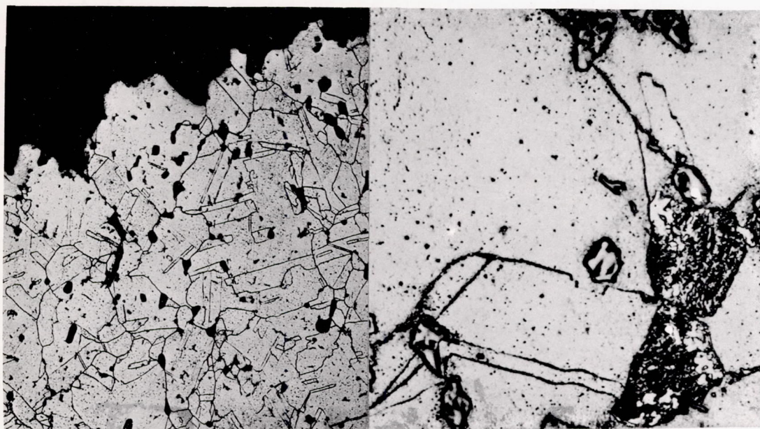
100X 1000X (a) Creep specimen 1Z; 1129 hours under 30,000 psi.
