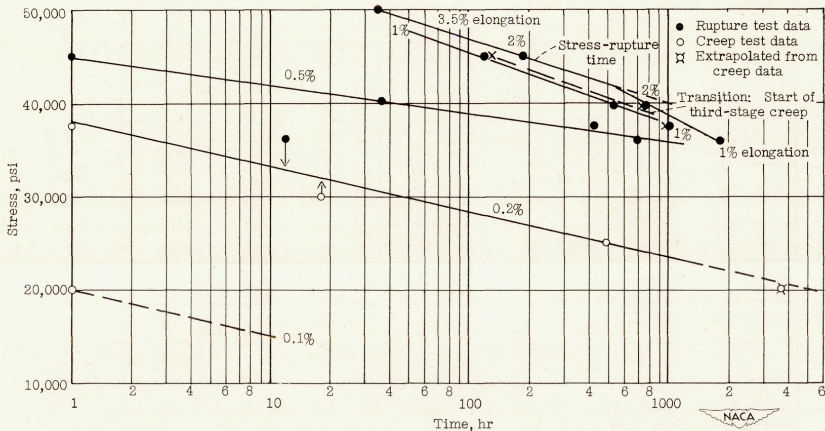
Figure 7.- Curves of stress against time for total deformation at 1200° F for contour disc EXC44 of 19-9DL alloy. (Treatment: Forged; solution-treated; hot-cold-worked at 1250° F; stress-relieved.)
