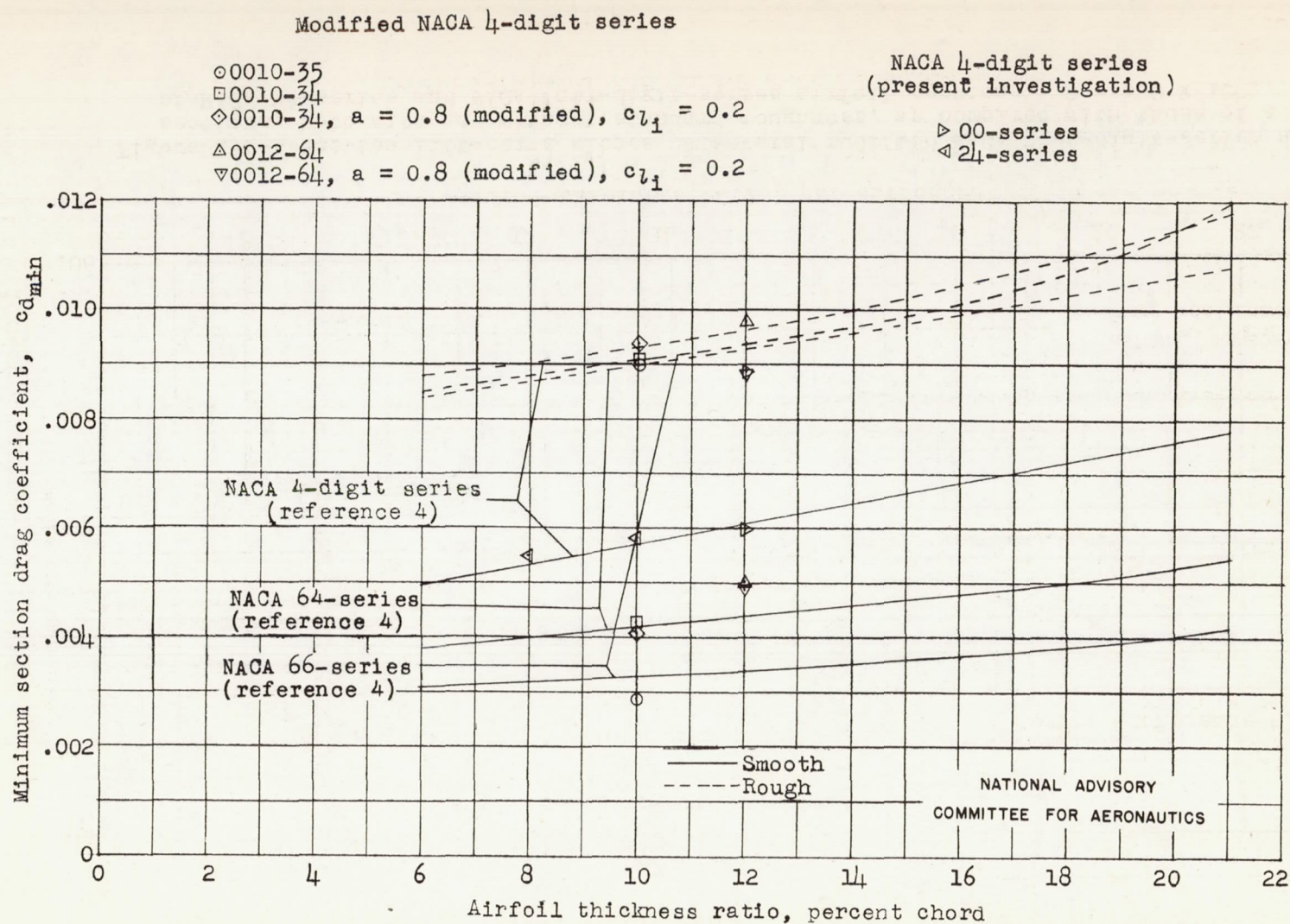
Figure 18.- Minimum section drag coefficients of several modified NACA four-digit-series airfoil sections, both with and without standard roughness, as compared with those of a number of NACA 6-series and NACA four-digit-series airfoil sections. R = 6.0 \times 10^6 .
