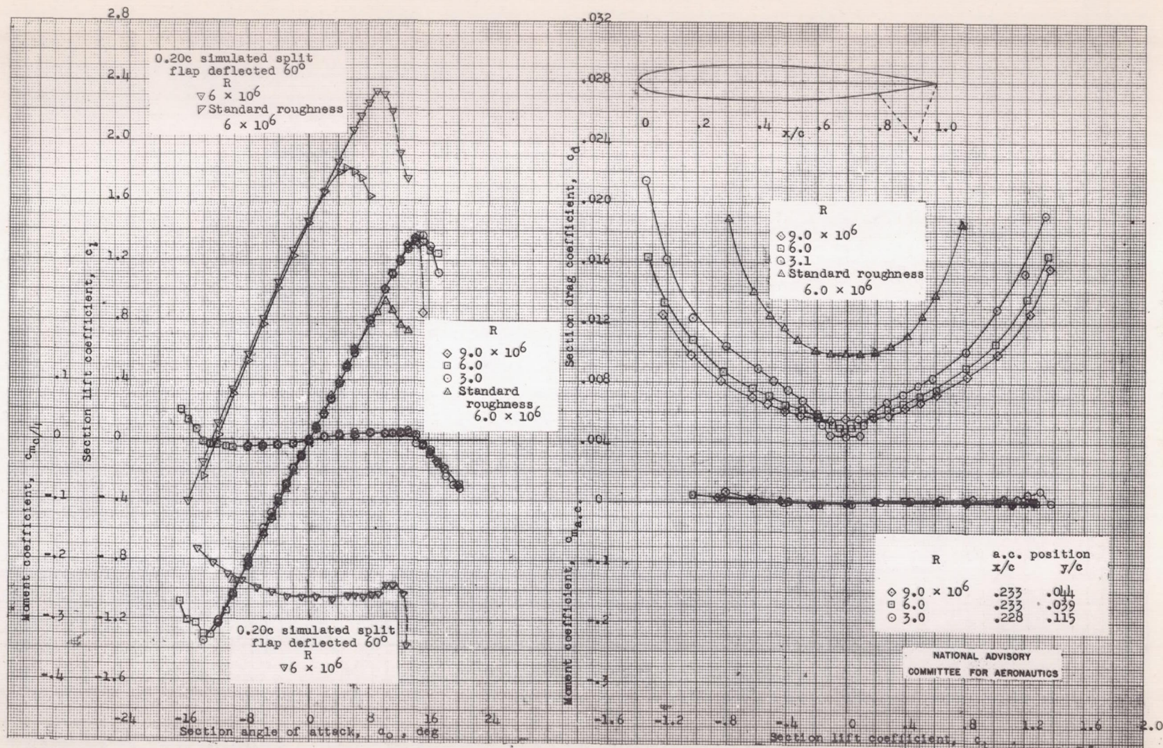
Figure 13.- Aerodynamic characteristics of the NACA 0012-64 airfoil section, 24-inch chord.
