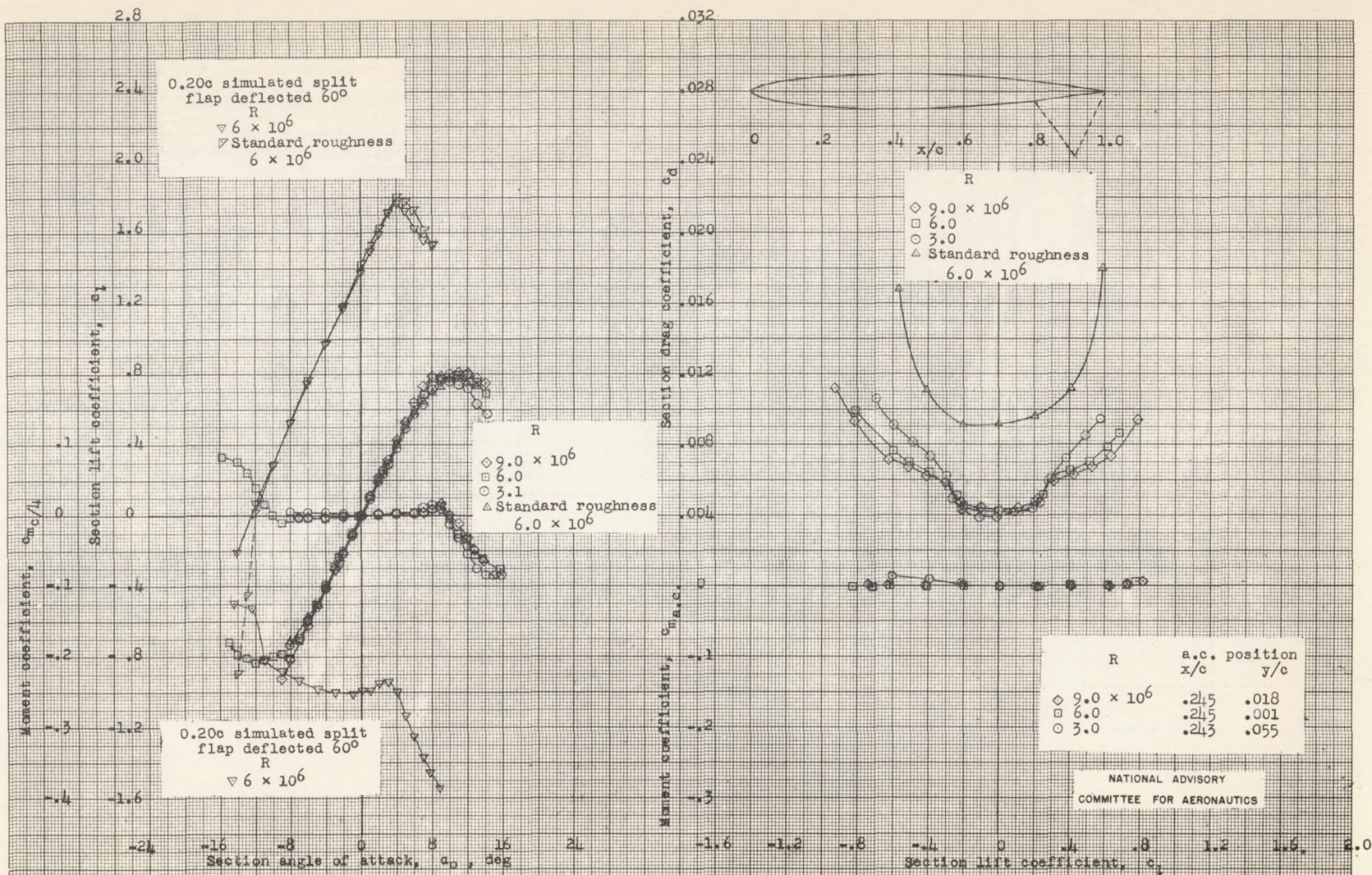
Figure 10.- Aerodynamic characteristics of the NACA 0010-34 airfoil section, 24-inch chord.
