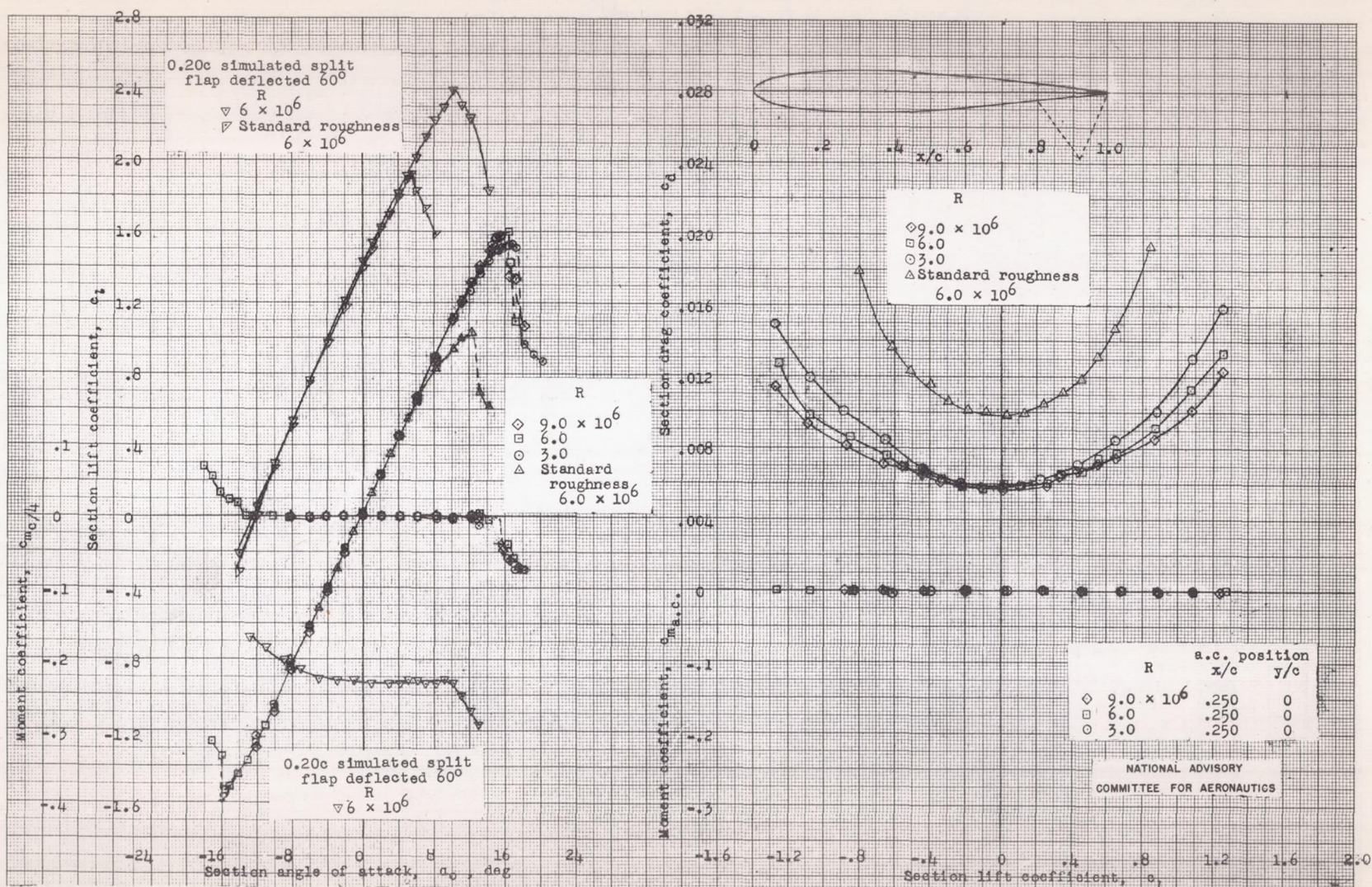
Figure 15.- Aerodynamic characteristics of the NACA 0012 airfoil section, 24-inch chord.
