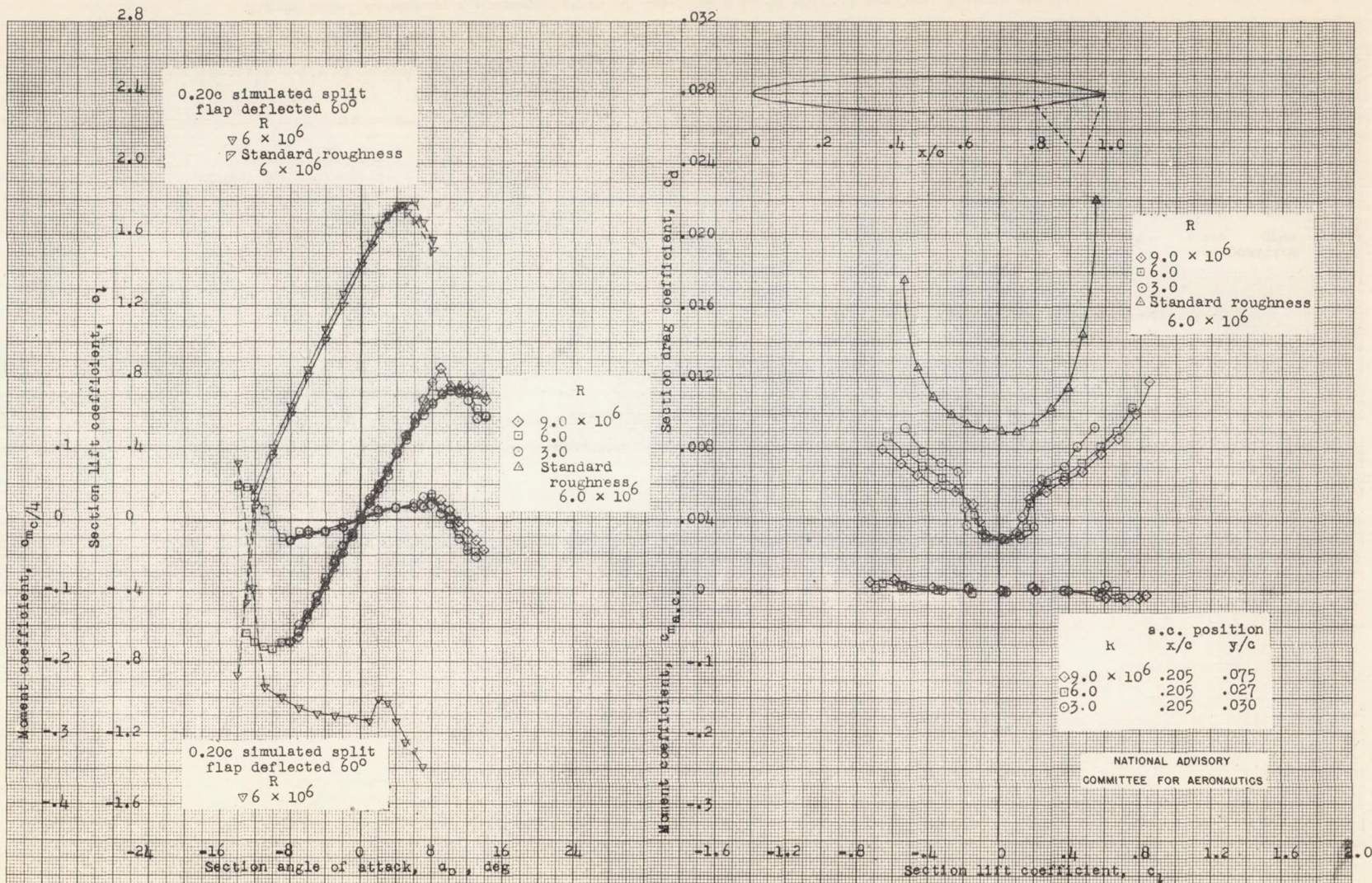
Figure 12.- Aerodynamic characteristics of the NACA 0010-35 airfoil section, 24-inch chord.
