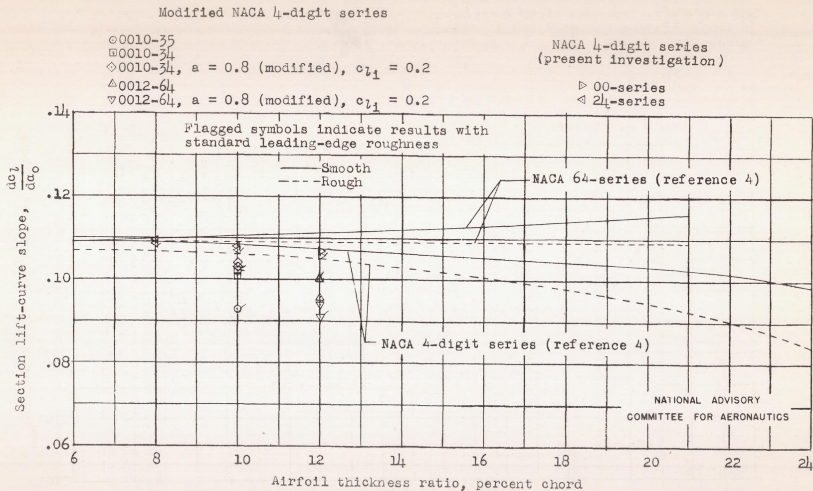
Figure 19.- Section lift-curve slopes of several modified NACA four-digit-series airfoil sections, both with and without standard roughness, as compared with those of a number of NACA 64-series and NACA four-digit-series airfoil sections. R = 6.0 \times 10^6 .
