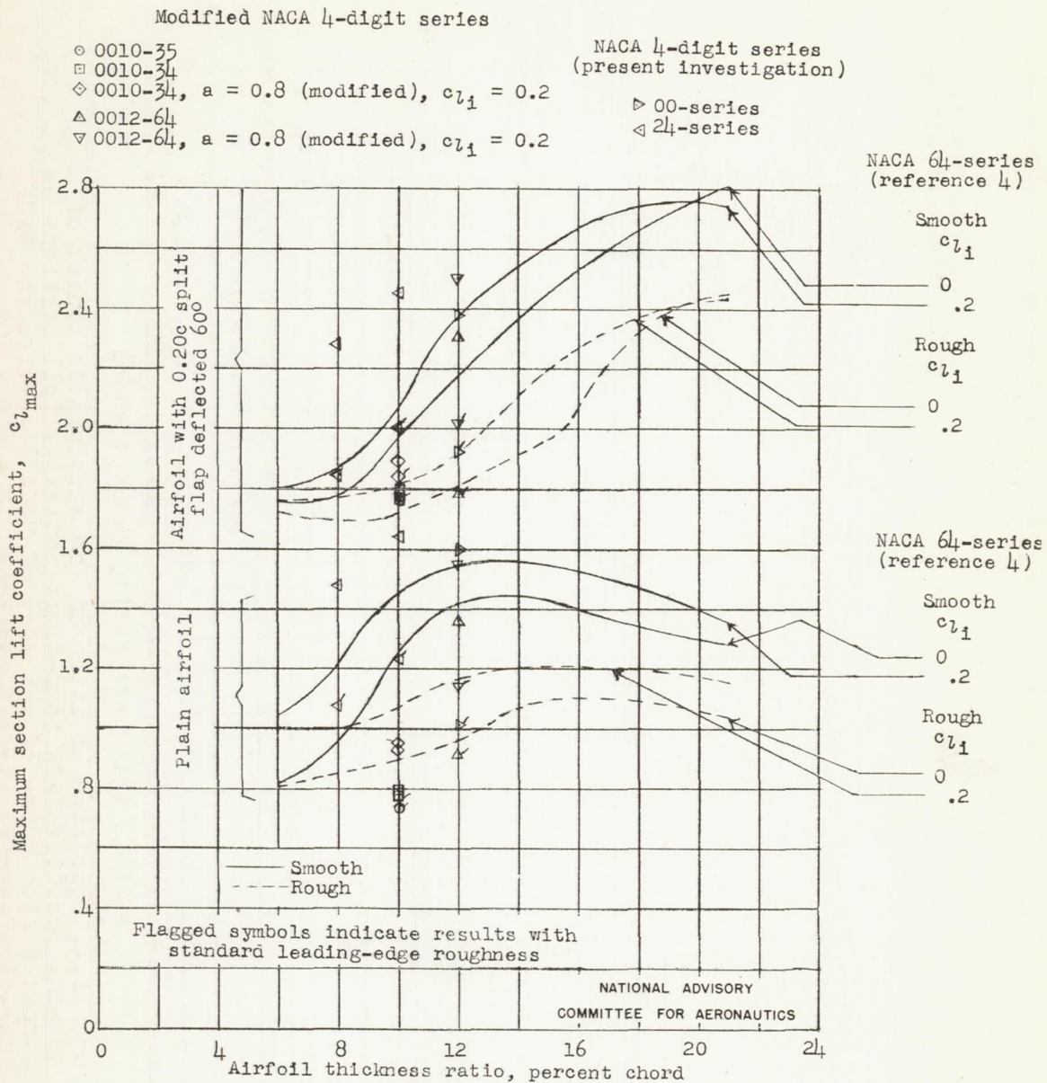
Figure 20.- Maximum section lift coefficients of several modified NACA four-digit-series airfoil sections, both with and without standard roughness and split flaps, as compared with those of a number of NACA 64-series and NACA four-digit-series airfoil sections. R = 6.0 \times 10^6 .
