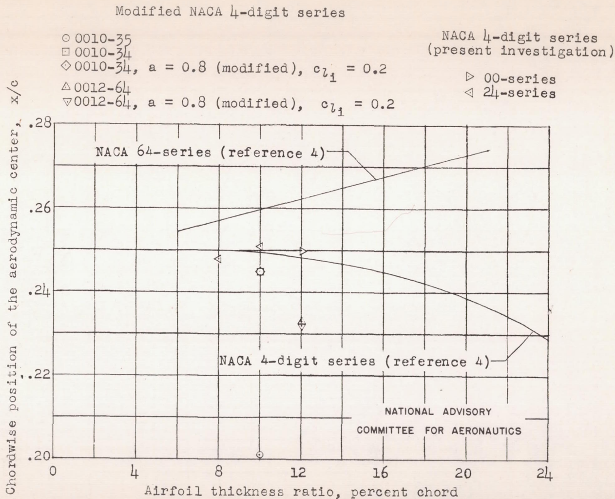
Figure 21.- Chordwise position of the aerodynamic center of several modified NACA four-digit-series airfoil sections as compared with those of a number of NACA 64-series and NACA four-digit-series airfoil sections. R = 6.0 \times 10^6 .
