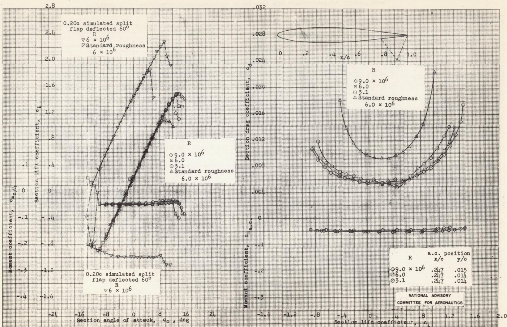
Figure 16.- Aerodynamic characteristics of the NACA 2408 airfoil section, 24-inch chord.
