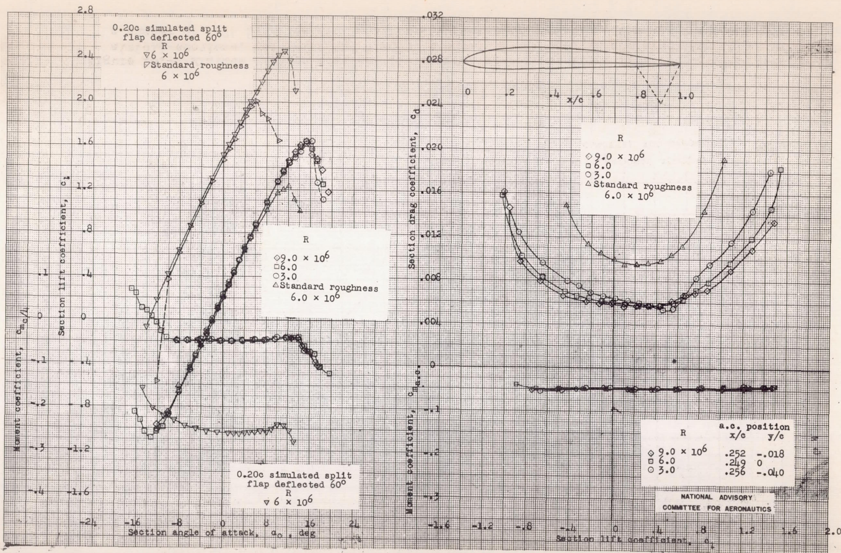
Figure 17.- Aerodynamic characteristics of the NACA 2410 airfoil section, 24-inch chord.
