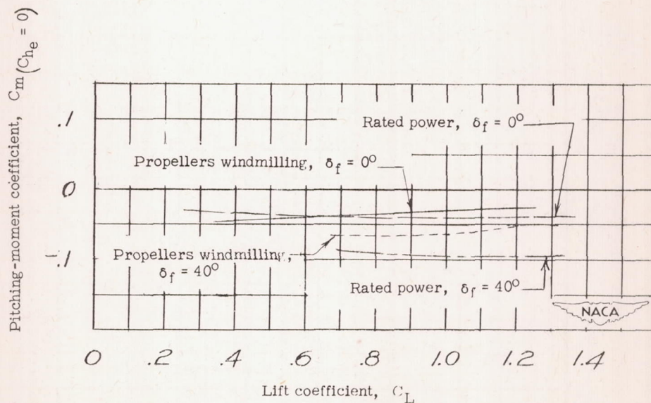
Figure 7.- Effect of power and flap deflection on the variation of C_m with C_L . Stick free; center of gravity at 0.23 mean aerodynamic chord; i_t = 1.4^\circ ; \delta_a = 0^\circ ; \delta_r = 0^\circ .
