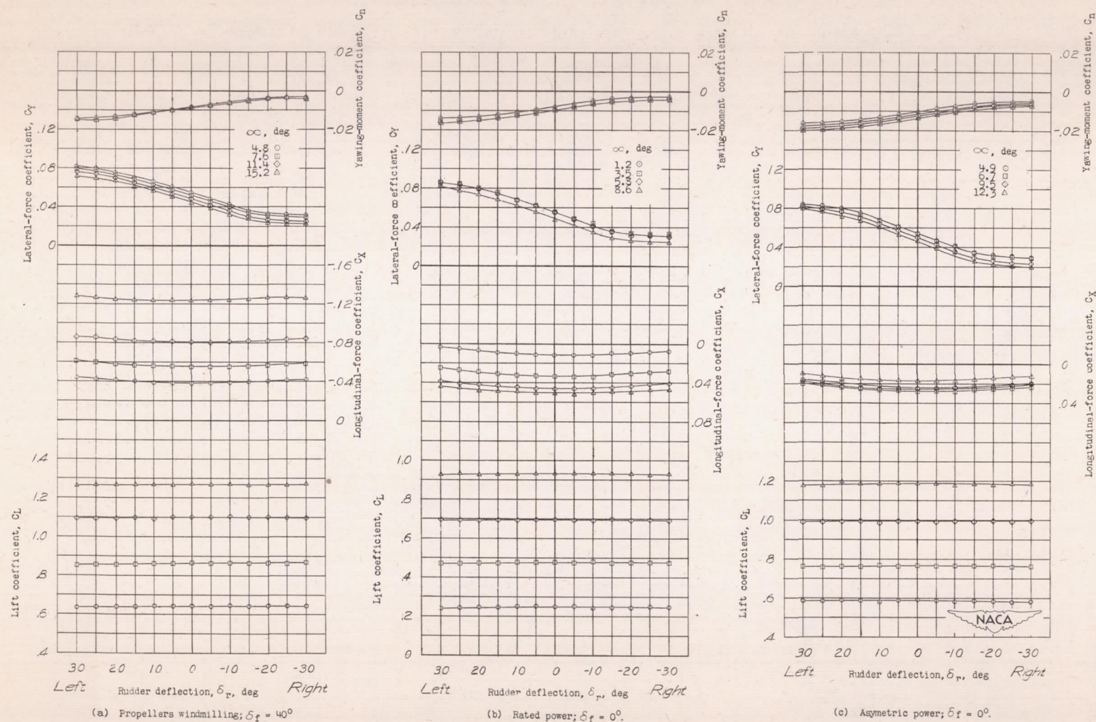
Figure 33.- Effect of angle of attack, power, and flap deflection on the variation of C_L , C_X , C_Y , and C_N with \delta_r . \psi = 15^\circ ; i_t = 5.4^\circ ; \delta_a = 0^\circ ; \delta_e = 0^\circ .
