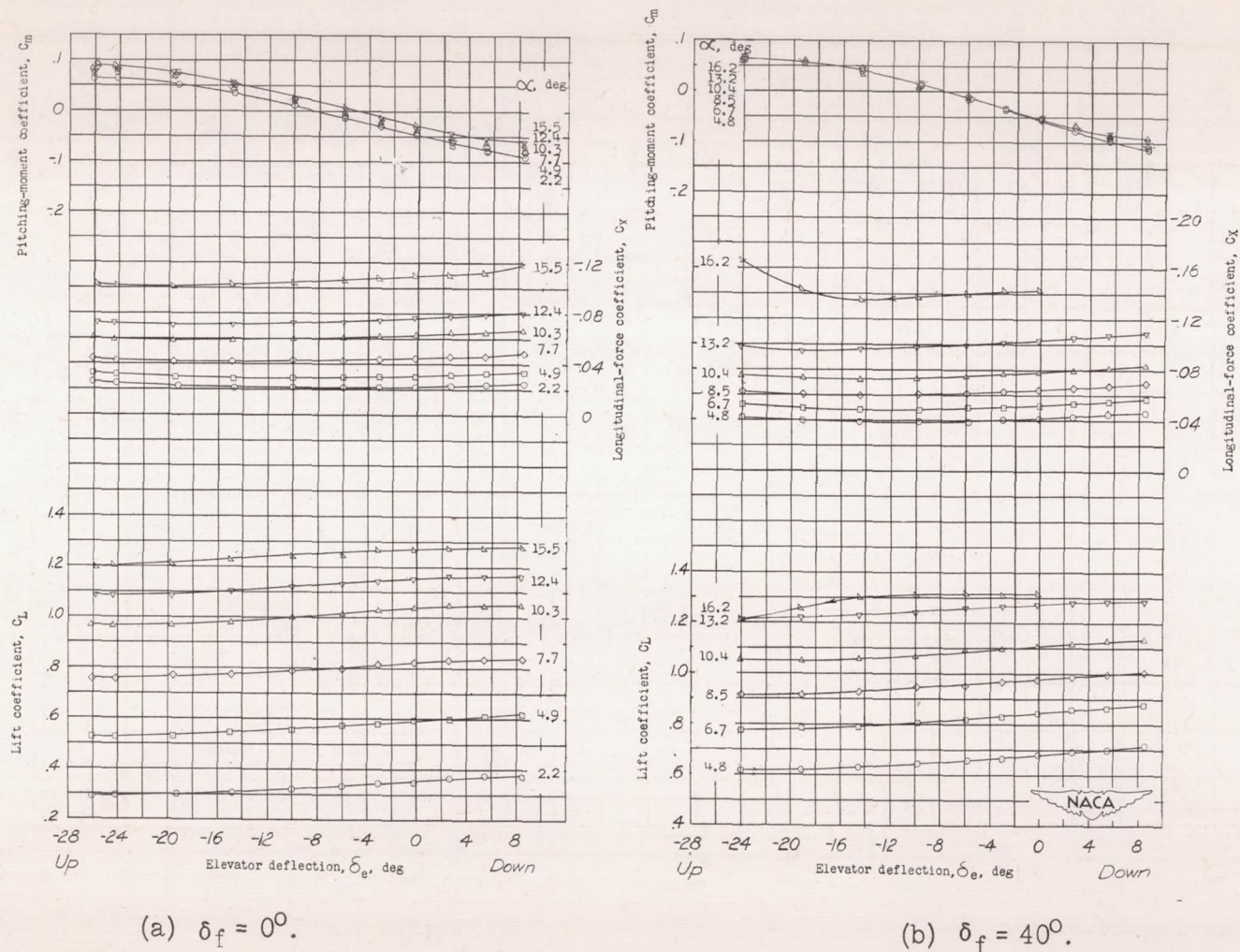
Figure 21.- Effect of \alpha and \delta_f on the variation of C_L , C_X , and C_m with \delta_e . Propellers windmilling; \psi = 0^\circ ; i_t = 5.4^\circ ; \delta_a = 0^\circ ; \delta_r = 0^\circ .
