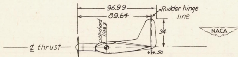
(b) All-wing model.
