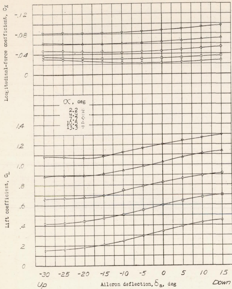
Figure 29.- Effect of \alpha and \delta_f on the variation of C_L , C_X , C_l , and C_n with \delta_a . Propellers windmilling; \psi = 0^\circ ; i_t = 5.4^\circ ; \delta_e = 0^\circ ; \delta_r = 0^\circ .
