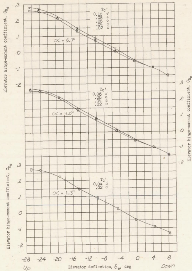
Figure 26.- Effect of \alpha , T_c' , and \delta_f on the variation of C_{he} with \delta_e . \psi = 0^\circ ; i_t = 5.4^\circ ; \delta_a = 0^\circ ; \delta_r = 0^\circ .
