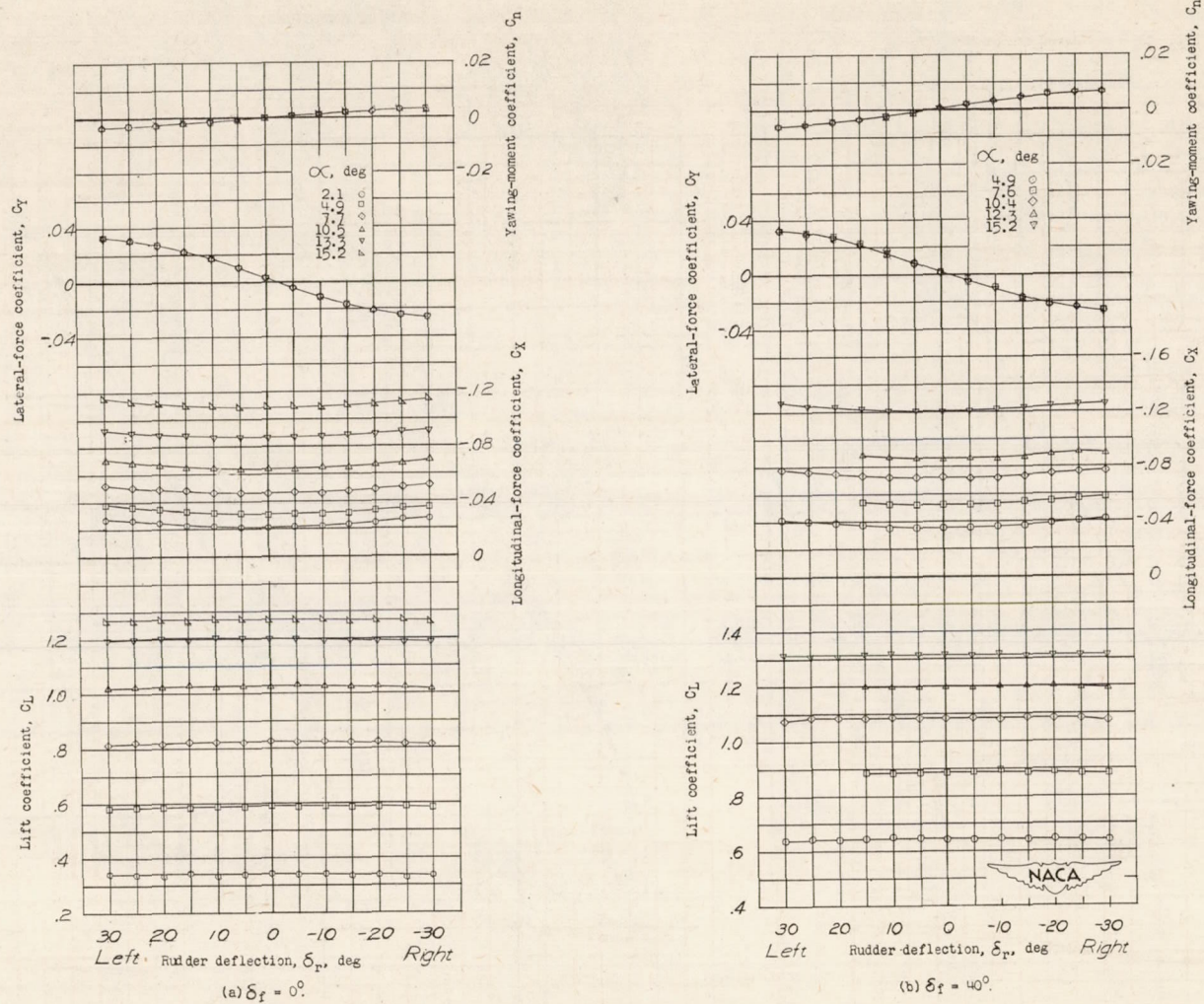
Figure 27.- Effect of \alpha and \delta_f on the variation of C_L , C_X , C_Y , and C_N with \delta_r . Propellers windmilling; \psi = 0^\circ ; i_t = 5.4^\circ ; \delta_a = 0^\circ ; \delta_e = 0^\circ .
