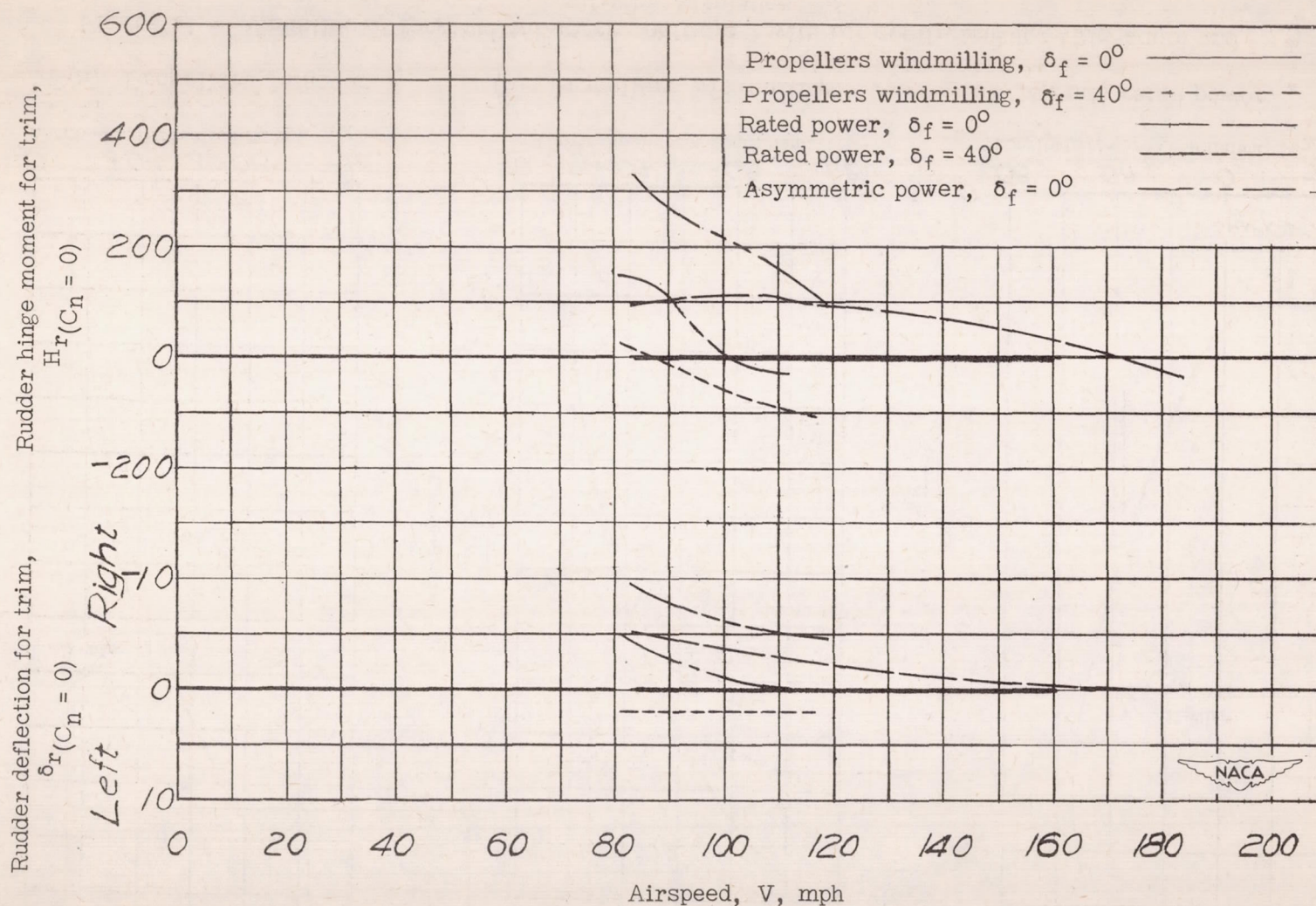
Figure 13.- Effect of power and flap deflection on the variation of rudder deflection and rudder hinge moment for trim with airspeed. Sea level; \psi = 0^\circ ; \delta_a = 0^\circ ; \delta_e = 0^\circ .
