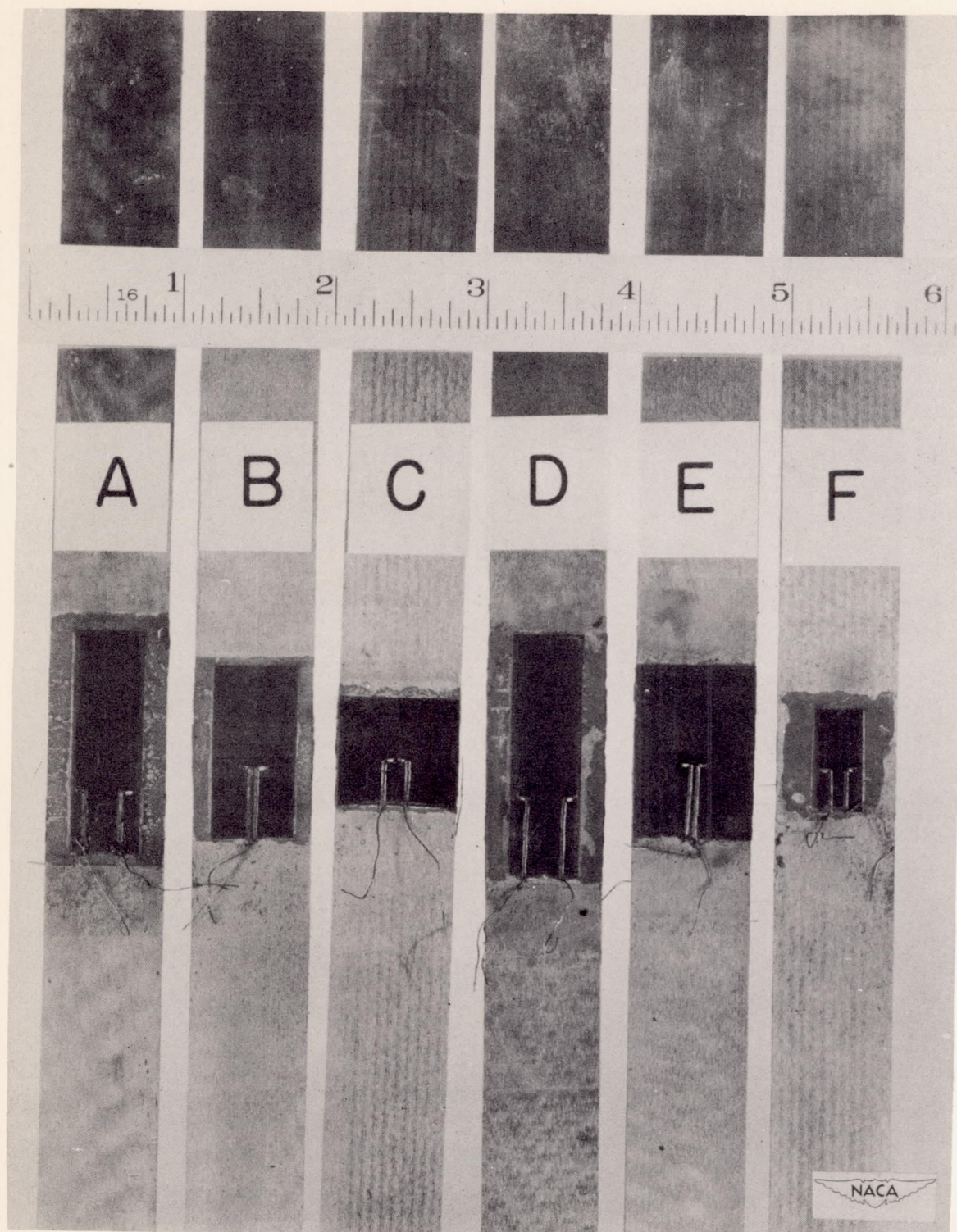
Figure 1.- Gages attached to test strips for calibration.
