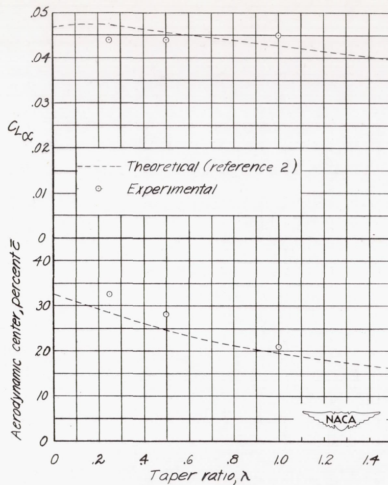
Figure 6.- Comparison of theoretical and experimental variations of C_L \alpha and position of aerodynamic center with taper ratio for wings tested. C_L < 0.6 .
