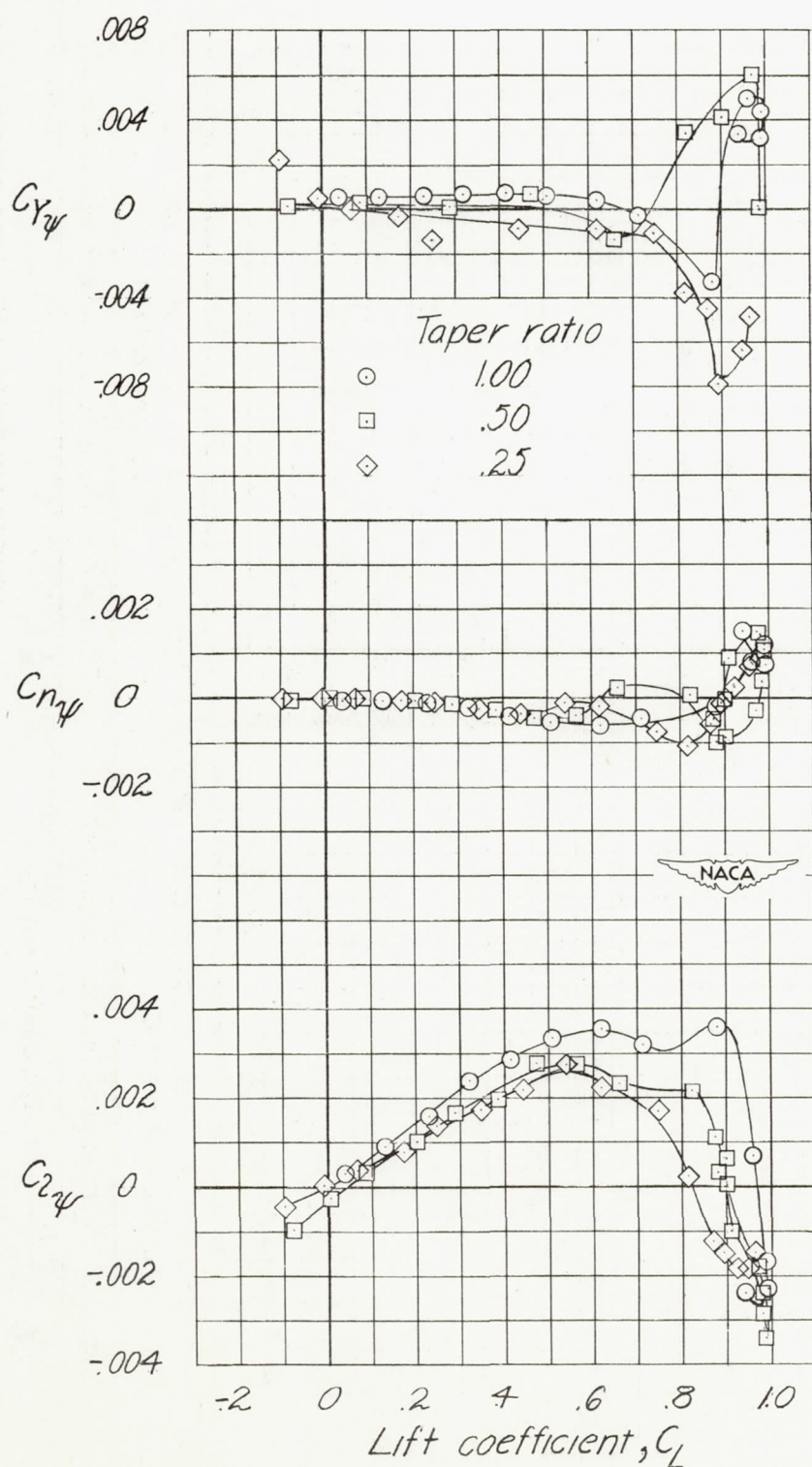
Figure 7.- Variation of C_{Y\psi} , C_{n\psi} , and C_{l\psi} with lift coefficient for wings tested.
