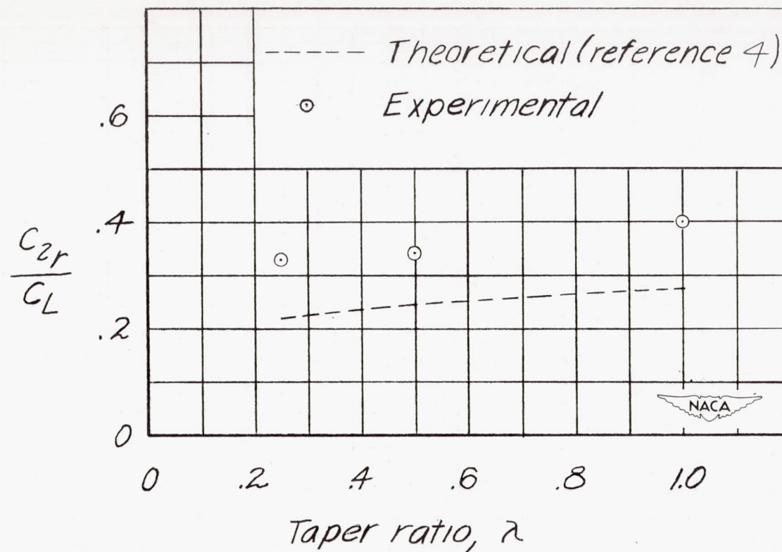
Figure 10.- Comparison of theoretical and experimental variation of C_{lr}/C_L with taper ratio for wings tested. \psi = 0^\circ ; C_L < 0.6 .
