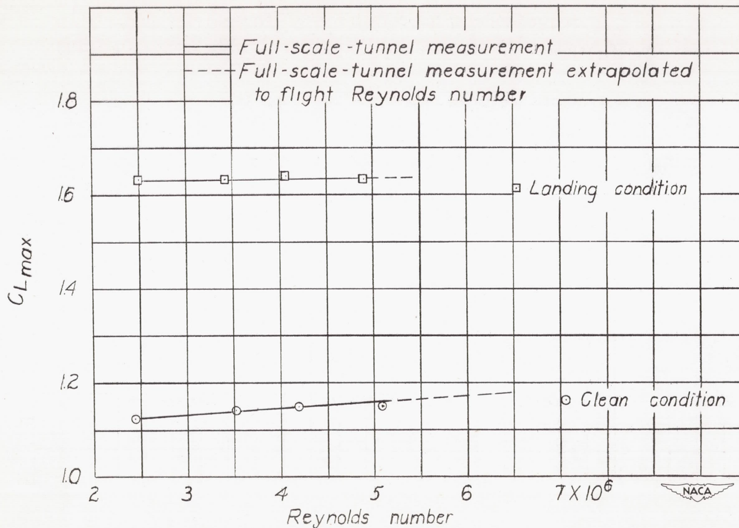
Figure 3.- Effect of Reynolds number on the maximum lift coefficient of the fighter-type airplane. Propeller removed; \bar{c} \frac{da}{dt} = 0 .
