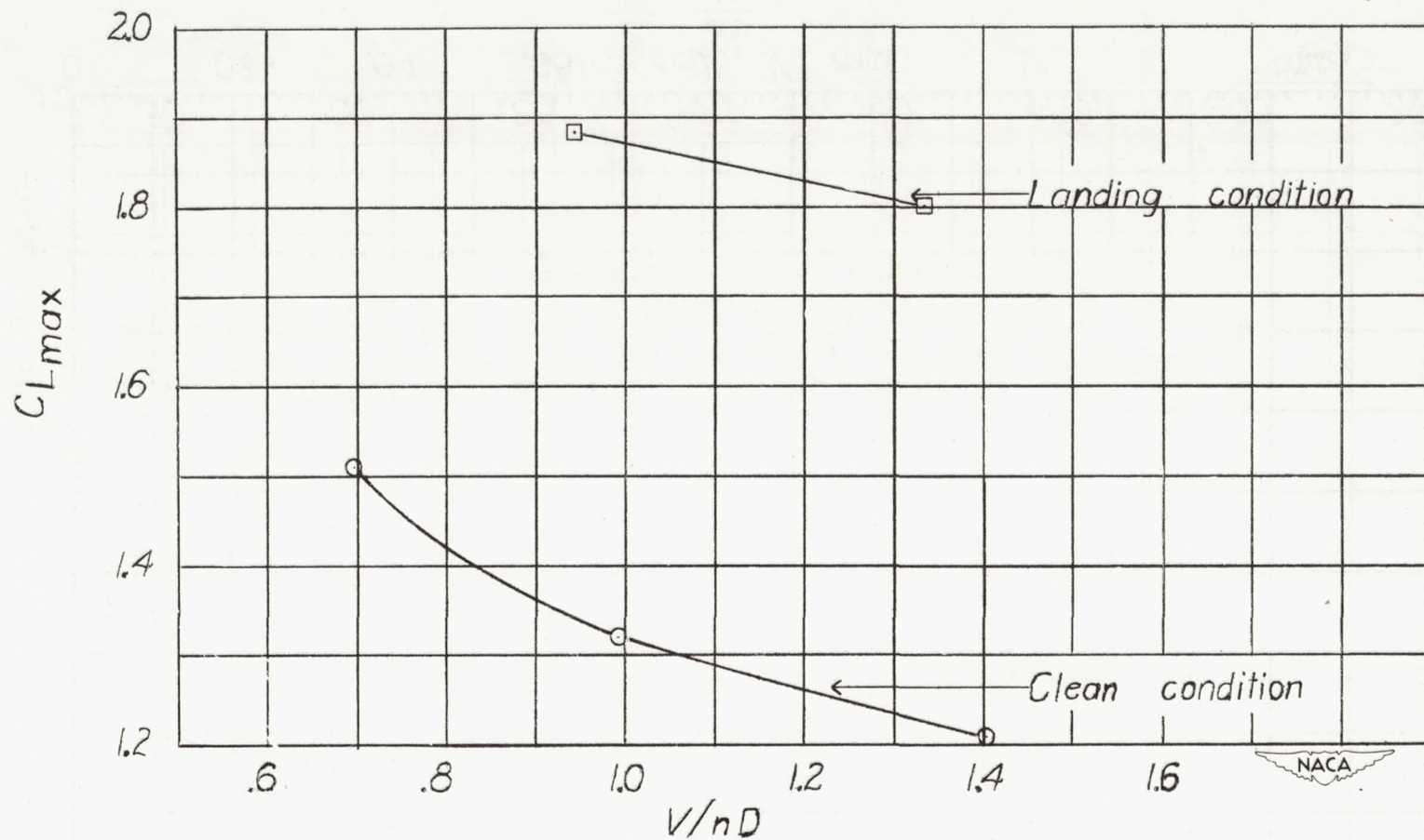
Figure 10.- Effect of propeller operation on the maximum lift coefficient. \frac{da}{dt} = 0 .
