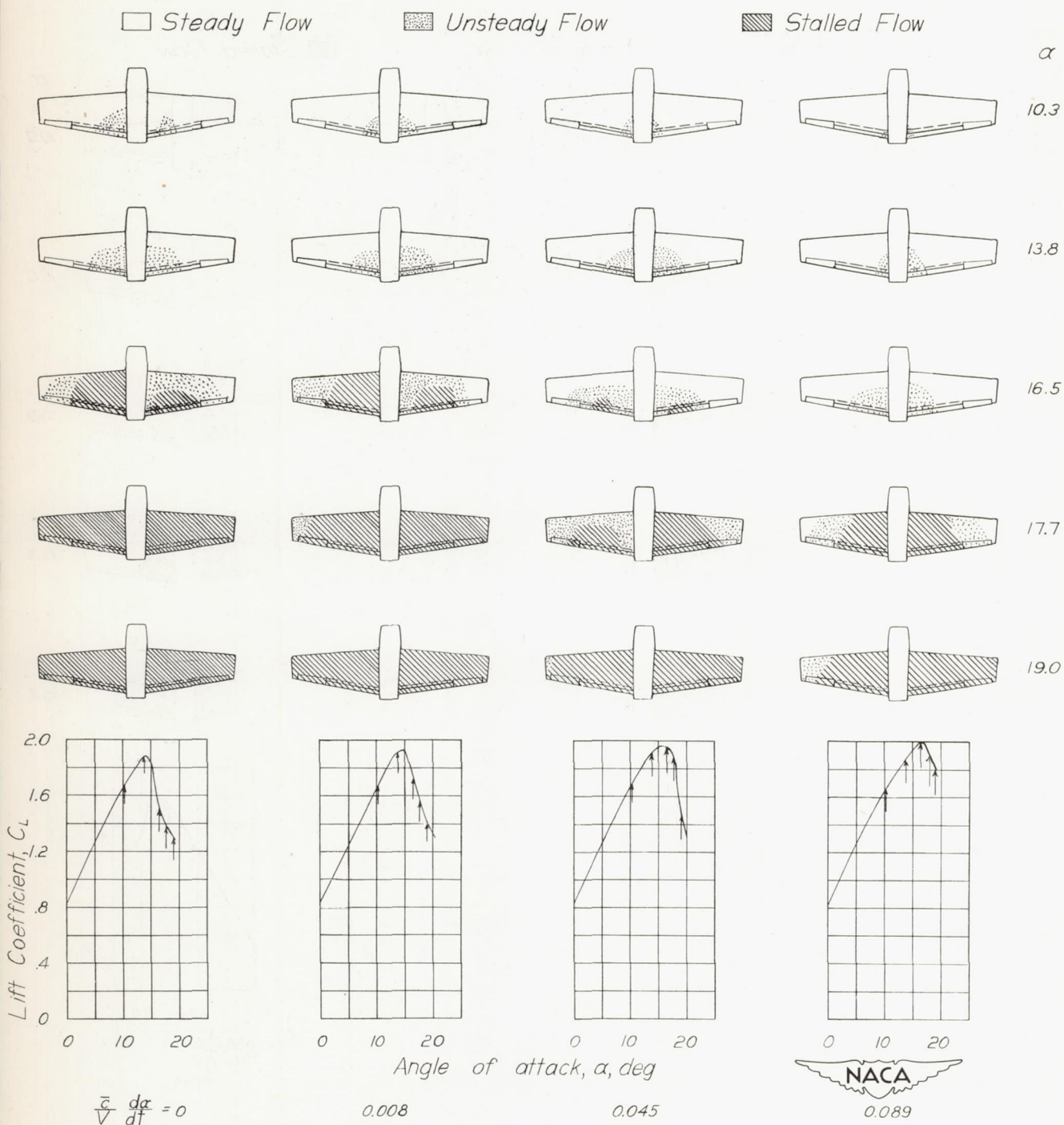
Figure 14.- Effect of time rate of change of angle of attack on the stall progression and maximum lift of the fighter-type airplane. Flaps and landing gear extended; propeller idling; approximate \frac{V}{nD} , 0.97; canopy open; approximate test velocity, 50 miles per hour.
