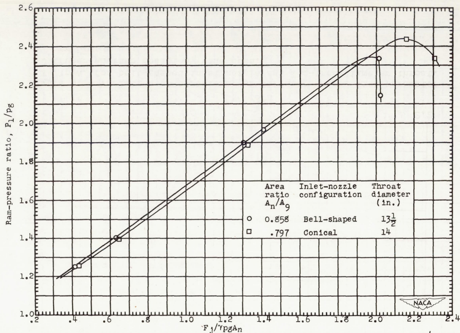
Figure 8. - Comparison of ram-pressure ratio obtained with bell-shaped inlet nozzle and 13\frac{1}{2} -inch-diameter throat with ram-pressure ratio obtained with conical inlet nozzle and 14-inch-diameter throat. Diffuser-shutter position, wide open.
