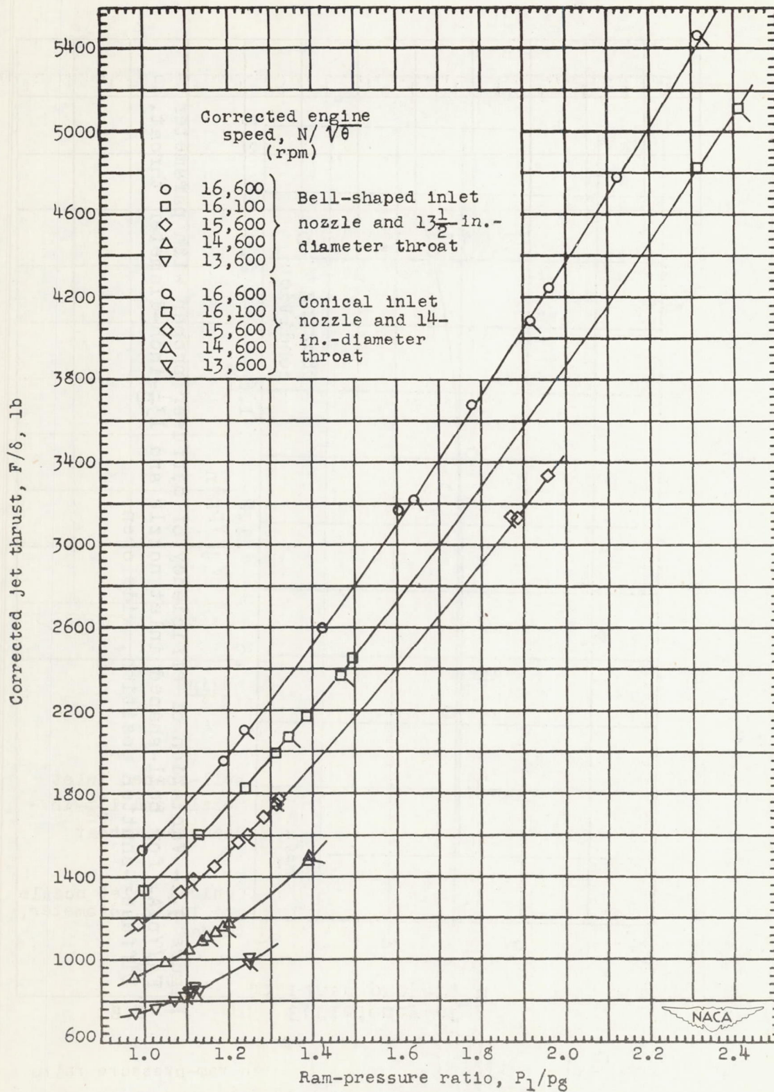
Figure 10. - Variation of corrected jet thrust with ram-pressure ratio for various corrected engine speeds.
