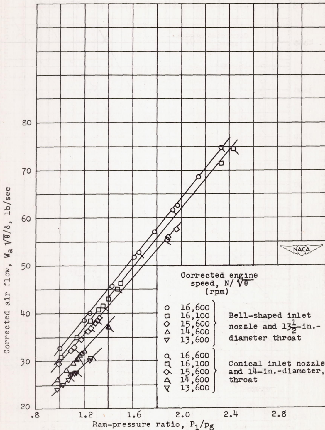
Figure 11. - Variation of corrected air flow with ram-pressure ratio for various corrected engine speeds.
