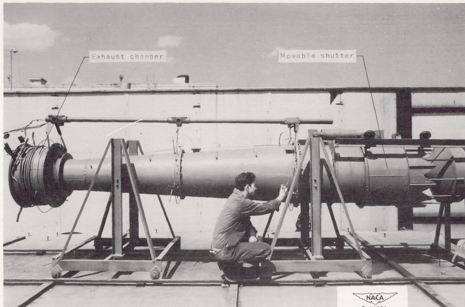
Figure 2. - Jet diffuser mounted on movable frame.
