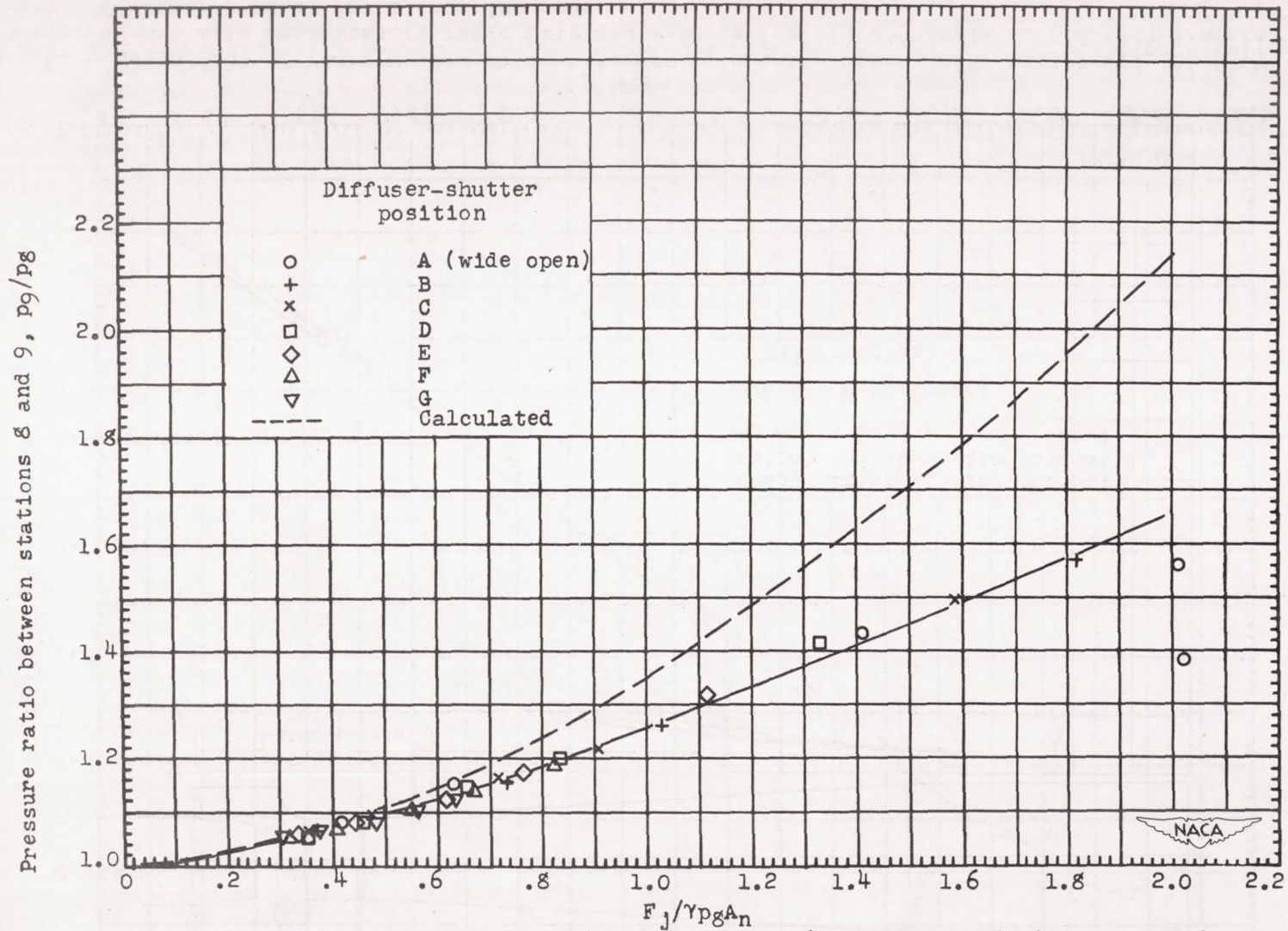
Figure 7. - Comparison of calculated and experimental values of pressure ratio between stations 8 and 9 for bell-shaped inlet nozzle and 13\frac{1}{2} -inch-diameter throat.
