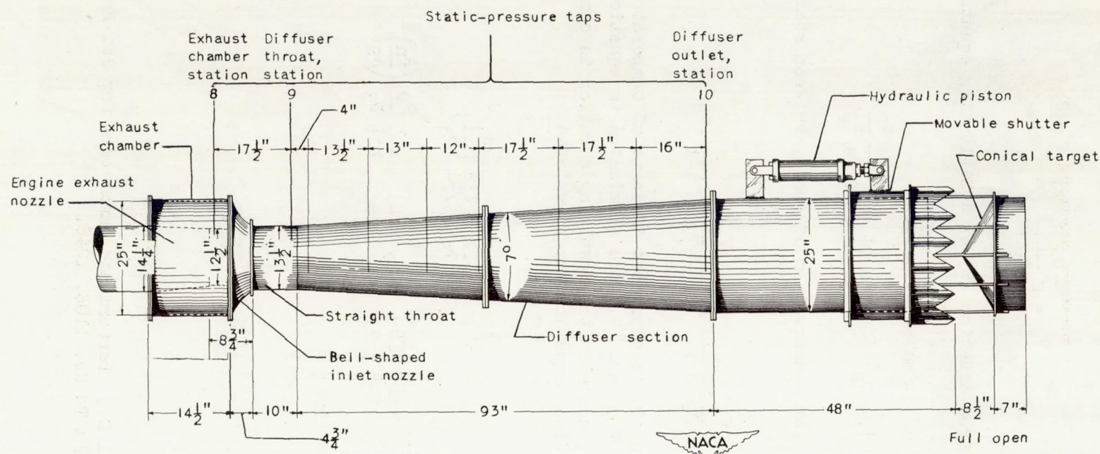
Figure 1. - Diagram of jet-diffuser assembly for turbojet engine with a 12 1/2-inch-diameter exhaust-nozzle outlet showing location of pressure taps. (Additional static-pressure taps in exhaust chamber, inlet nozzle, and throat are shown in fig. 3).
