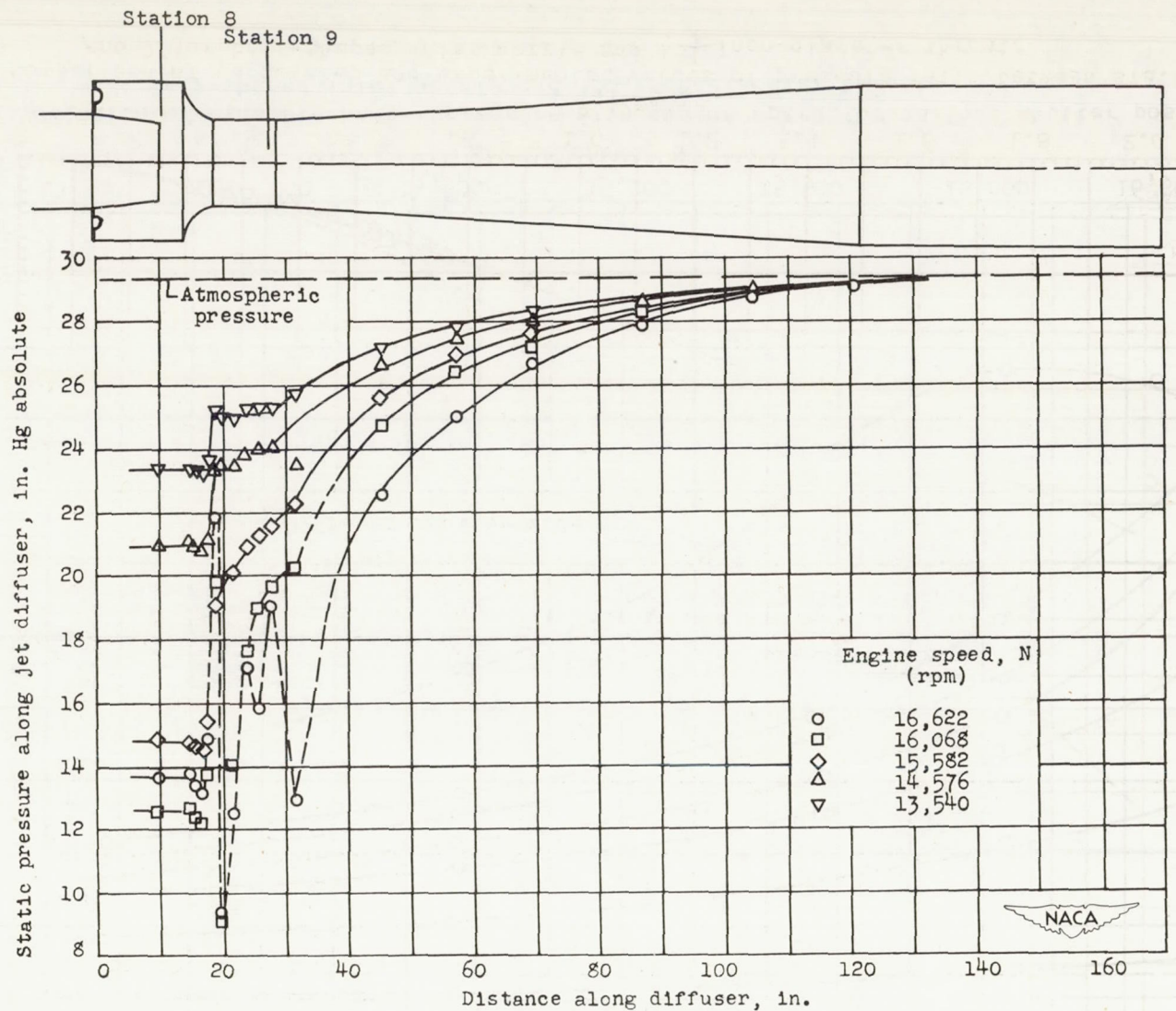
Figure 6. - Variation of static pressures along jet diffuser for wide-open shutter position. Bell-shaped inlet nozzle and 1\frac{1}{2} -inch-diameter throat.
