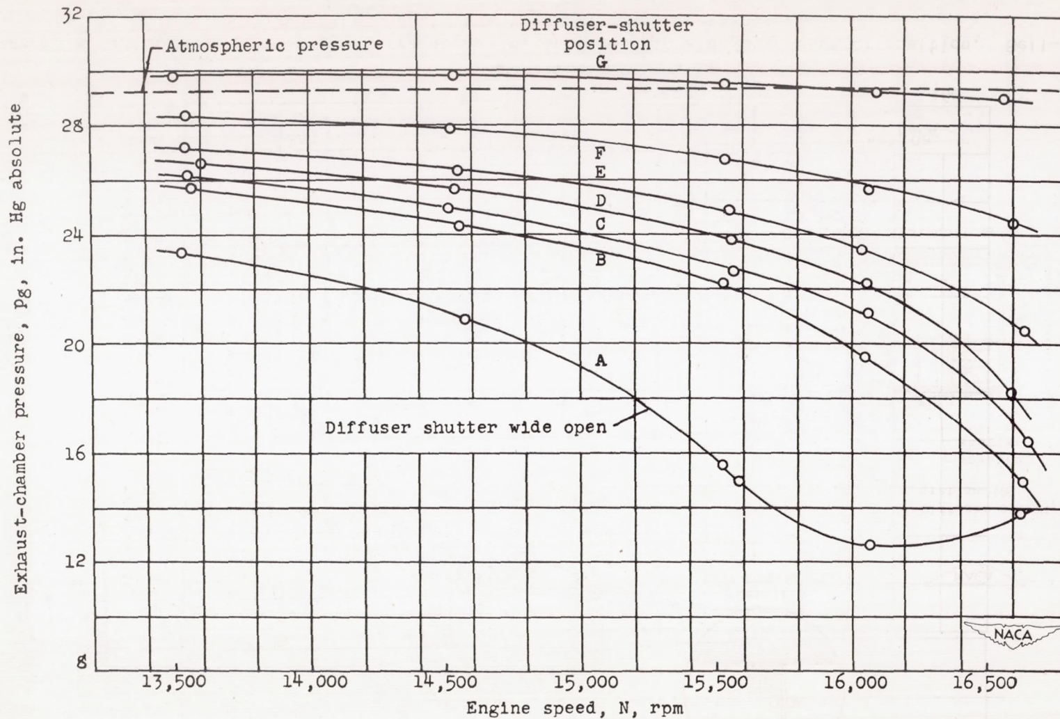
Figure 5. - Variation of exhaust-chamber pressure with engine speed for various shutter positions. Bell-shaped inlet nozzle and 13\frac{1}{2} -inch-diameter throat.
