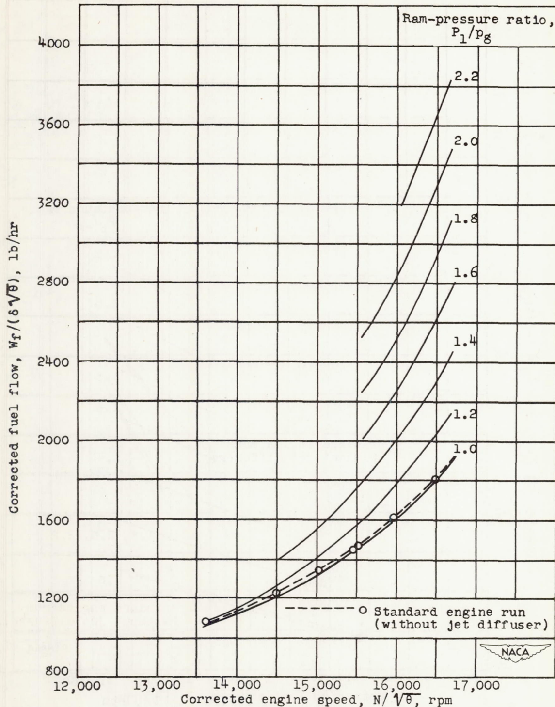
Figure 16. - Variation of corrected fuel flow with corrected engine speed for various ram-pressure ratios.
