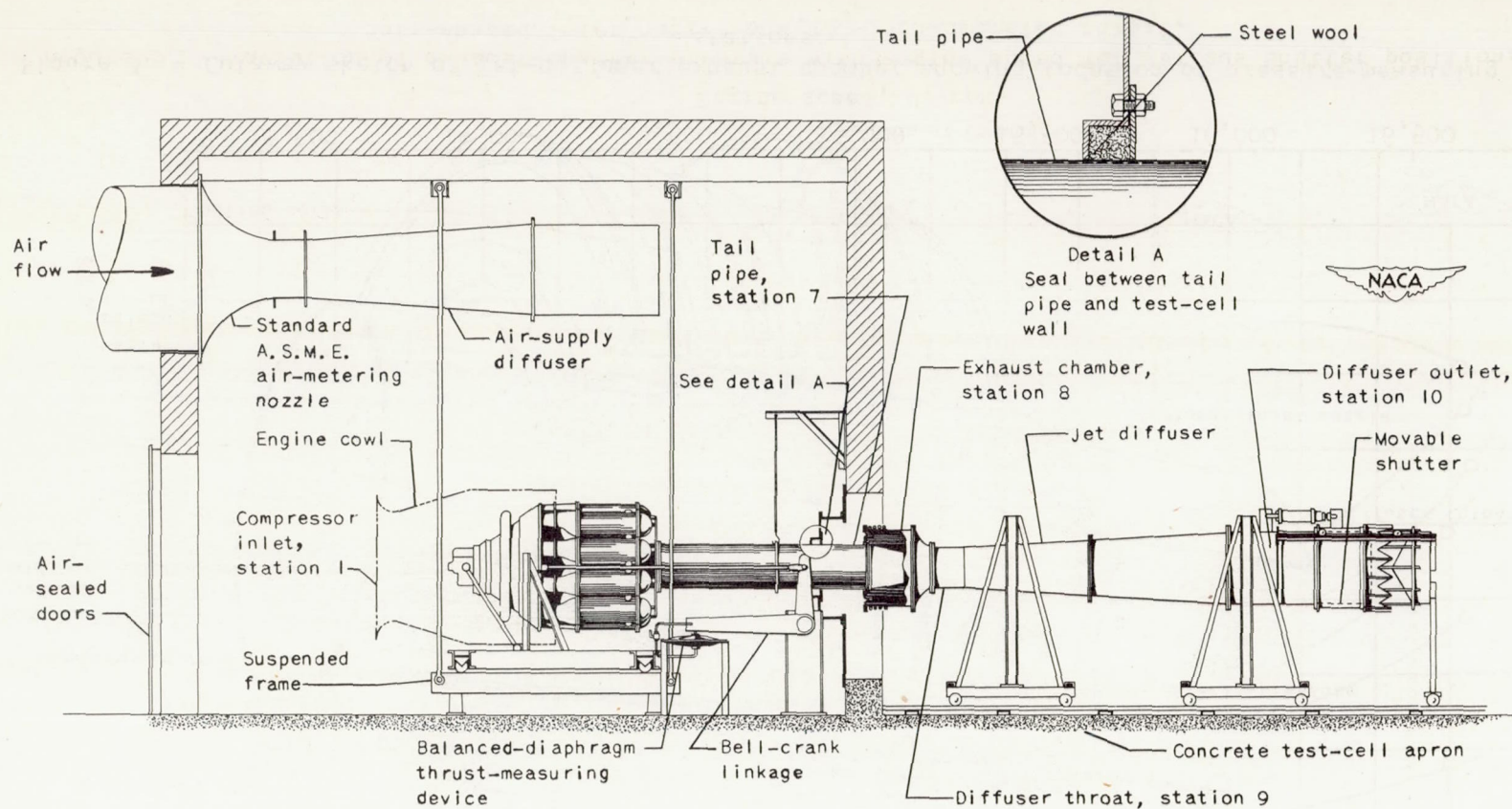
Figure 4. - Schematic diagram of apparatus for jet-diffuser investigation.
