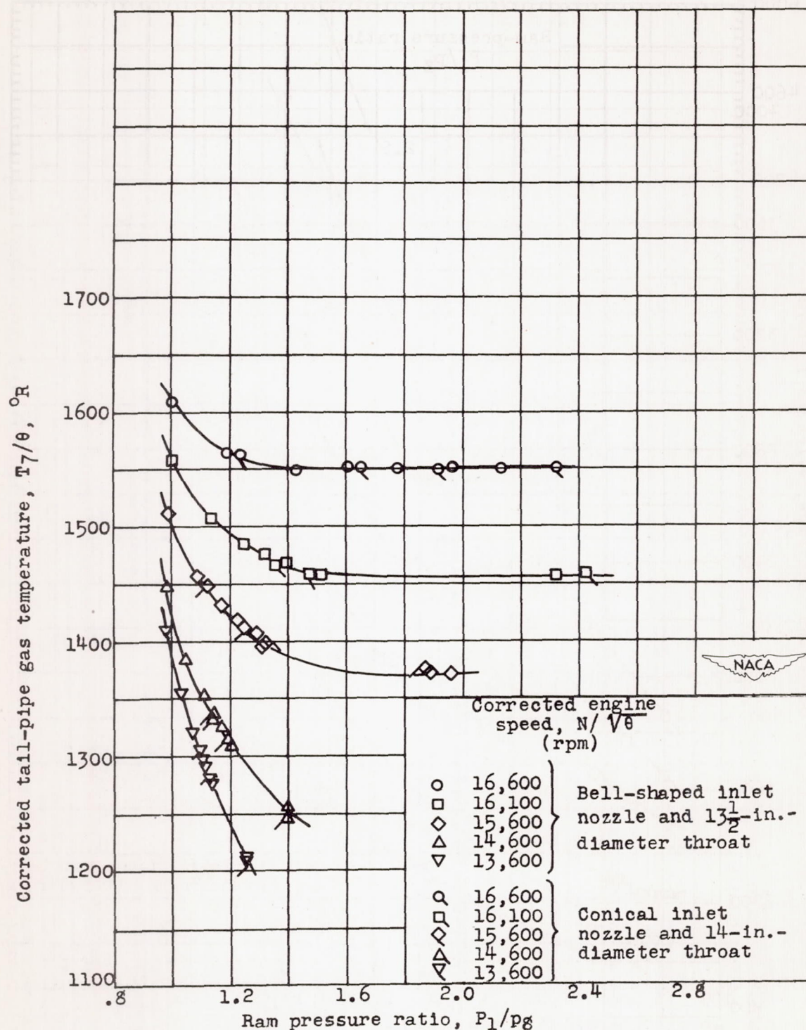
Figure 13. - Variation of corrected tail-pipe gas temperature with ram-pressure ratio for various corrected engine speeds.
