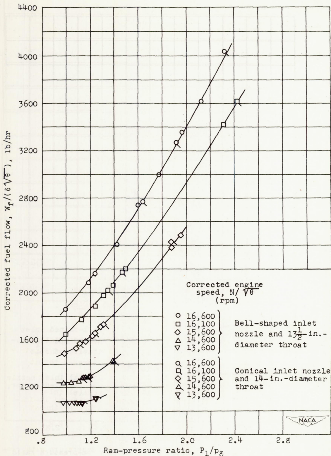
Figure 12. - Variation of corrected fuel flow with ram-pressure ratio for various corrected engine speeds.
