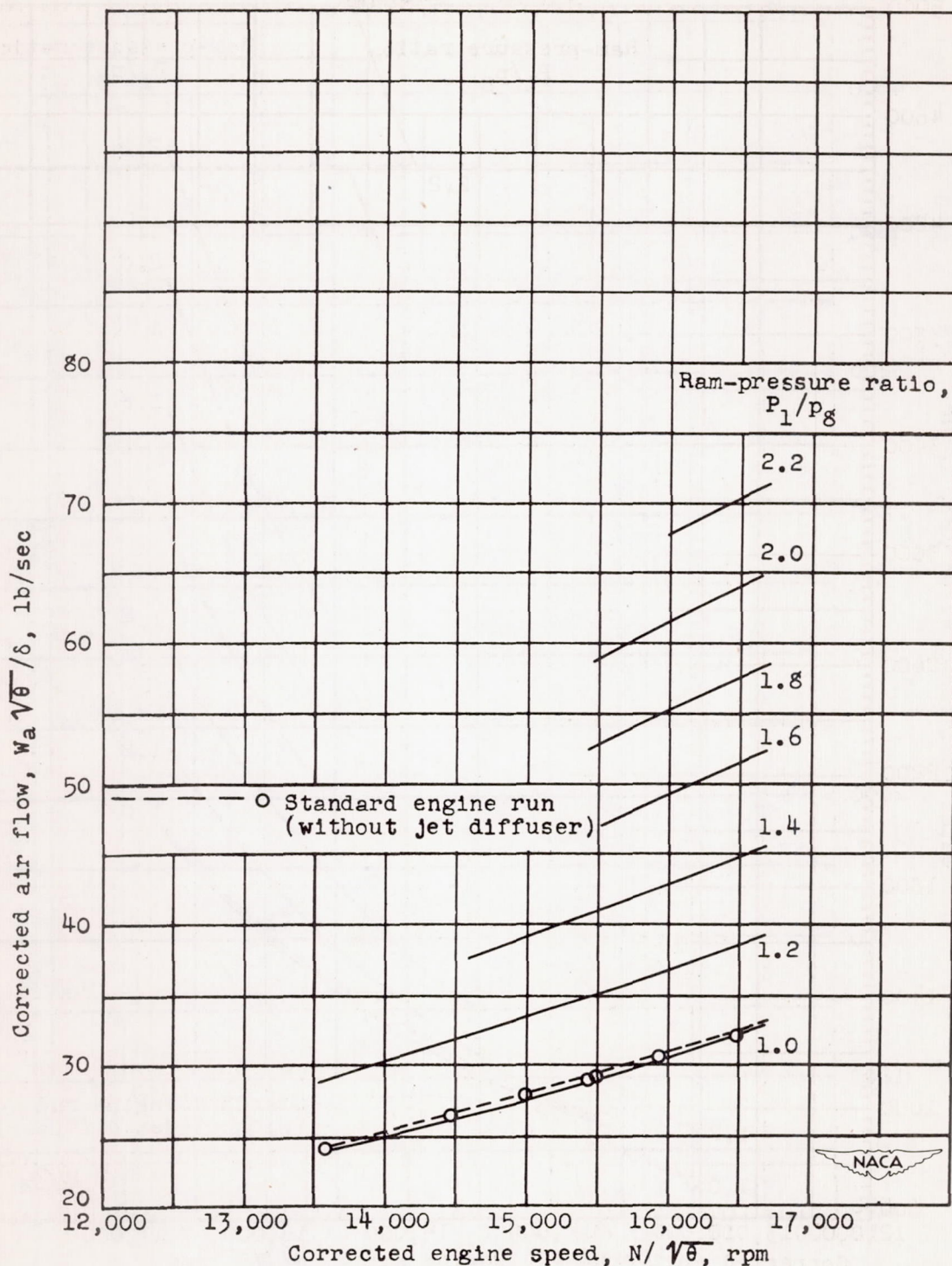
Figure 15. - Variation of corrected air flow with corrected engine speed for various ram-pressure ratios.
