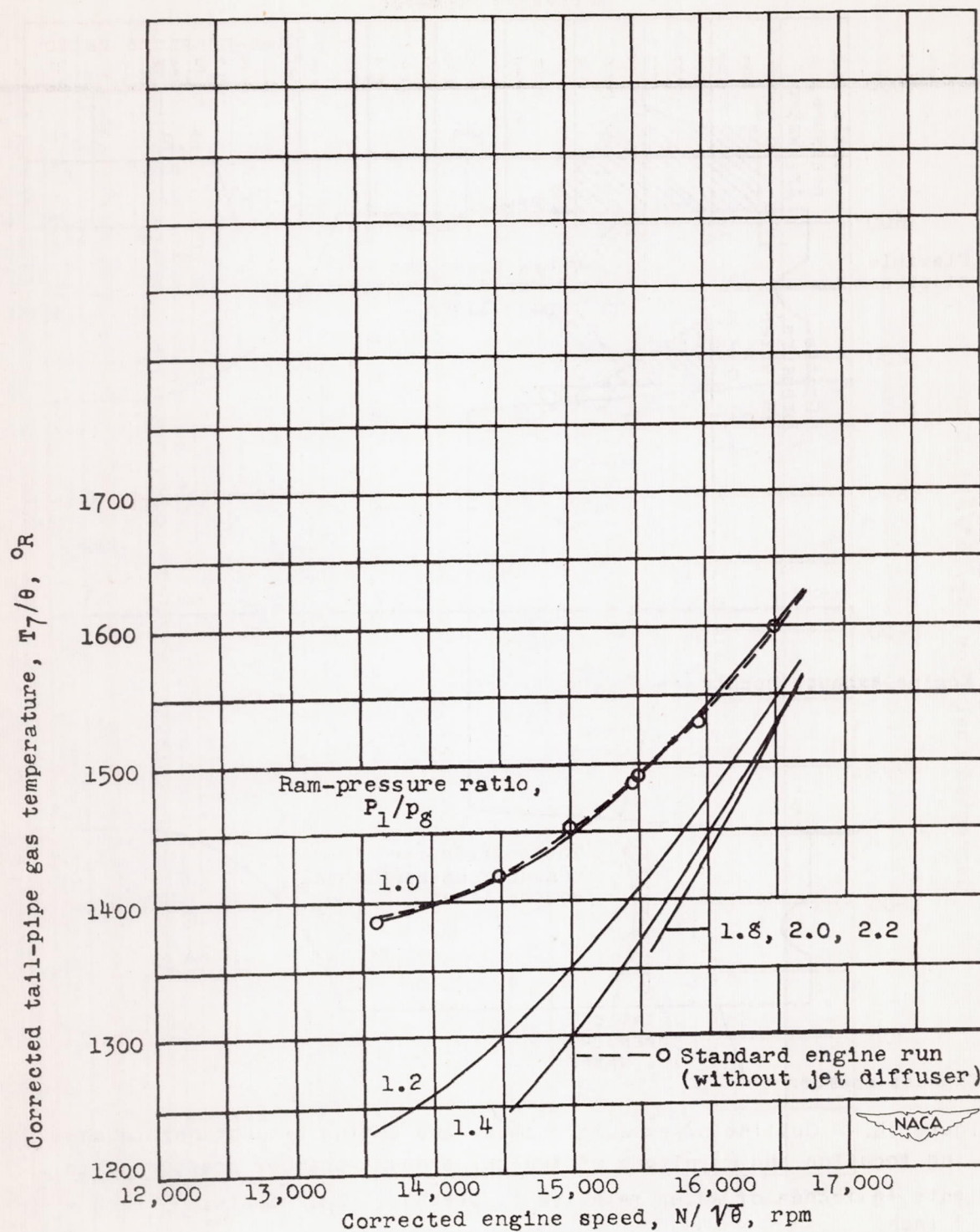
Figure 17. - Variation of corrected tail-pipe gas temperature with corrected engine speed for various ram-pressure ratios.
