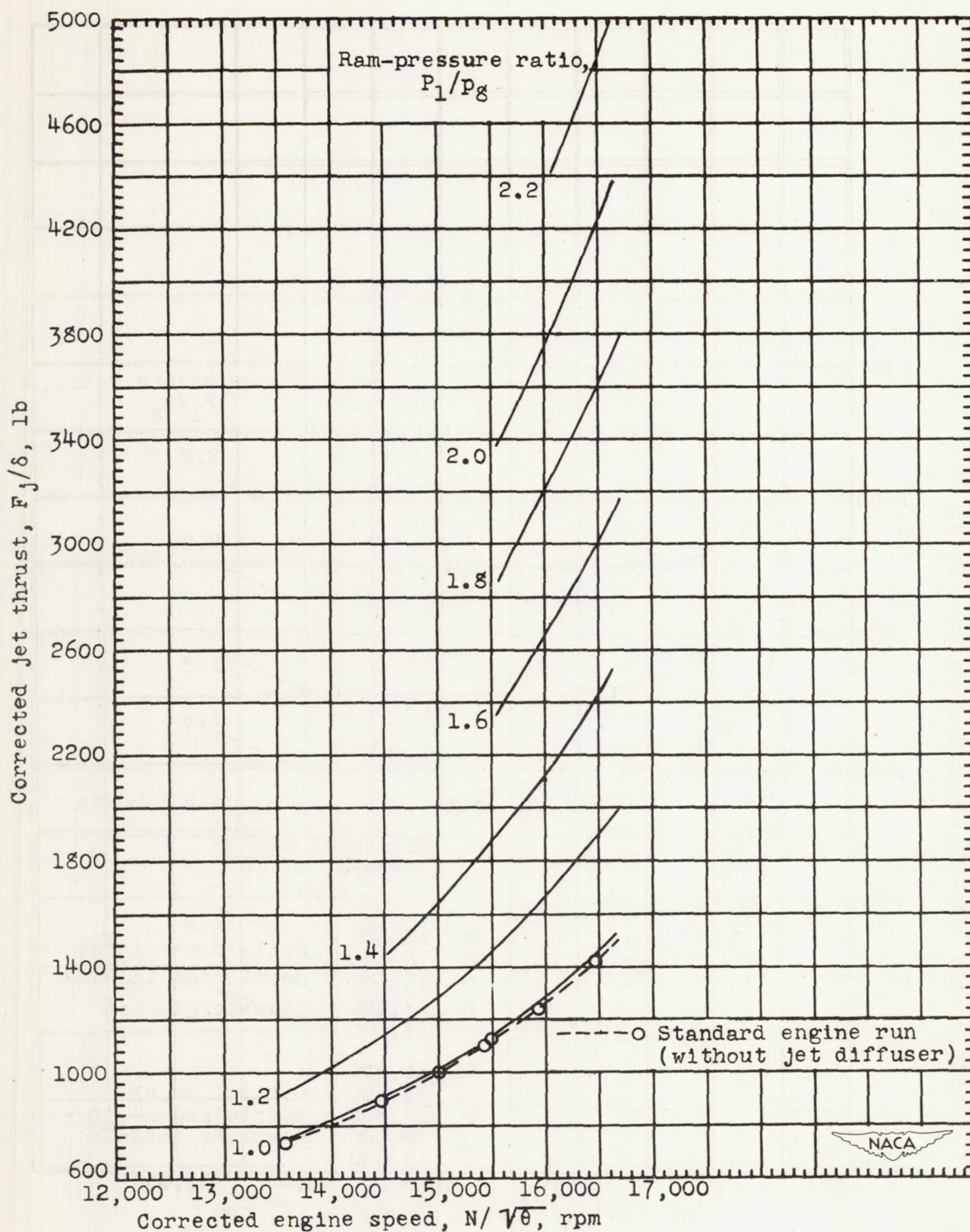
Figure 14. - Variation of corrected jet thrust with corrected engine speed for various ram-pressure ratios.
