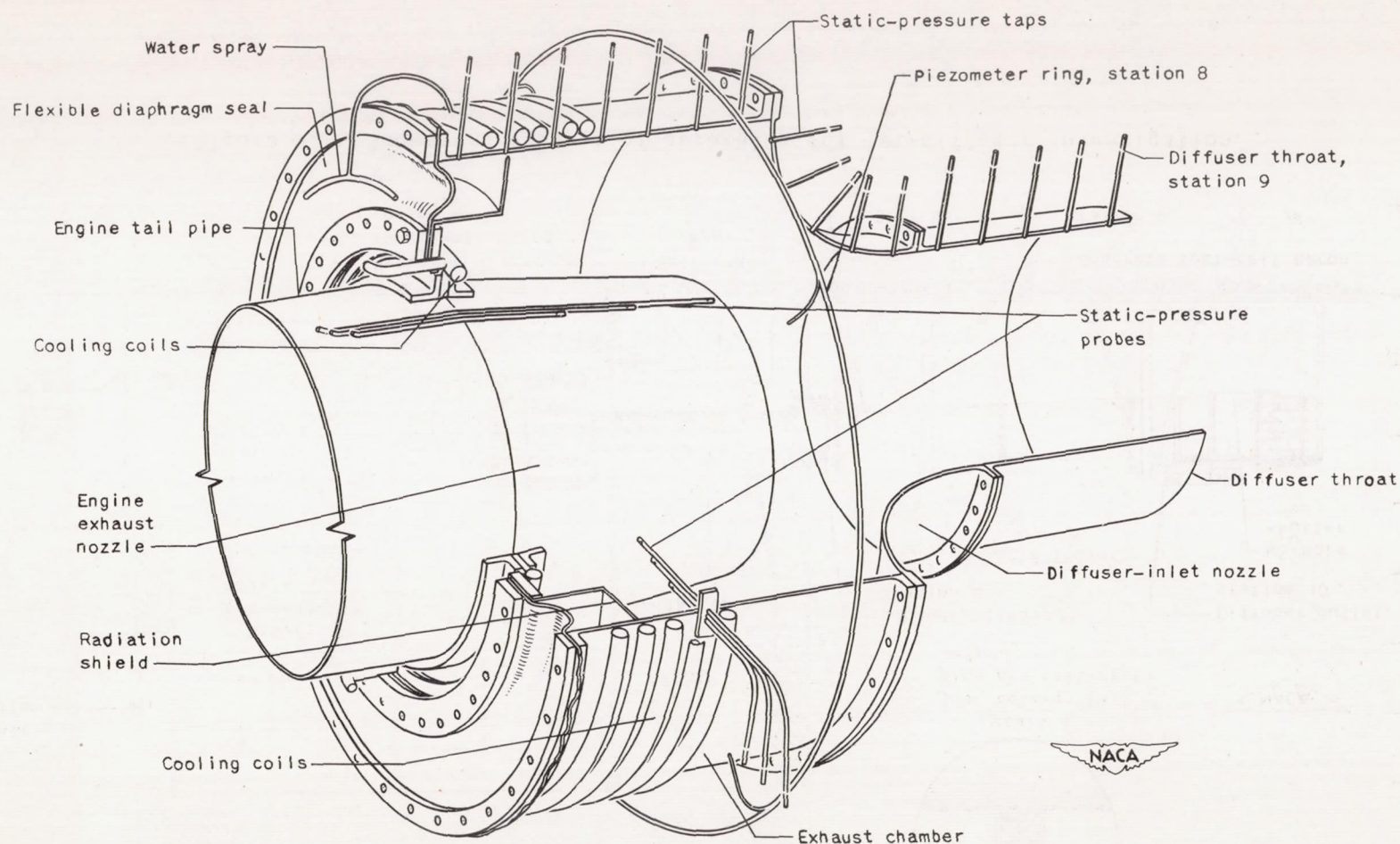
Figure 3. - Cutaway sketch of jet-diffuser exhaust chamber showing location of pressure-measuring stations.
