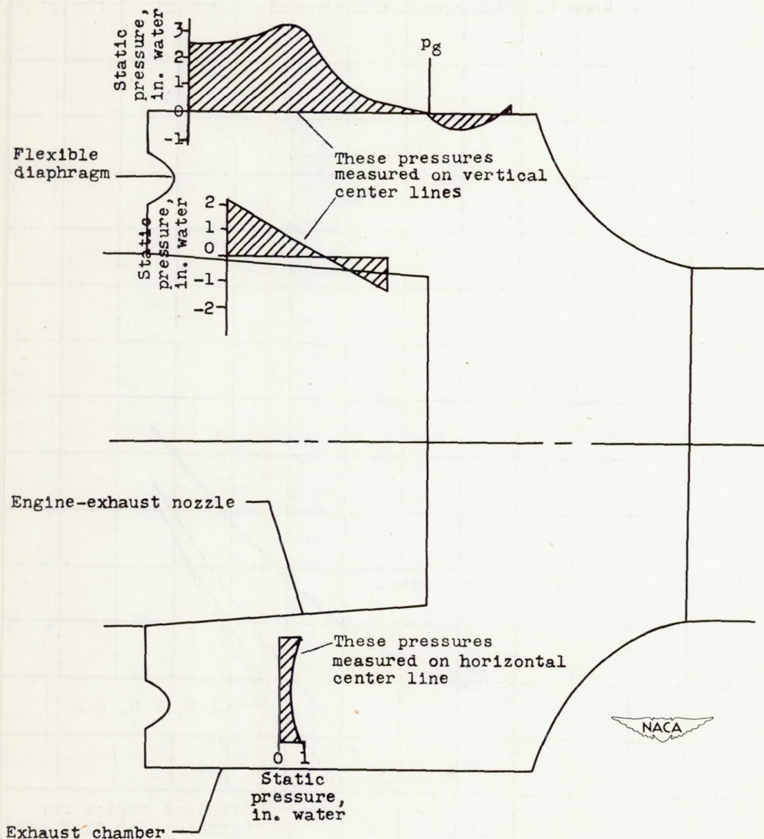
Figure 18. - Outline of exhaust chamber and engine exhaust nozzle showing location and magnitude of typical exhaust-chamber pressure gradients in inches of water relative to pressure p_g . Scale: \frac{1}{4} inch = 1 inch.
