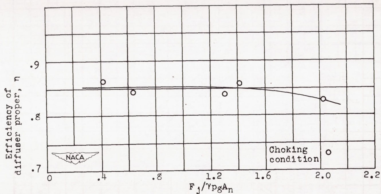
Figure 9. - Variation of efficiency of diffuser proper with parameter F_j/\gamma p g A_n for bell-shaped inlet nozzle and 1\frac{1}{2} -inch-diameter throat. Diffuser-shutter position, wide open.
