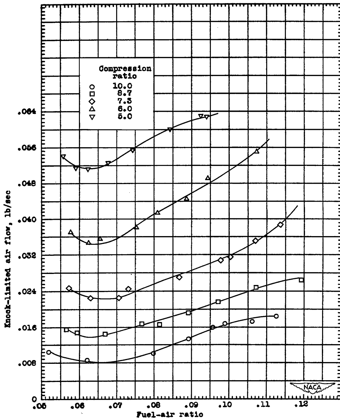
(a) 2,2,3,3-Tetramethylpentane.
