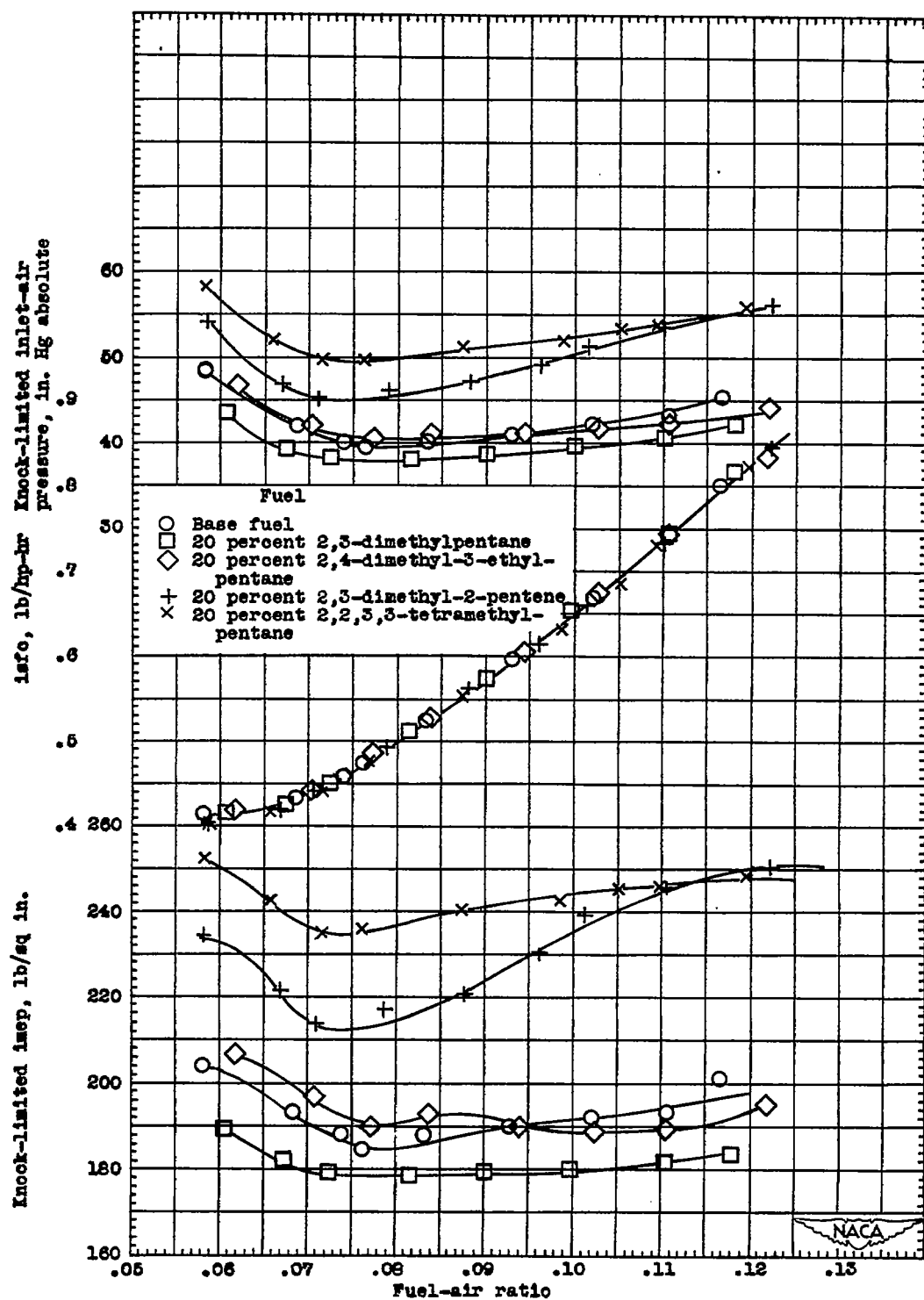
Figure 2. - Knock-limited performance of 20-percent blends of four pure hydrocarbons in 8 reference fuel in 17.6 engine. Compression ratio, 7.0; engine speed, 1800 rpm; spark advance, 30° B.T.C.; coolant temperature, 212° F.
