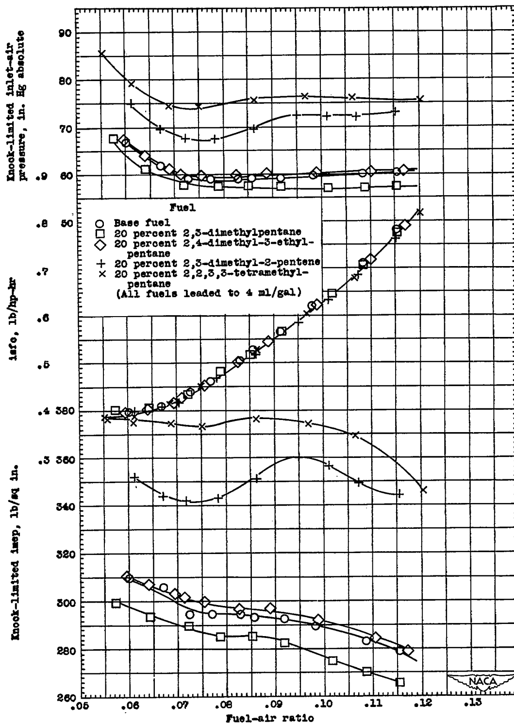
Figure 2. - Continued. Knock-limited performance of 20-percent blends of four pure hydrocarbons in S reference fuel in 17.6 engine. Compression ratio, 7.0; engine speed, 1800 rpm; spark advance, 30° B.T.C.; coolant temperature, 212° F.
