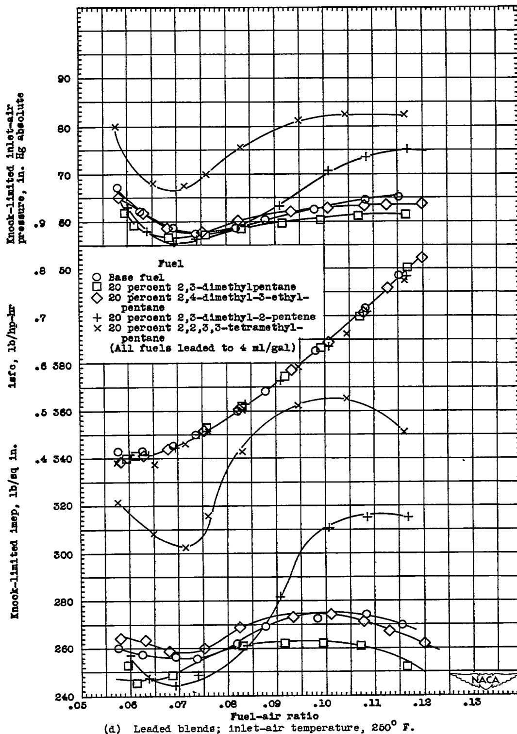
Figure 2. - Concluded. Knock-limited performance of 20-percent blends of four pure hydrocarbons in 8 reference fuel in 17.6 engine. Compression ratio, 7.0; engine speed, 1800 rpm; spark advance, 30° B.T.C.; coolant temperature, 212° F.
