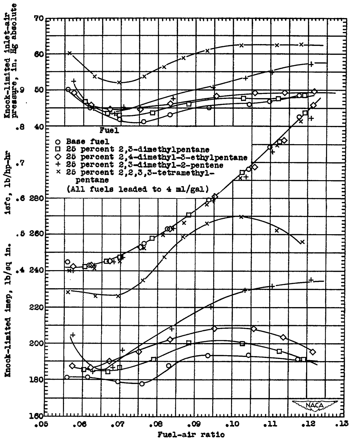
Figure 3. - Knock-limited performance of leaded 25-percent blends of four pure hydrocarbons in a base fuel consisting of 87.5 percent 8 reference fuel plus 12.5 percent n-heptane in 17.6 engine at inlet-air temperature of 250° F. Compression ratio, 7.0; engine speed, 1800 rpm; spark advance, 30° B.T.C.; coolant temperature, 212° F.
