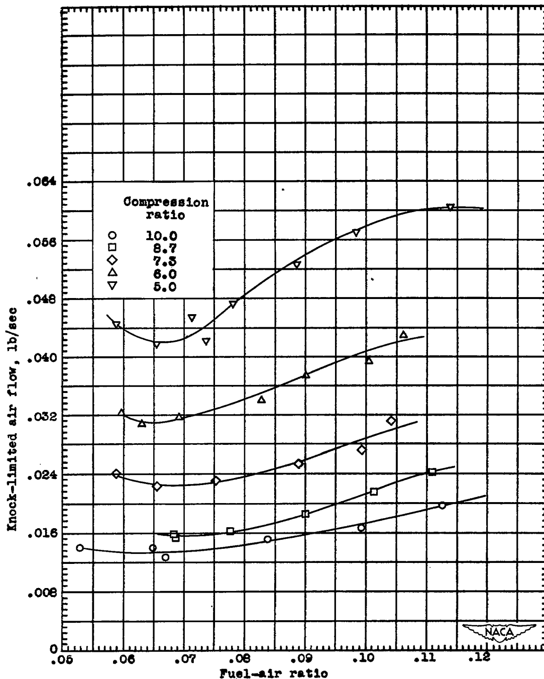
(e) 3,4,4-Trimethyl-2-pentene.
