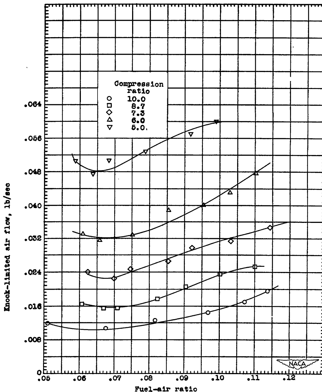
(c) 2,3-Dimethyl-2-pentene.
