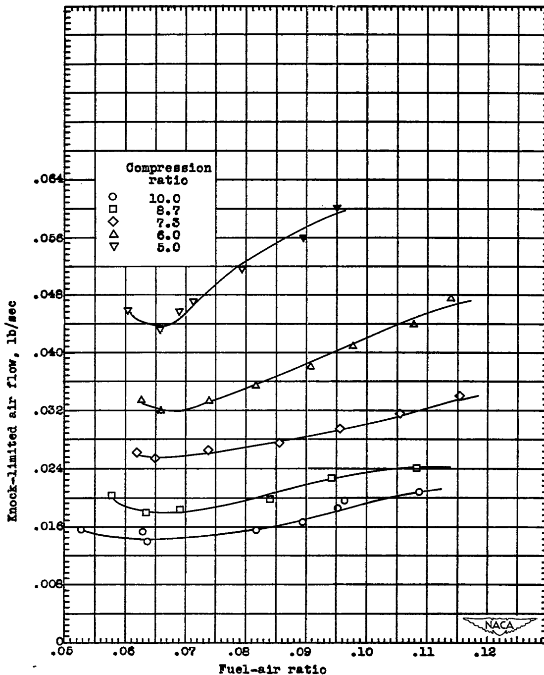
(b) 2,3-Dimethylpentane.
