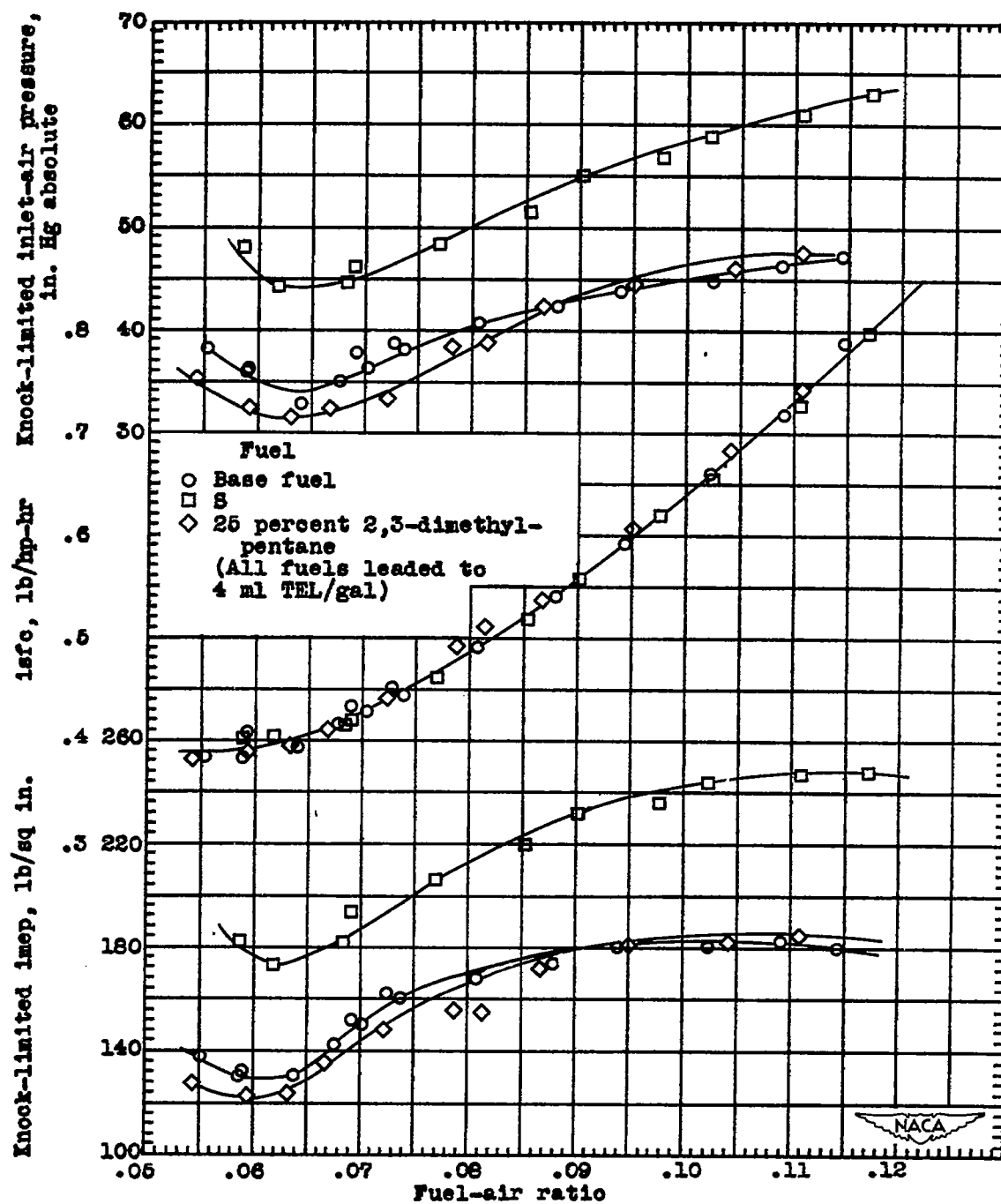
(c) 2,3-Dimethylpentane. Figure 1. - Continued. Knock-limited mixture response of leaded 25-percent blends of hydrocarbons in base fuel consisting of 87.5 percent S plus 12.5 percent n -heptane in F-4 engine.
