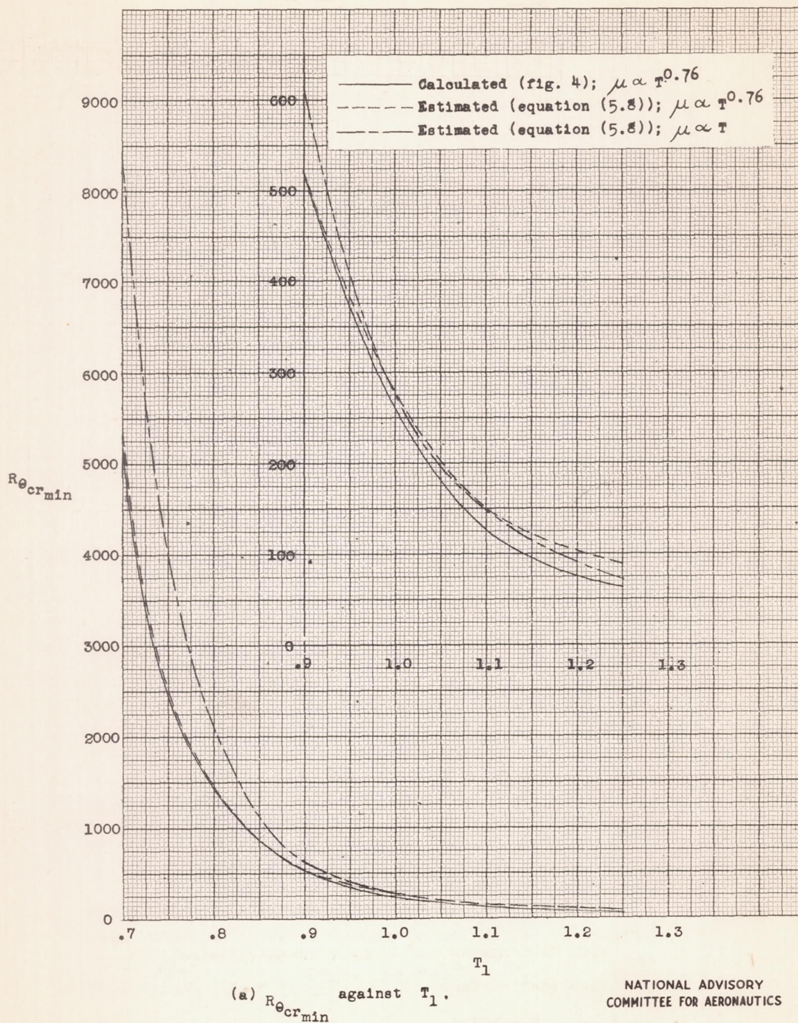
Figure 6.- Dependence of minimum critical Reynolds number on thermal conditions at solid surface. M_o = 0.70 .
