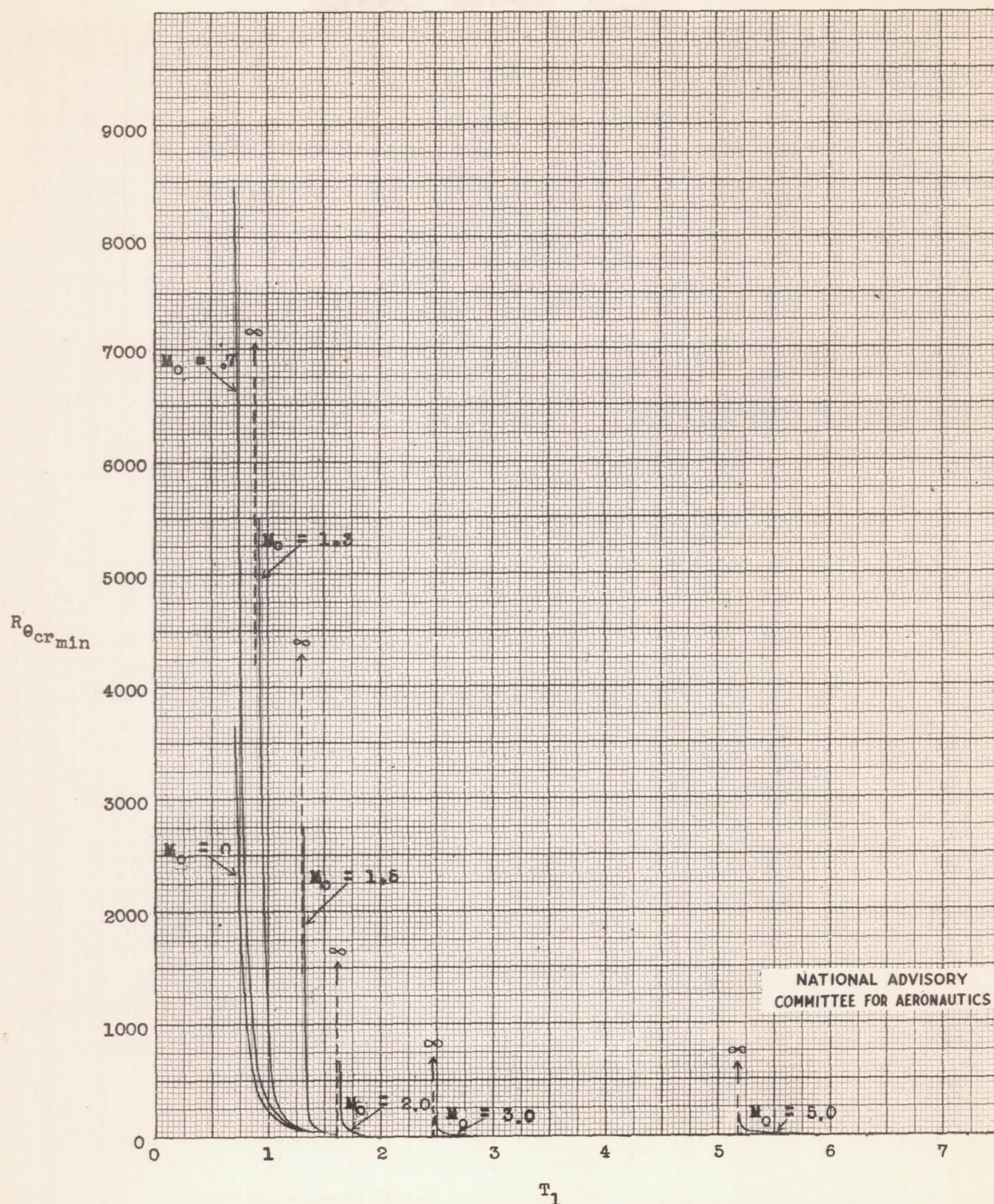
Figure 7.- Stabilizing effect at supersonic Mach numbers of withdrawal of heat from fluid through solid surface. At each value of M_o > 1 , there is a critical value of T_1 = T_{1cr} such that for T_1 \leq T_{1cr} the laminar boundary-layer flow is stable at all values of the Reynolds number. (Curves for M_o = 0 and M_o = 0.70 included for comparison.) Re_{crmin} estimated from equation (5.8). \mu \propto T ; \sigma = 1 .
