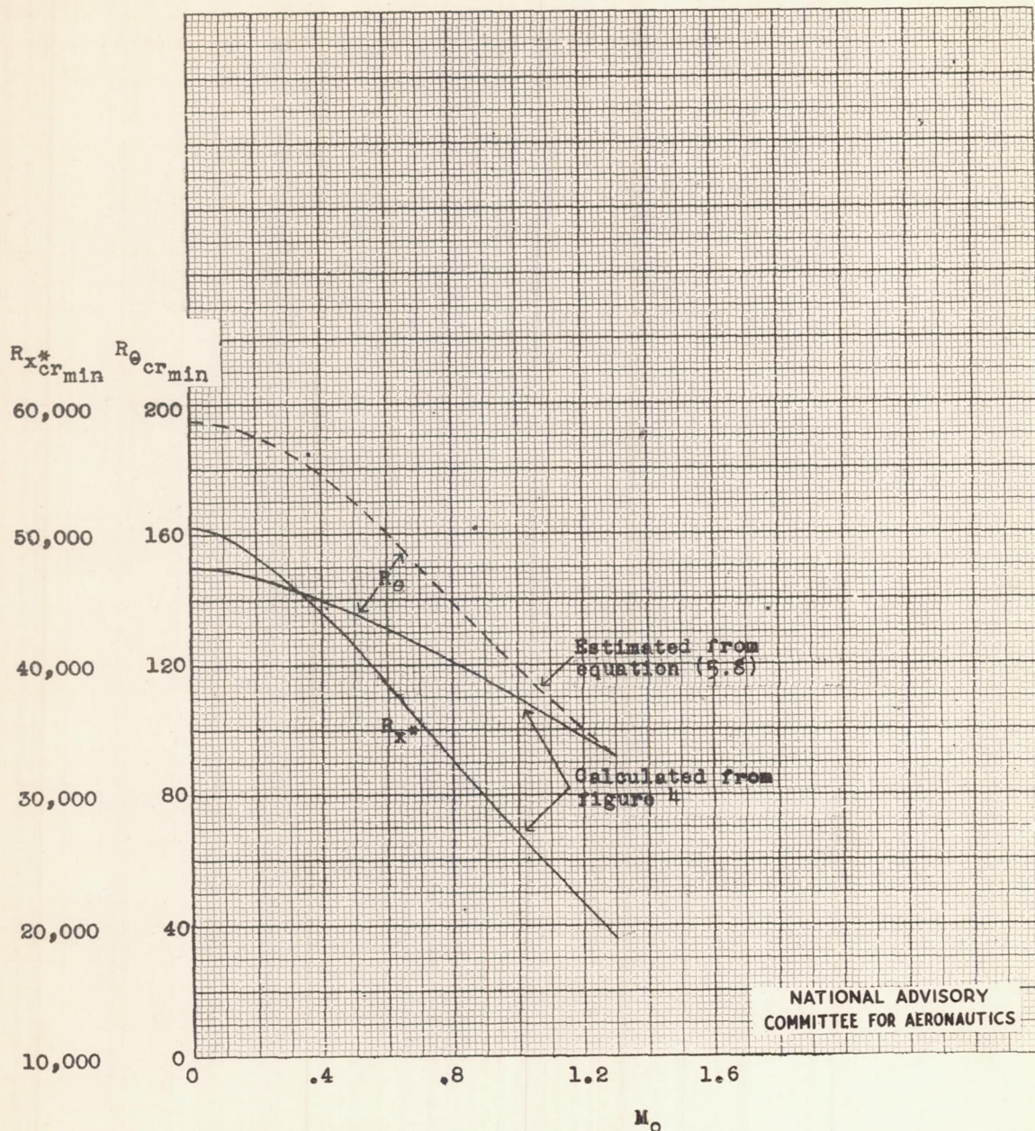
Figure 5.- Variation of minimum critical Reynolds number with Mach number for laminar boundary-layer flow.
