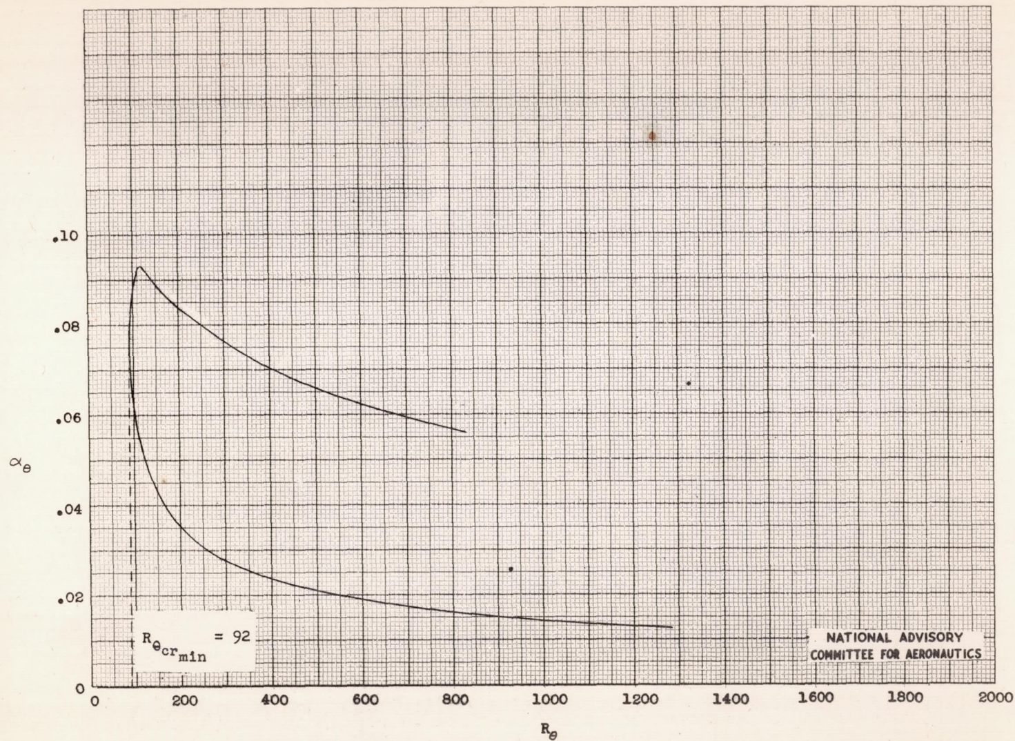
(f) Insulated surface. M_0 = 1.30 . Figure 4.- Continued.
