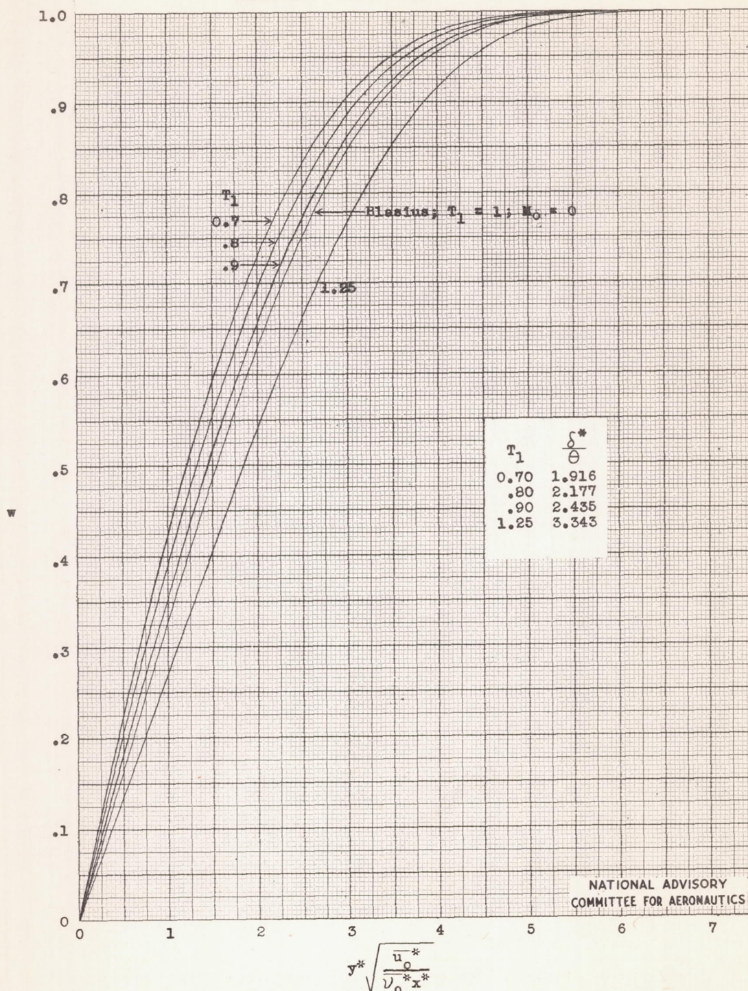
Figure 2.- Boundary-layer velocity profiles for noninsulated surface. M_o = 0.70 . T_1 is the ratio of surface temperature (deg abs.) to free-stream temperature (deg abs.). Inflection more pronounced and farther out into fluid for T_1 = 1.25 than for insulated surface ( T_1 = 1.10 ). No inflection for T_1 = 0.70, 0.80, 0.90 .
