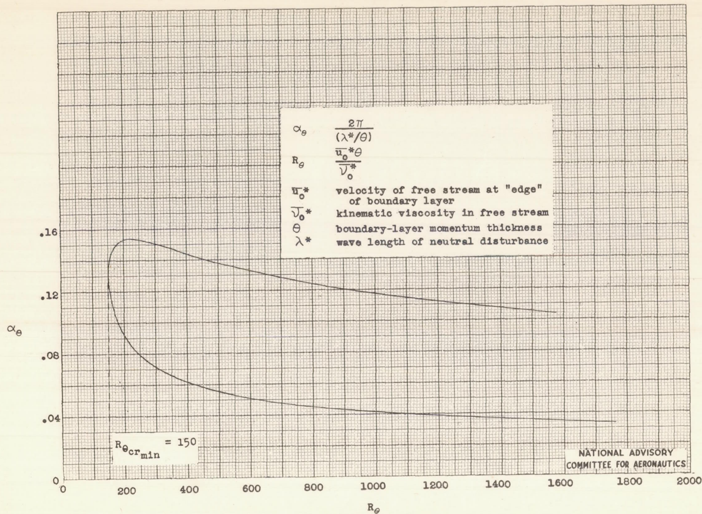
Figure 4.- Wave number \alpha_\theta against Reynolds number R_\theta for neutral stability of laminar boundary-layer flow.
