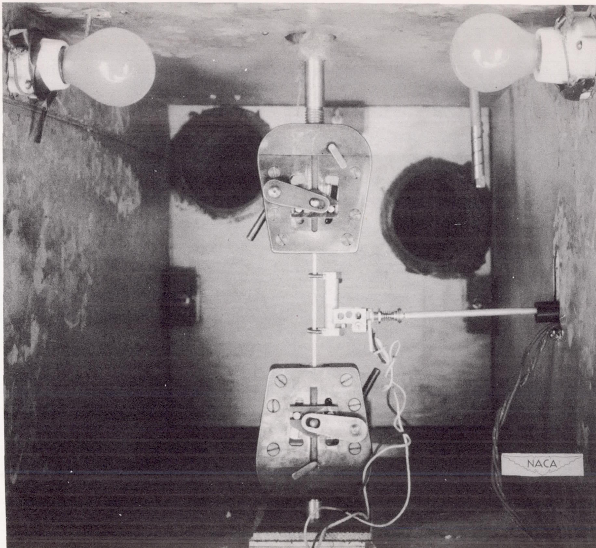
Figure 1.- Interior view of tensile test enclosure with specimen in grips and extensometer attached.
