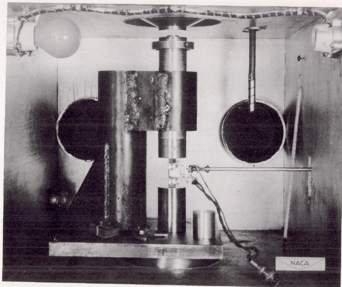
Figure 4.- Interior view of compression test enclosure with specimen in place in compression tool and extensometer attached.
