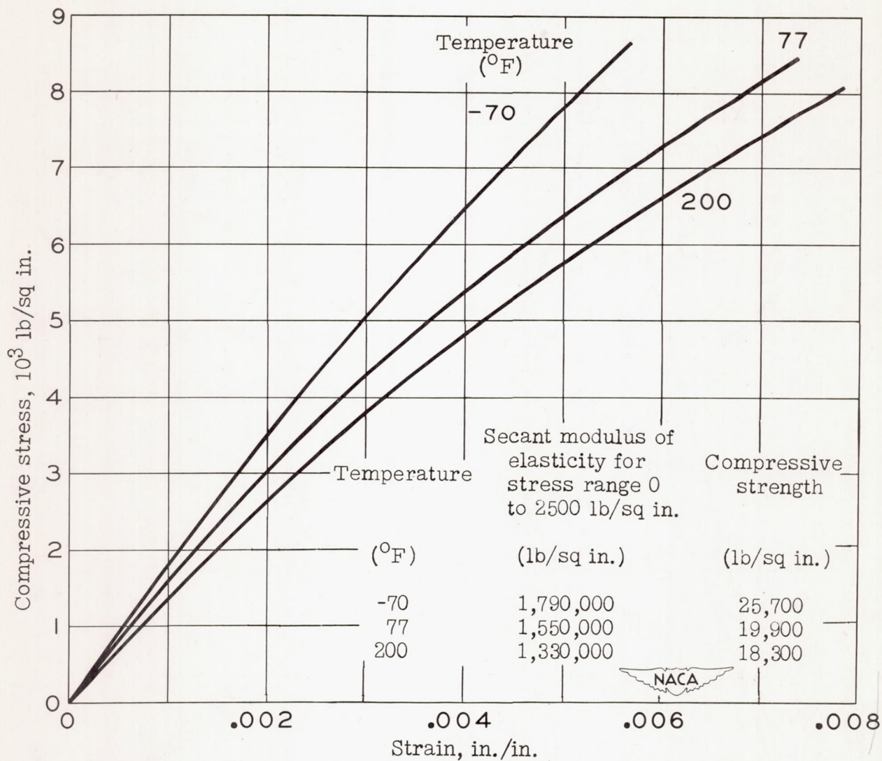
Figure 19.- Compressive stress-strain curves of grade AA asbestos-fabric phenolic laminate K2. Lengthwise specimens.
