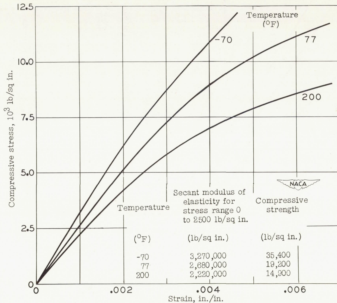
Figure 20.- Compressive stress-strain curves of high-strength-paper phenolic laminate S2. Lengthwise specimens.
