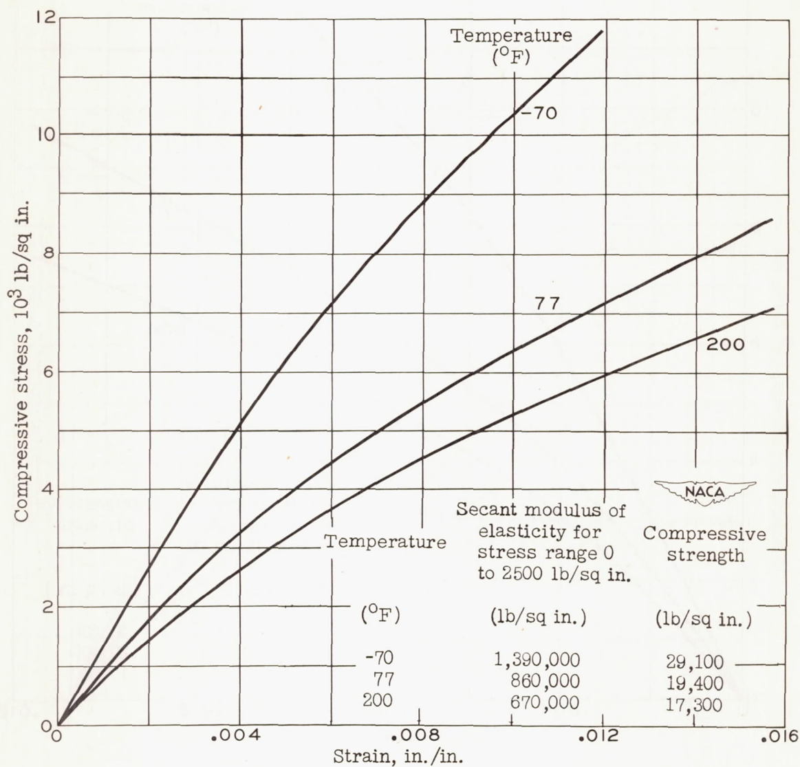
Figure 21.- Compressive stress-strain curves of low-pressure grade C phenolic laminate V2. Lengthwise specimens.
