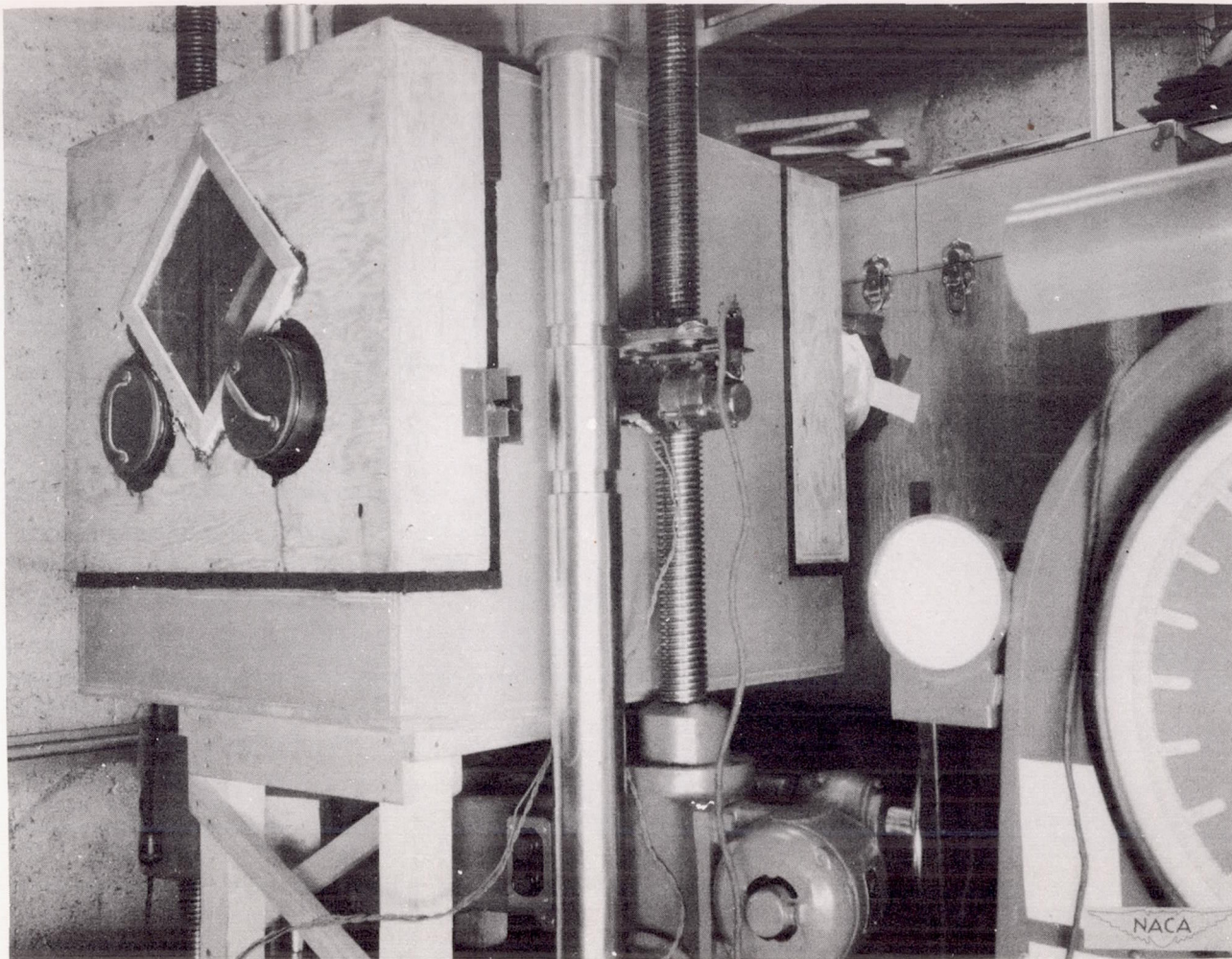
Figure 2.- Front view of tensile test enclosure in place in testing machine.
