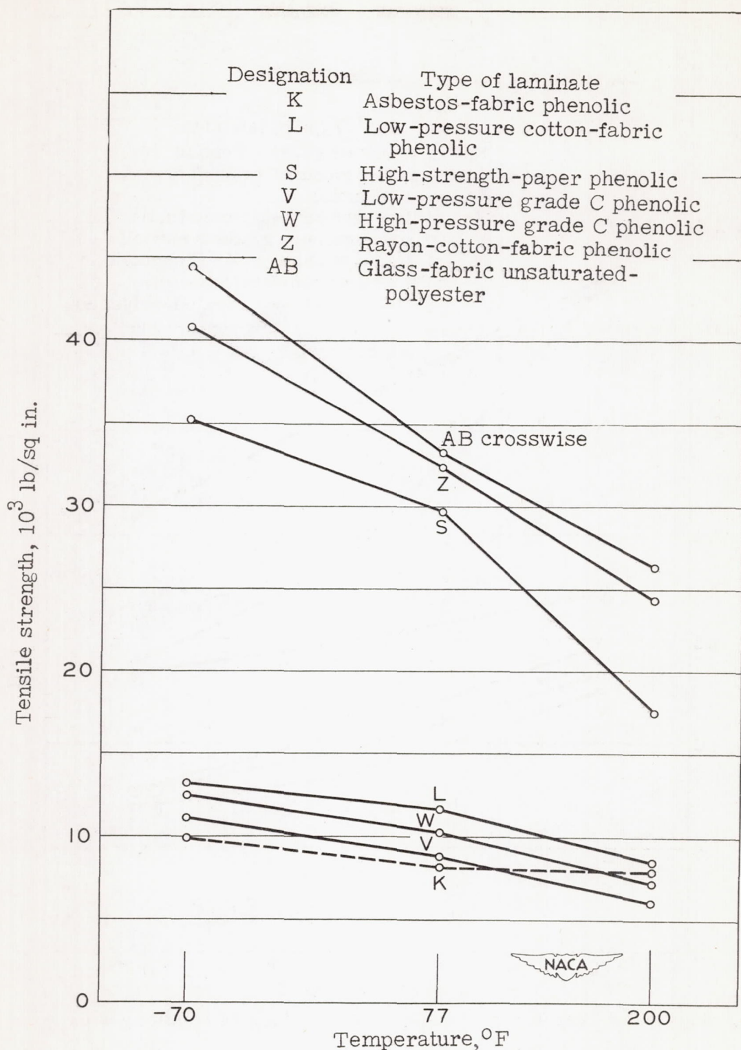
Figure 7.- Variation of tensile strength with temperature for \frac{1}{8} -inch-thick laminates. Lengthwise direction unless noted.
