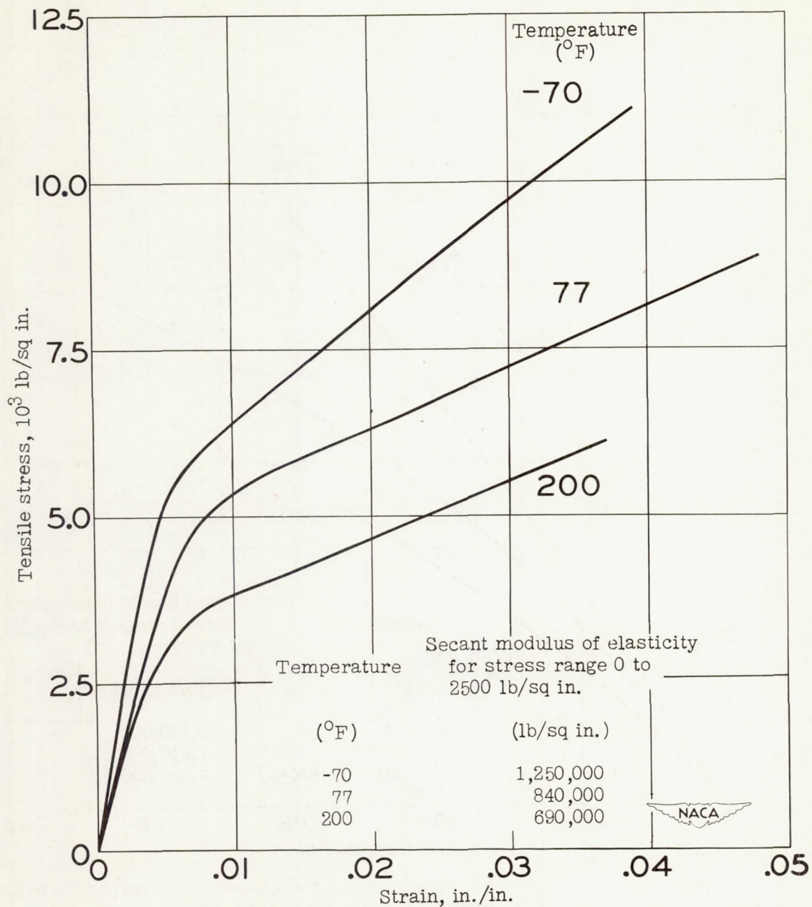
Figure 12.- Tensile stress-strain curves for low-pressure grade C phenolic laminate V1. Lengthwise specimens.
