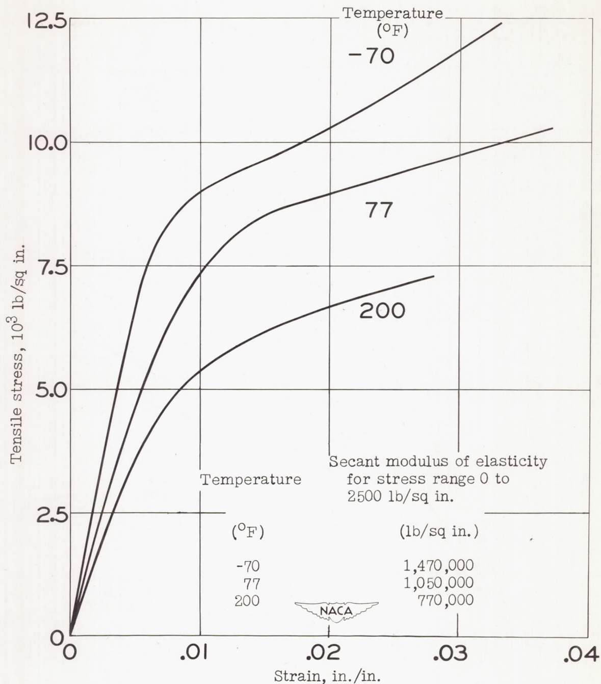
Figure 13.- Tensile stress-strain curves for high-pressure grade C phenolic laminate W1. Lengthwise specimens.
