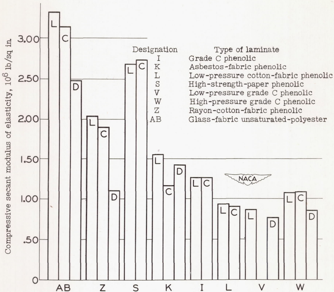
Figure 29.- Compressive secant moduli of elasticity (0 to 2500 lb/sq in.) for lengthwise, crosswise, and 45^\circ diagonal directions of \frac{1}{2} -inch-thick laminates at 77^\circ F.
