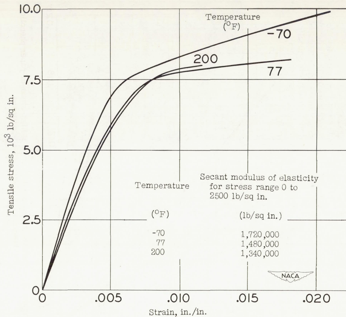
Figure 10.- Tensile stress-strain curves for grade AA asbestos-fabric phenolic laminate K1. Lengthwise specimens.
