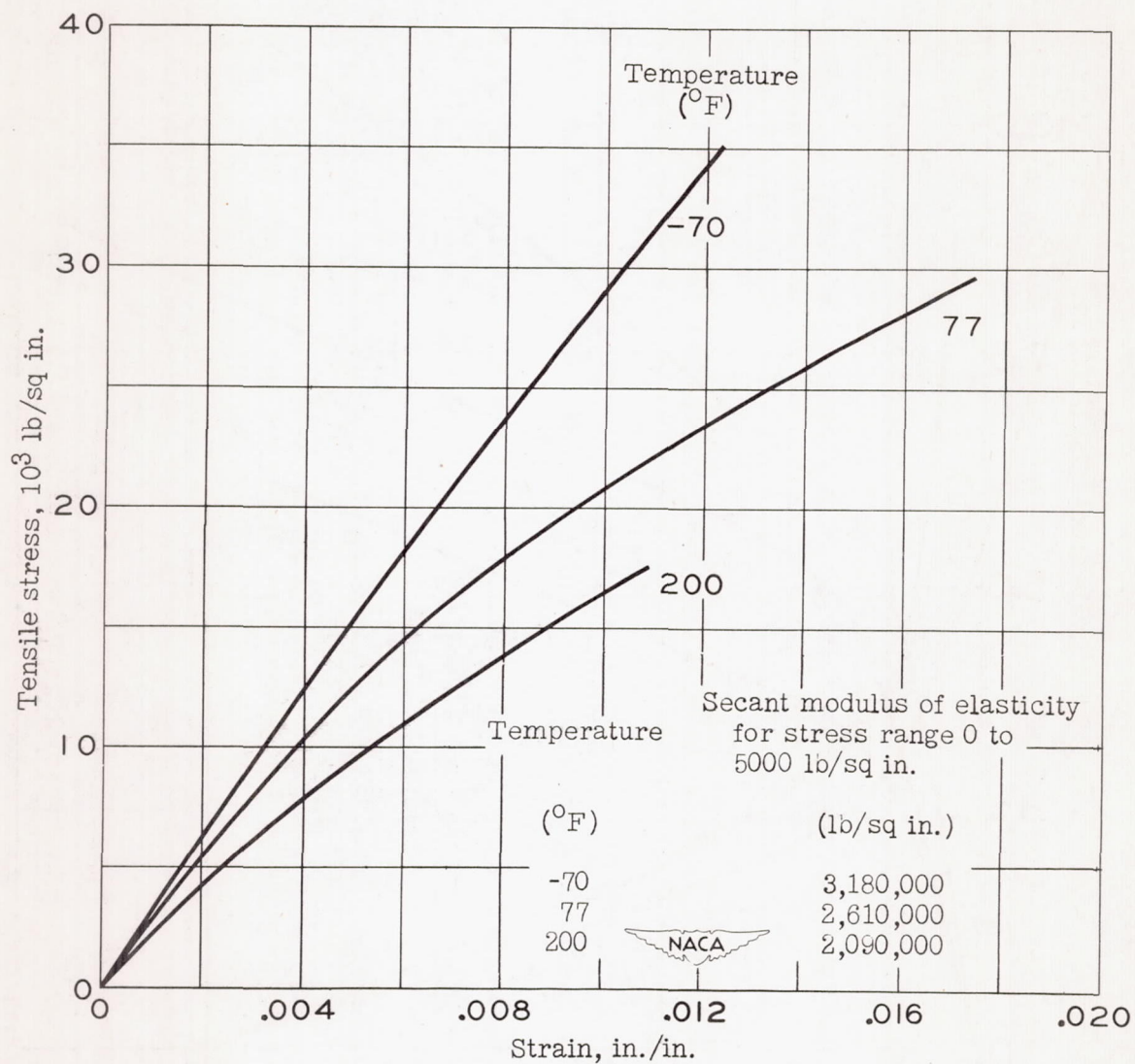
Figure 11.- Tensile stress-strain curves of high-strength-paper phenolic laminate S1. Lengthwise specimens.
