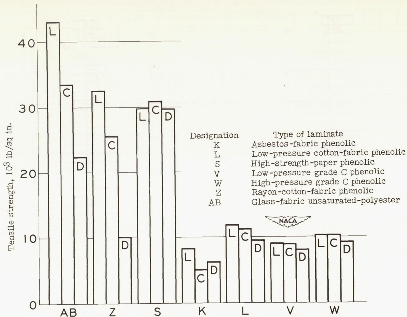
Figure 26.- Tensile strengths for lengthwise, crosswise, and 45° diagonal directions of \frac{1}{8} -inch-thick laminates.
