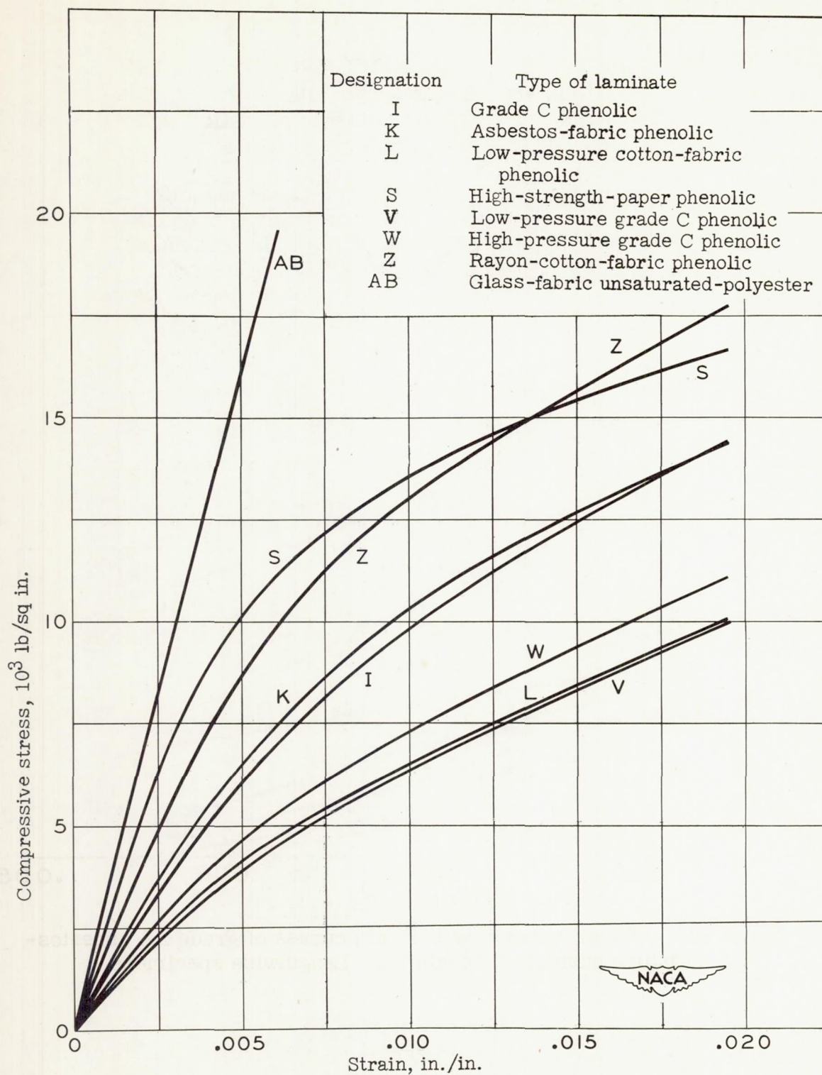
Figure 18.- Compressive stress-strain curves of plastic laminates at 77° F. Lengthwise direction.
