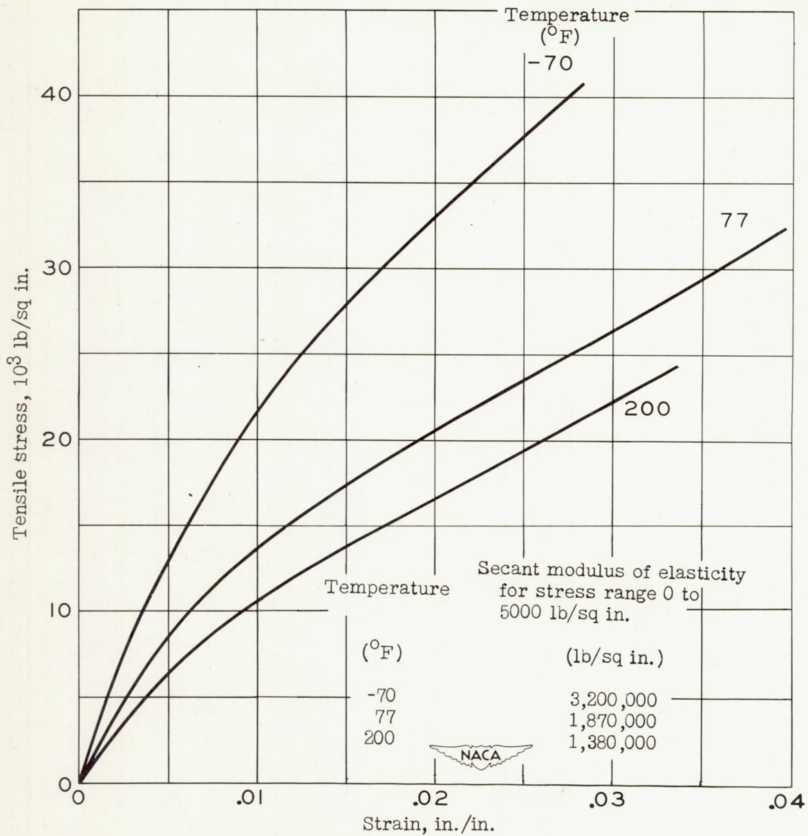
Figure 14.- Tensile stress-strain curves for rayon-cotton-fabric phenolic laminate Z1. Lengthwise specimens.
