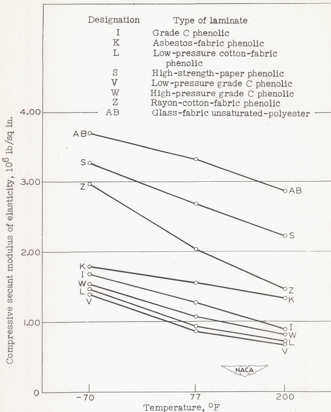
Figure 17.- Variation of compressive secant modulus of elasticity (0 to 2500 lb/sq in.) with temperature for \frac{1}{2} -inch-thick laminates.
