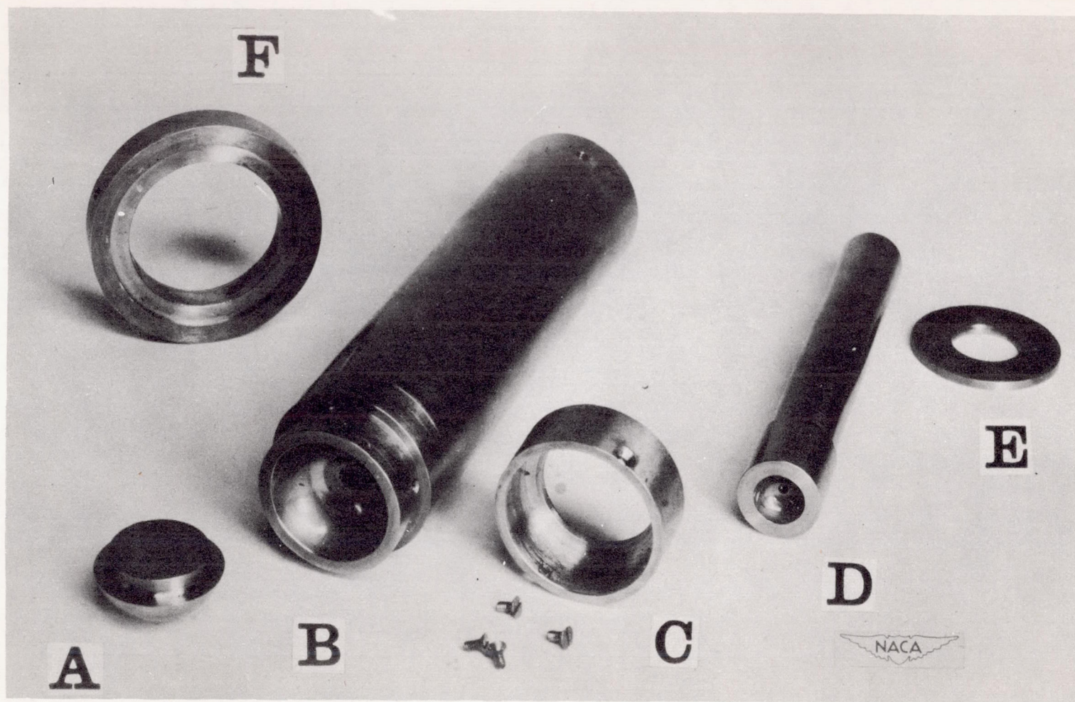
Figure 6.- Disassembled compression tool plunger. A, spherically seated bearing block; B, plunger (ball through which load is transmitted from rod D to plunger is inside latter); C, retainer for bearing block; D, loading rod; E, centering washer for rod D; F, limit collar for plunger.
