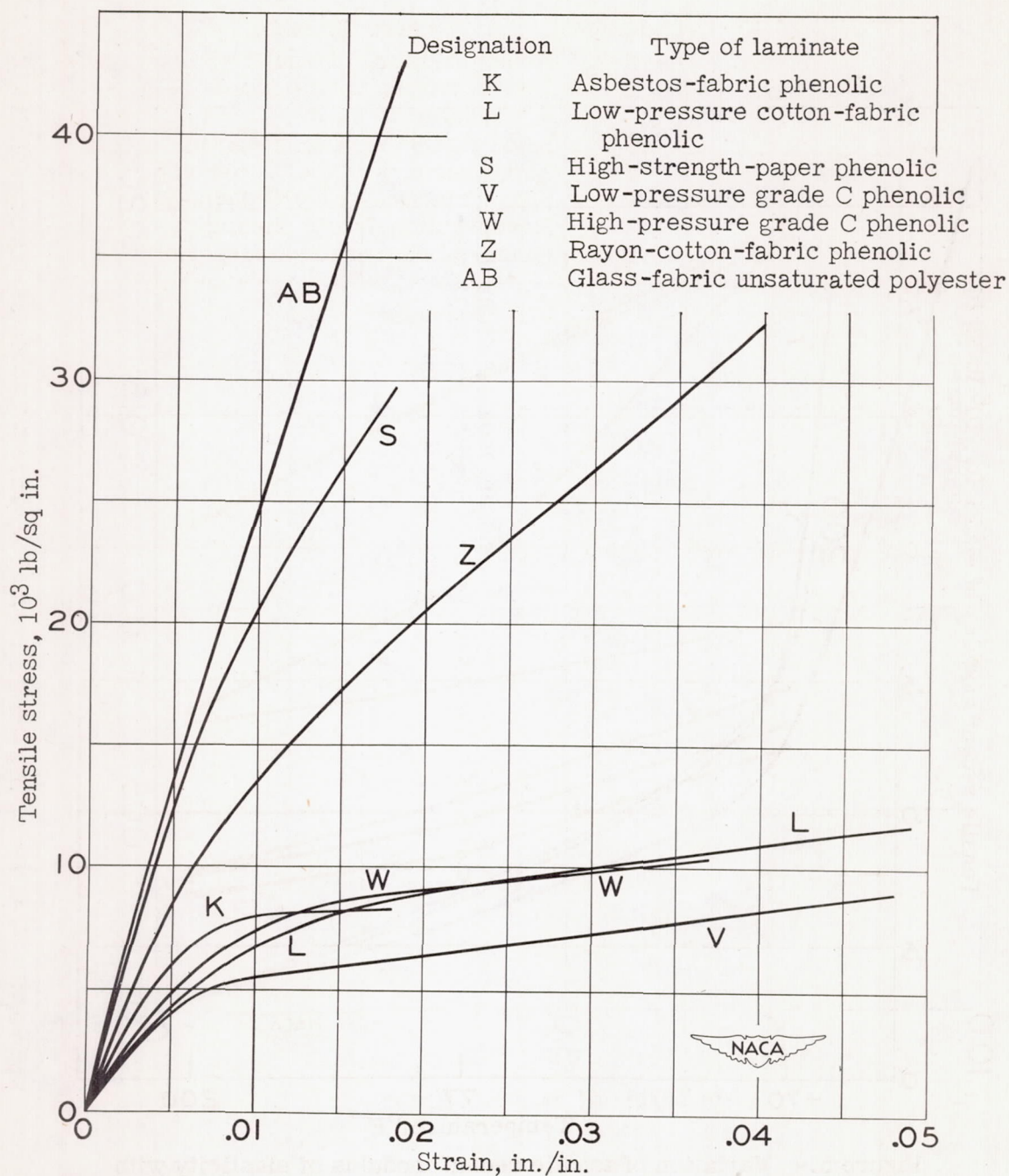
Figure 9.- Tensile stress-strain curves of plastic laminates at 77° F. Lengthwise direction.
