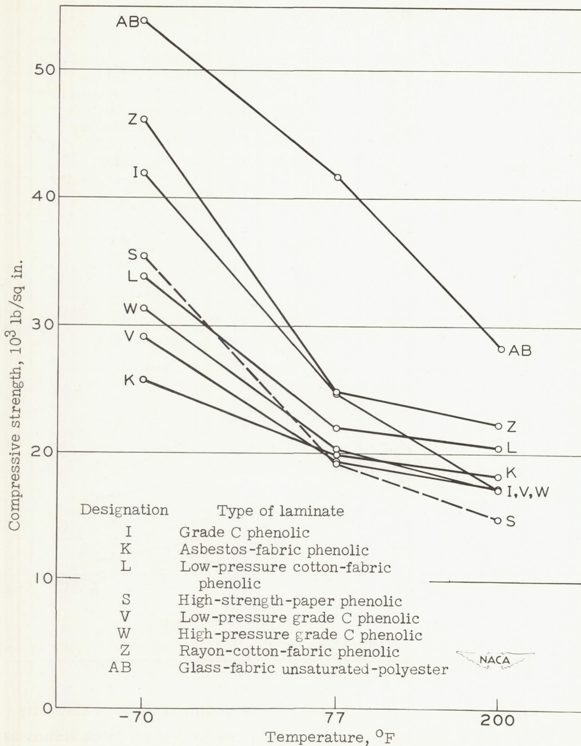
Figure 16.- Variation of compressive strength with temperature for \frac{1}{2} -inch-thick laminates.
