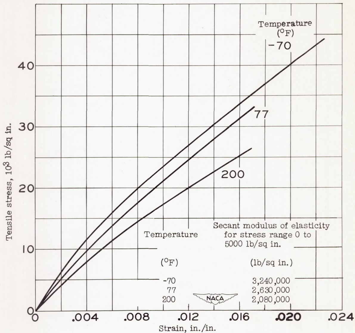
Figure 15.- Tensile stress-strain curves for glass-fabric unsaturated-polyester laminate AB1. Crosswise specimens.
