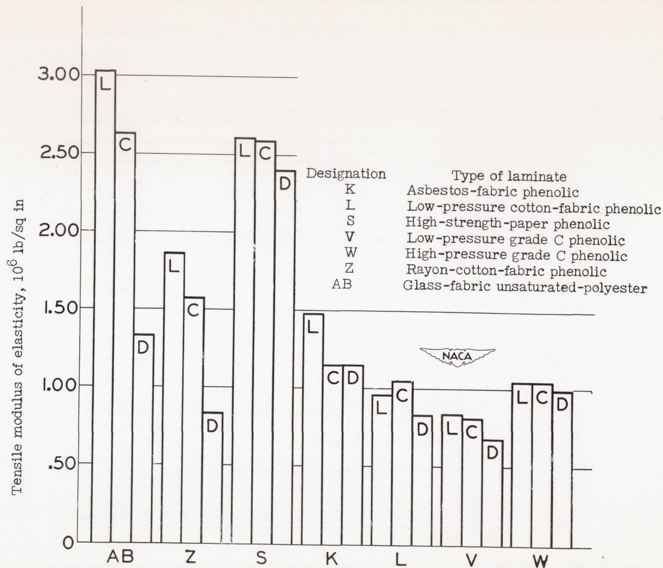
Figure 27.- Tensile secant moduli of elasticity for lengthwise, crosswise, and 45° diagonal directions of \frac{1}{8} -inch-thick laminates at 77° F. Stress ranges: 0 to 5000 pounds per square inch for AB, Z, and S; 0 to 2500 pounds per square inch for K, L, V, and W.
