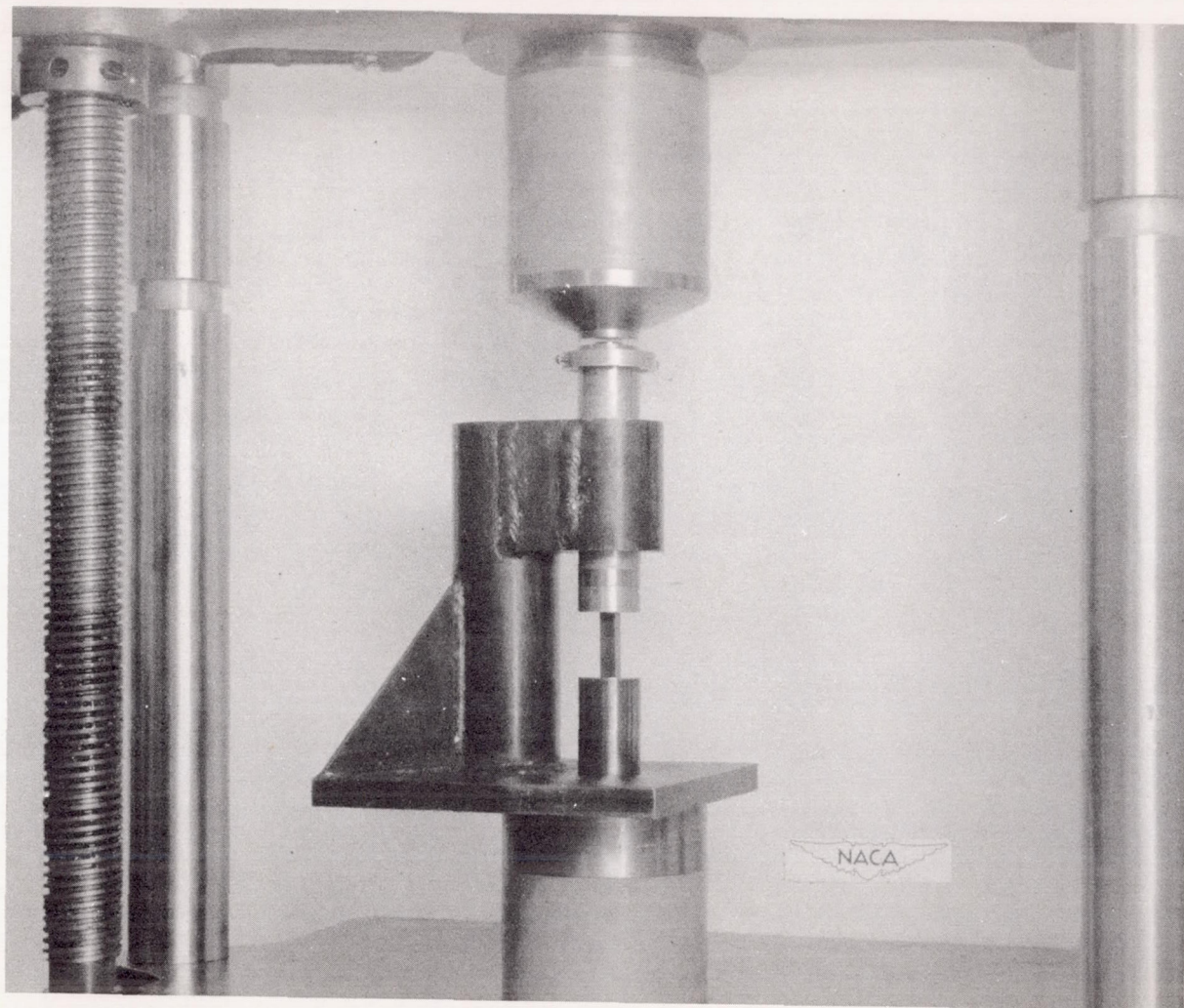
Figure 5.- Compression tool in place with insulated support and loading blocks.
