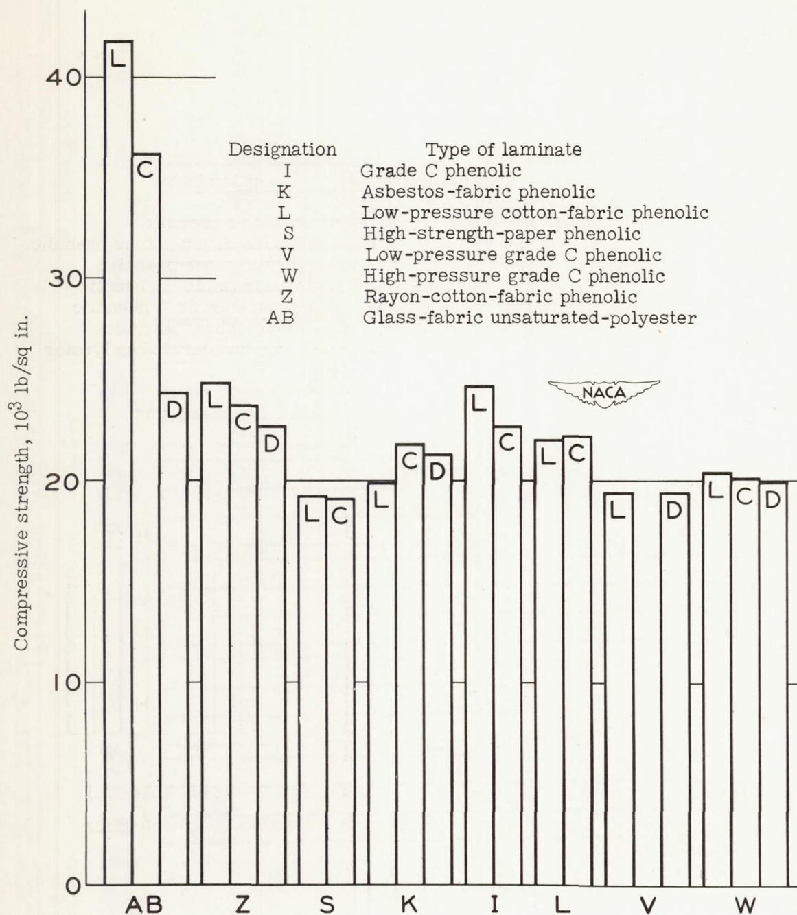
Figure 28.- Compressive strengths for lengthwise, crosswise, and 45^\circ diagonal directions of \frac{1}{2} -inch-thick laminates at 77^\circ F.
