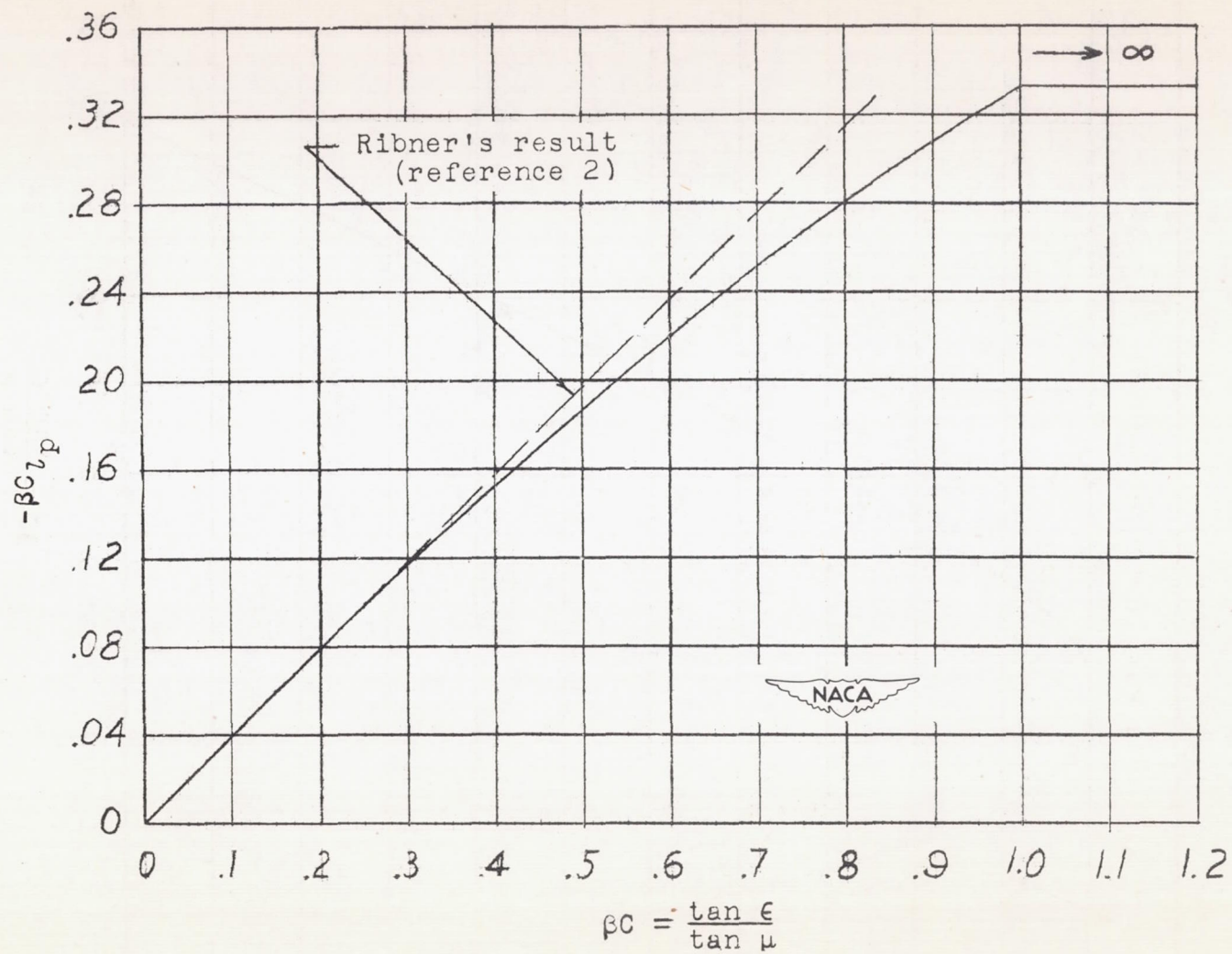
Figure 3.- Stability derivative C_{l_p} for triangular wings.
