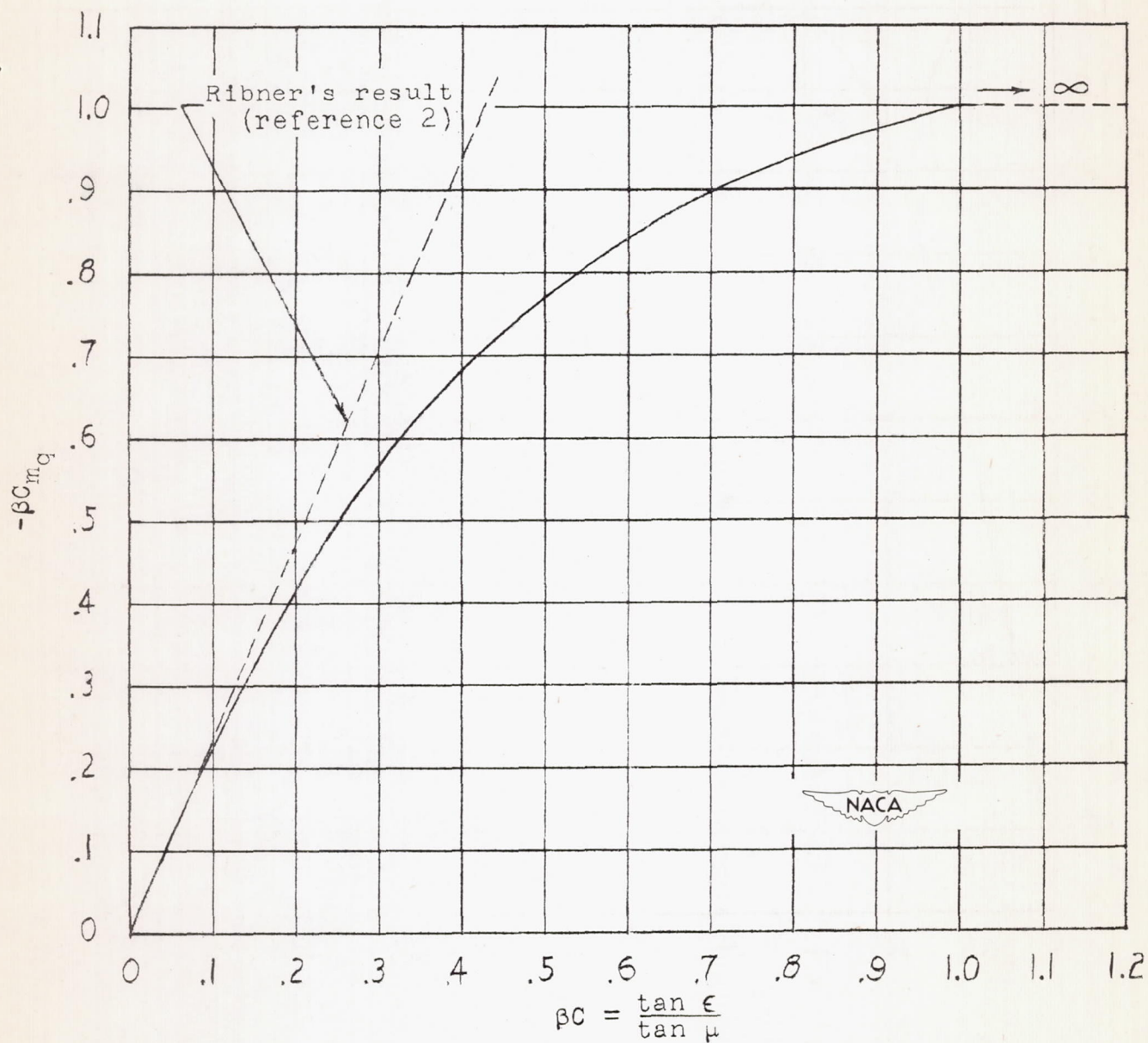
Figure 5.- Stability derivative C_{mq} about the \frac{2}{3}c point for triangular wings.
